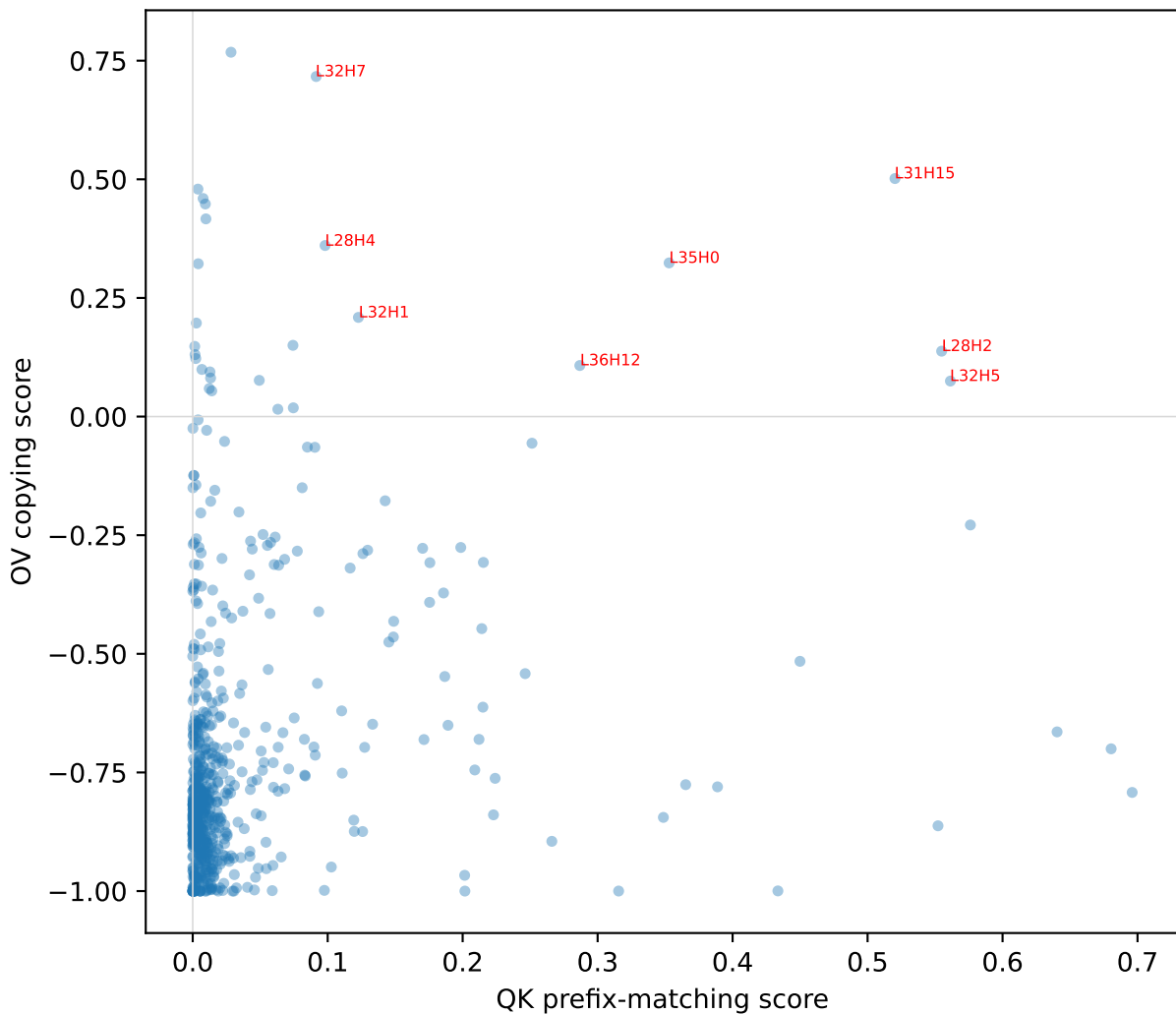
Gemma: QK vs OV per head (true induction heads = top-right: high on both)
