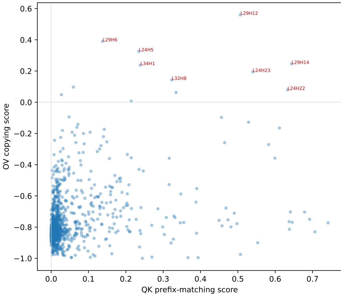
Qwen: QK vs OV per head (true induction heads = top-right: high on both)
