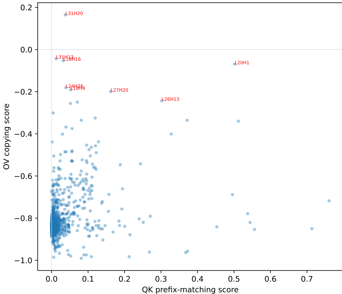
Llama: QK vs OV per head (true induction heads = top-right: high on both)
