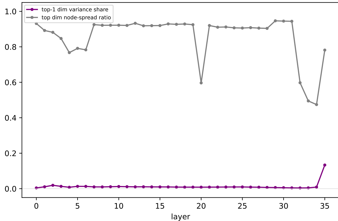
Qwen/square_grid: outlier dim — dominance & whether it codes node identity
