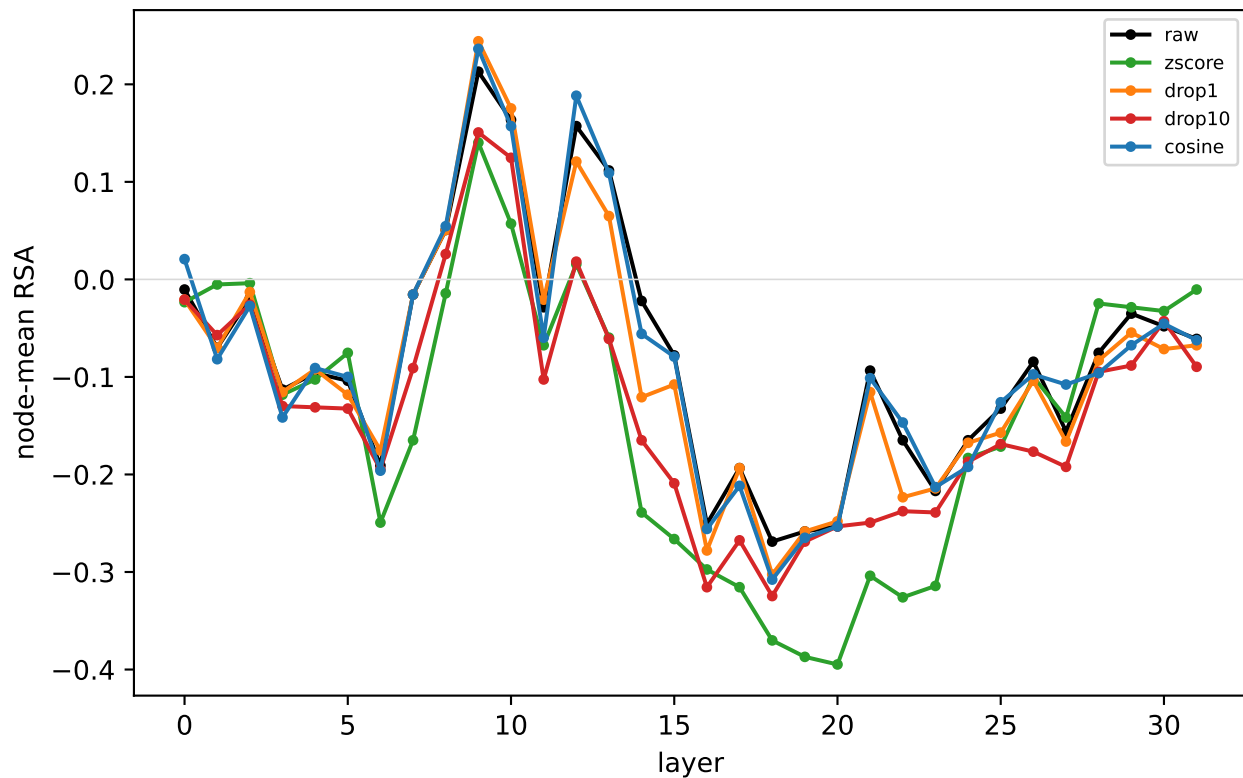
Llama/days: RSA by metric
