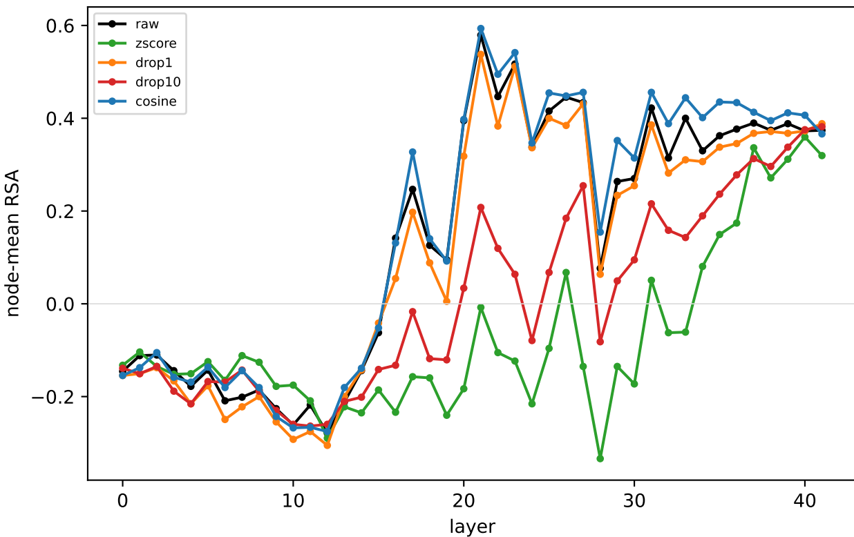
Gemma/days: RSA by metric
