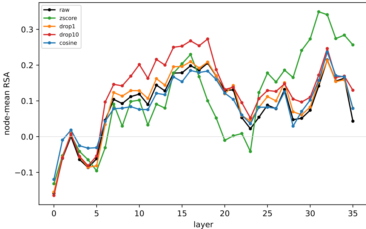
Qwen/square_grid: RSA by metric
