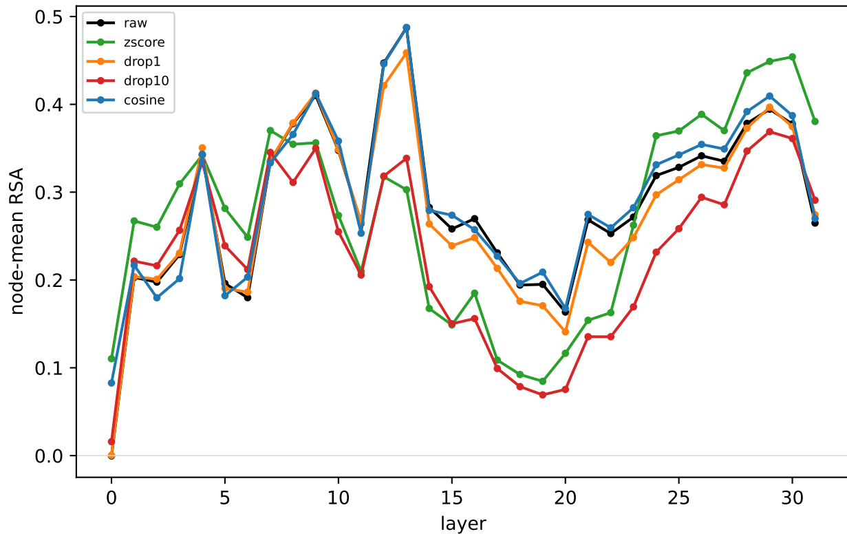
Llama/square_grid: RSA by metric
