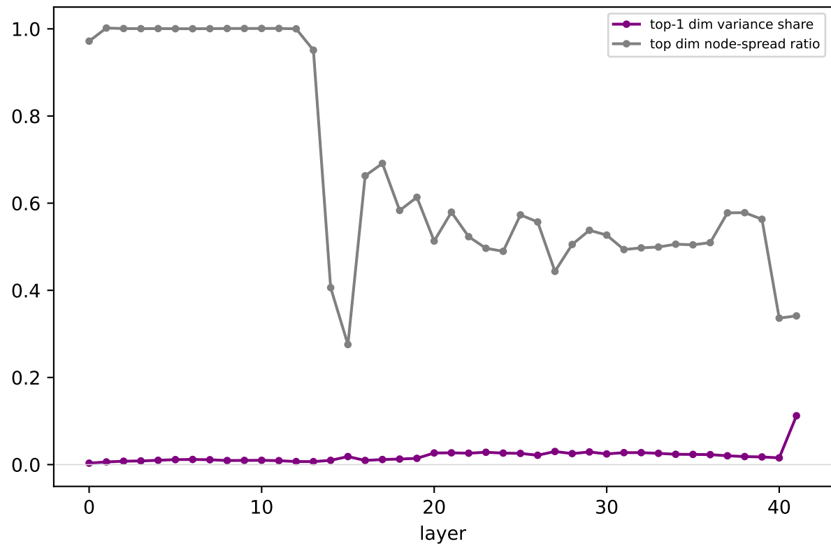
Gemma/days: outlier dim — dominance & whether it codes node identity
