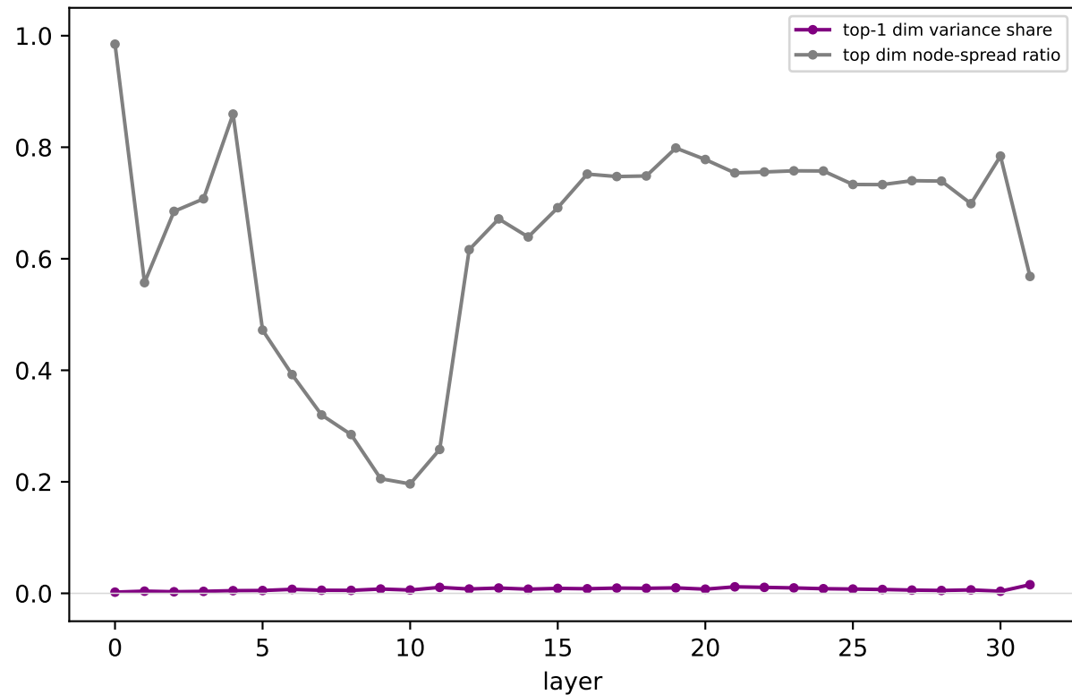
Llama/square_grid: outlier dim — dominance & whether it codes node identity
