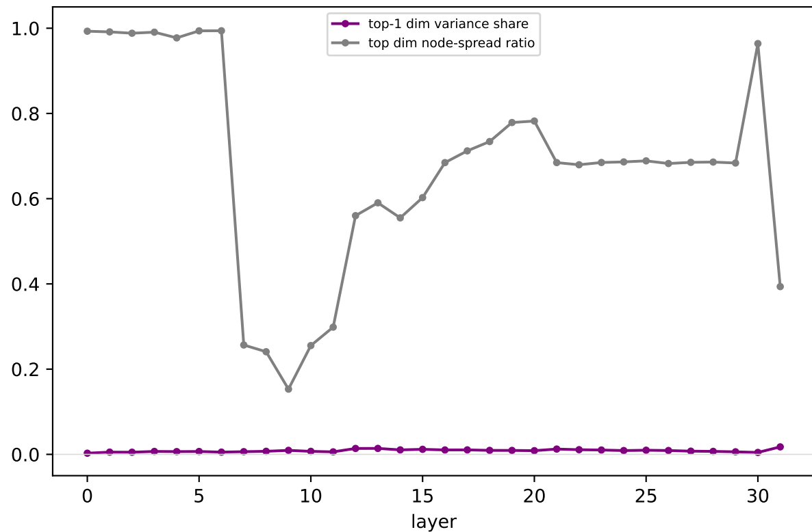
Llama/days: outlier dim — dominance & whether it codes node identity
