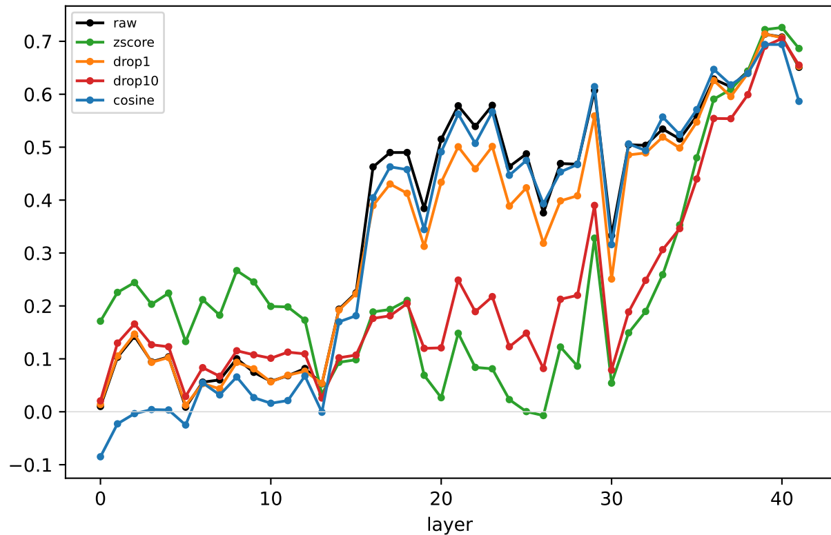
Gemma/square_grid: RSA by metric
