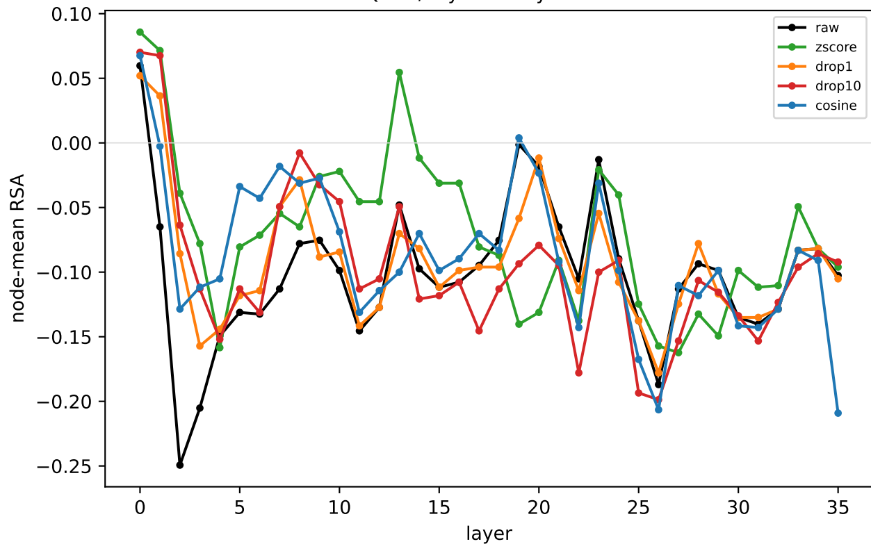
Qwen/days: RSA by metric
