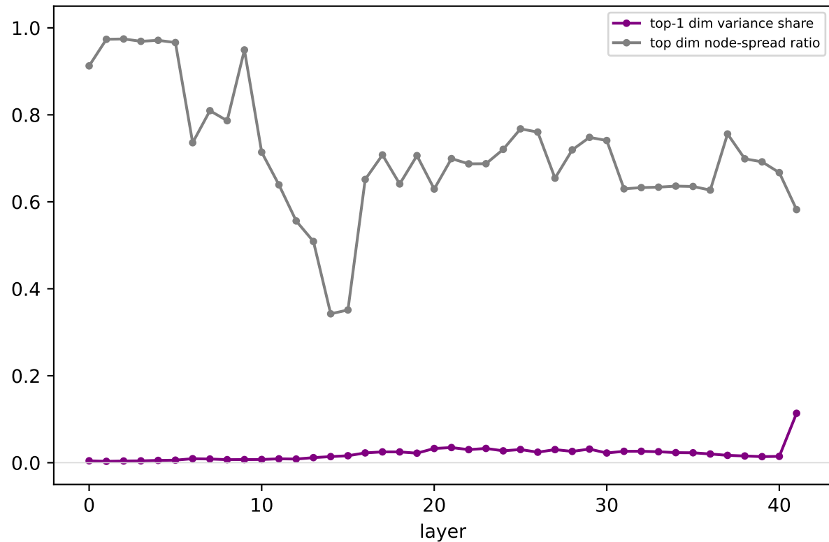
Gemma/square_grid: outlier dim — dominance & whether it codes node identity
