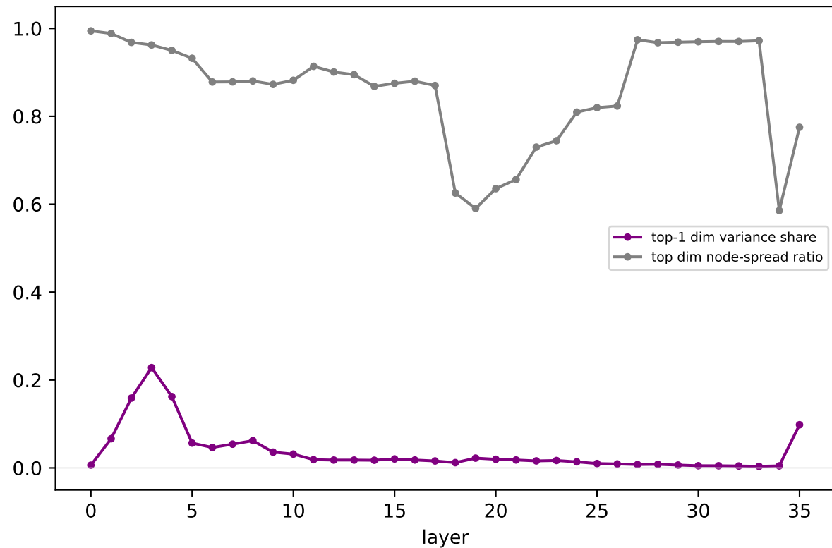
Qwen/days: outlier dim — dominance & whether it codes node identity
