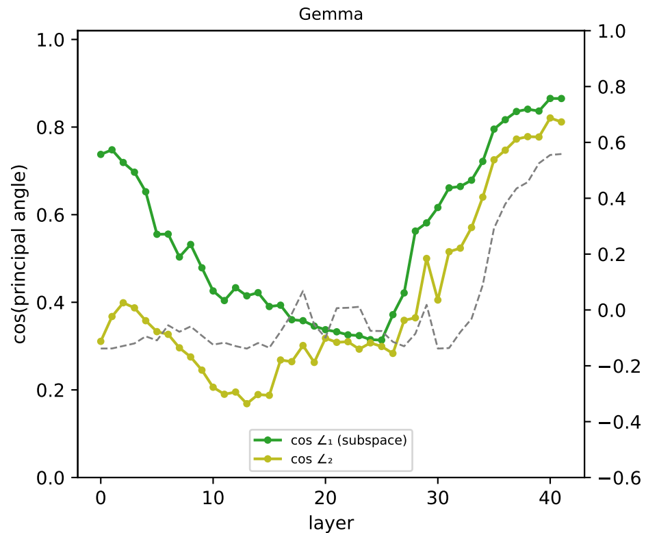
[hex] RSA best-2D subspace vs coord-probe readout subspace — cos of principal angles (1 = identical 2-D subspace)
