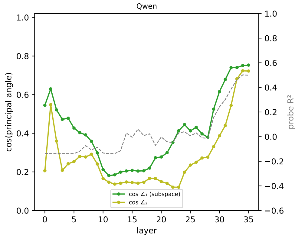
[hex] RSA best-2D subspace vs coord-probe readout subspace — cos of principal angles (1 = identical 2-D subspace)
