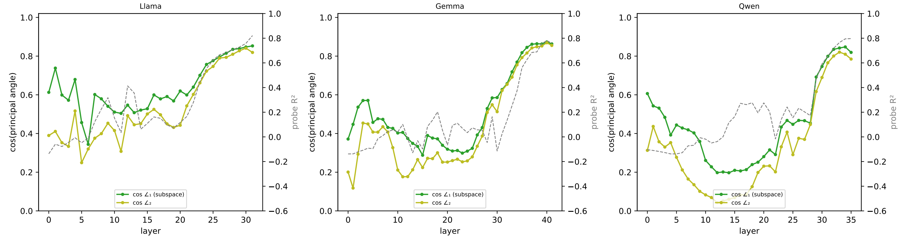
[ring] RSA best-2D subspace vs coord-probe readout subspace — cos of principal angles (1 = identical 2-D subspace)
