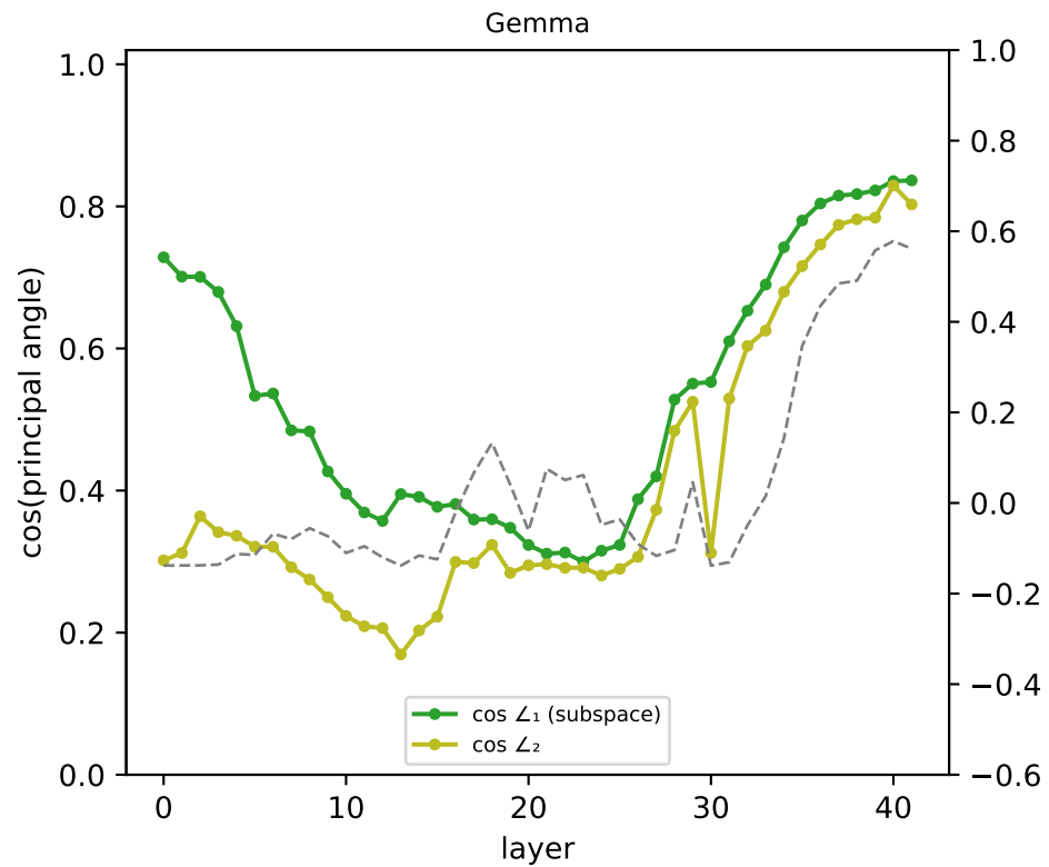
[square_grid] RSA best-2D subspace vs coord-probe readout subspace — cos of principal angles (1 = identical 2-D subspace)
