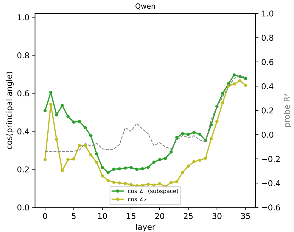
[square_grid] RSA best-2D subspace vs coord-probe readout subspace — cos of principal angles (1 = identical 2-D subspace)
