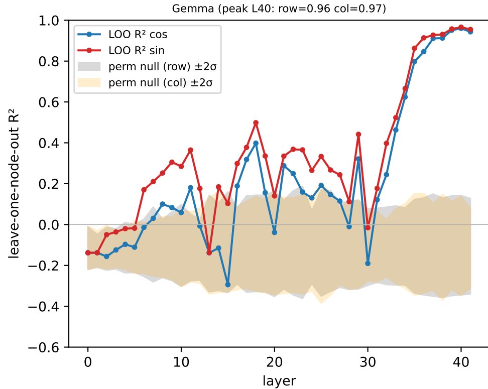
[ring] leave-one-node-out linear decodability of grid coordinates per layer
