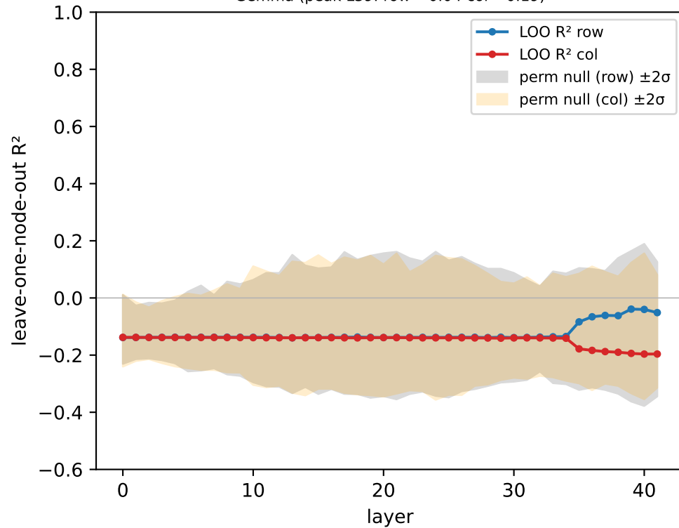
Gemma (peak L39: row=-0.04 col=-0.19)
