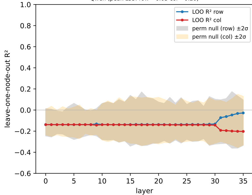
Qwen (peak L35: row=-0.03 col=-0.20)
