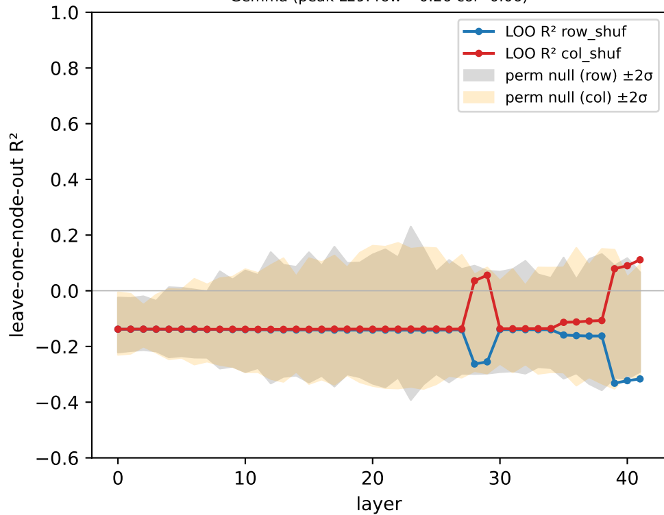
Gemma (peak L29: row=-0.26 col=0.06)
