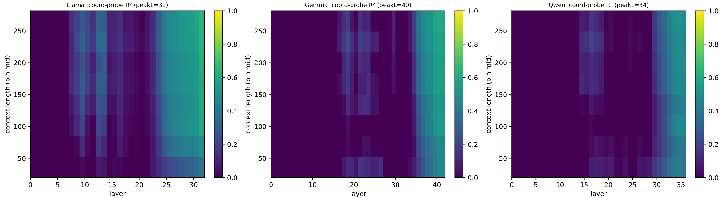
coord-probe R 2 vs (context length x layer) — where/when the map crystallizes
