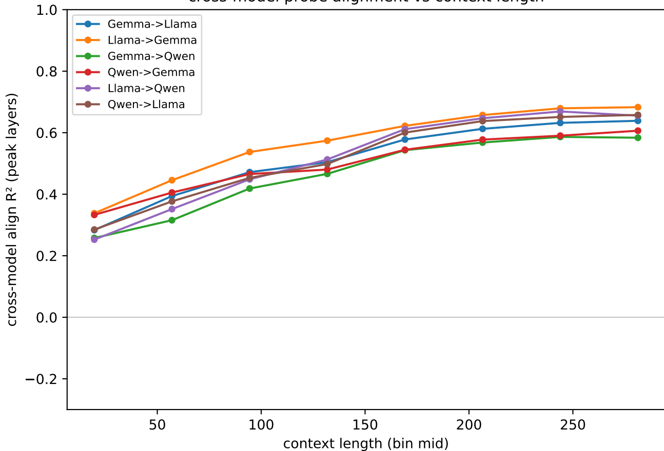
cross-model probe alignment vs context length
