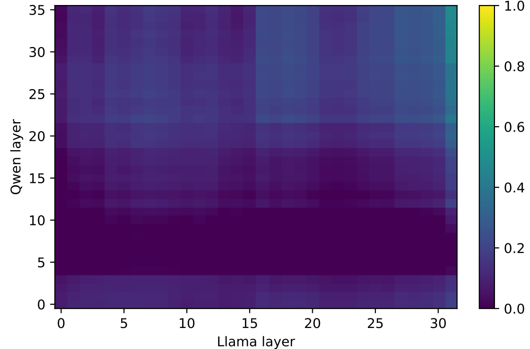
predict Llama from Qwen (max 0.47)
