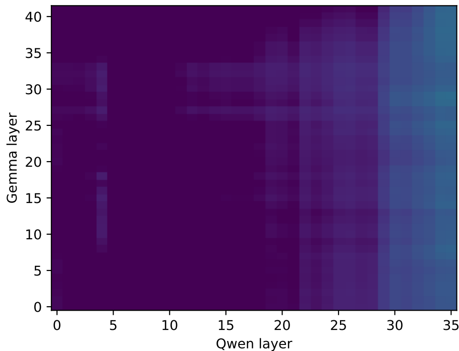
predict Qwen from Gemma (max 0.35)
