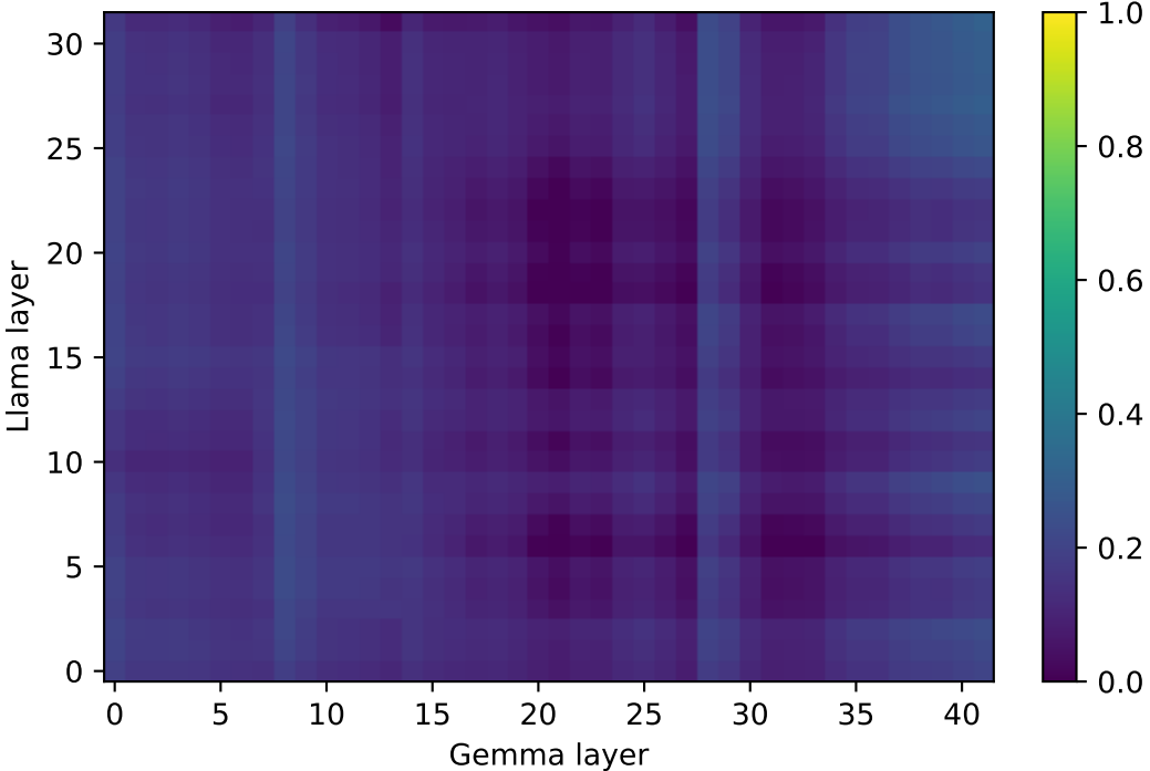
predict Gemma from Llama (max 0.31)
