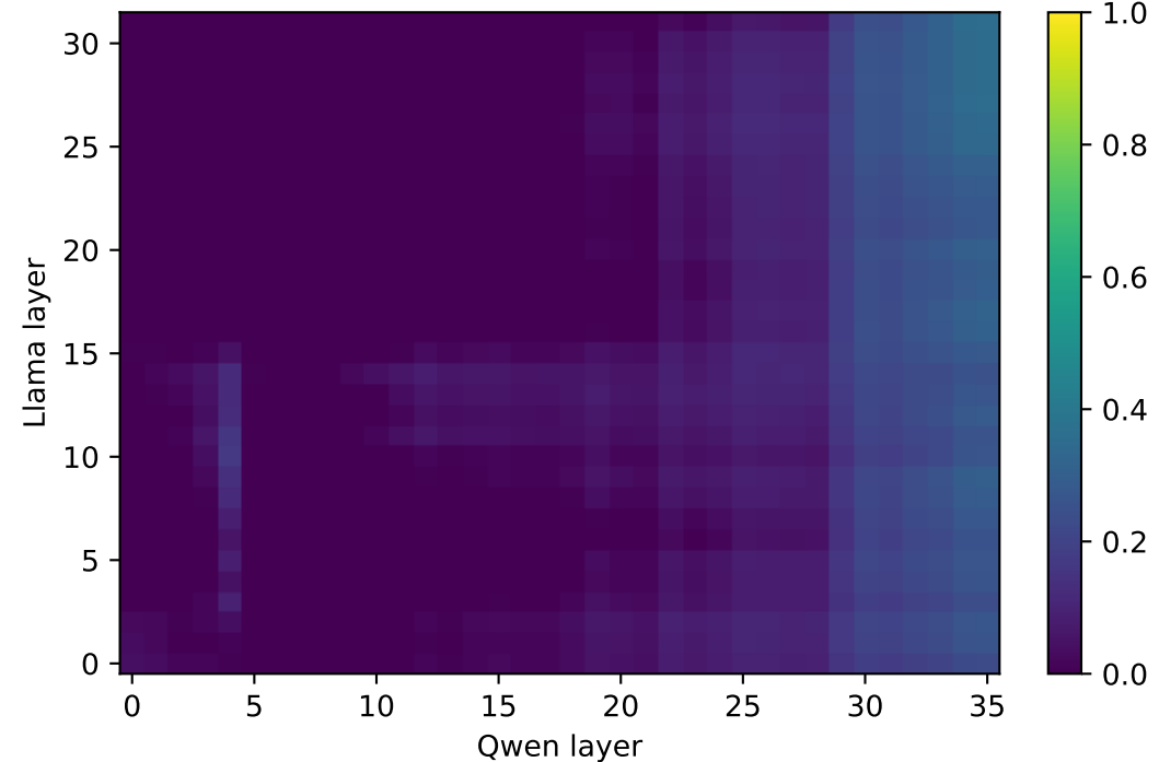
predict Qwen from Llama (max 0.36)
