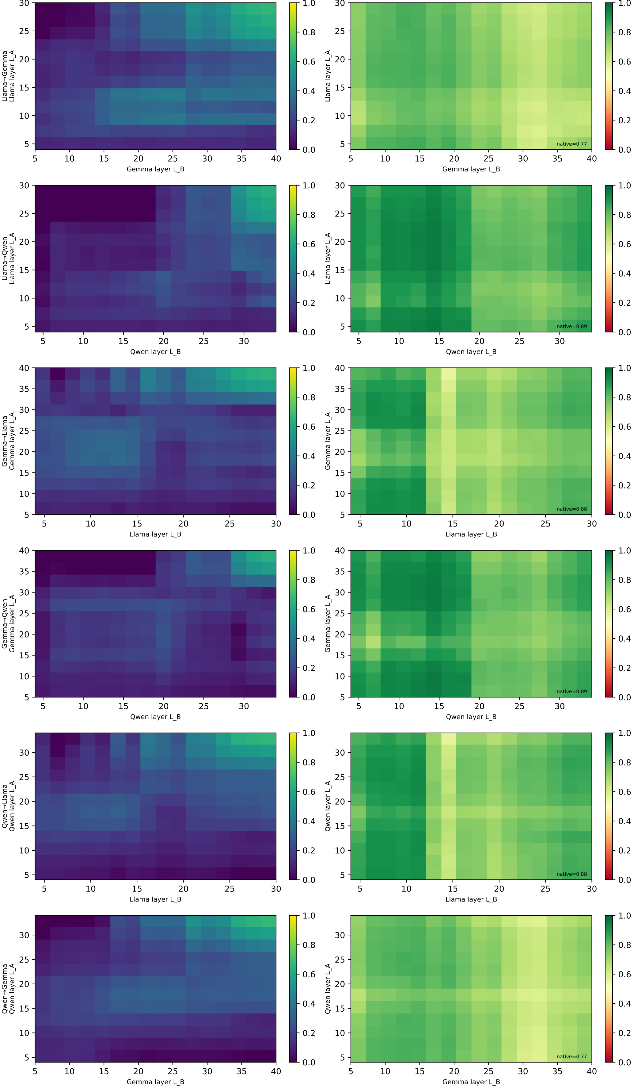
[ring] injection spreadsheet — 6 model pairs × (alignment R 2 | injected behaviour) over L A × L B
