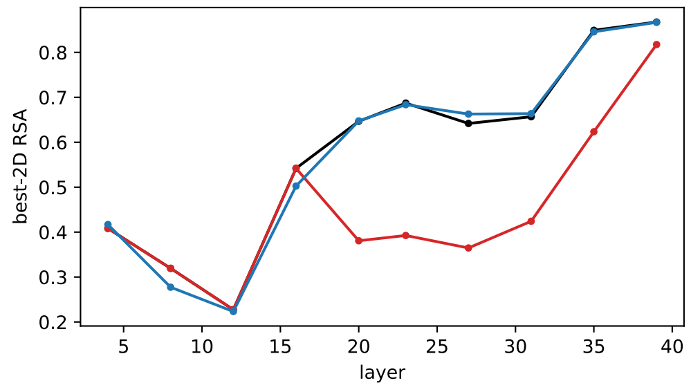
Qwen PROBED best-2D RSA (supervised)
