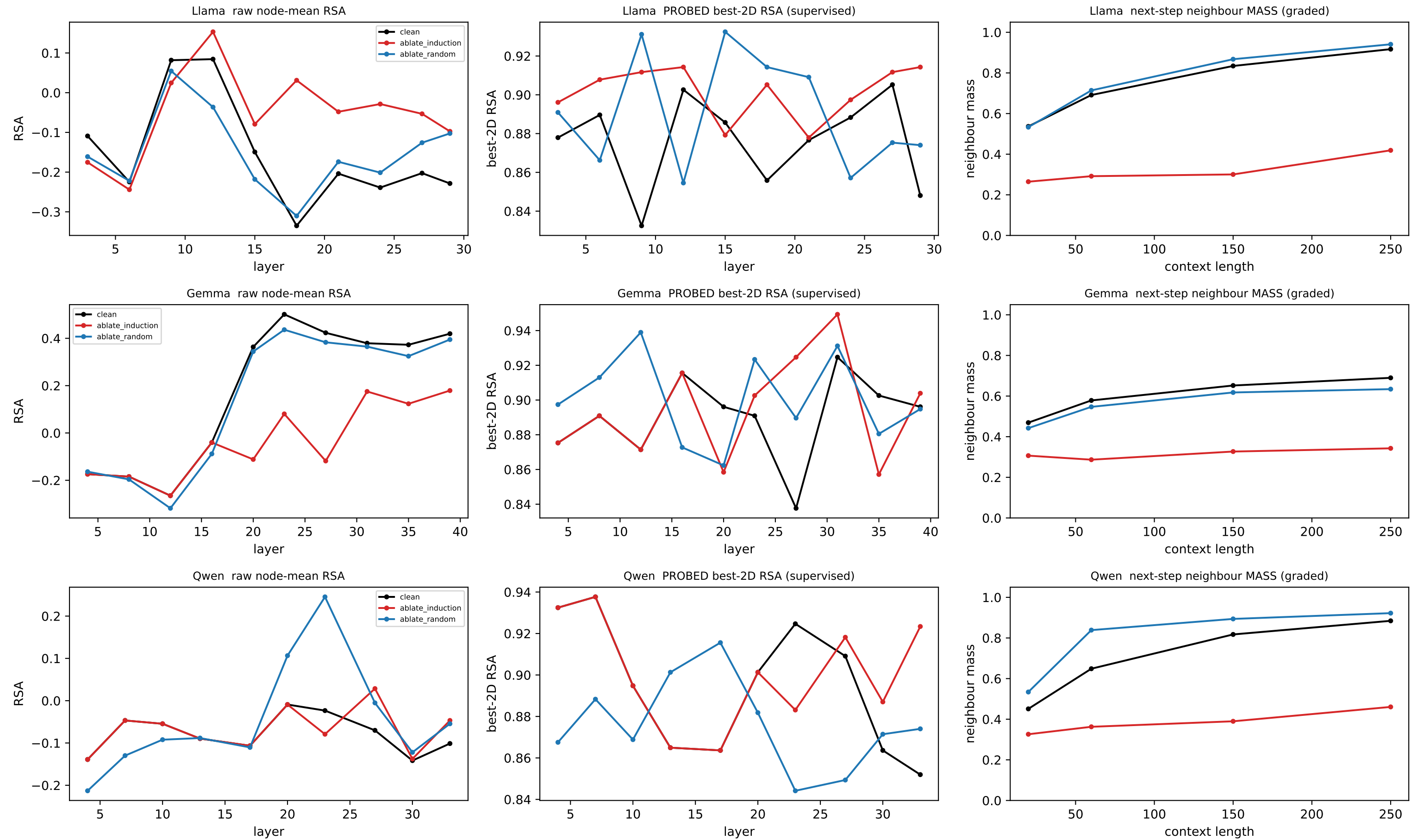
Induction-head ablation [days]: raw geometry | PROBED best-2D geometry | behaviour black = clean, red = ablate induction heads, blue = ablate random heads
