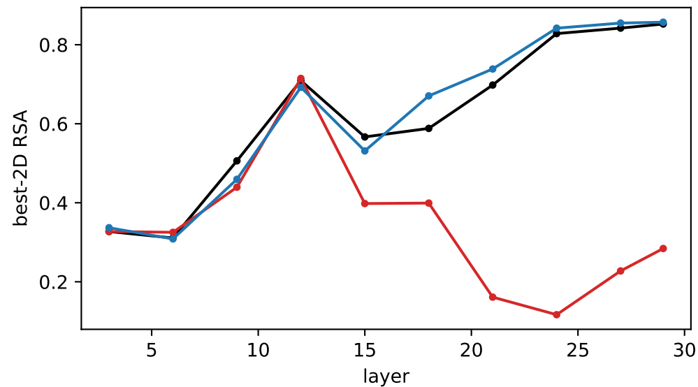
Gemma PROBED best-2D RSA (supervised)
