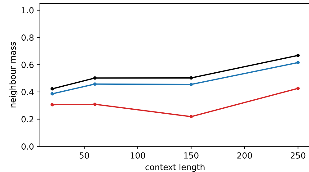
Qwen next-step neighbour MASS (graded)
