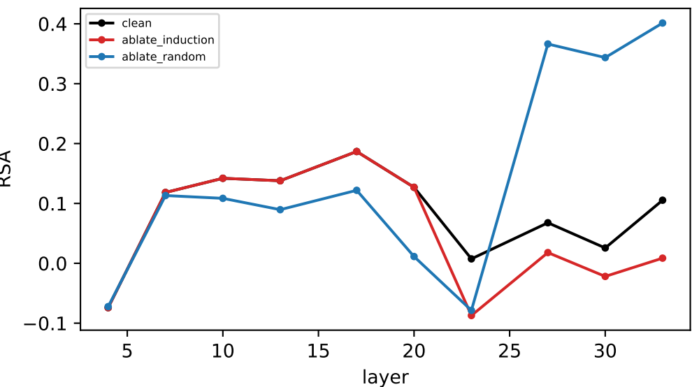
Qwen raw node-mean RSA
