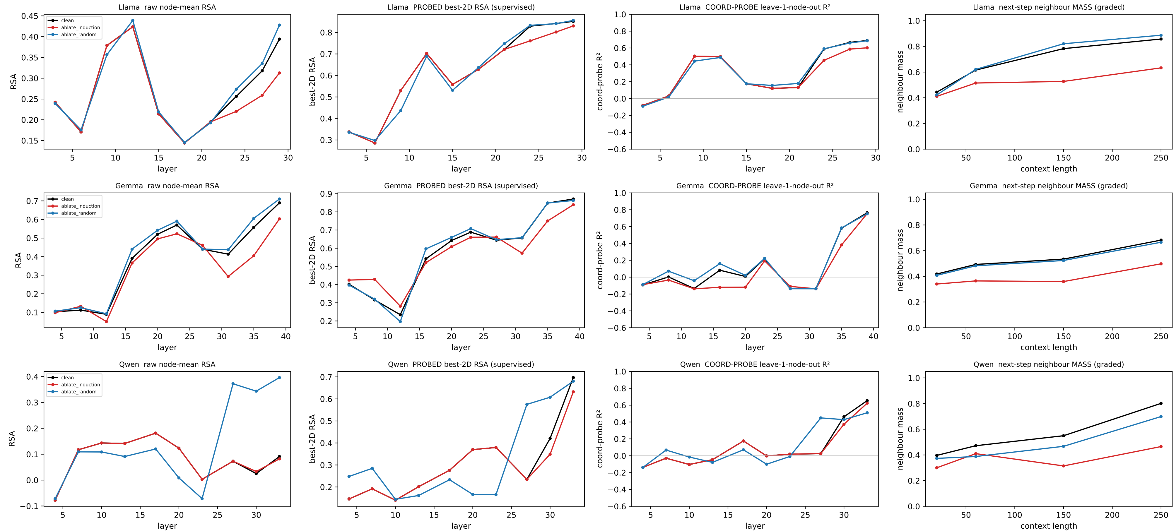
Induction-head ablation [square_grid]: raw geometry | PROBED best-2D geometry | COORD-PROBE R 2 | behaviour black = clean, red = ablate induction heads, blue = ablate random heads
