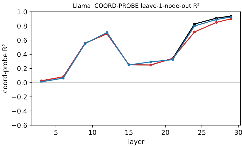
Induction-head ablation [ring]: raw geometry | PROBED best-2D geometry | COORD-PROBE R 2 | behaviour black = clean, red = ablate induction heads, blue = ablate random heads
