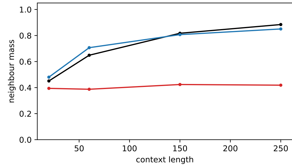
Qwen next-step neighbour MASS (graded)
