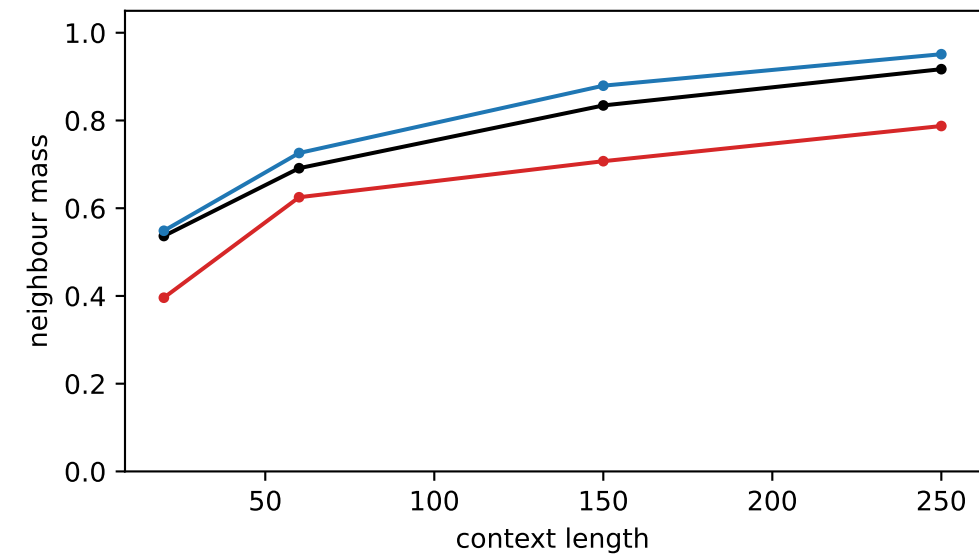
Gemma next-step neighbour MASS (graded)
