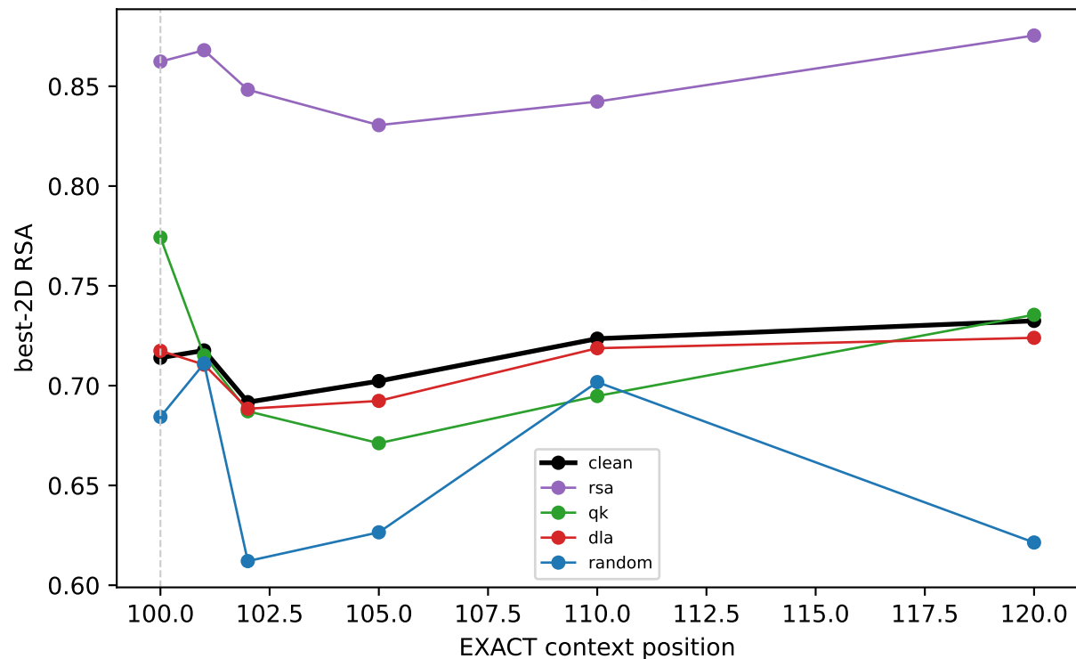
Qwen [square_grid]
