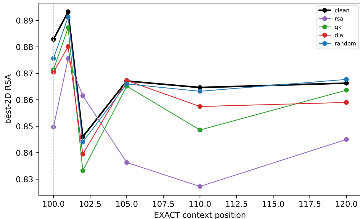
Gemma [square_grid]
