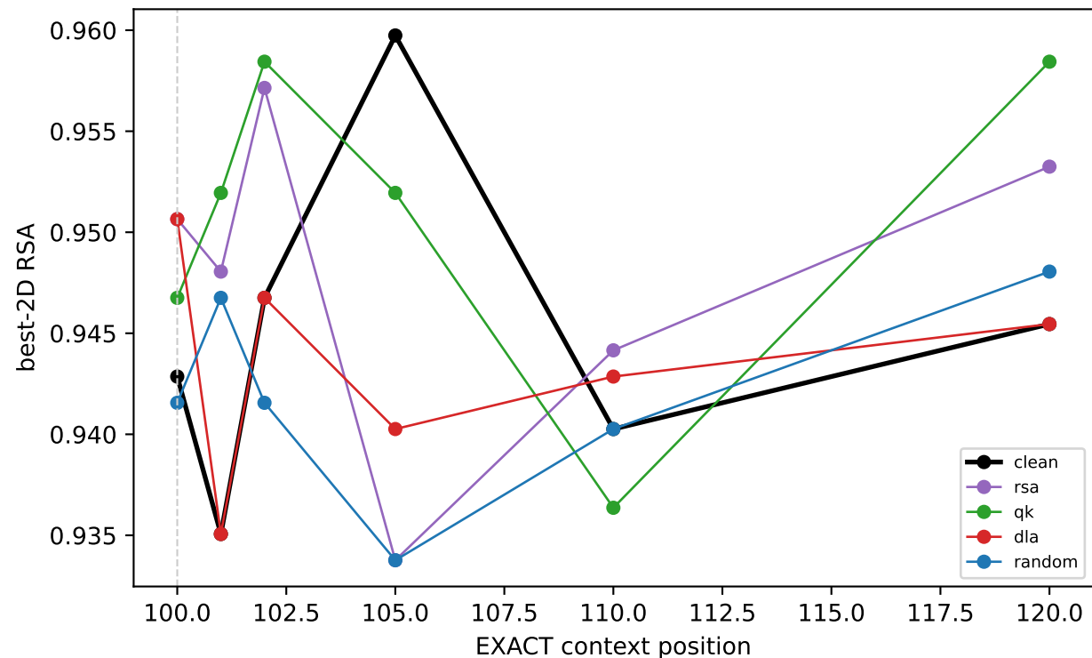
Qwen [days]
