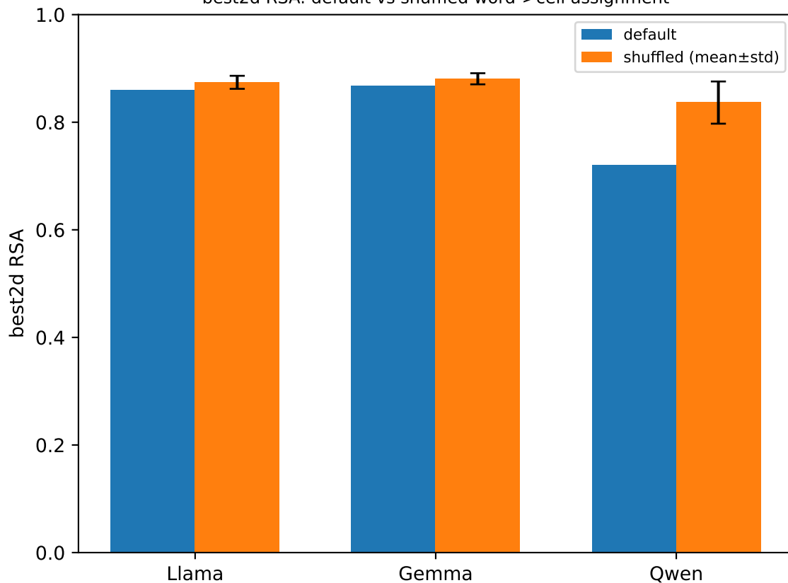
best2d RSA: default vs shuffled word->cell assignment
