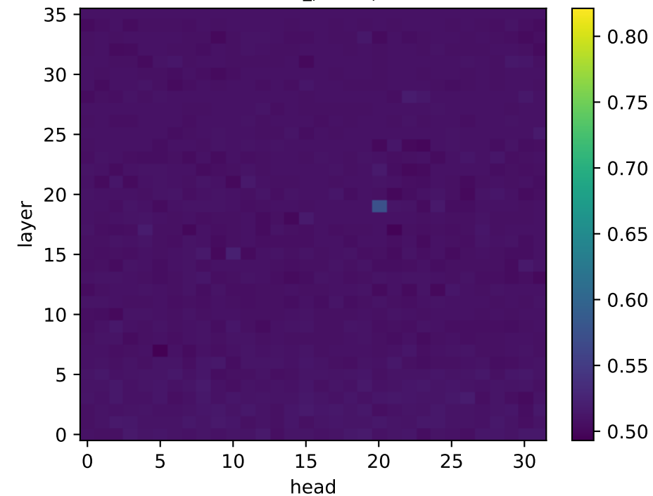
Qwen: \Delta RSA (restoration)
