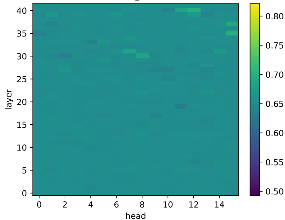
Gemma: \Delta RSA (restoration)
