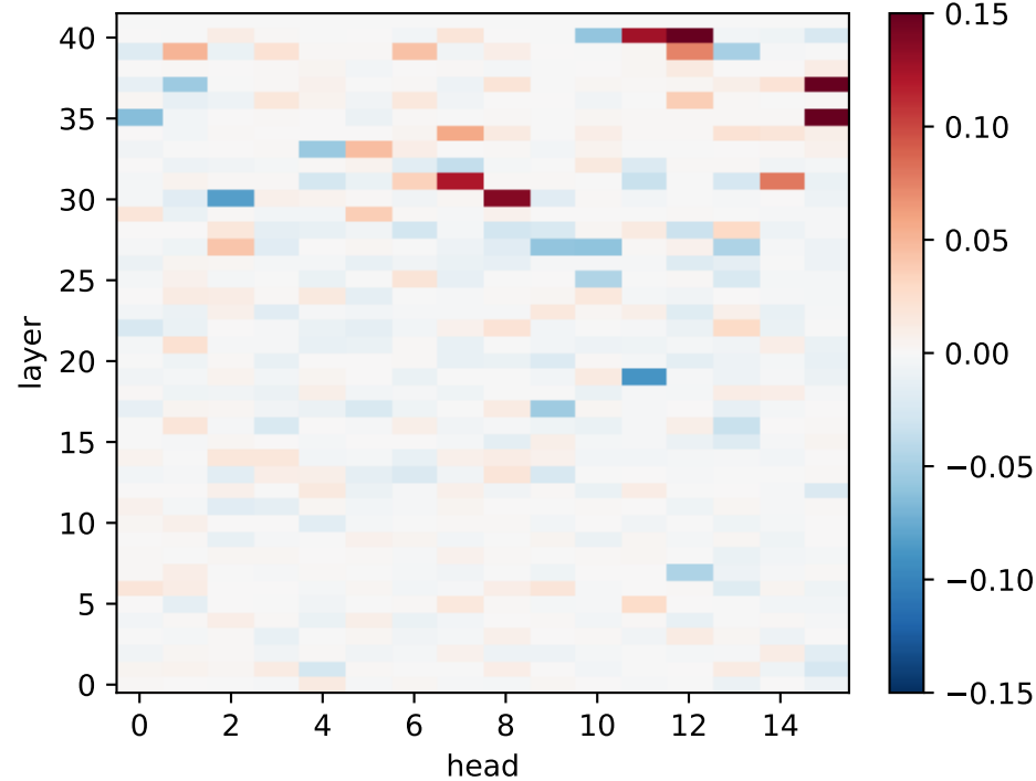
Gemma: \Delta RSA (restoration)
