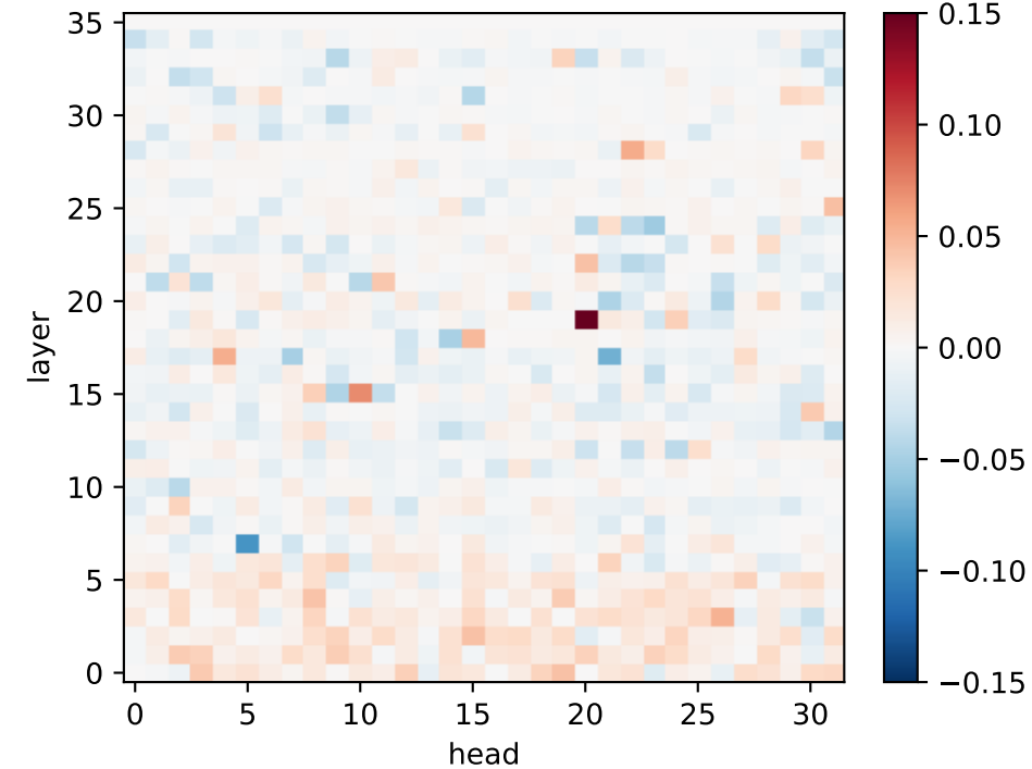
Qwen: \Delta RSA (restoration)
