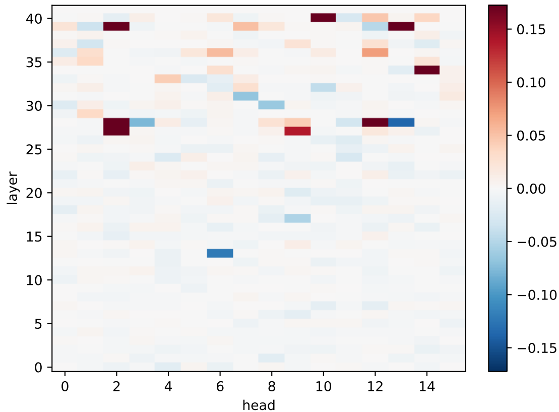
Gemma: \Delta RSA \rightarrow ring (geometry)
