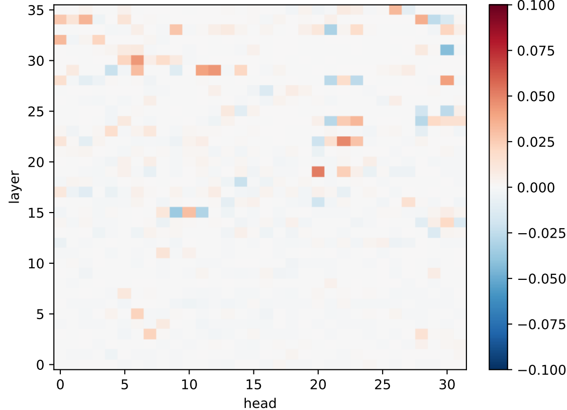
Qwen: \Delta ring-neighbour mass (behaviour)
