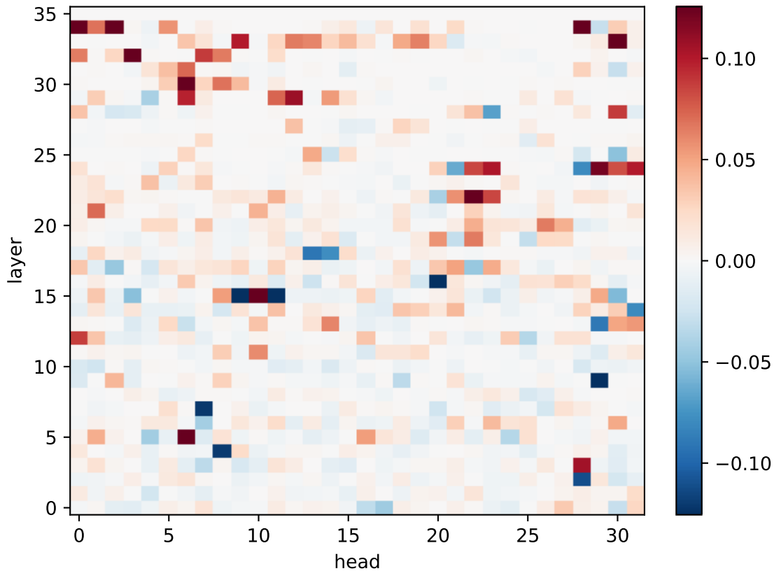
Qwen: \Delta RSA \rightarrow ring (geometry)
