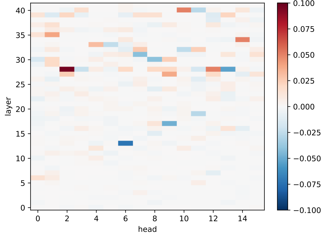
Gemma: \Delta ring-neighbour mass (behaviour)
