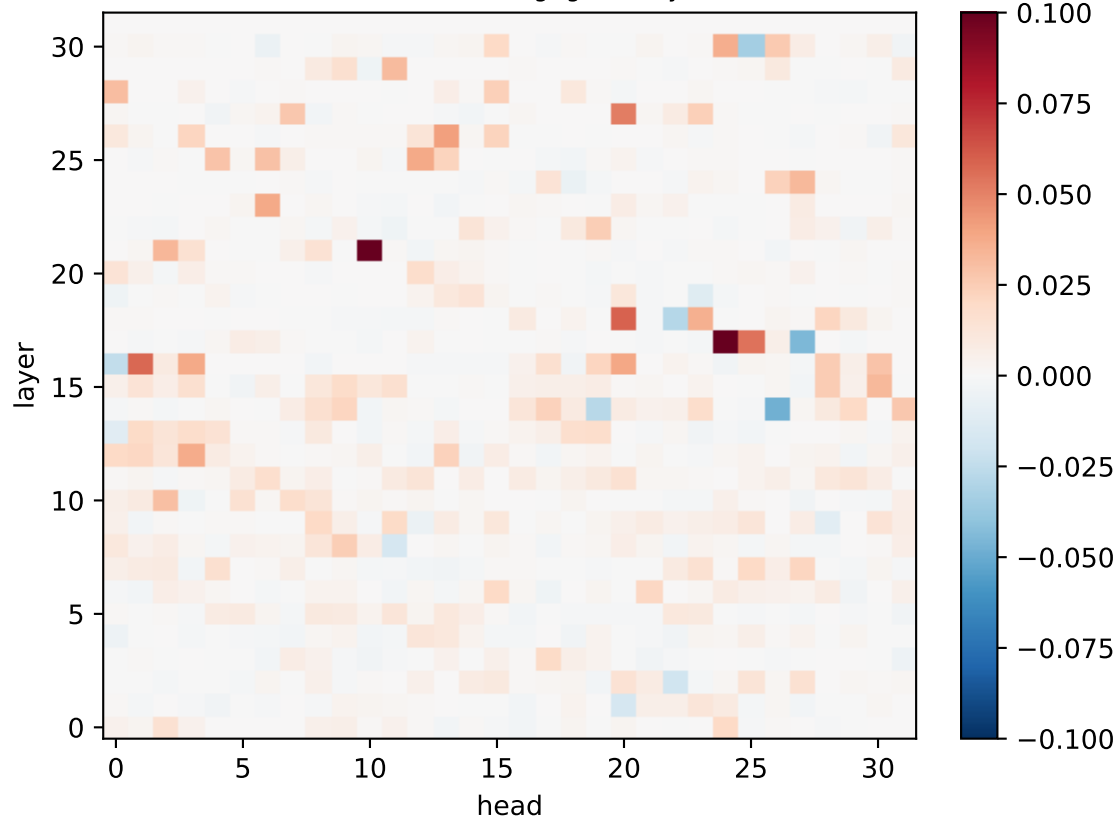
Llama: \Delta RSA \rightarrow ring (geometry)
