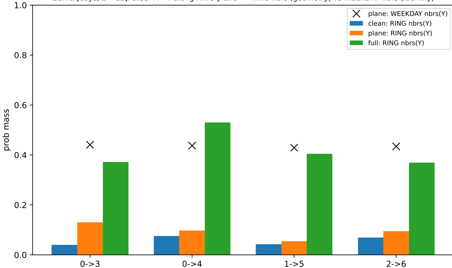
Llama [days, L*=12]: steer X->Y along RING plane -> RING nbrs (geometry) vs WEEKDAY nbrs (identity)
