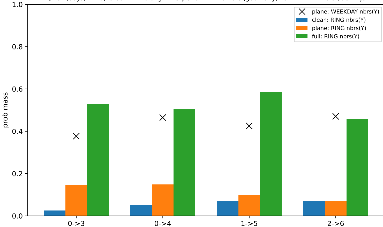
Qwen [days, L*=0]: steer X->Y along RING plane -> RING nbrs (geometry) vs WEEKDAY nbrs (identity)
