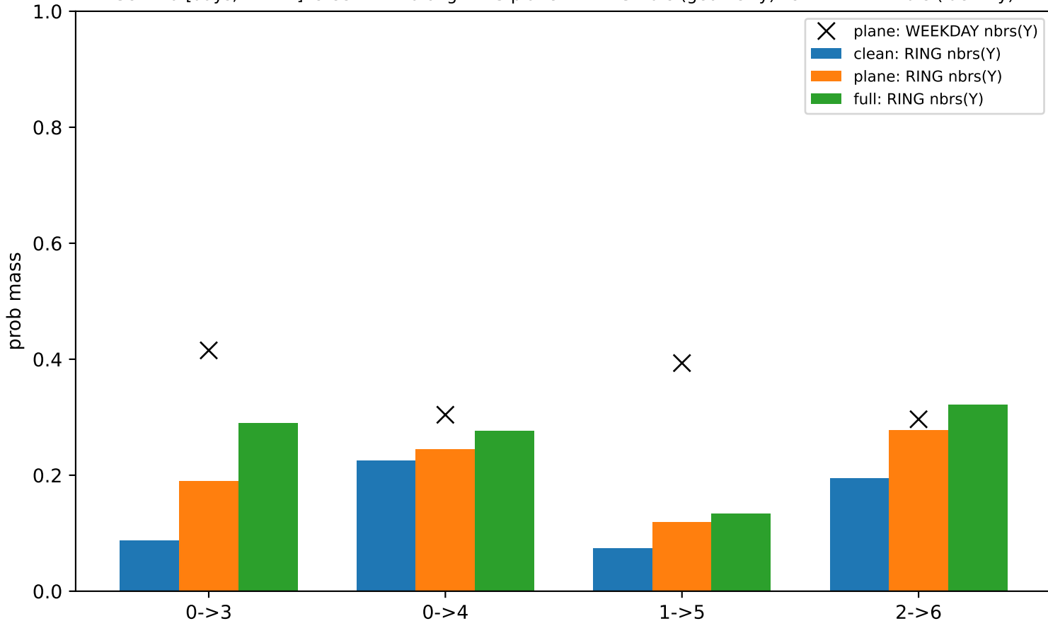
Gemma [days, L*=21]: steer X->Y along RING plane -> RING nbrs (geometry) vs WEEKDAY nbrs (identity)
