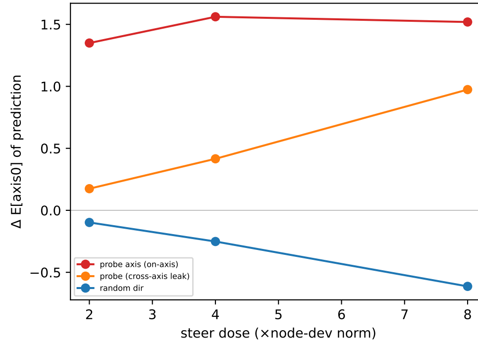
Gemma axis 1 ( L^*=33 , \text{probeR}^2=0.25 )
