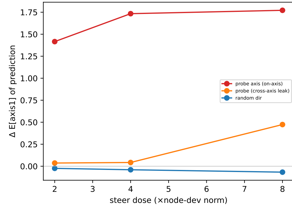
Llama axis 1 ( L^*=25 , \text{probeR}^2=0.63 )
