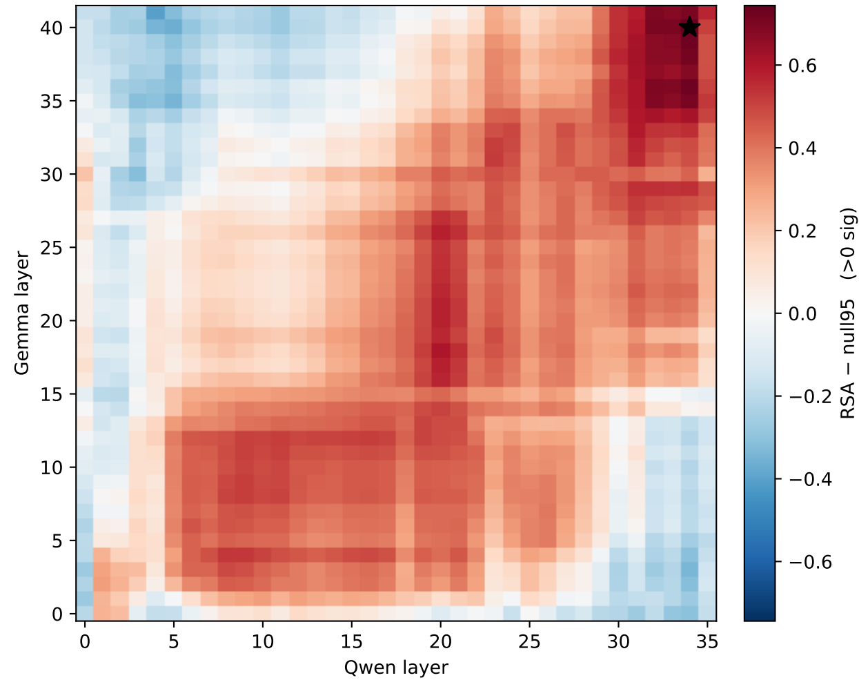
Gemma vs Qwen (null95=0.16; 76% sig)
