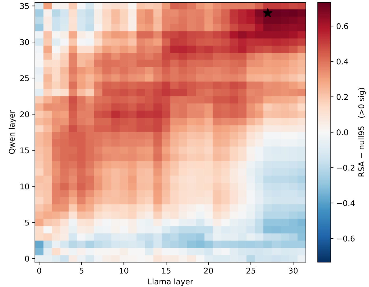
Qwen vs Llama (null95=0.16; 78% sig)
