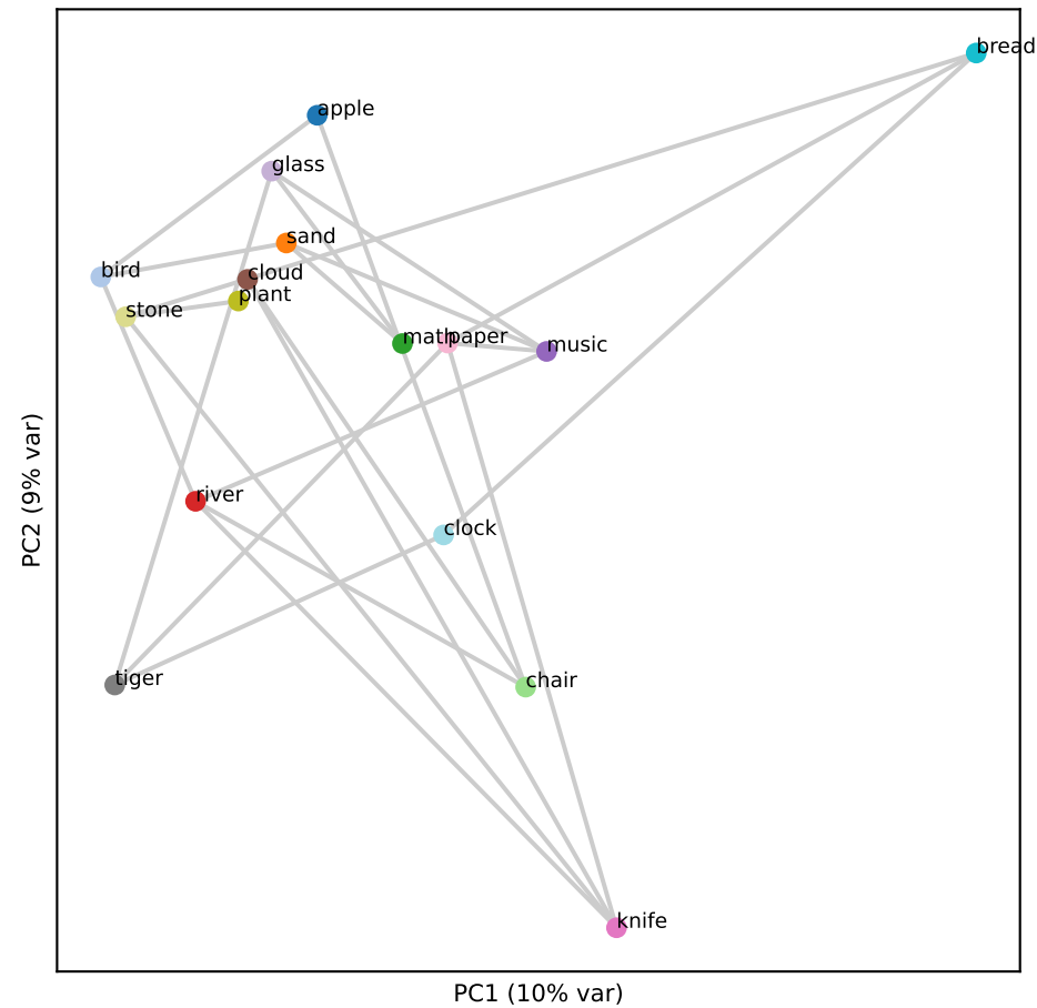
Qwen L4 (RSA -0.10)
