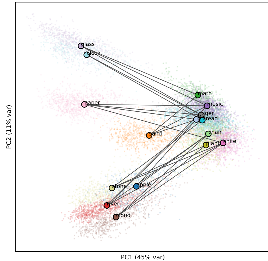
Qwen L35 (RSA -0.03)
