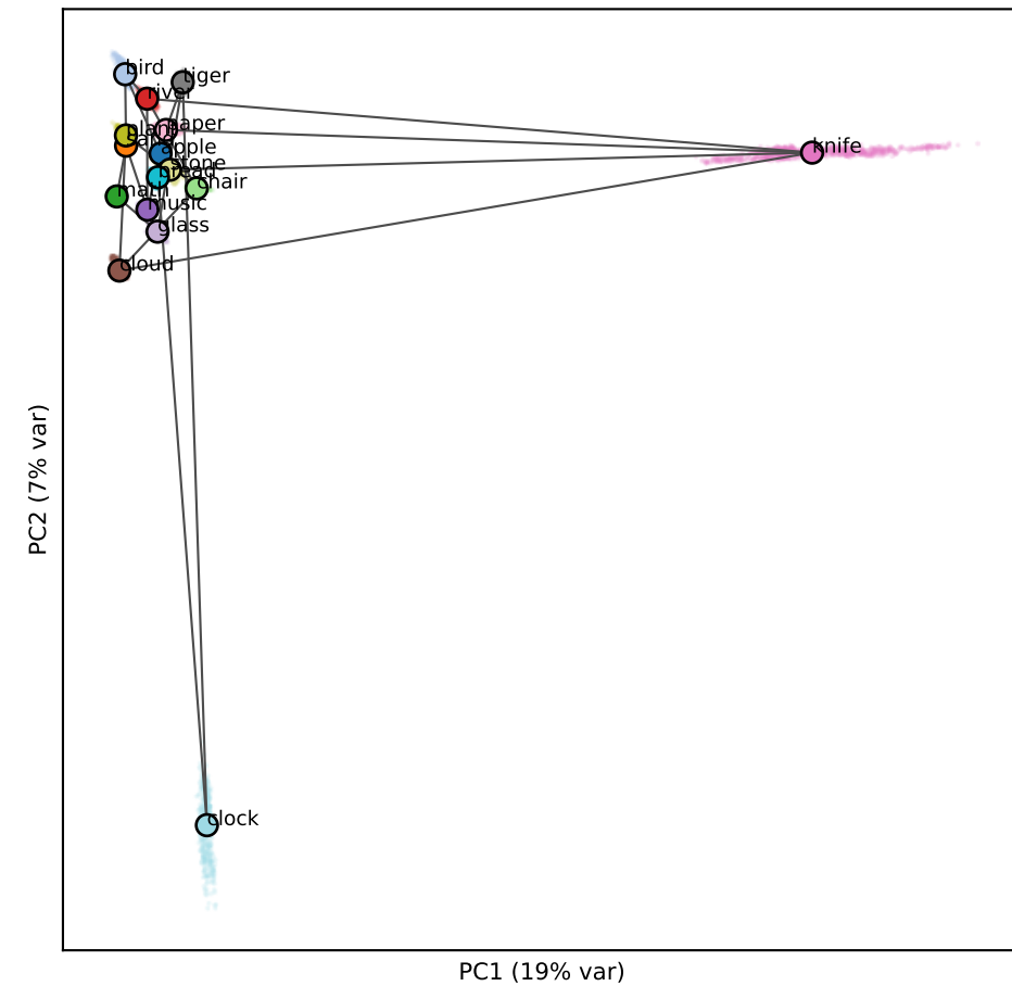
Qwen L1 (RSA -0.06)
