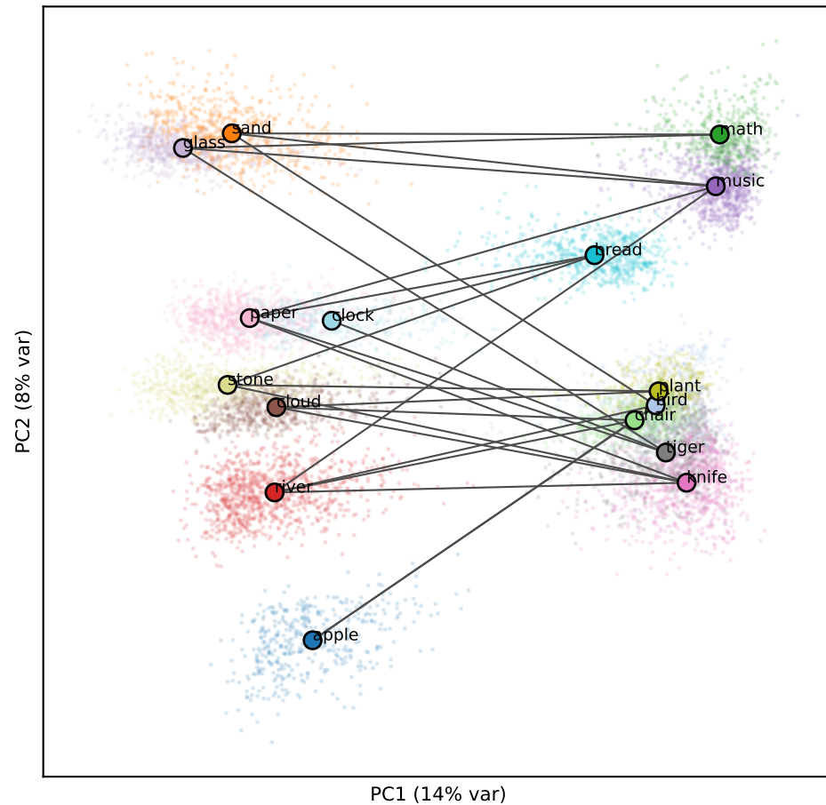
Qwen L24 (RSA -0.03)
