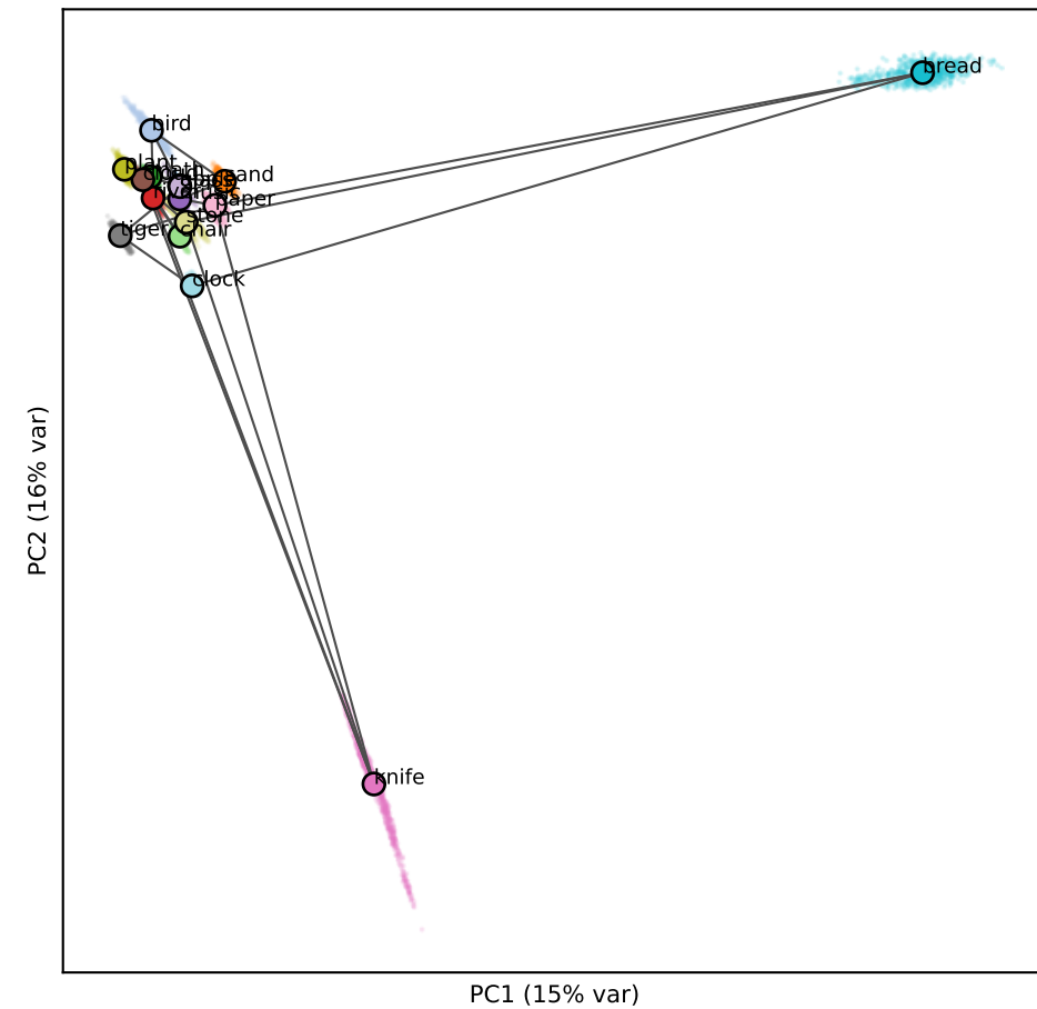
Qwen L2 (RSA 0.02)
