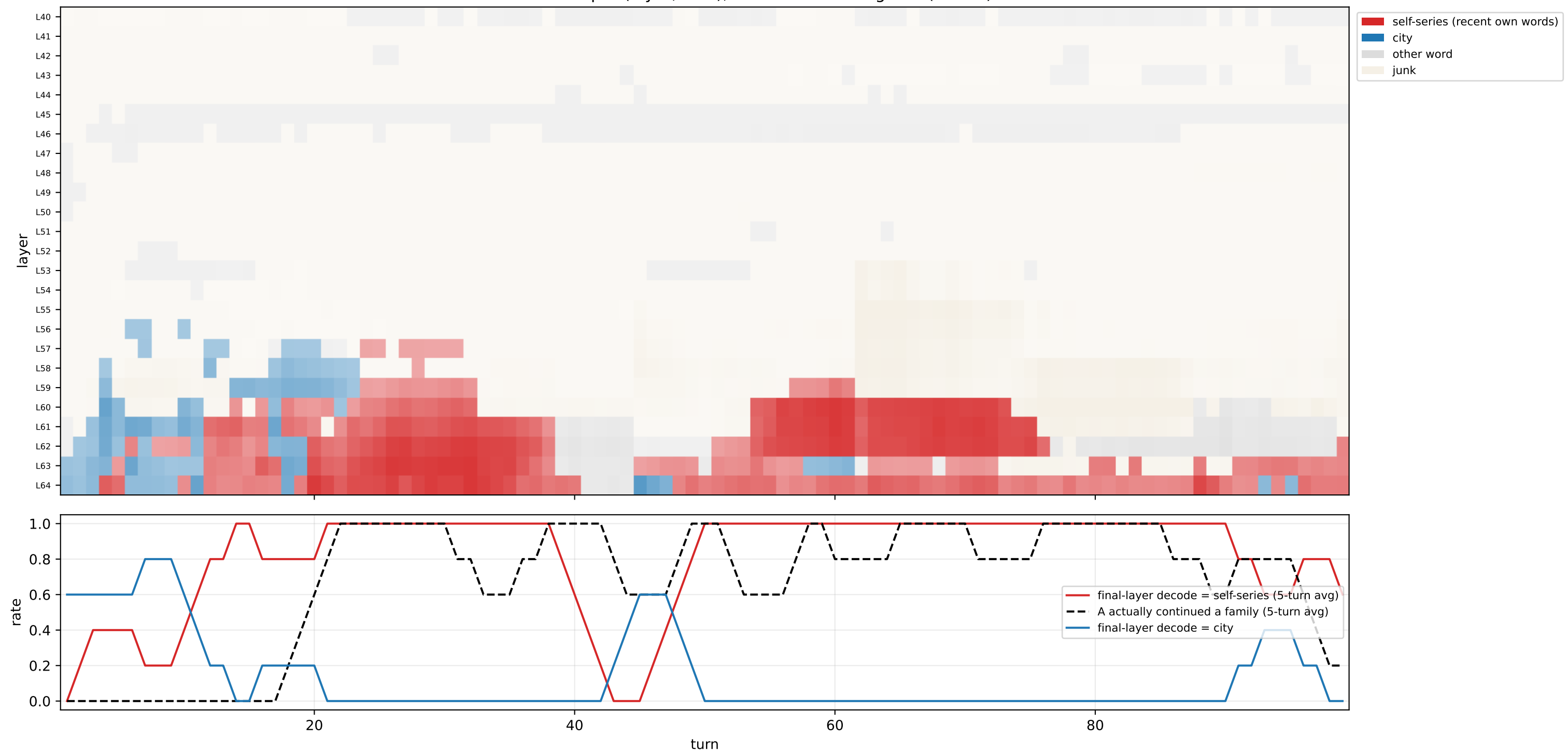
Force-decoded class per (layer, turn), 99-turn no-meet game (roll 23)
