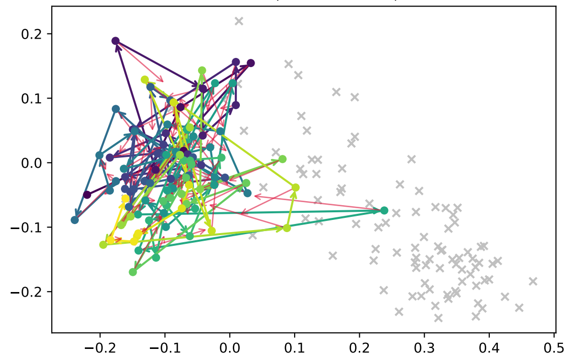
met game 10: model vs walk (colored = actual step, red = OU model prediction)
