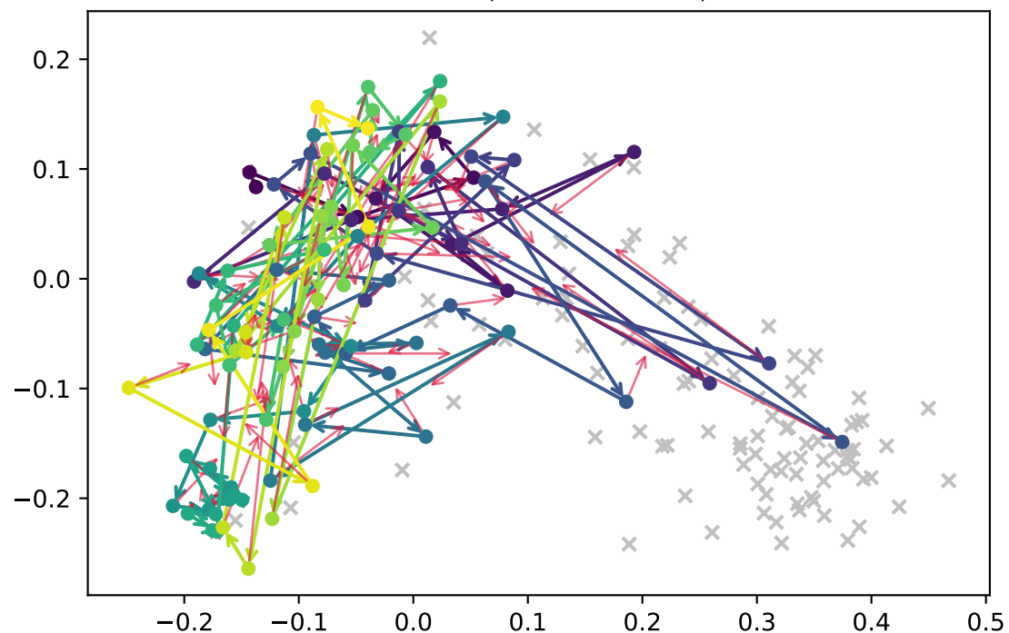
stuck game 0: model vs walk (colored = actual step, red = OU model prediction)
