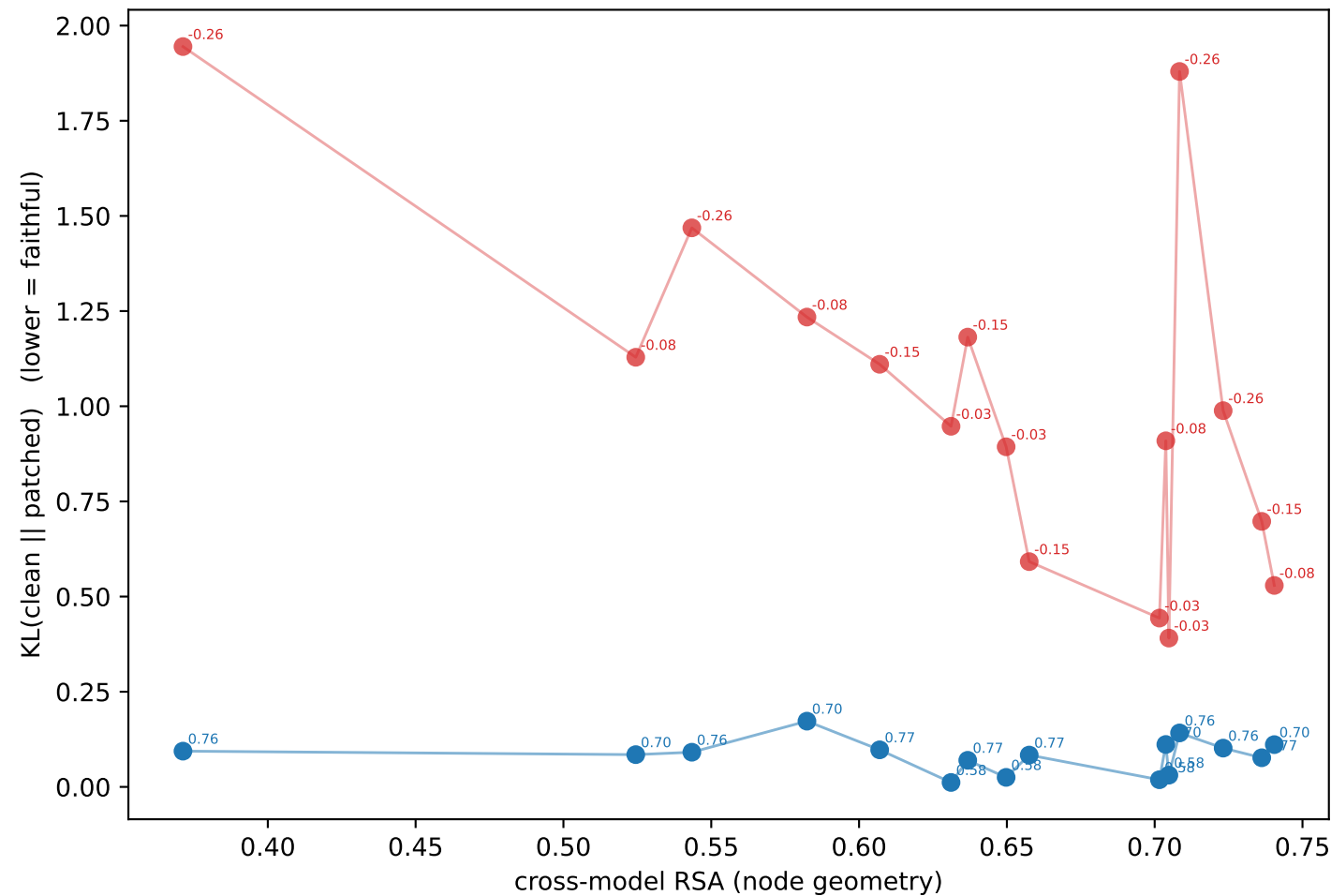
KL vs RSA (Spearman: real=+0.08, ctrl=-0.60)
