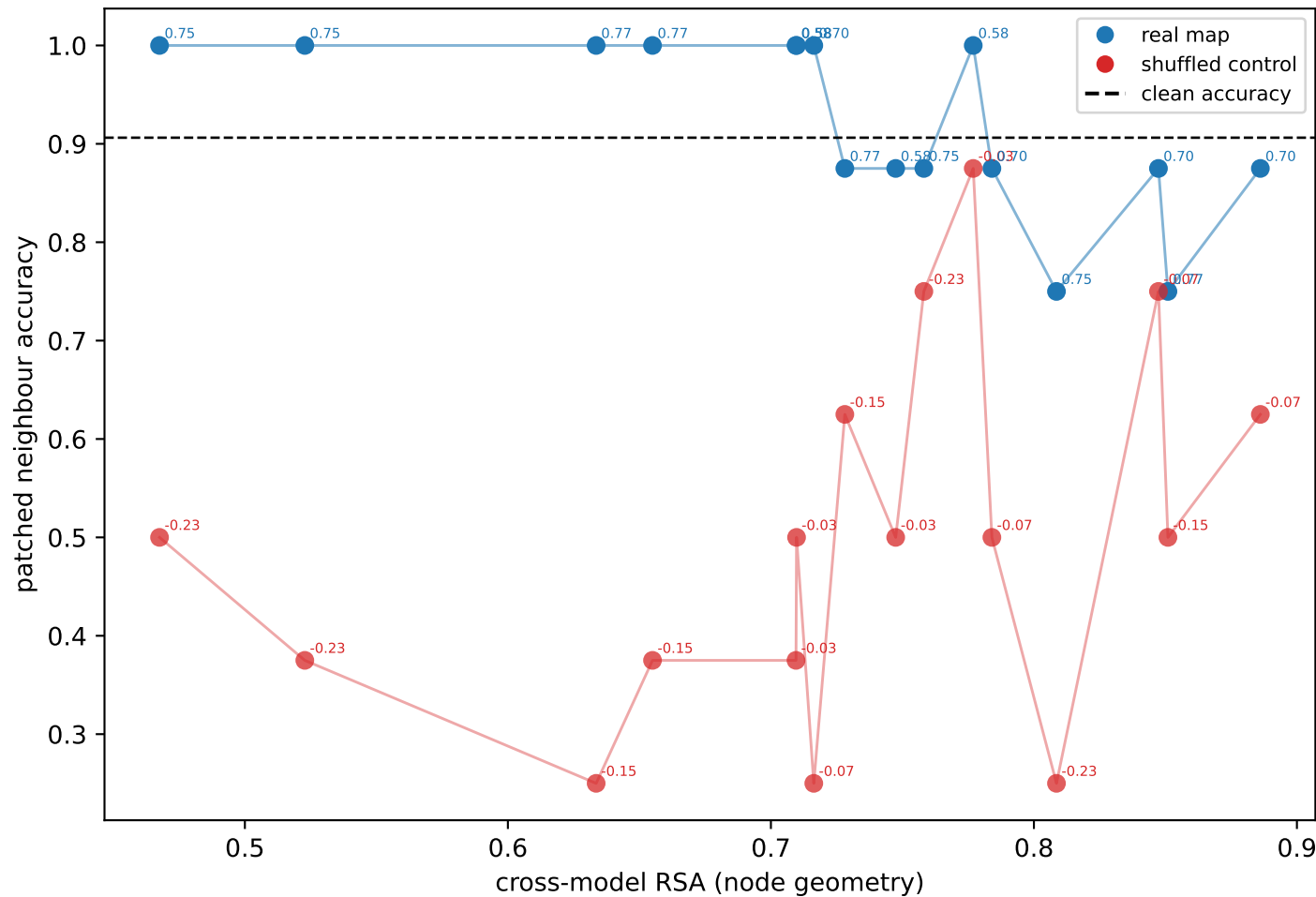
accuracy vs RSA (Spearman: real=-0.90, ctrl=+0.43)
