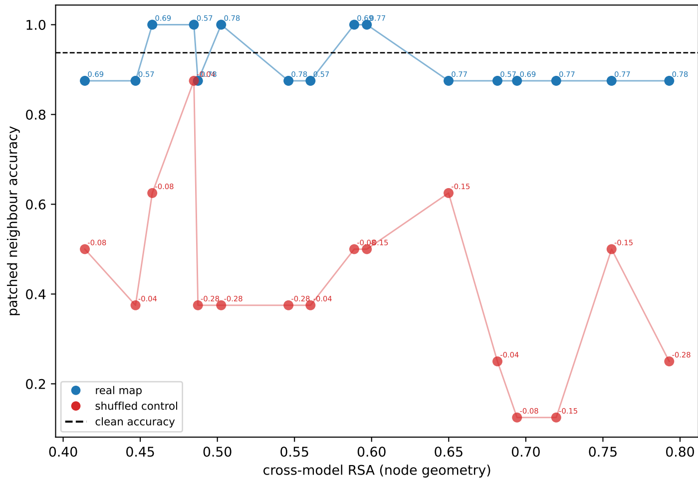
accuracy vs RSA (Spearman: real=-0.19, ctrl=-0.41)
