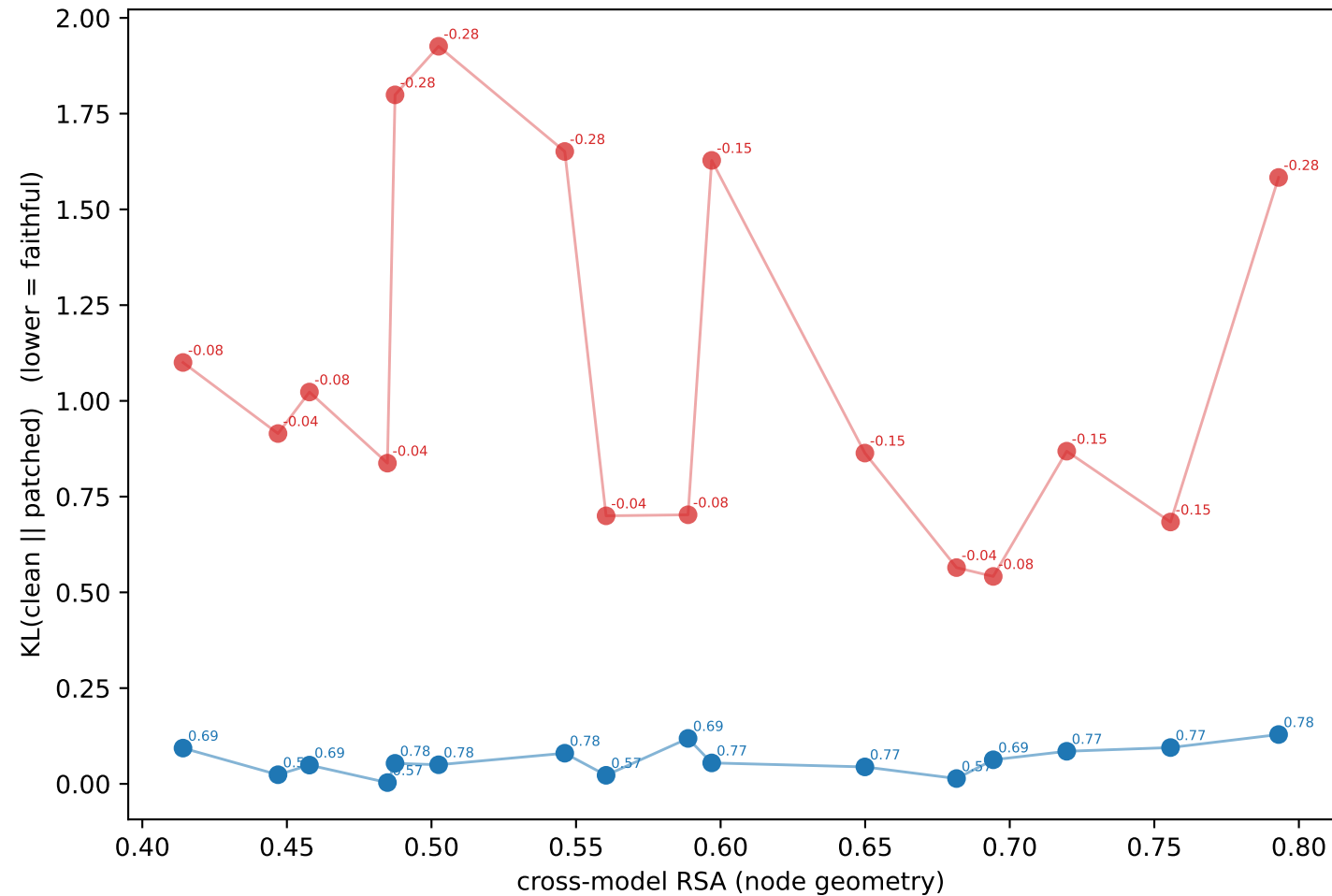
KL vs RSA (Spearman: real=+0.41, ctrl=-0.39)
