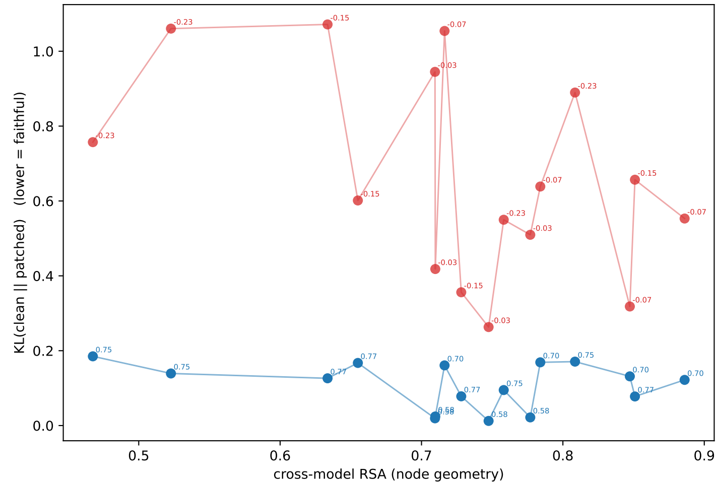
KL vs RSA (Spearman: real=-0.16, ctrl=-0.43)
