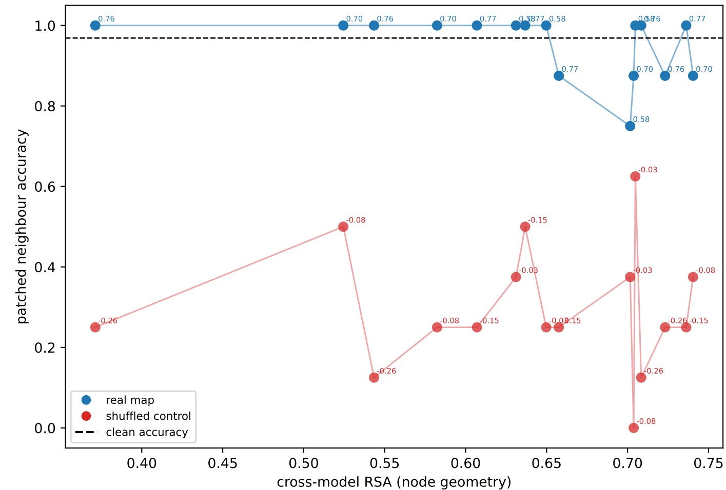
accuracy vs RSA (Spearman: real=-0.54, ctrl=-0.04)
