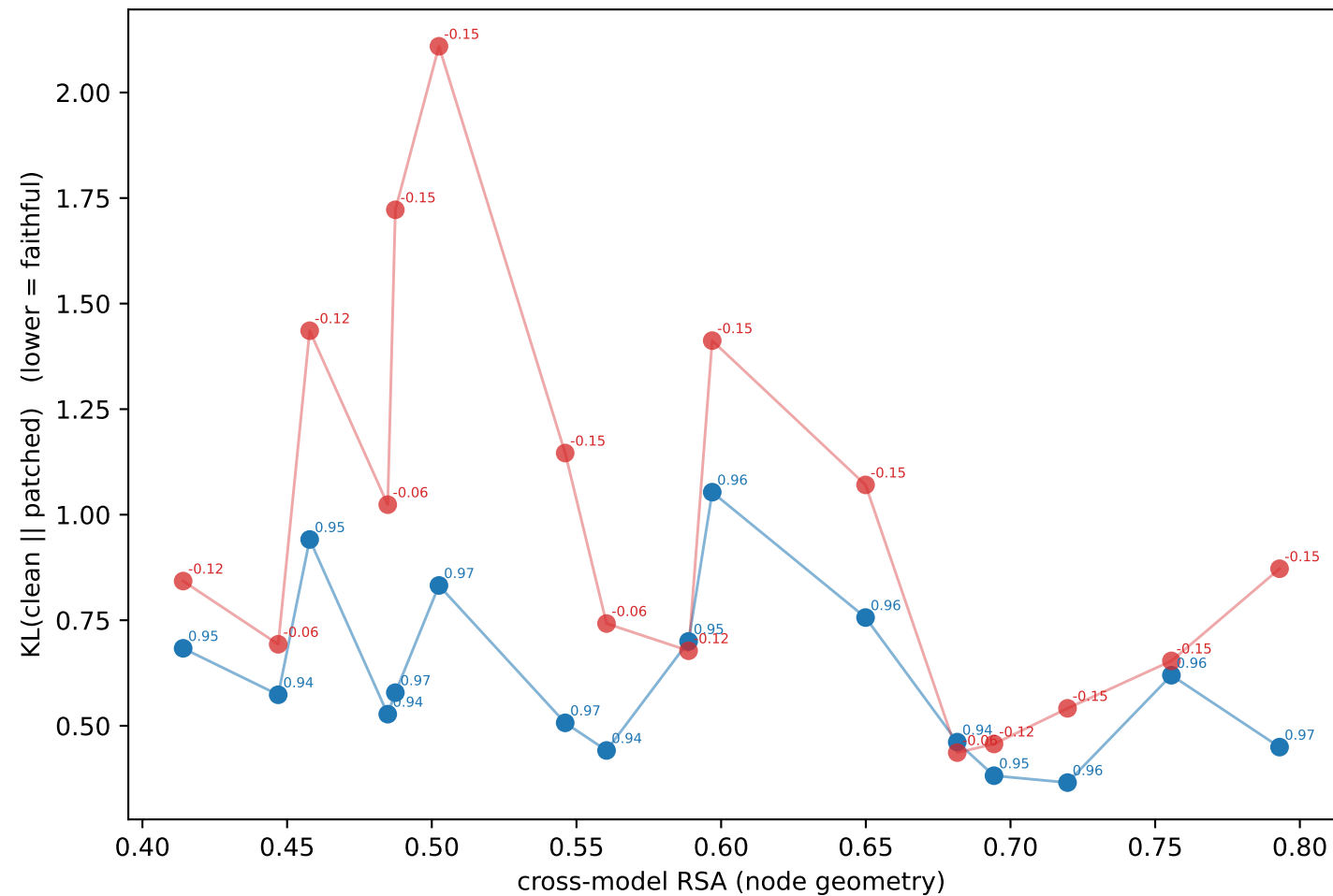
KL vs RSA (Spearman: real=-0.40, ctrl=-0.48)
