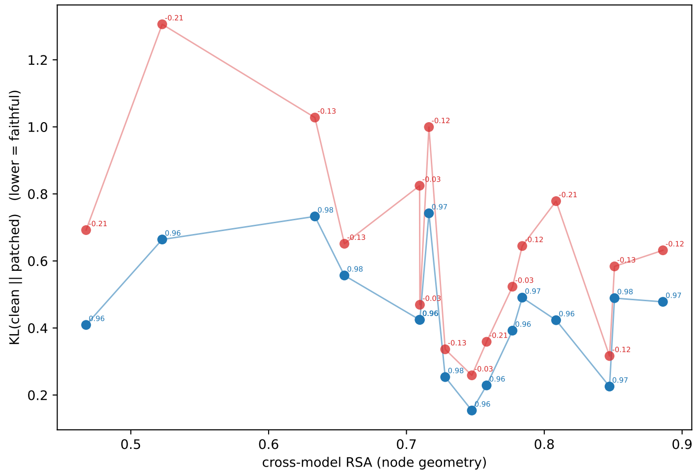
KL vs RSA (Spearman: real=-0.31, ctrl=-0.50)
