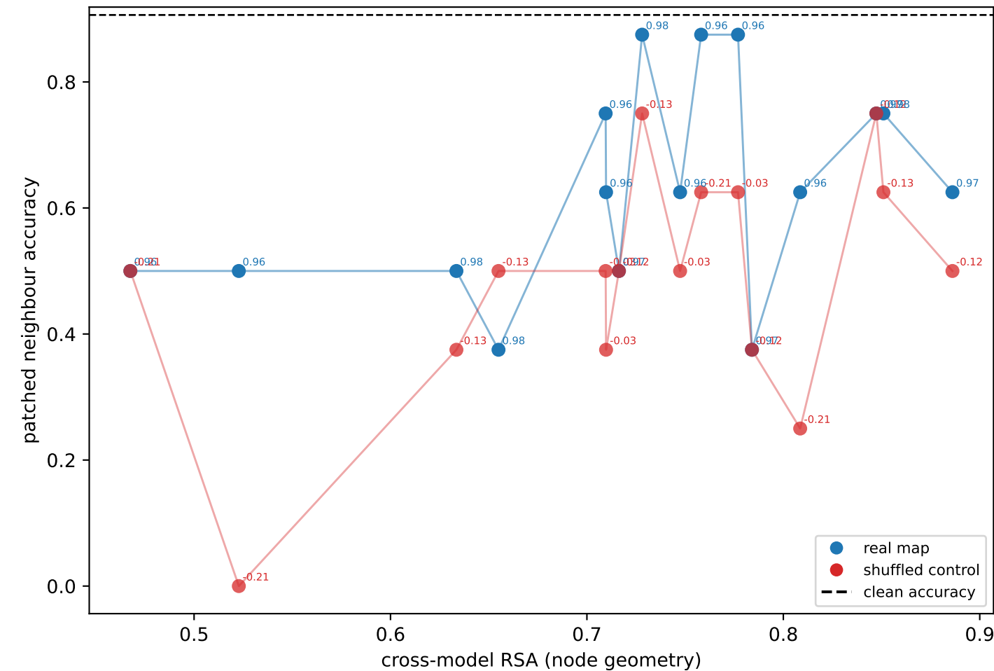
accuracy vs RSA (Spearman: real=+0.44, ctrl=+0.26)
