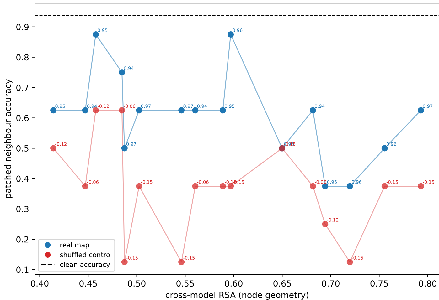
accuracy vs RSA (Spearman: real=-0.49, ctrl=-0.32)
