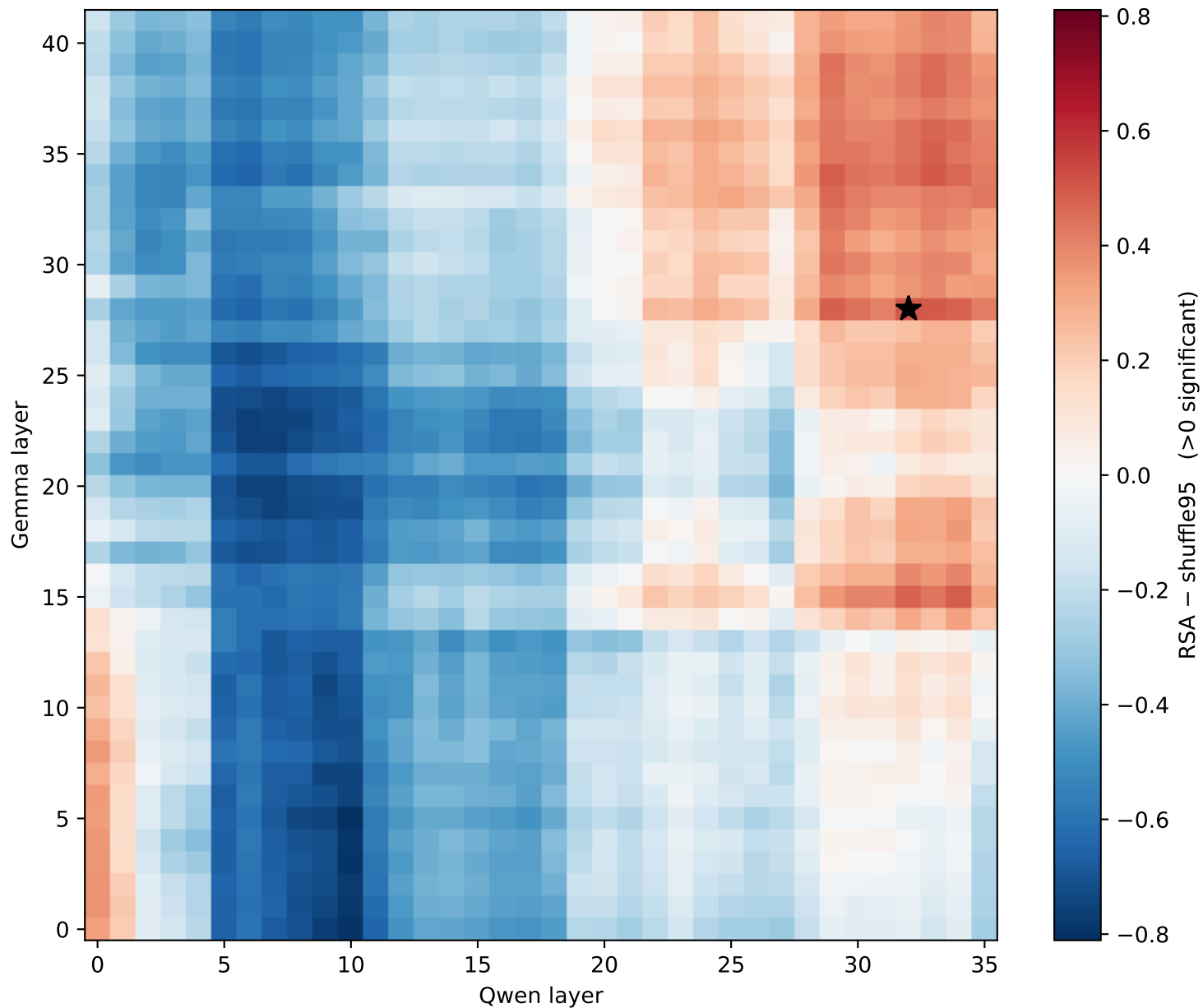
days [v1] Gemma vs Qwen: RSA – per-cell shuffle-null95 red = above shuffle null; 30% of cells > null
