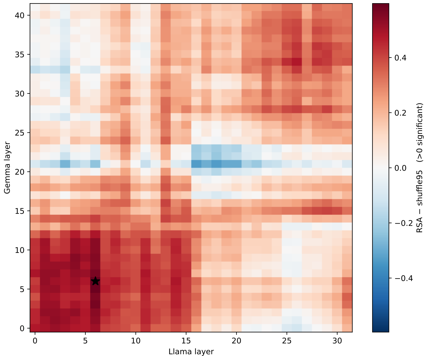
days [v1] Gemma vs Llama: RSA – per-cell shuffle-null95 red = above shuffle null; 89% of cells > null
