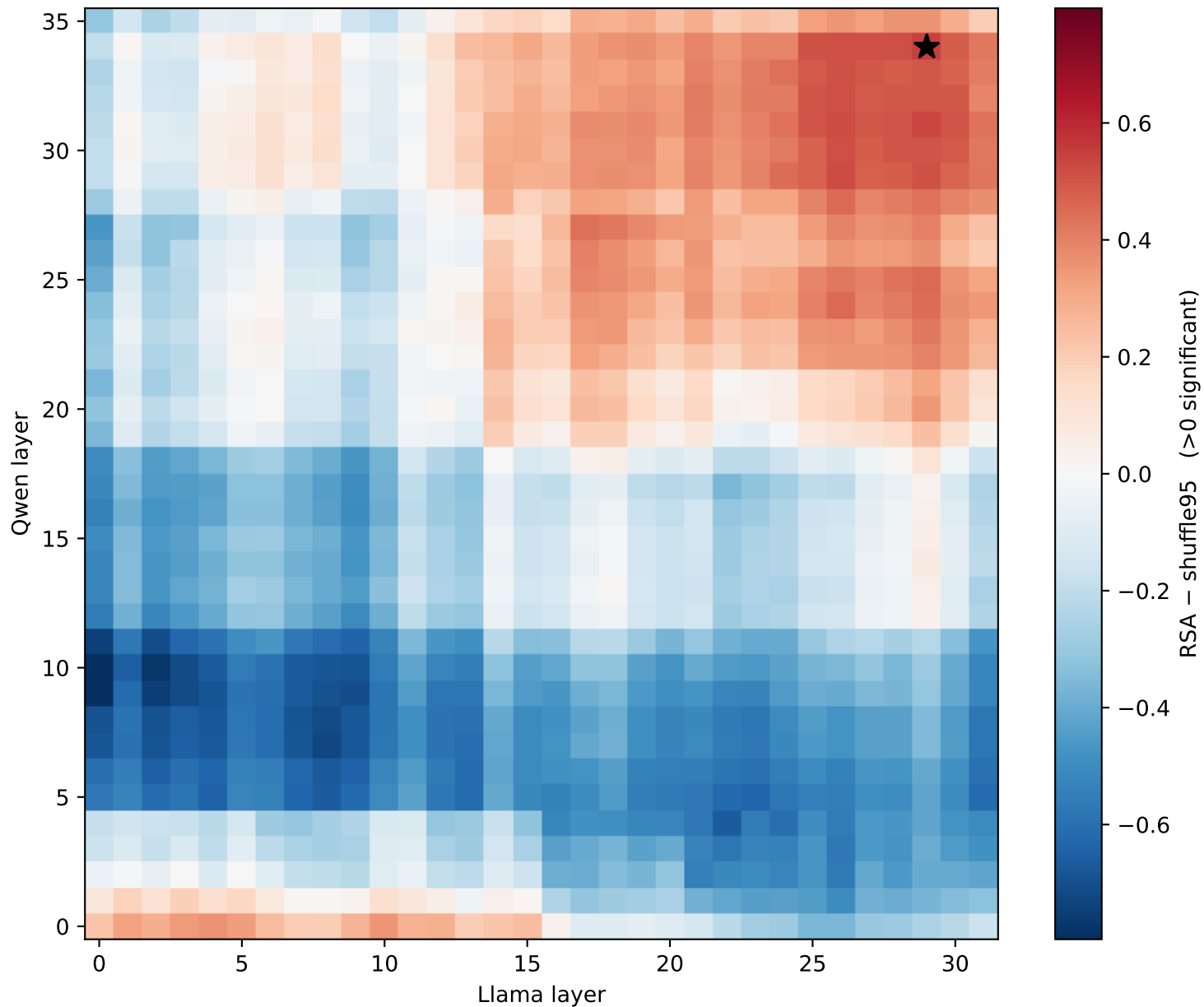
days [v1] Qwen vs Llama: RSA – per-cell shuffle-null95 red = above shuffle null; 36% of cells > null
