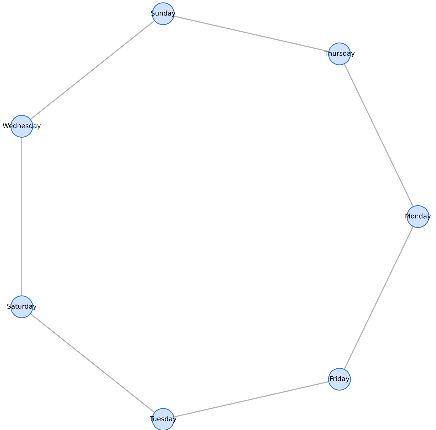
Graph: 7 nodes
