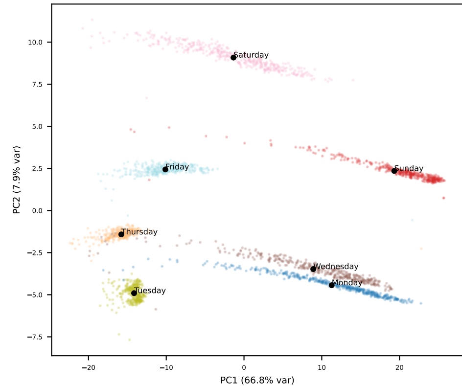
Qwen L4
