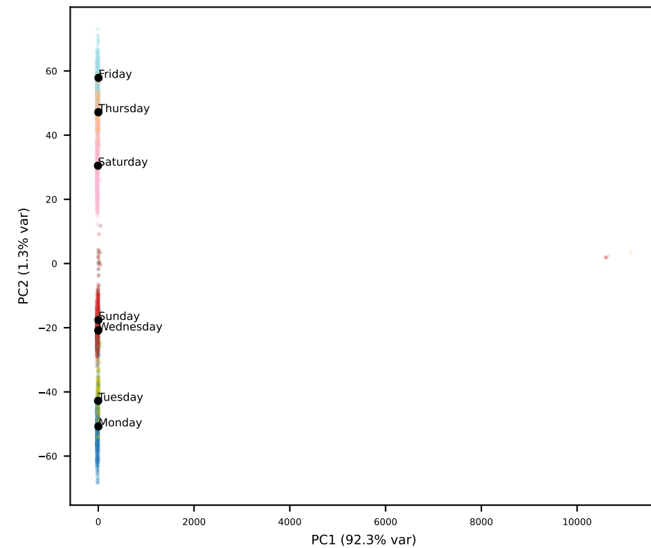
Qwen L26
