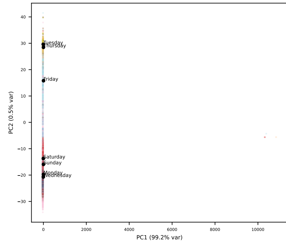
Qwen L8
