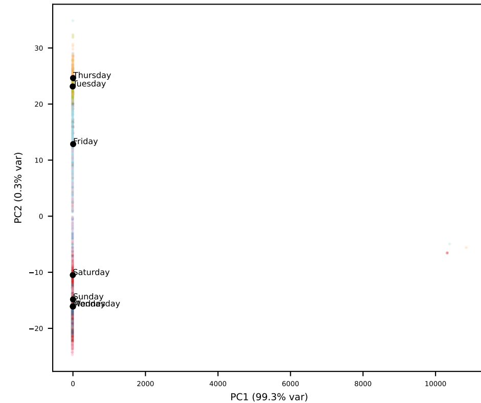
Qwen L10
