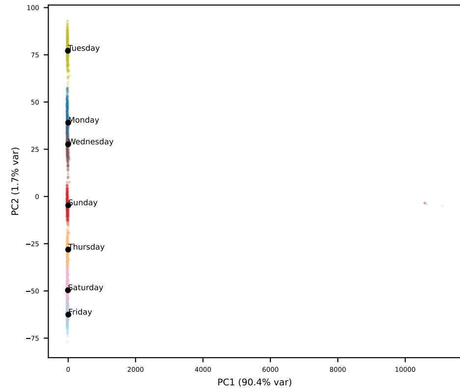
Qwen L27
