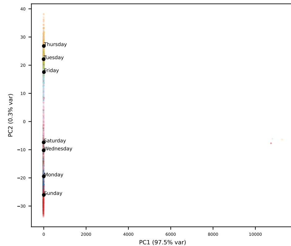
Qwen L20
