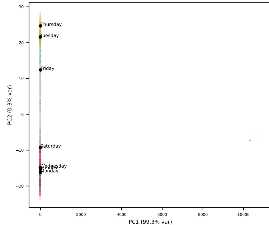
Qwen L11
