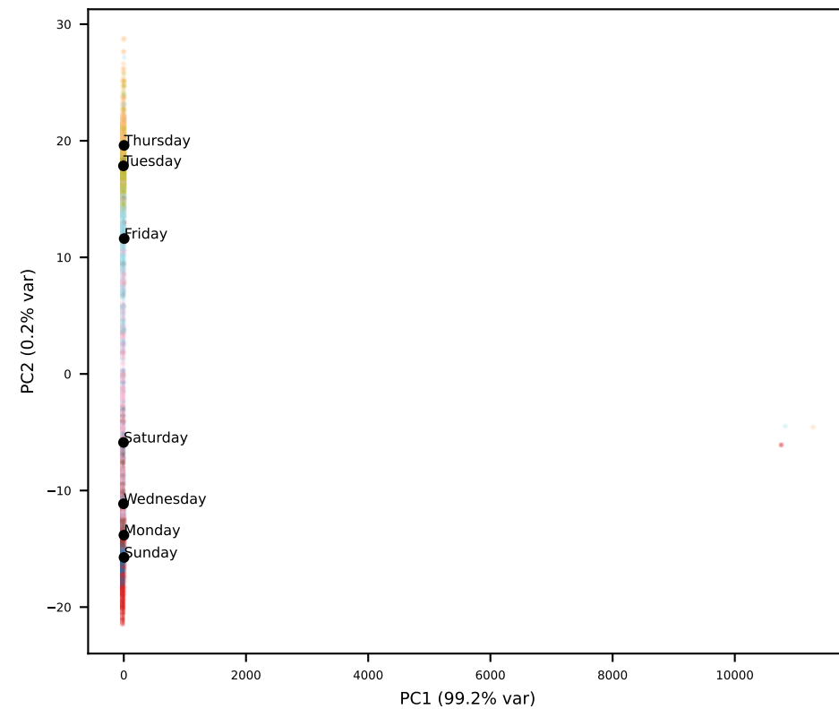
Qwen L16
