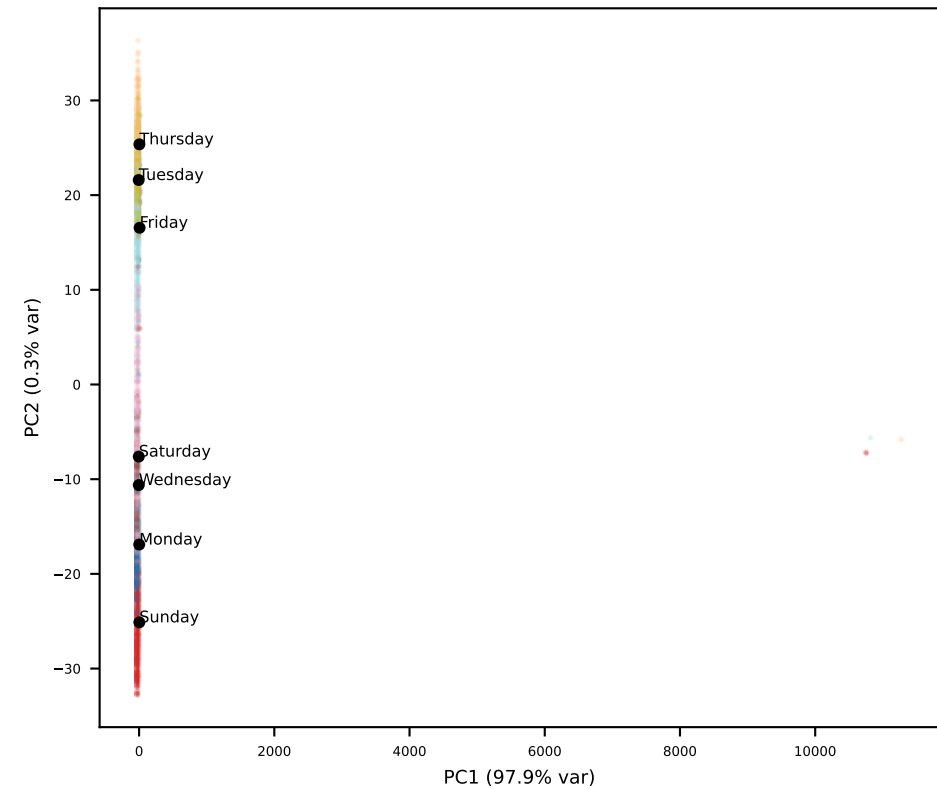
Qwen L19
