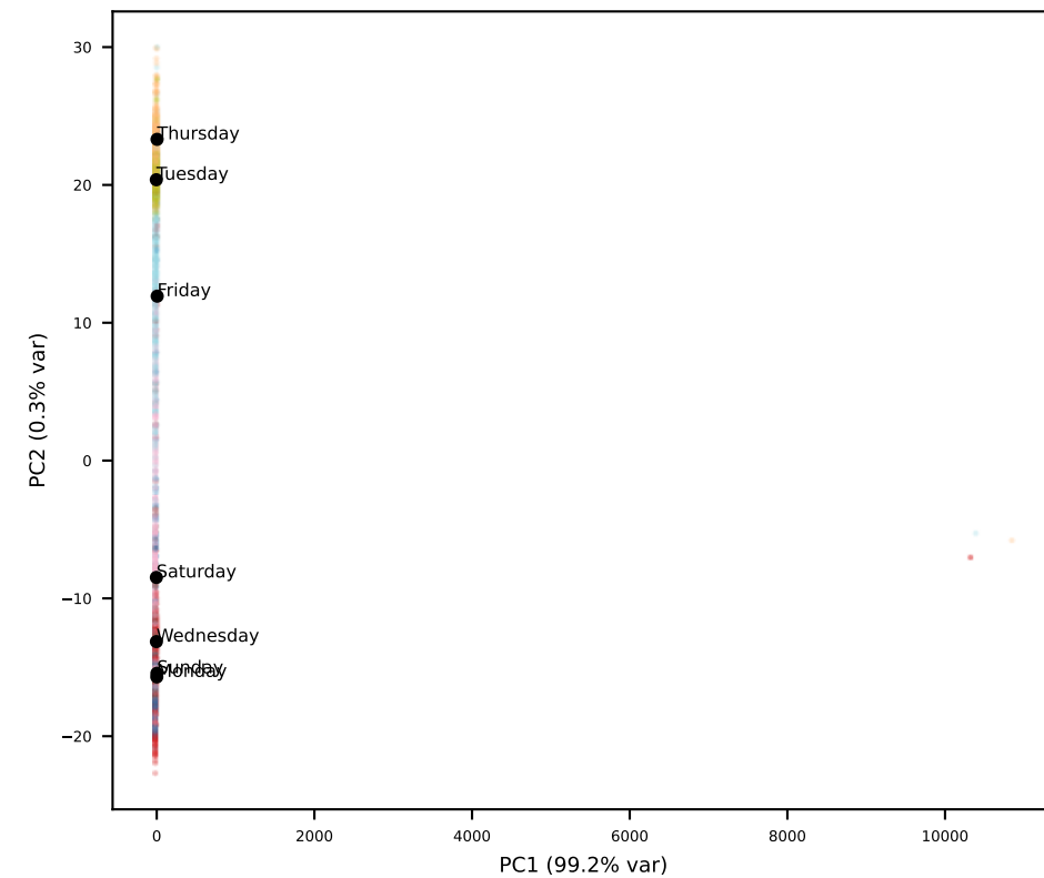
Qwen L12
