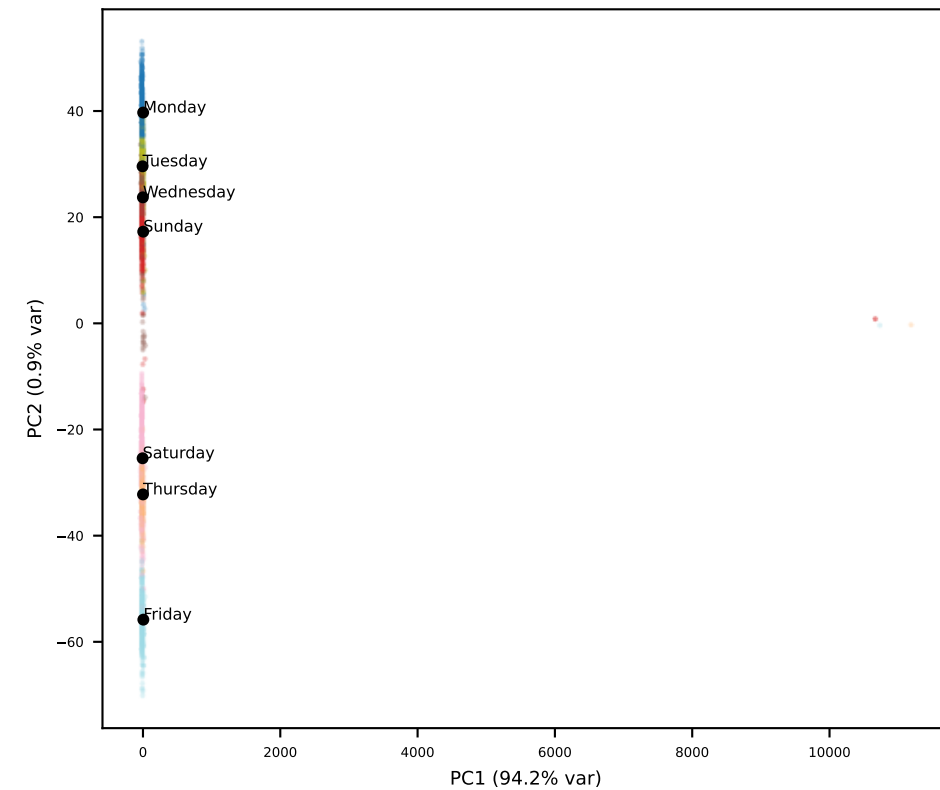
Qwen L24
