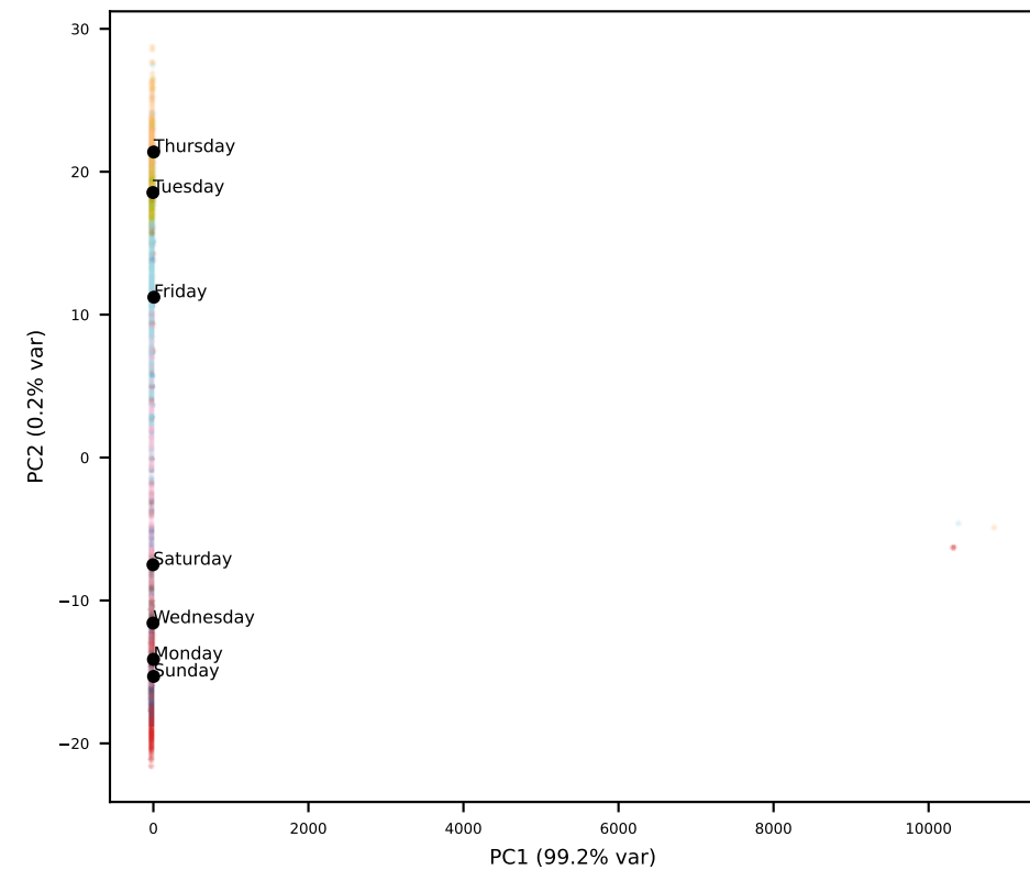
Qwen L14
