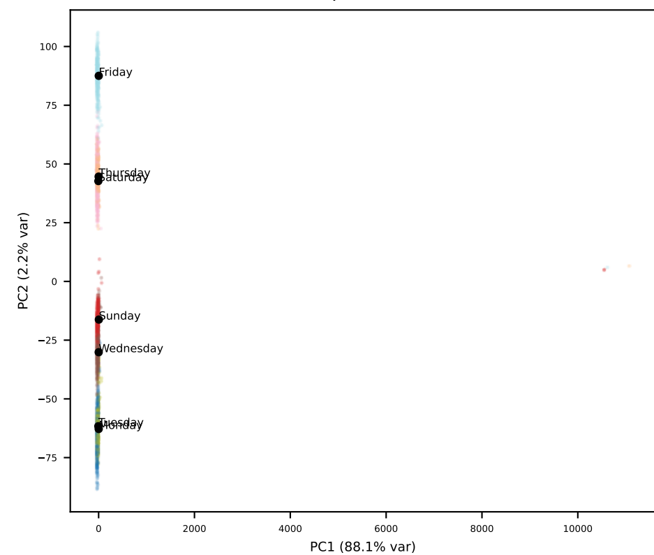
Qwen L28
