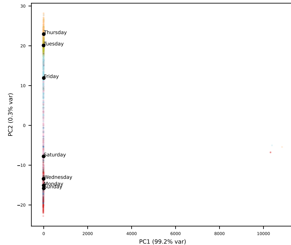
Qwen L13
