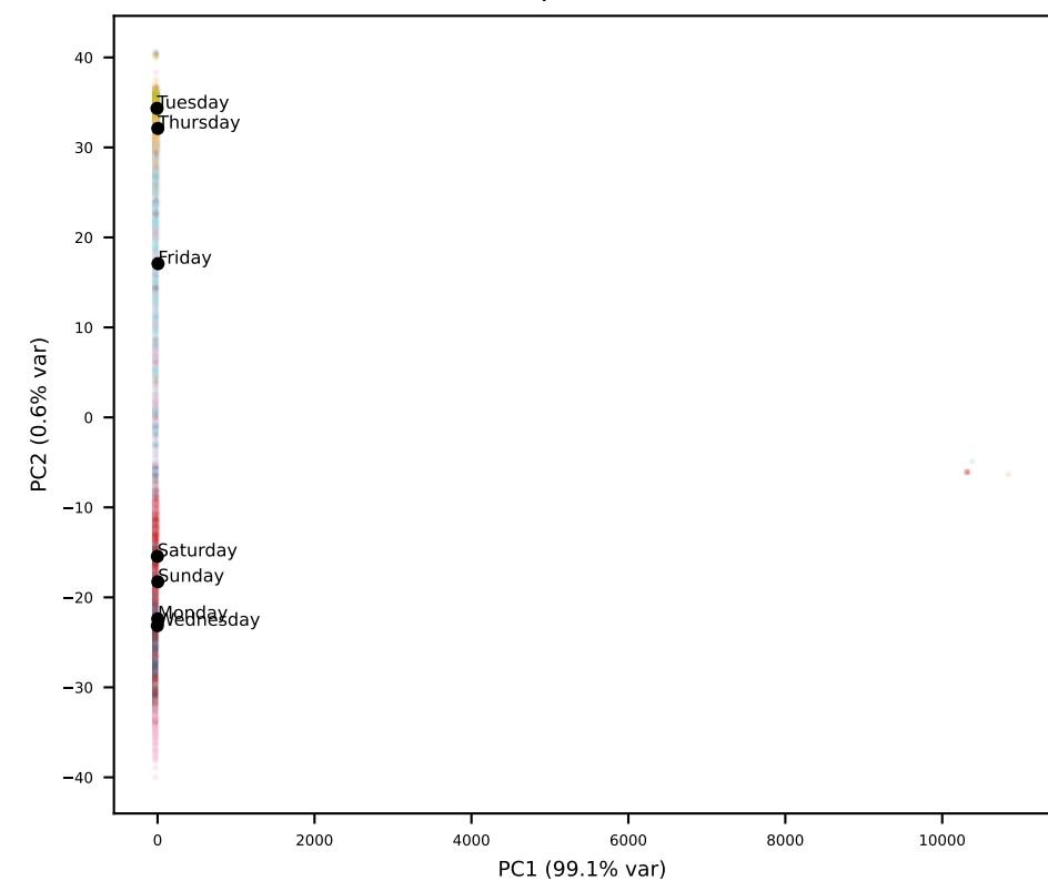
Qwen L6
