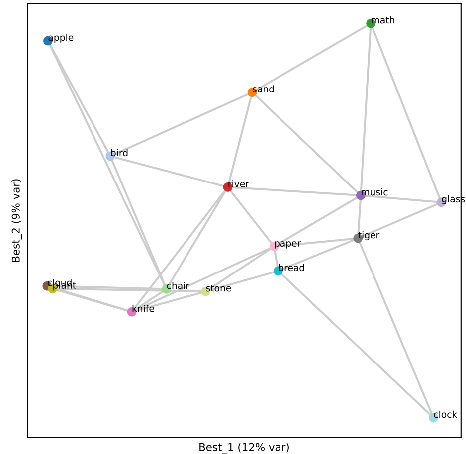
Qwen L29 (RSA 0.78)
