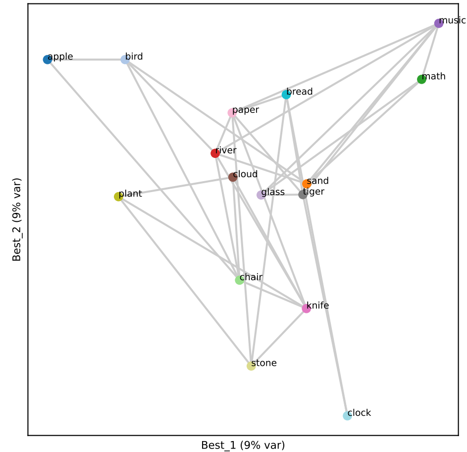
Qwen L13 (RSA 0.28)
