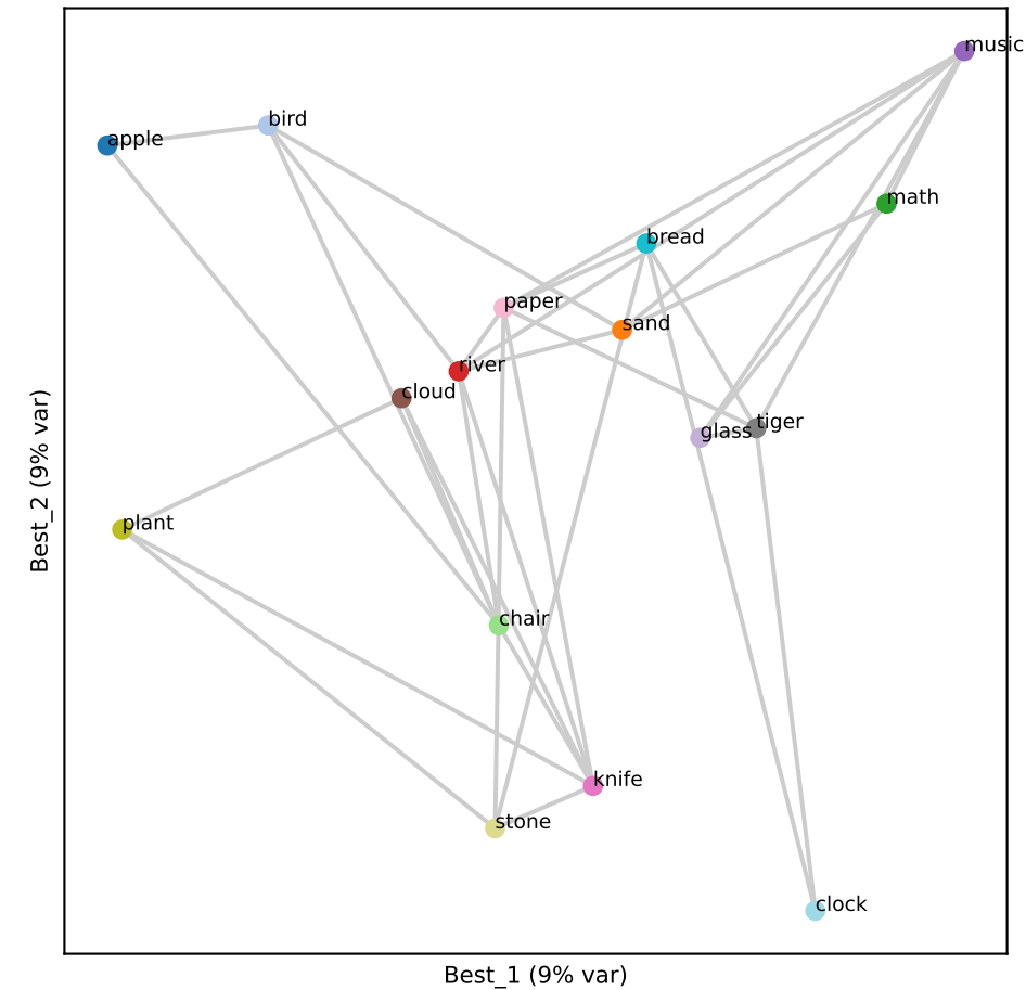
Qwen L17 (RSA 0.41)
