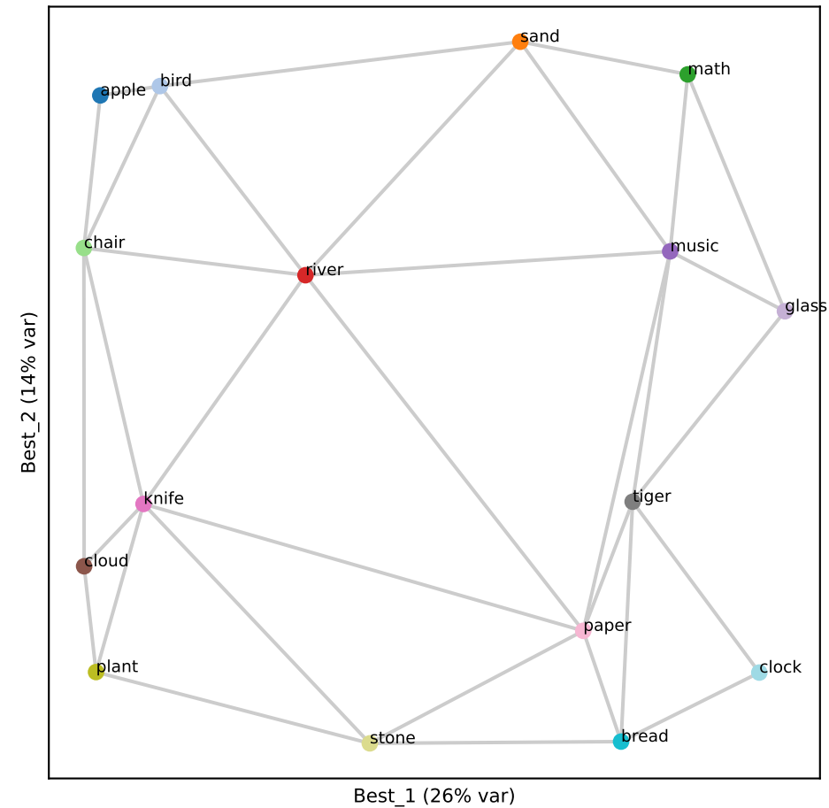
Qwen L35 (RSA 0.87)
