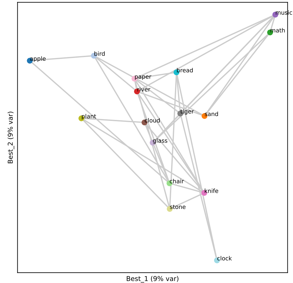
Qwen L11 (RSA 0.23)
