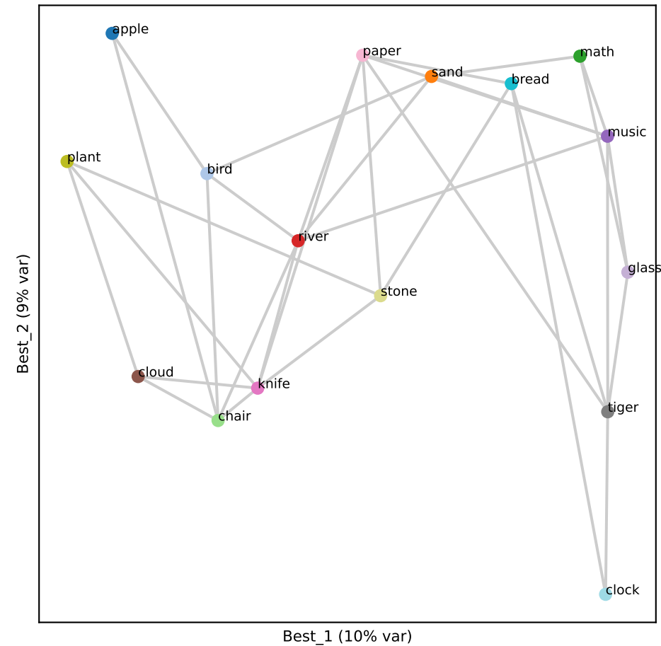
Qwen L22 (RSA 0.65)
