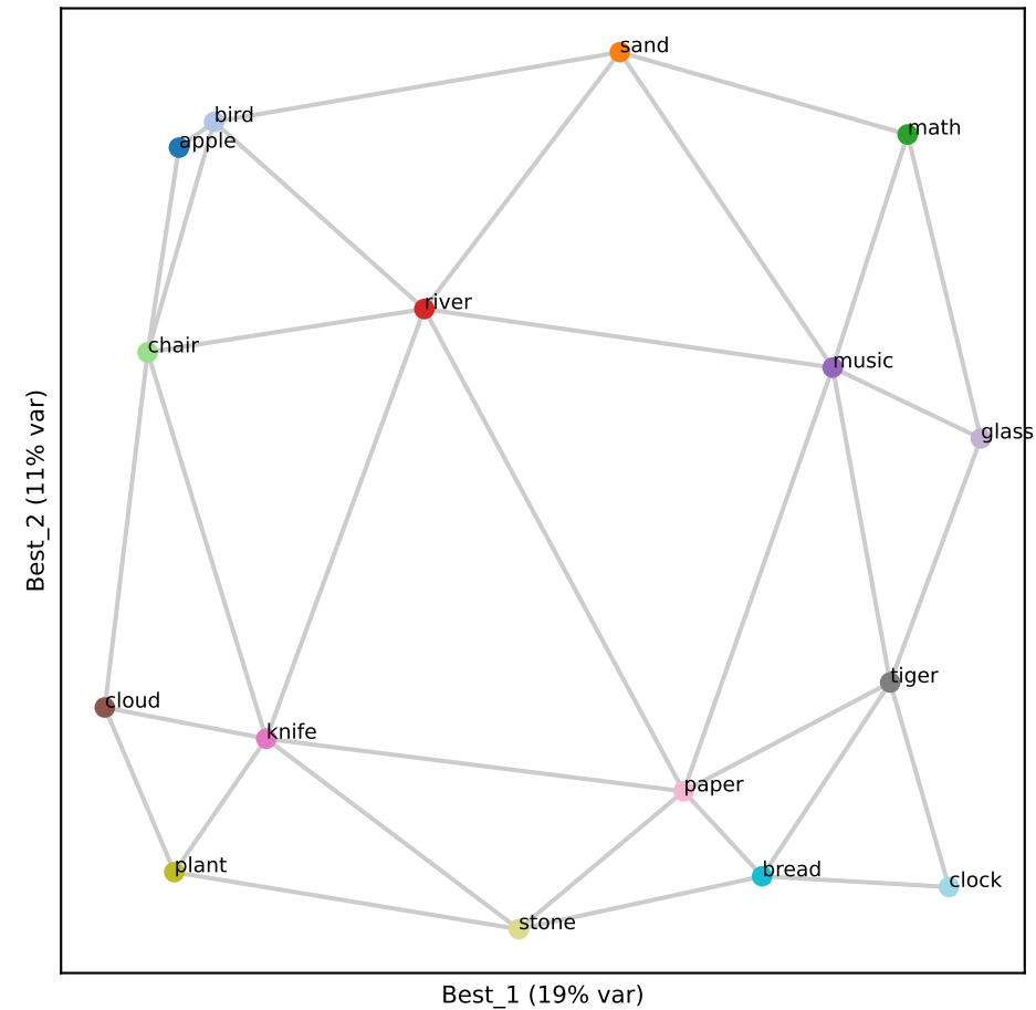
Qwen L32 (RSA 0.89)
