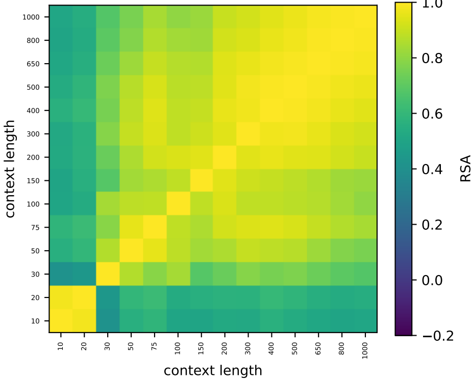
Qwen L27 perm-null 95%
