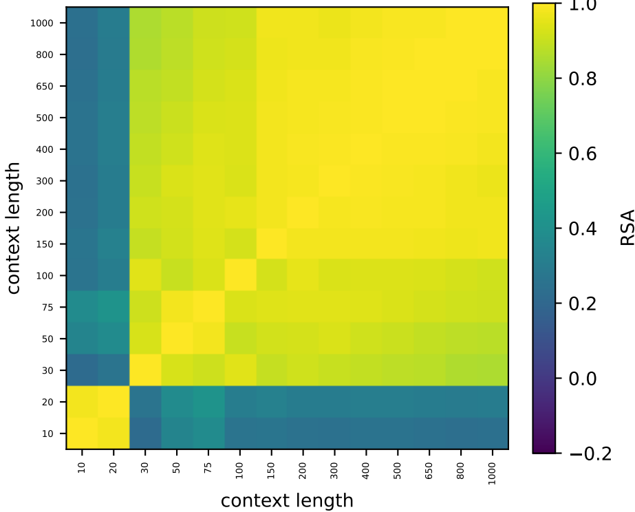
Qwen L14 perm-null 95%
