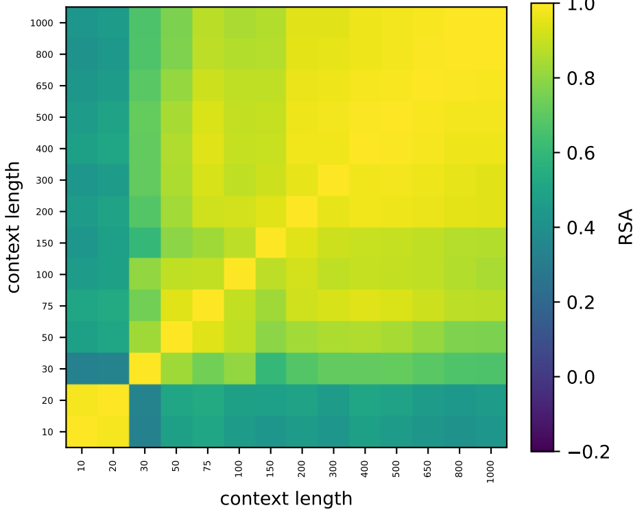
Qwen L26
