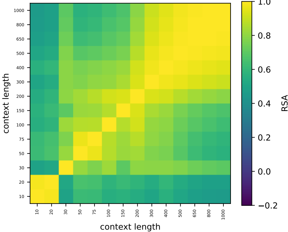
Qwen L32
