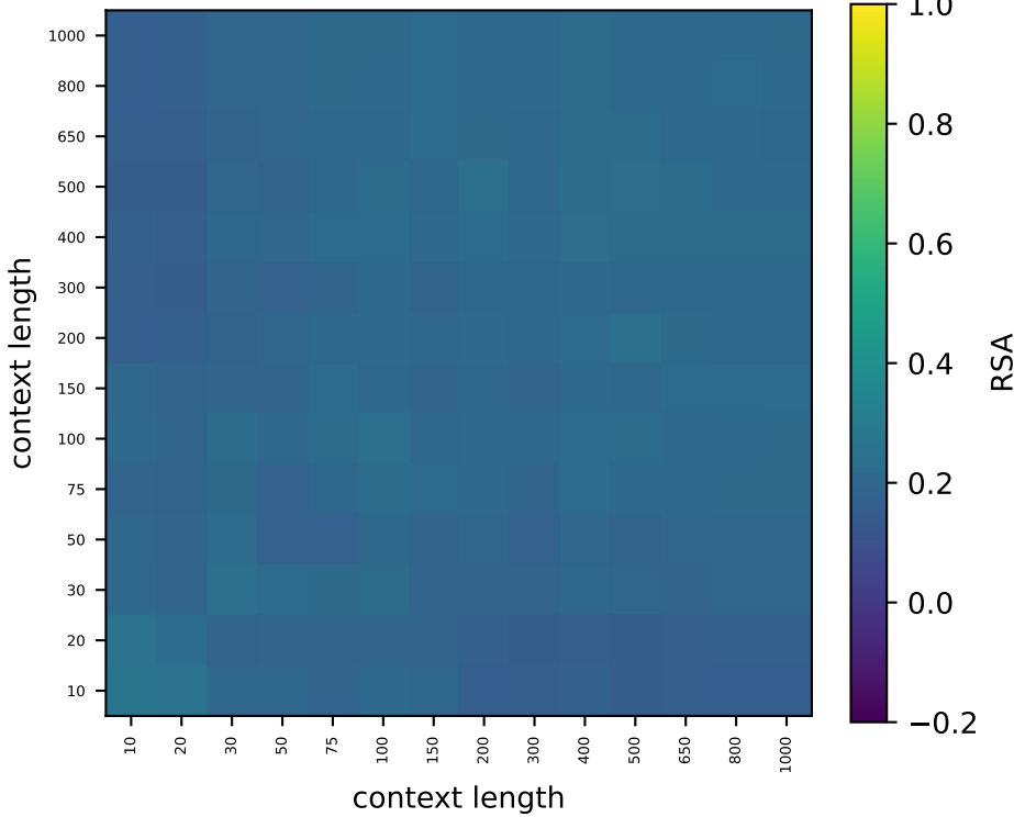
Qwen L23 perm-null 95%
