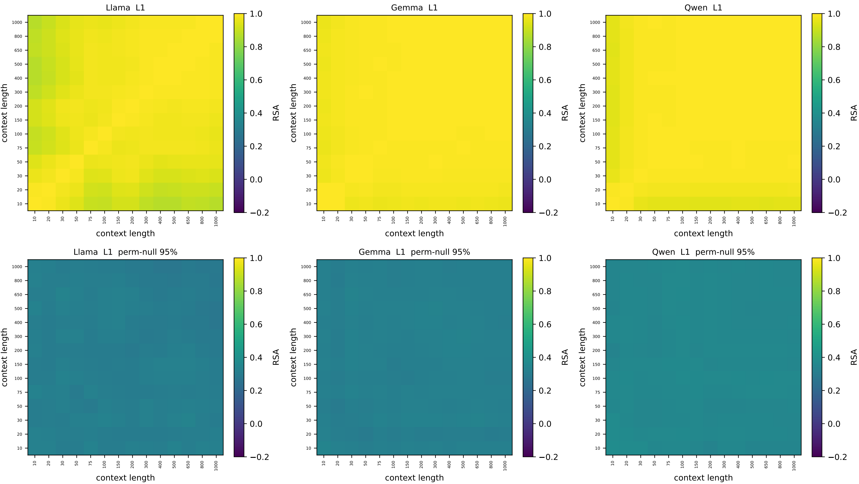
hex [v1] context-vs-context node-geometry RSA — relative depth 0.02 top: observed | bottom: node-label permutation null (95th pct)
