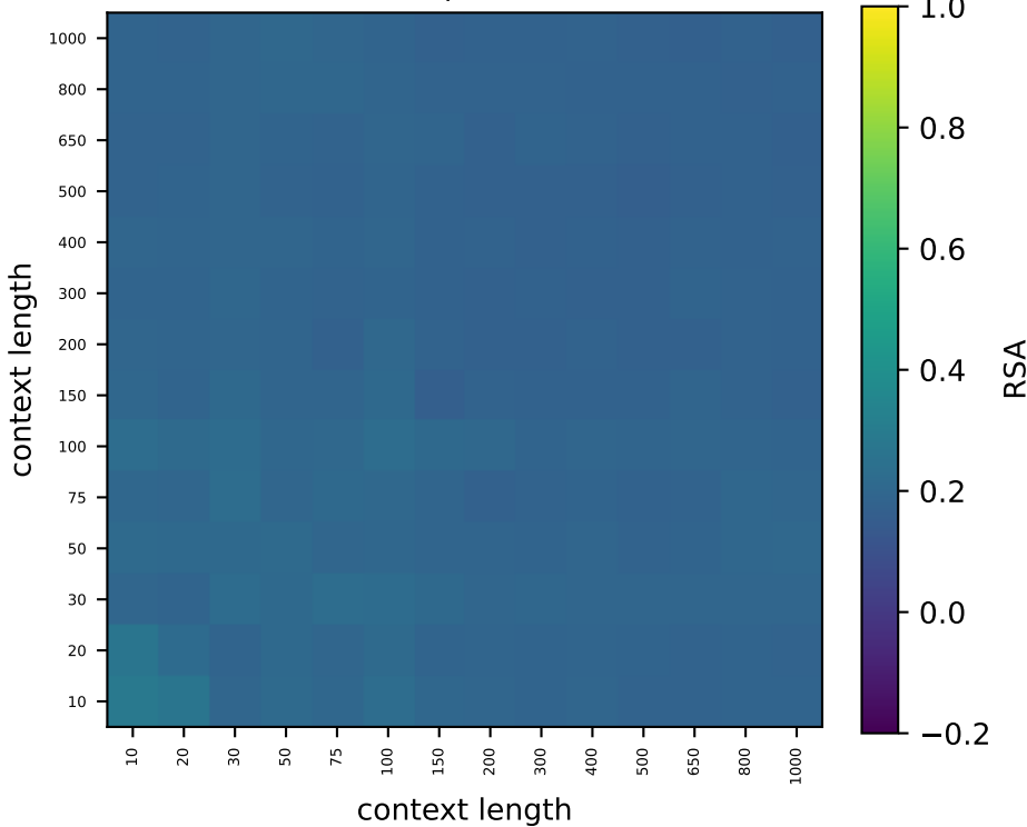
Qwen L13 perm-null 95%
