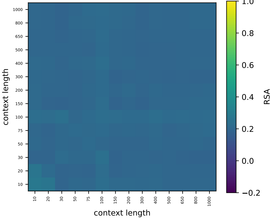
Qwen L16 perm-null 95%
