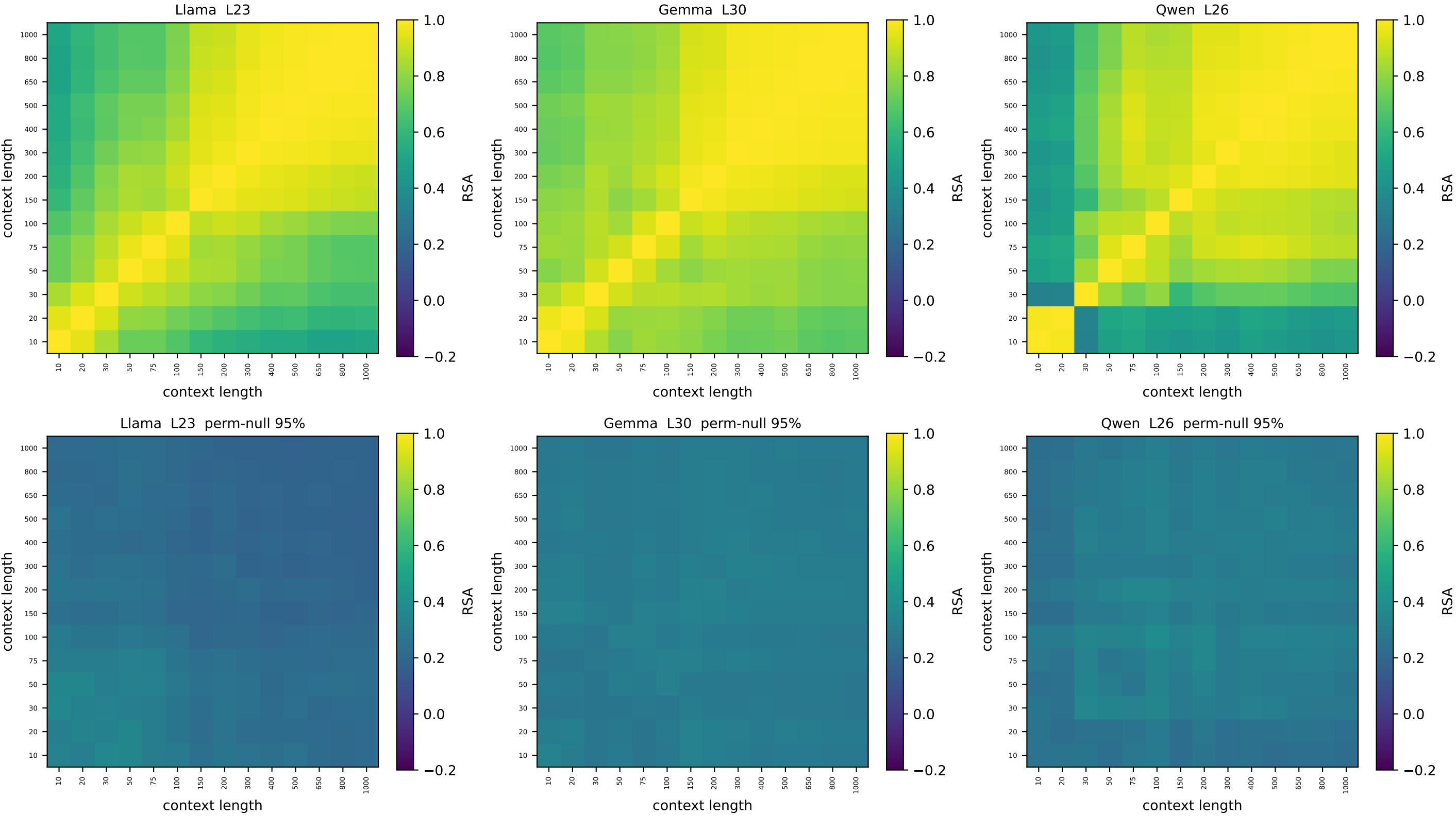
hex [v1] context-vs-context node-geometry RSA — relative depth 0.73 top: observed | bottom: node-label permutation null (95th pct)
