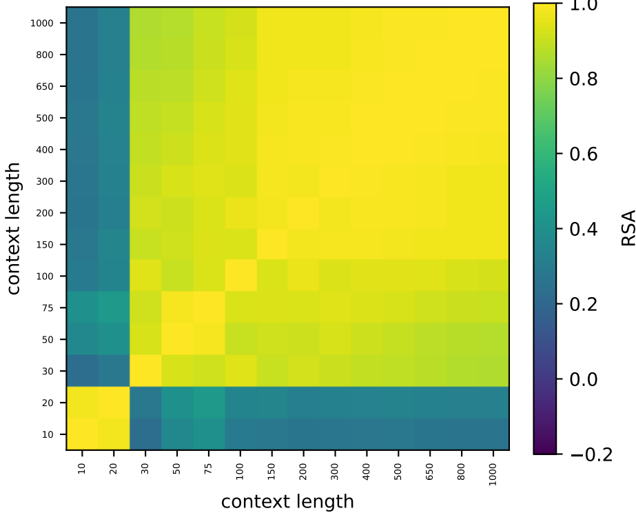
Qwen L16
