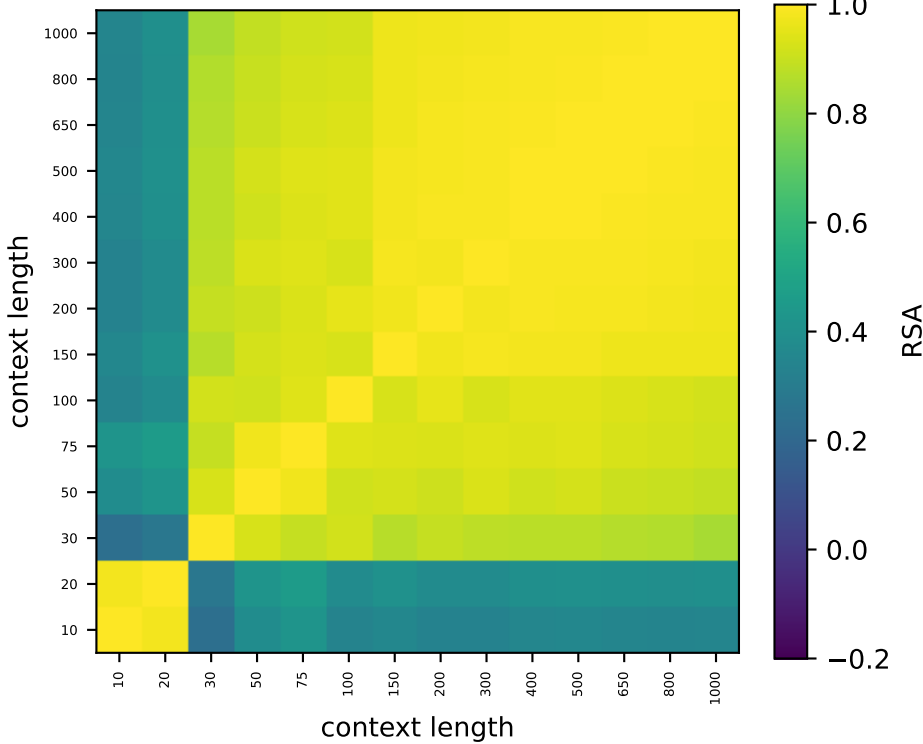
Qwen L19
