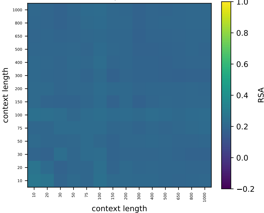
Qwen L17 perm-null 95%
