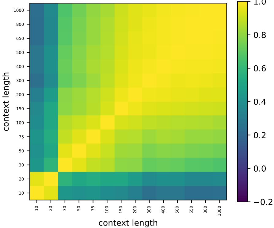
Gemma L16 perm-null 95%
