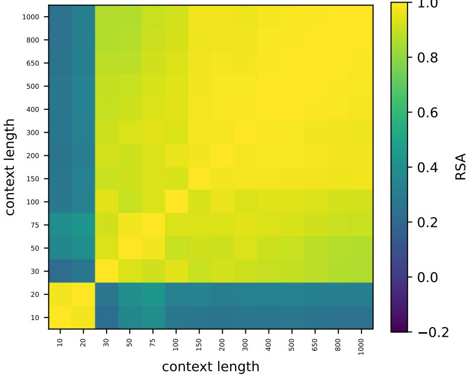
Qwen L15
