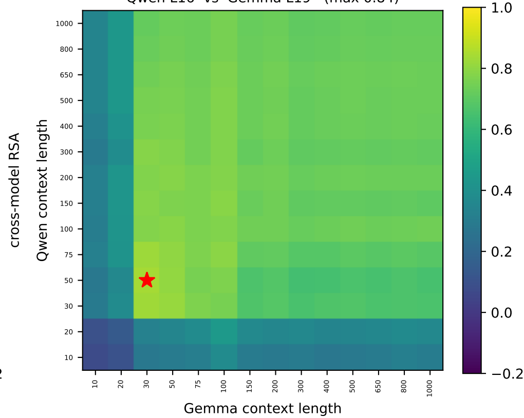
Qwen L16 vs Gemma L19 (max 0.84)
