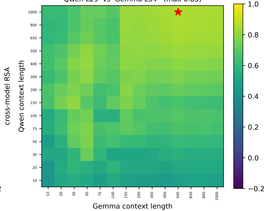
Qwen L29 vs Gemma L34 (max 0.85)
