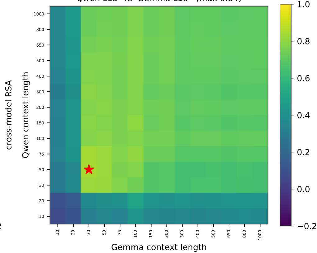
Qwen L15 vs Gemma L18 (max 0.84)
