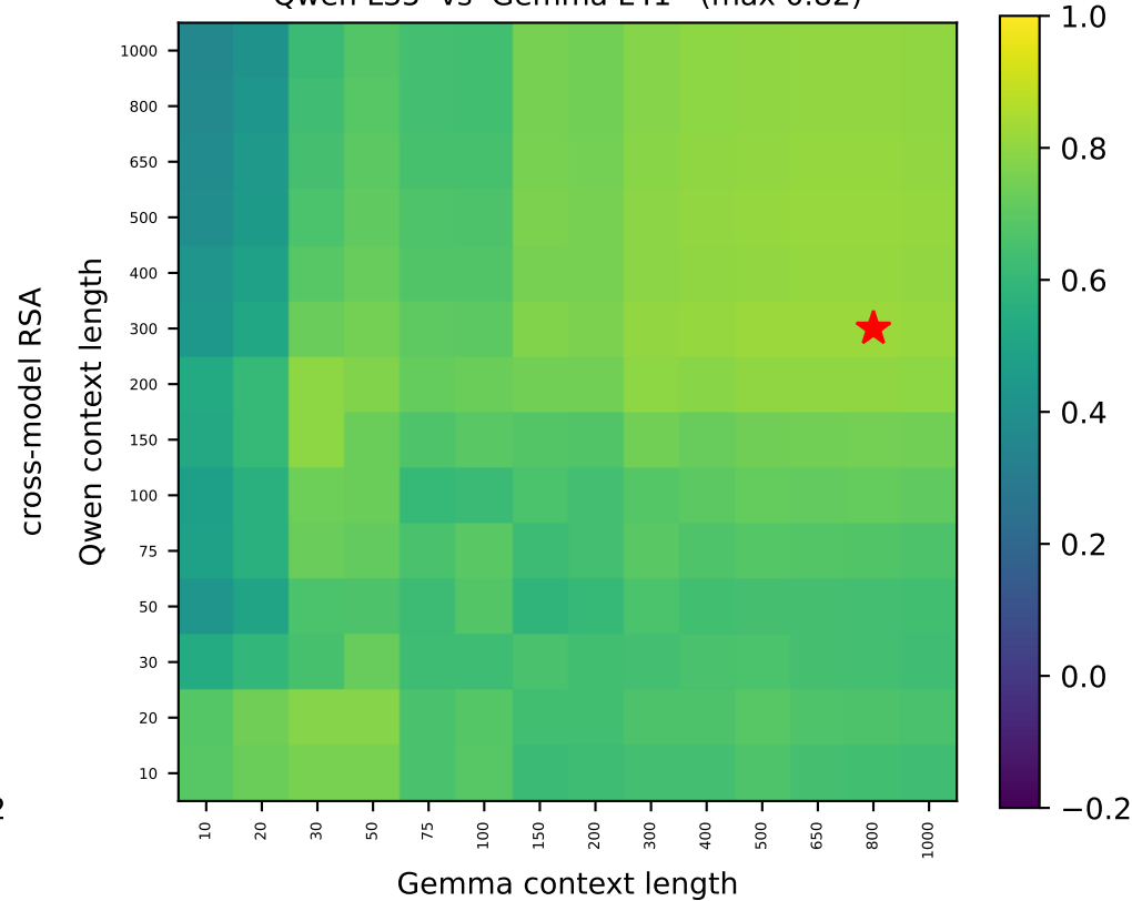
Qwen L35 vs Gemma L41 (max 0.82)
