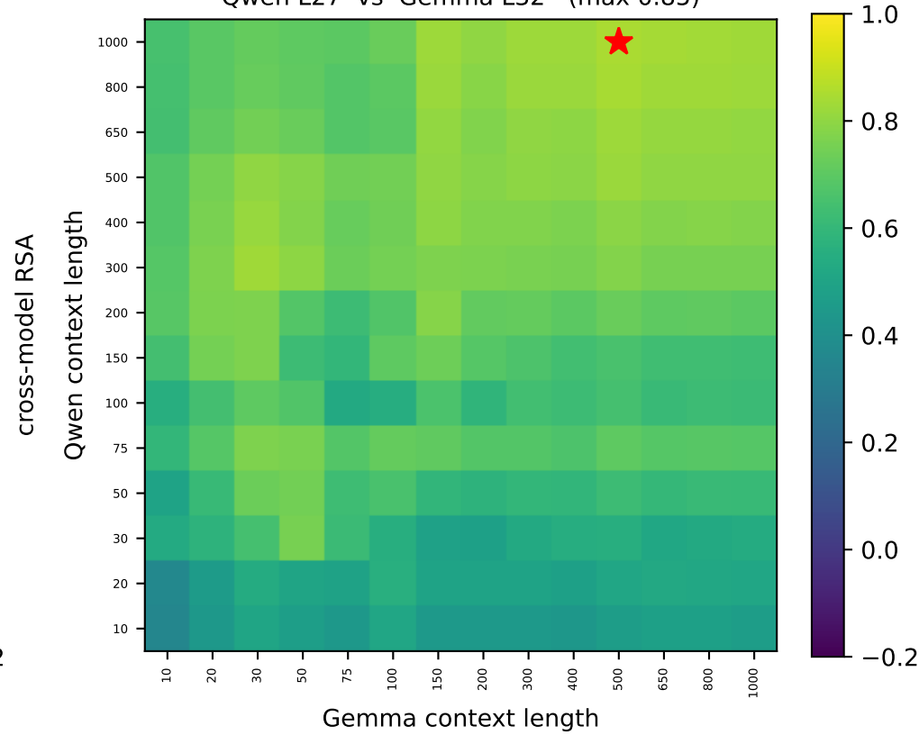
Qwen L27 vs Gemma L32 (max 0.85)
