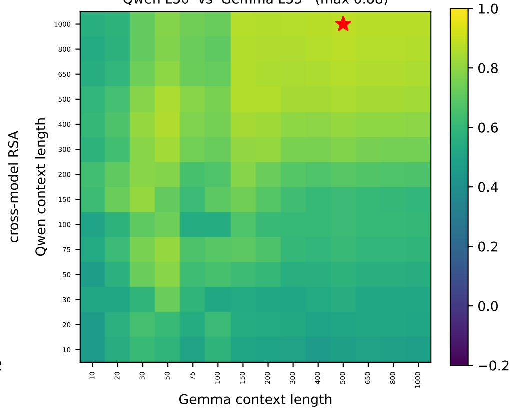
Qwen L30 vs Gemma L35 (max 0.88)
