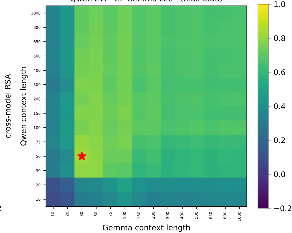
Qwen L17 vs Gemma L20 (max 0.83)
