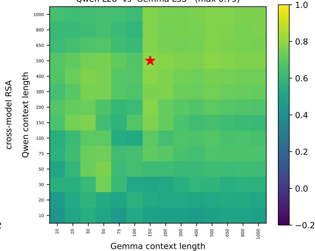
Qwen L28 vs Gemma L33 (max 0.79)
