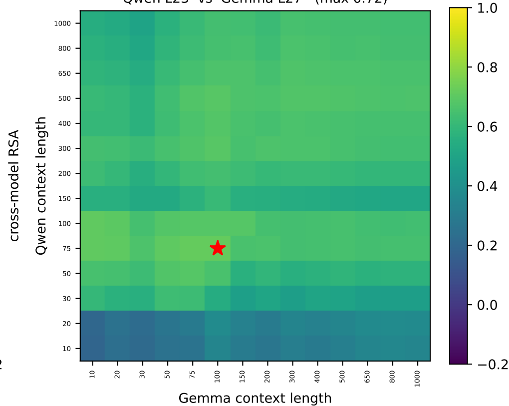
Qwen L23 vs Gemma L27 (max 0.72)
