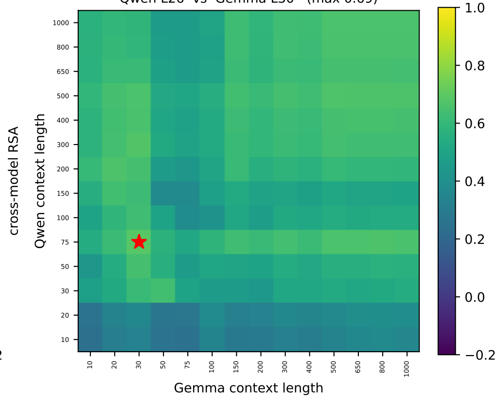
Qwen L26 vs Gemma L30 (max 0.69)
