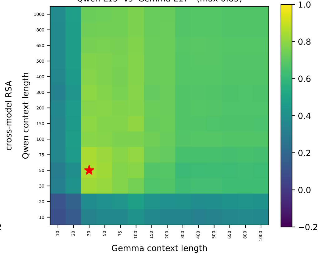
Qwen L15 vs Gemma L17 (max 0.85)
