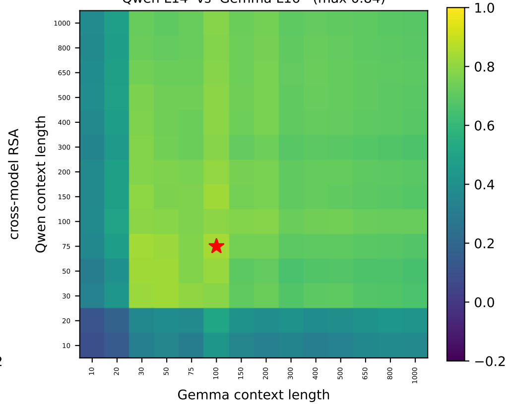
Qwen L14 vs Gemma L16 (max 0.84)
