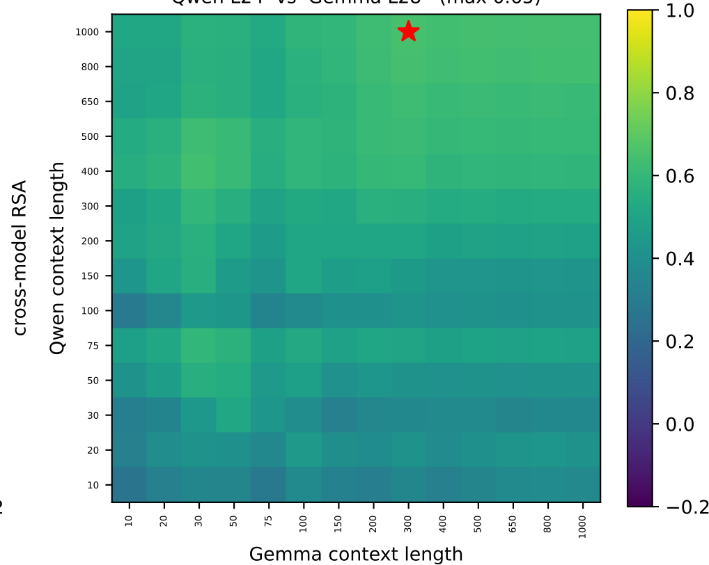
Qwen L24 vs Gemma L28 (max 0.65)
