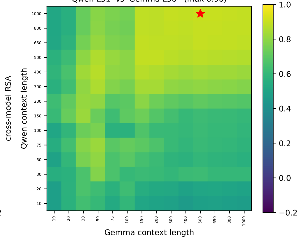
Qwen L31 vs Gemma L36 (max 0.90)
