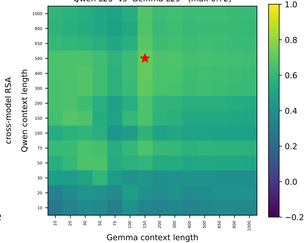
Qwen L25 vs Gemma L29 (max 0.72)
