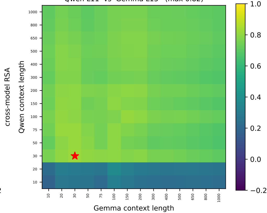
Qwen L11 vs Gemma L13 (max 0.82)
