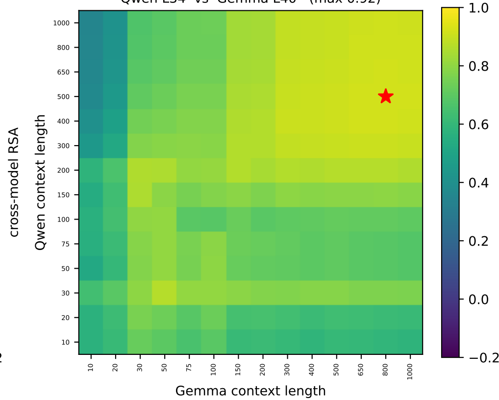
Qwen L34 vs Gemma L40 (max 0.92)
