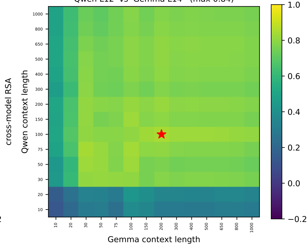
Qwen L12 vs Gemma L14 (max 0.84)
