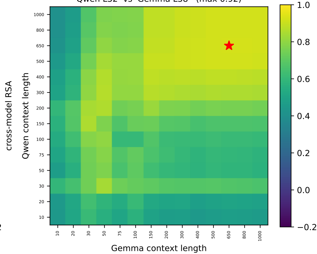
Qwen L32 vs Gemma L38 (max 0.92)
