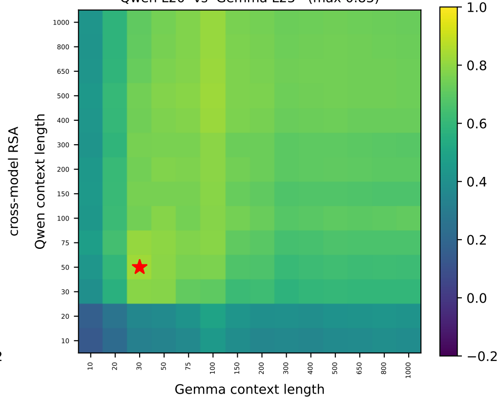
Qwen L20 vs Gemma L23 (max 0.83)
