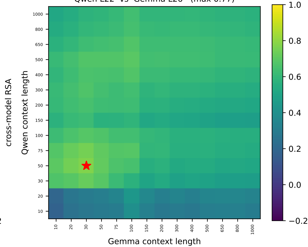
Qwen L22 vs Gemma L26 (max 0.77)
