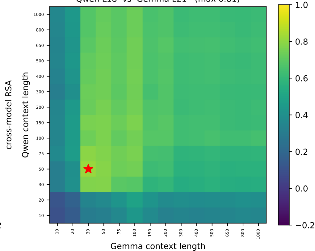
Qwen L18 vs Gemma L21 (max 0.81)
