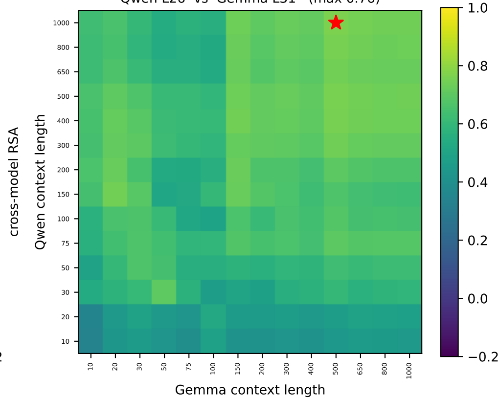
Qwen L26 vs Gemma L31 (max 0.76)
