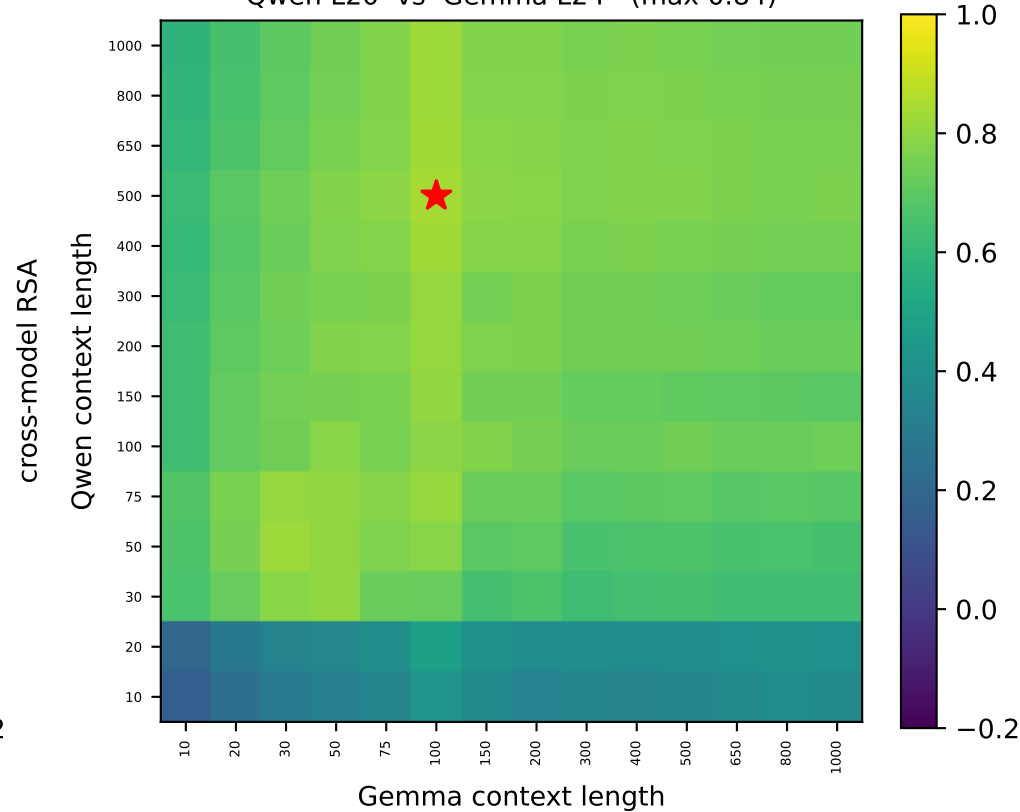
Qwen L20 vs Gemma L24 (max 0.84)
