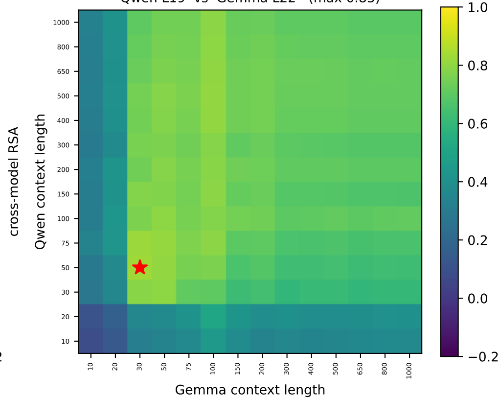
Qwen L19 vs Gemma L22 (max 0.83)
