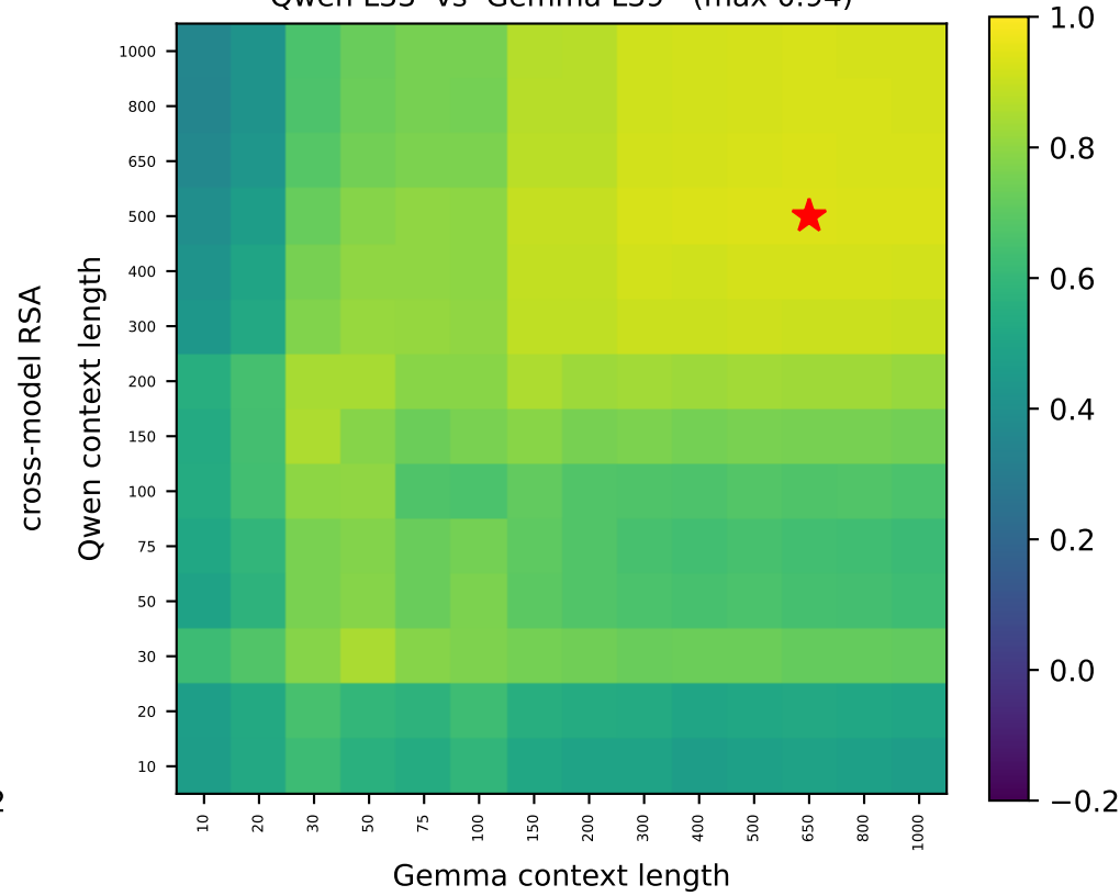
Qwen L33 vs Gemma L39 (max 0.94)
