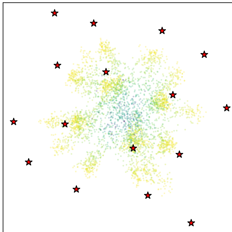
Qwen L34: recovered from acts ( R^2=0.87 )
