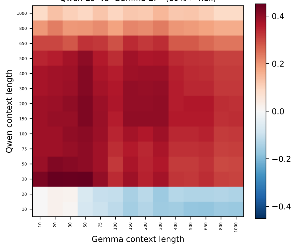
Qwen L6 vs Gemma L7 (89% > null)
