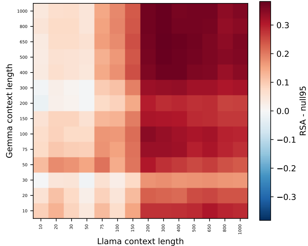
Gemma L11 vs Llama L8 (97% > null)
