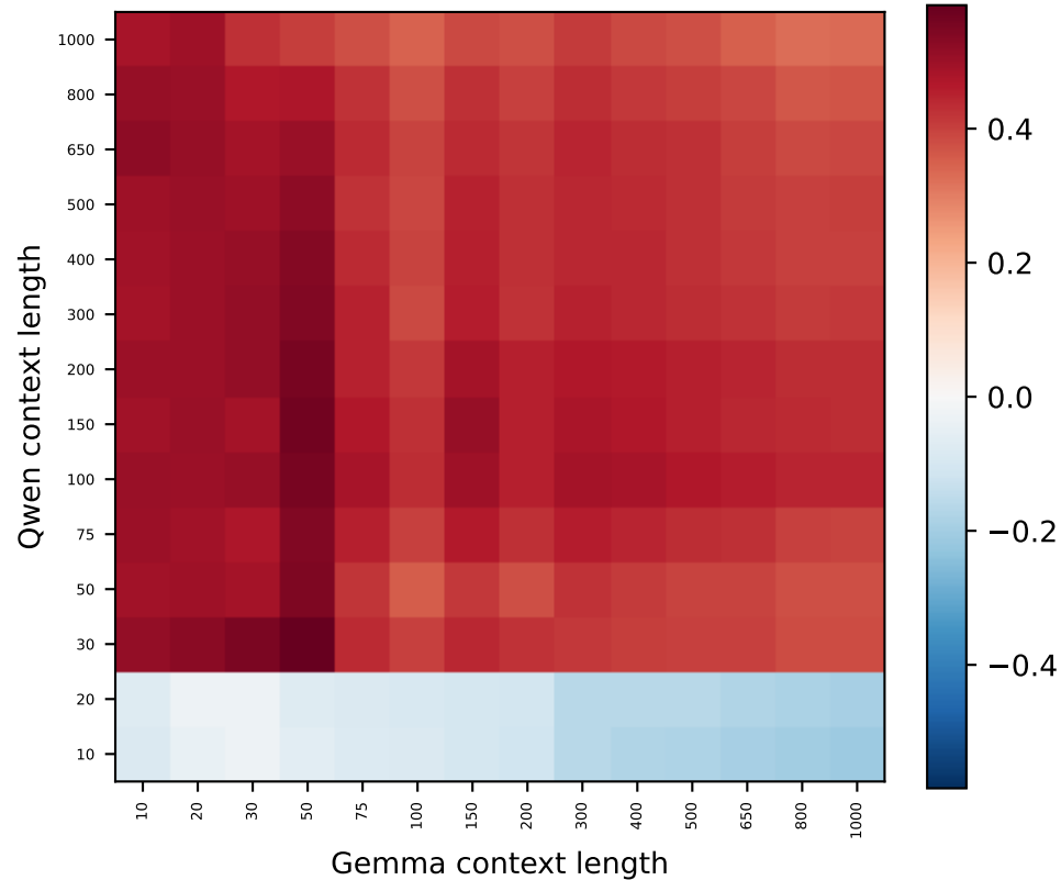
Qwen L8 vs Gemma L9 (86% > null)
