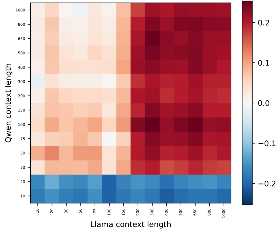
Qwen L9 vs Llama L8 (84% > null)
