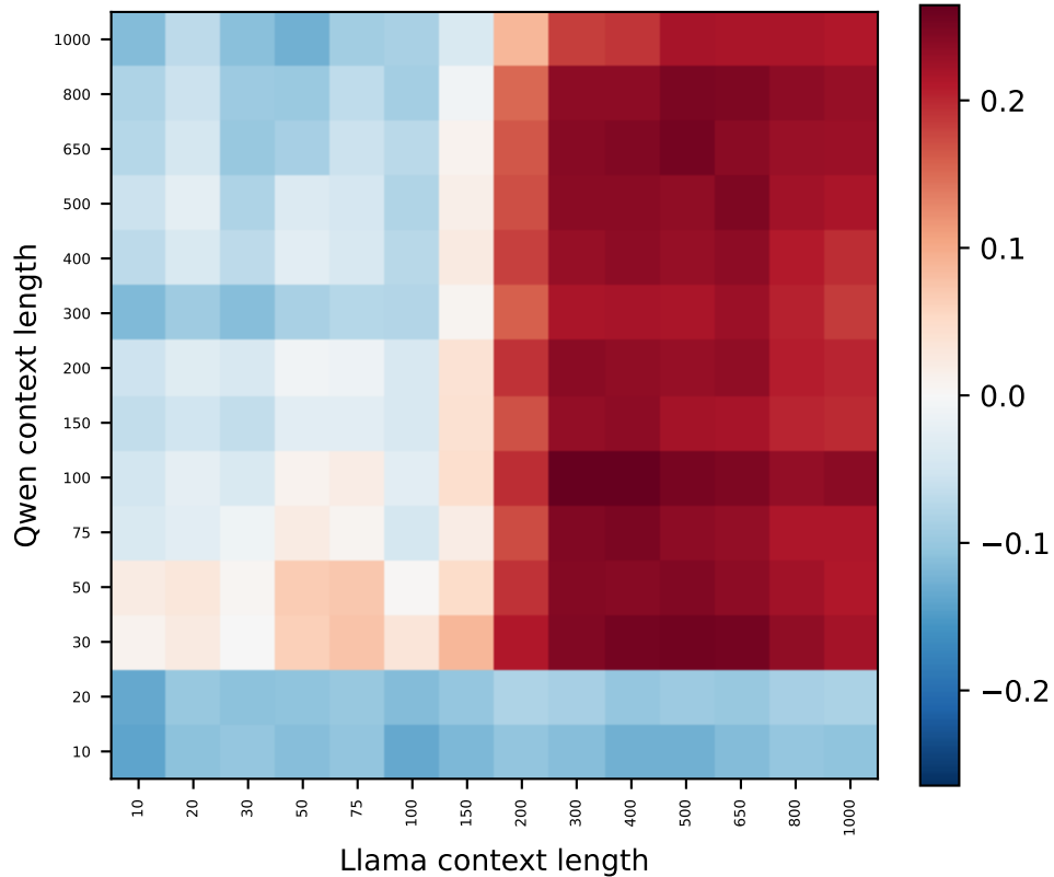
Qwen L8 vs Llama L7 (56% > null)
