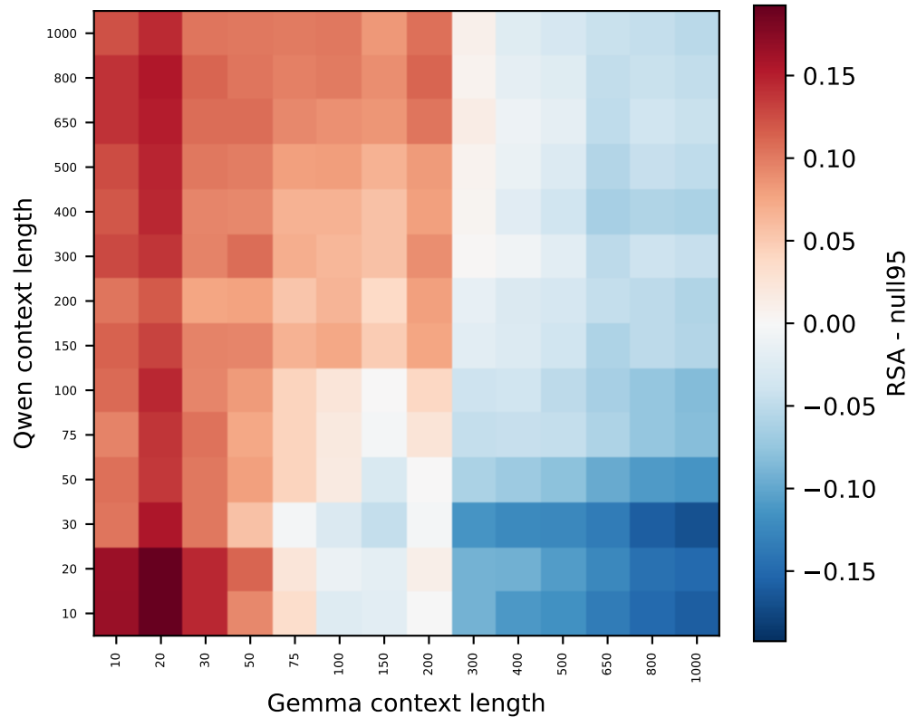
Qwen L4 vs Gemma L5 (55% > null)
