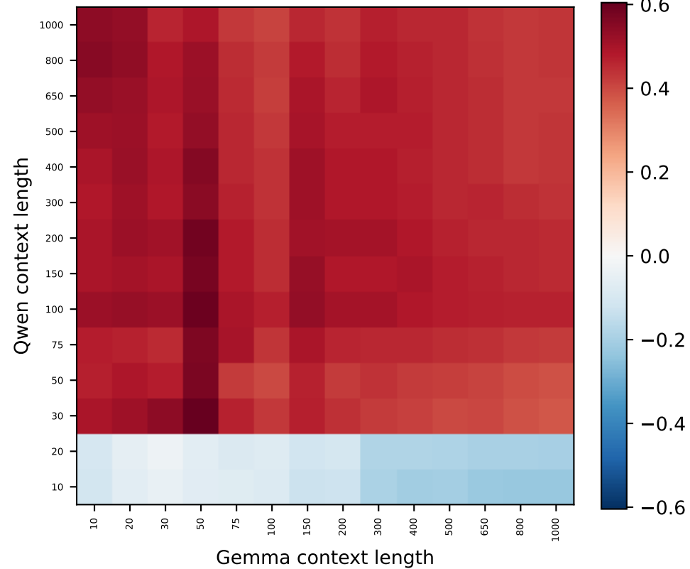
Qwen L9 vs Gemma L10 (86% > null)
