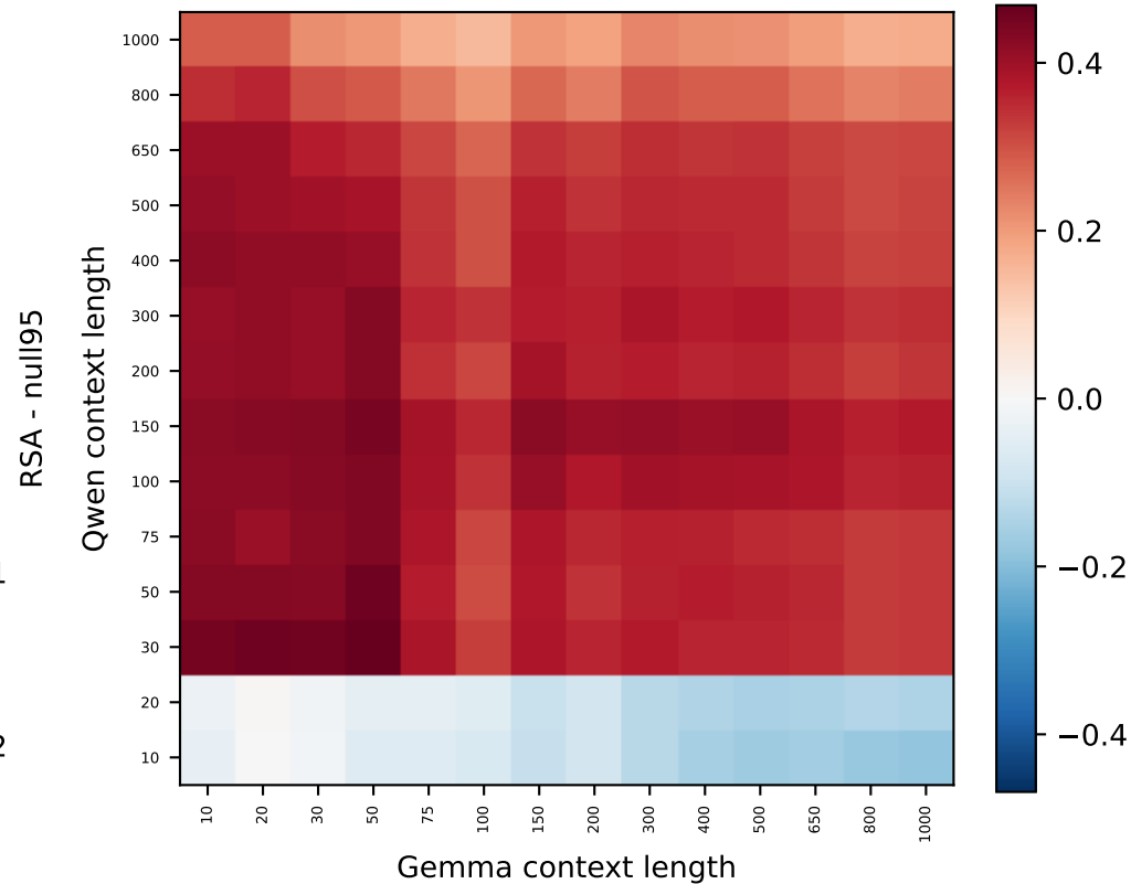
Qwen L7 vs Gemma L8 (86% > null)
