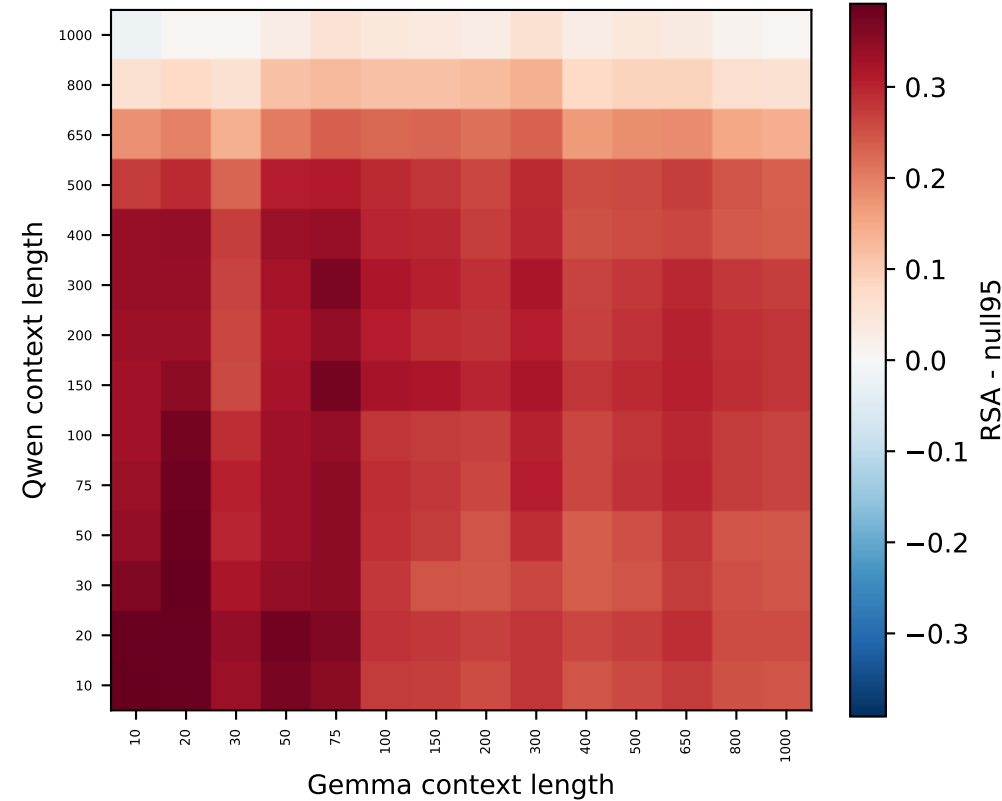
Qwen L5 vs Gemma L6 (99% > null)
