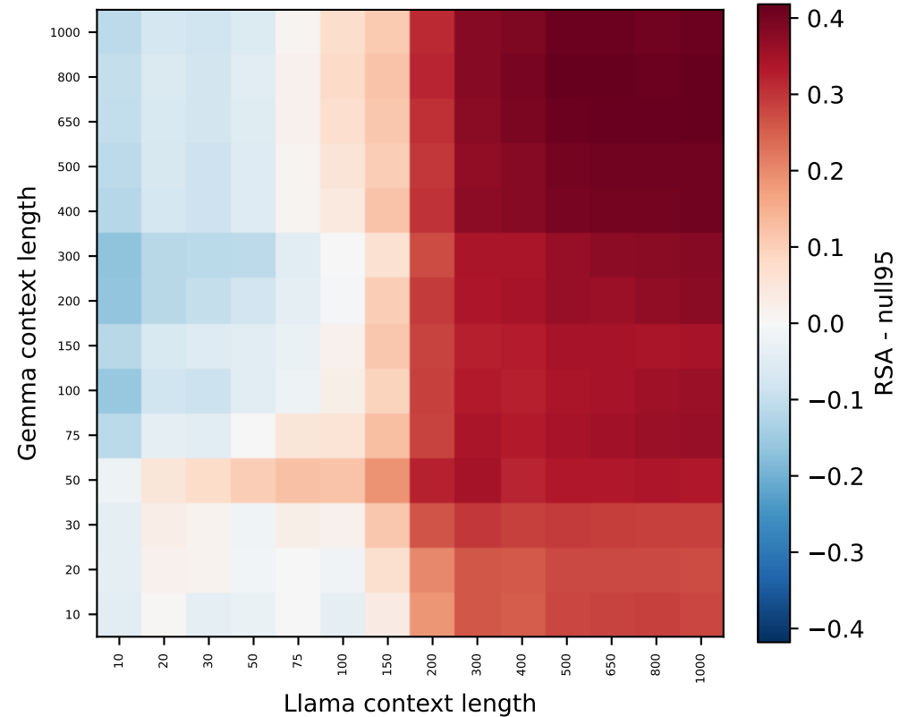
Gemma L8 vs Llama L6 (71% > null)
