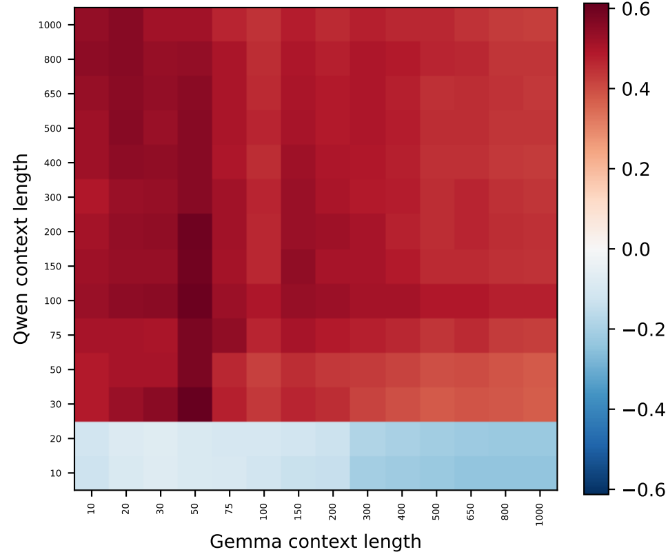
Qwen L9 vs Gemma L11 (86% > null)
