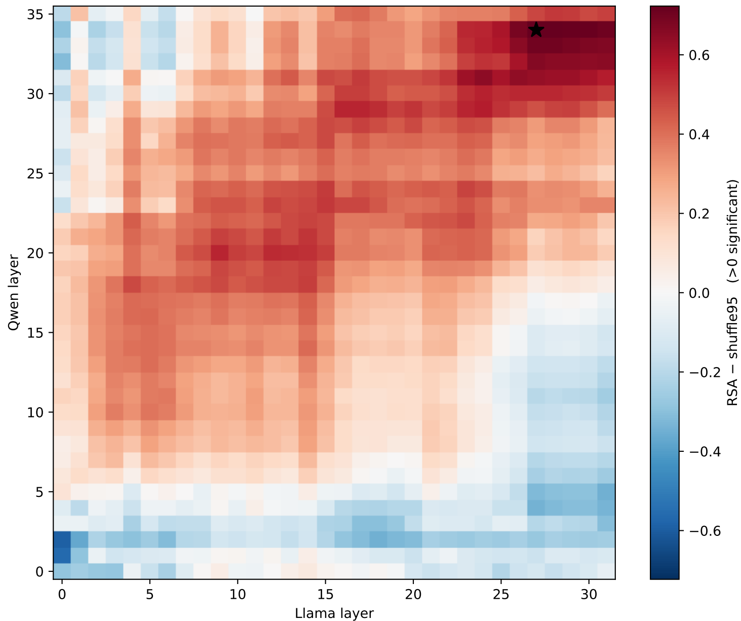
ring [v1] Qwen vs Llama: RSA – per-cell shuffle-null95 red = above shuffle null; 75% of cells > null
