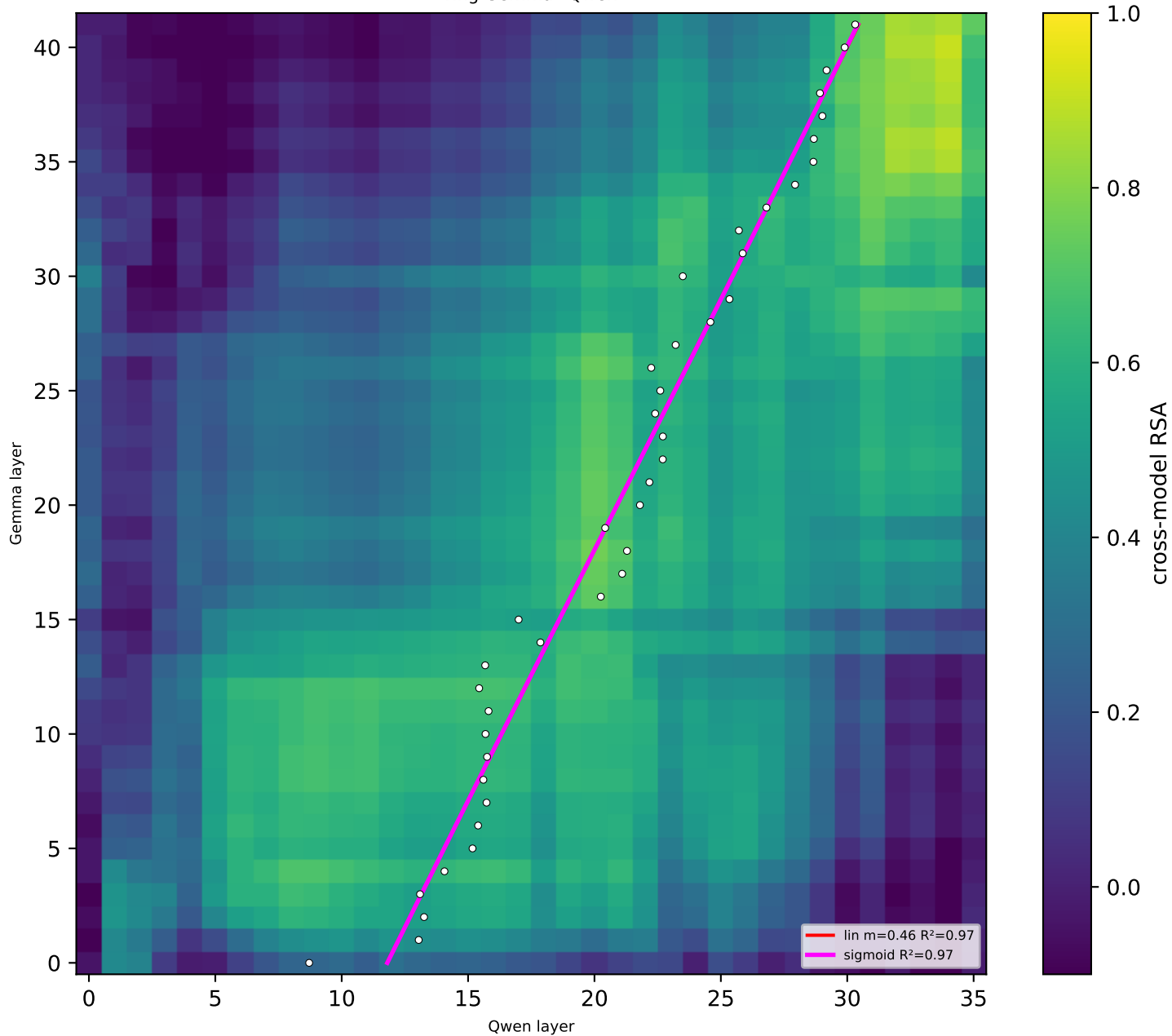
ring Gemma×Qwen
