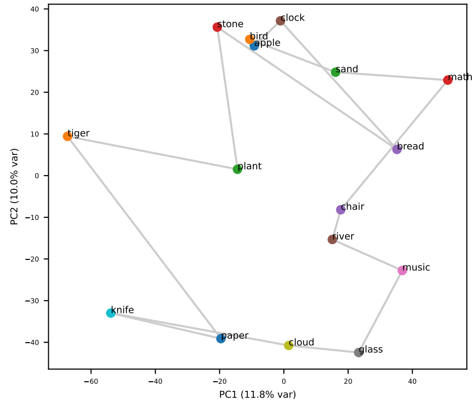
Qwen L24 (grid RSA=+0.31)
