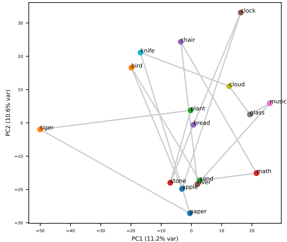
Gemma L12 (grid RSA=+0.02)
