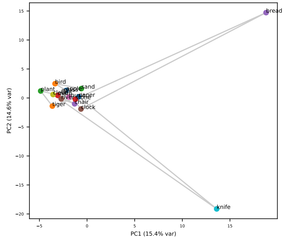
Qwen L2 (grid RSA=+0.01)
