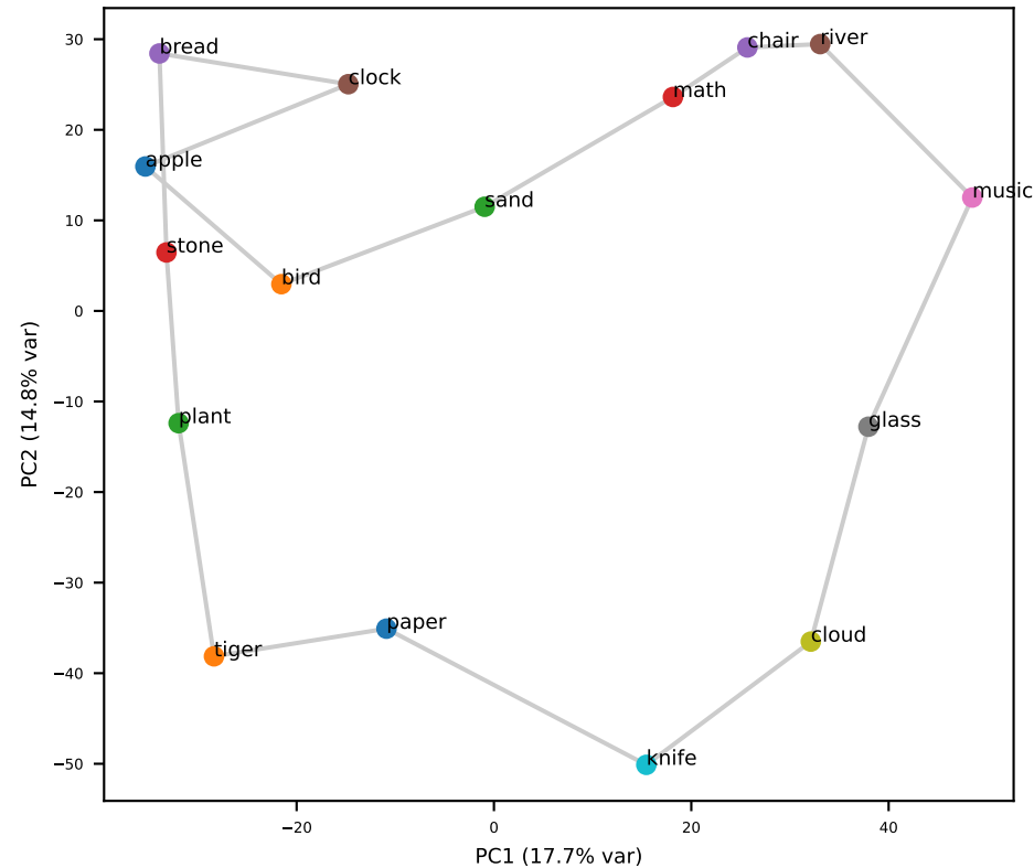
Gemma L21 (grid RSA=+0.62)
