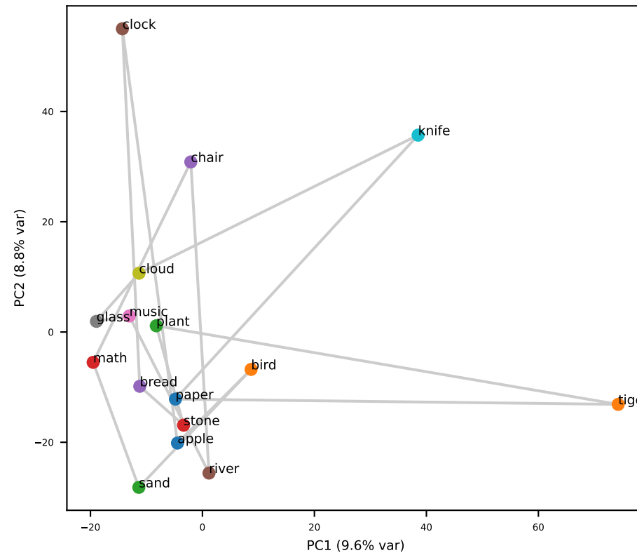
Gemma L3 (grid RSA=+0.00)
