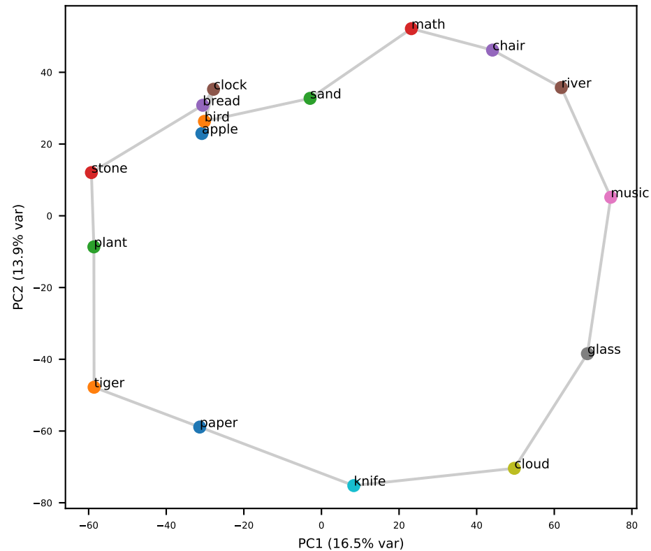
Gemma L29 (grid RSA=+0.59)
