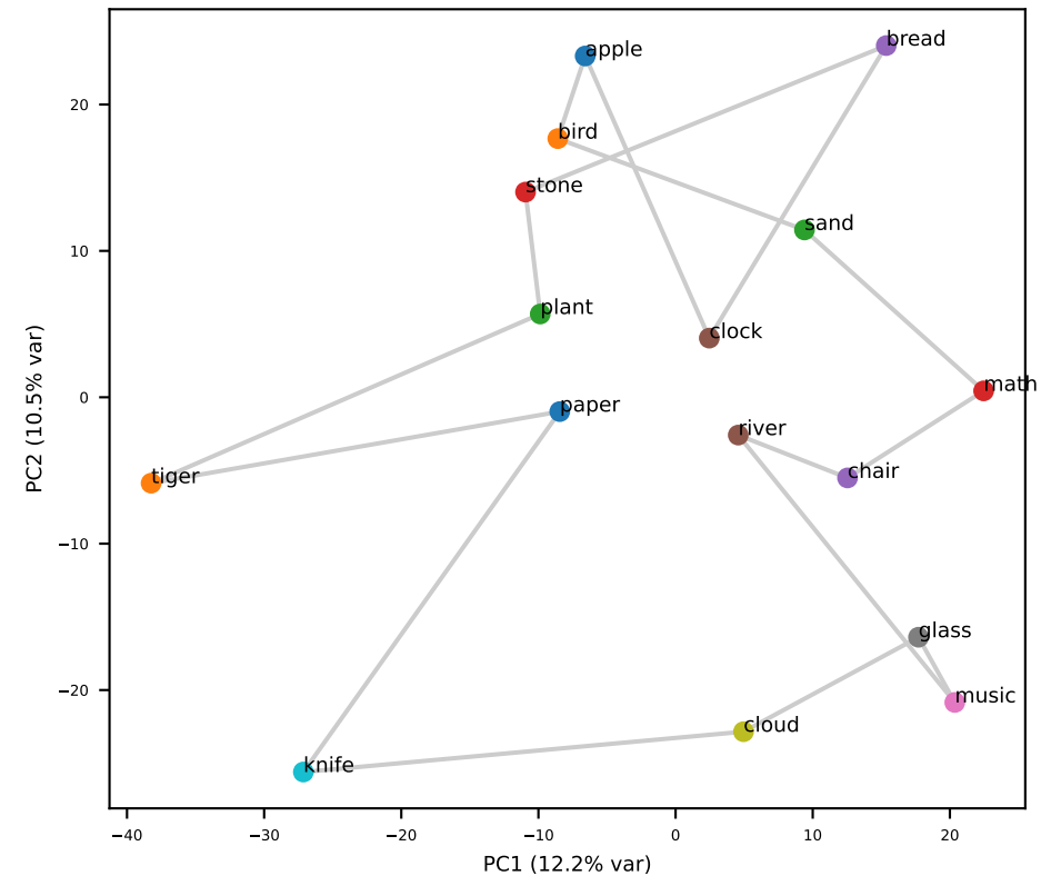
Qwen L20 (grid RSA=+0.39)
