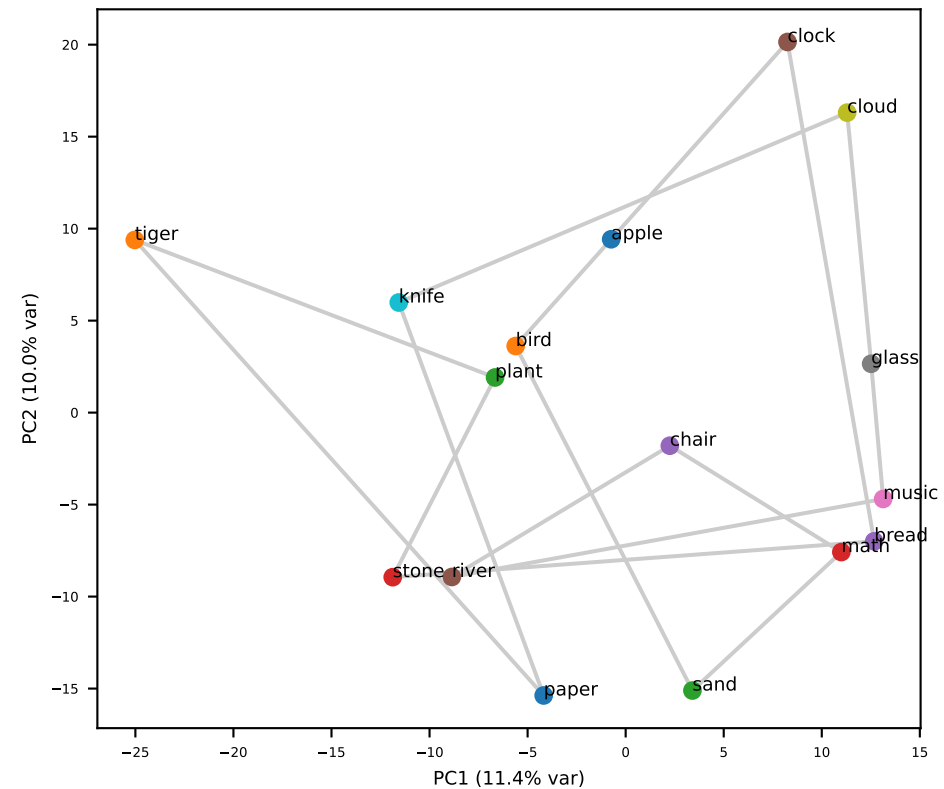
Qwen L14 (grid RSA=+0.03)
