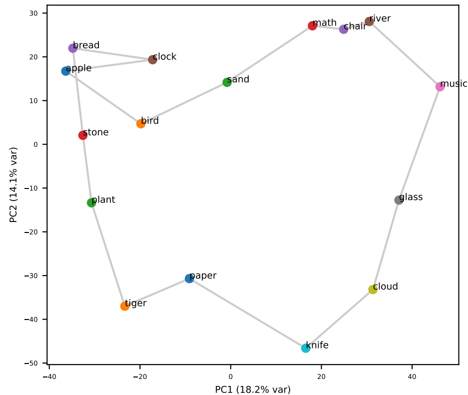
Gemma L22 (grid RSA=+0.64)
