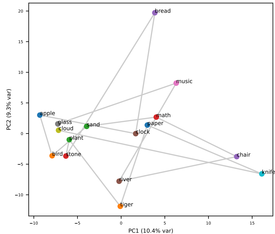
Qwen L4 (grid RSA=-0.03)
