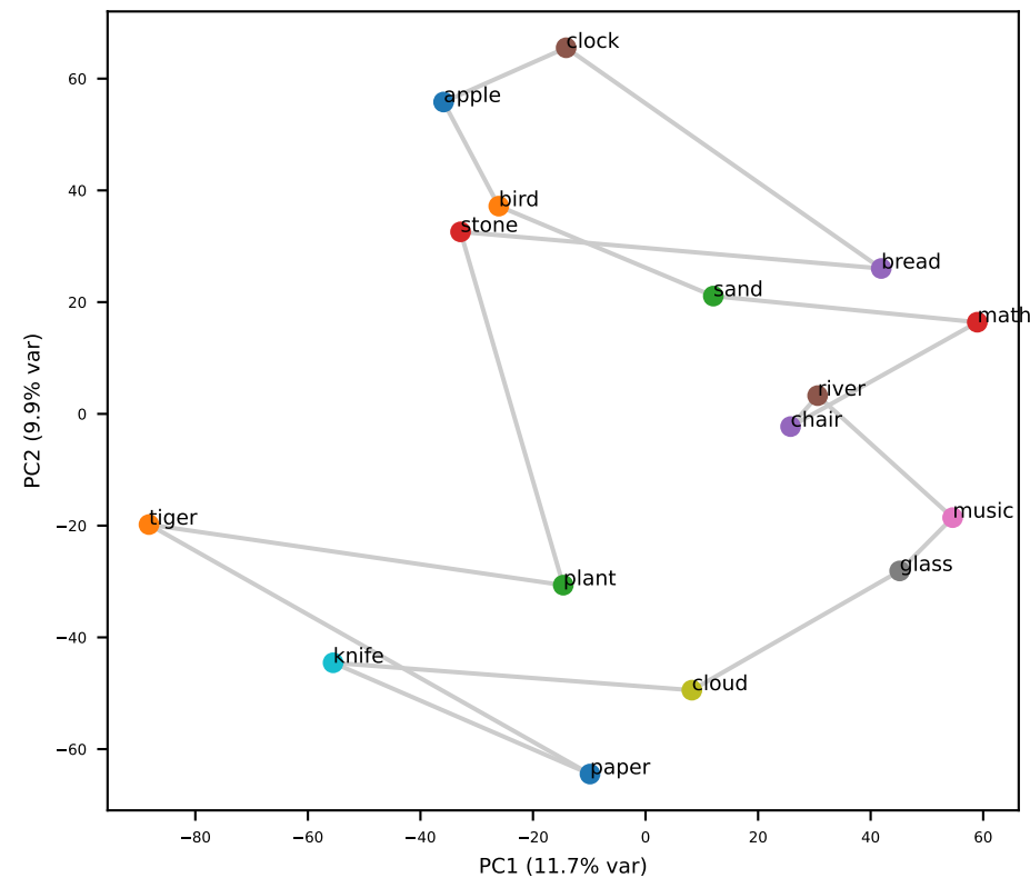
Qwen L27 (grid RSA=+0.33)
