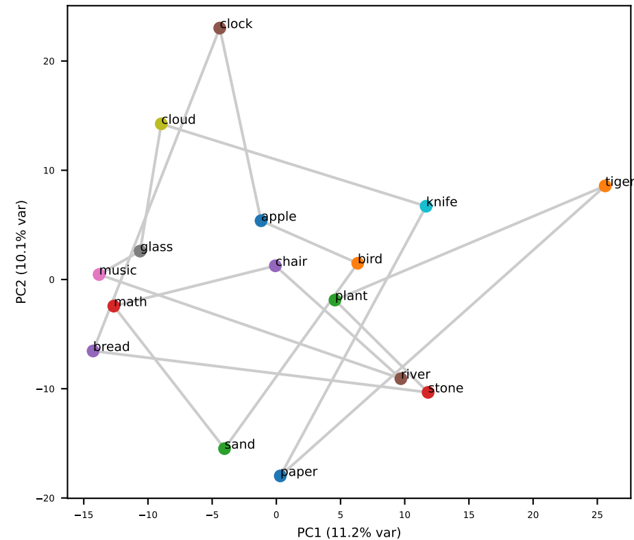
Qwen L12 (grid RSA=-0.07)
