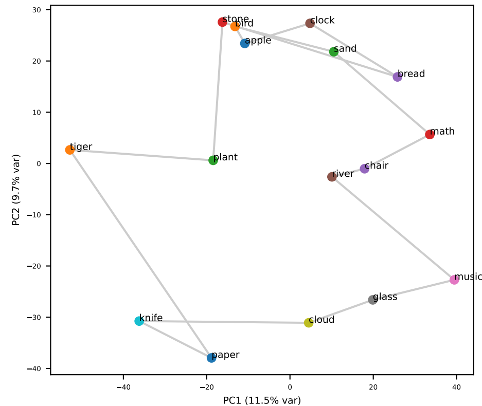
Qwen L23 (grid RSA=+0.34)
