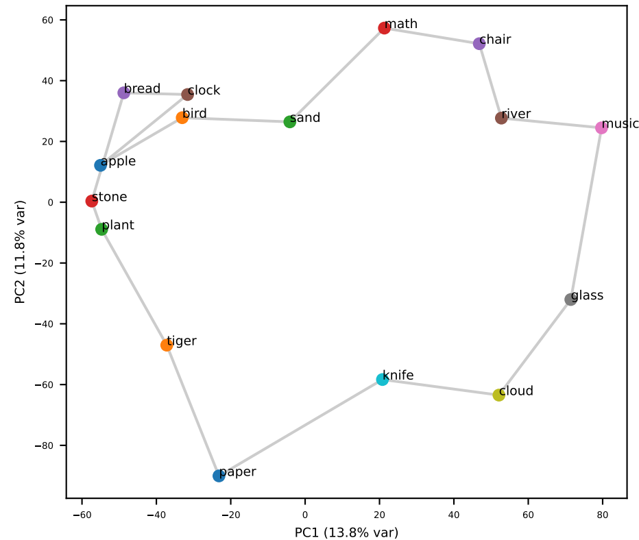
Gemma L31 (grid RSA=+0.58)
