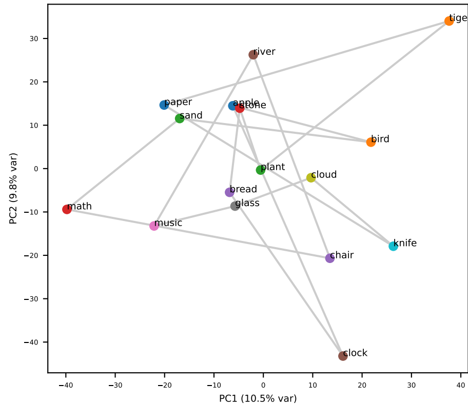
Gemma L7 (grid RSA=+0.03)
