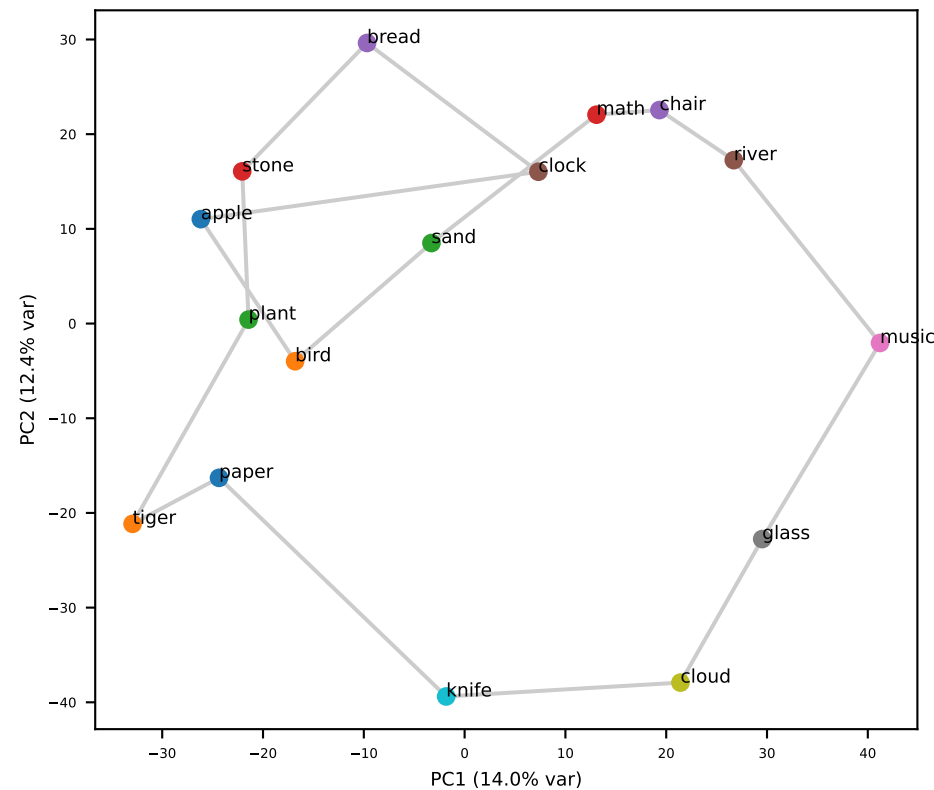
Gemma L16 (grid RSA=+0.41)
