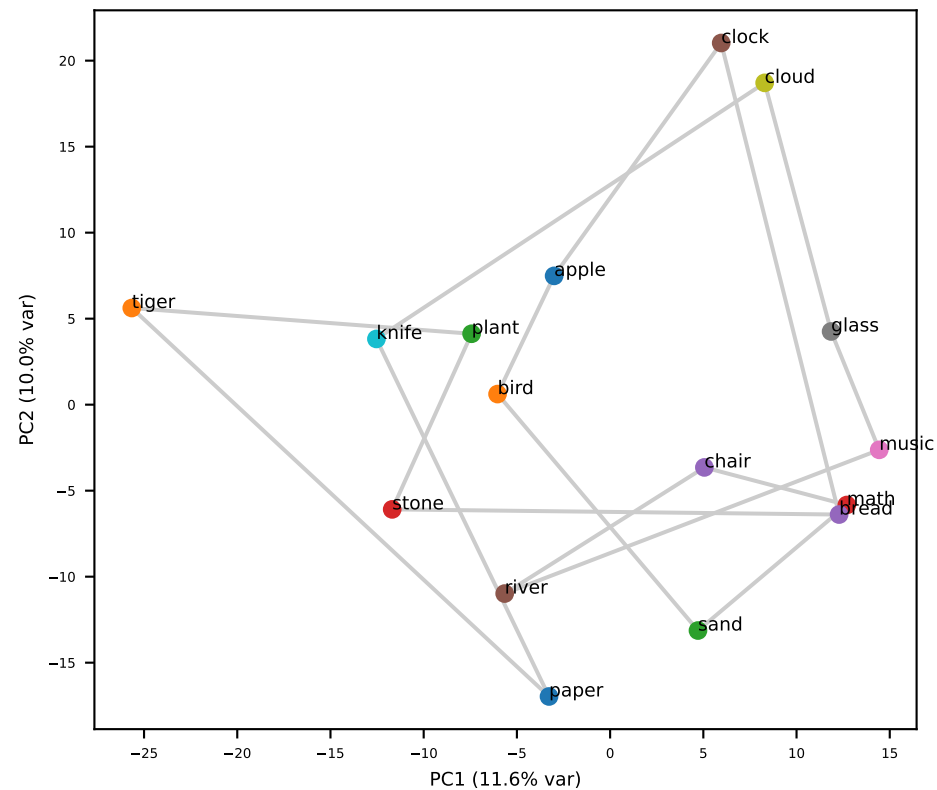
Qwen L16 (grid RSA=+0.11)
