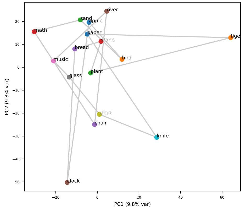
Gemma L4 (grid RSA=-0.01)
