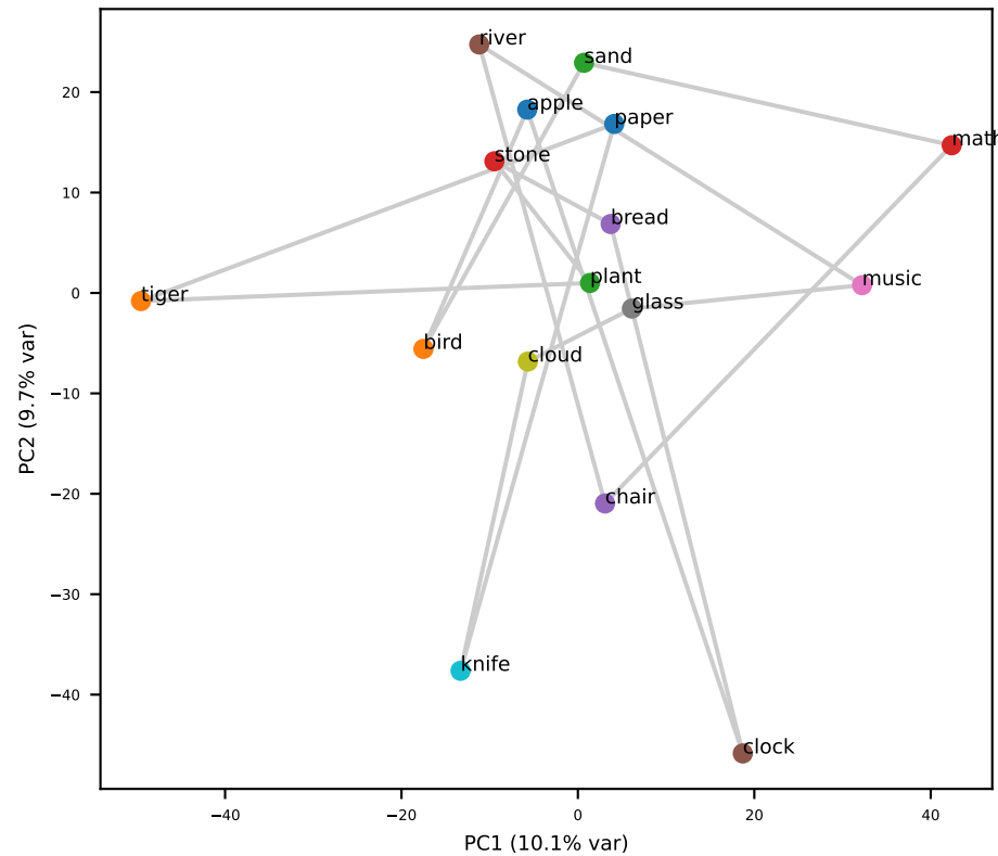
Gemma L6 (grid RSA=+0.04)
