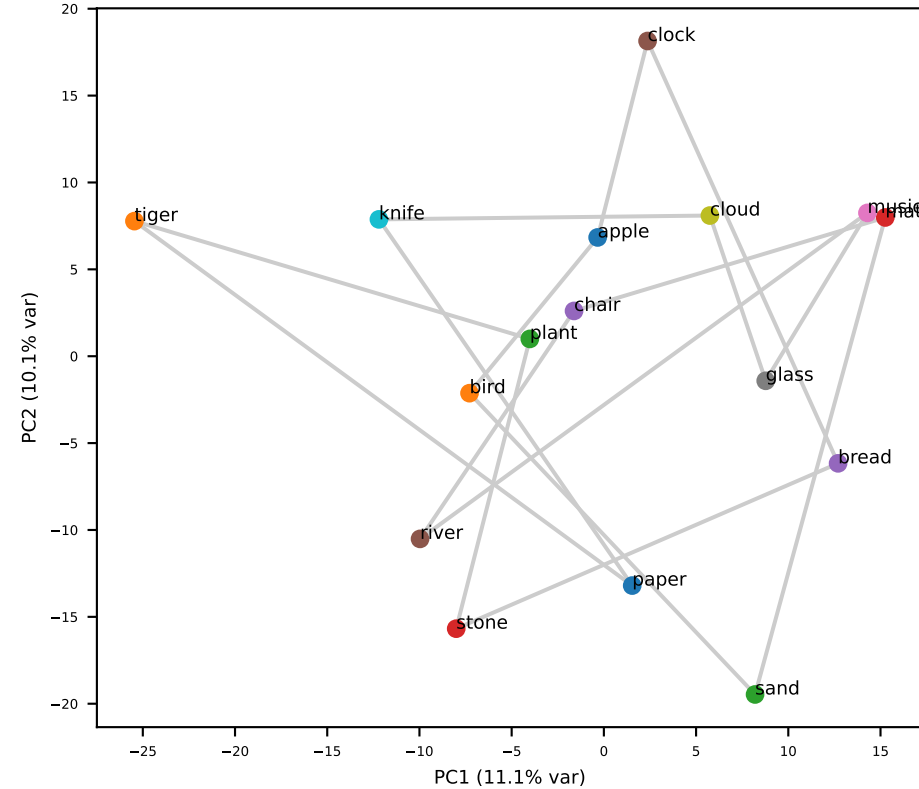
Qwen L11 (grid RSA=-0.08)
