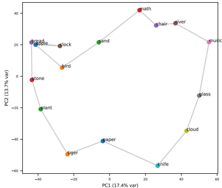
Gemma L27 (grid RSA=+0.66)
