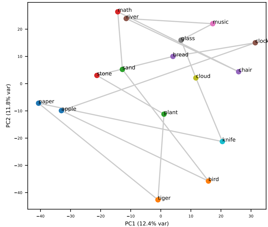
Gemma L15 (grid RSA=+0.08)
