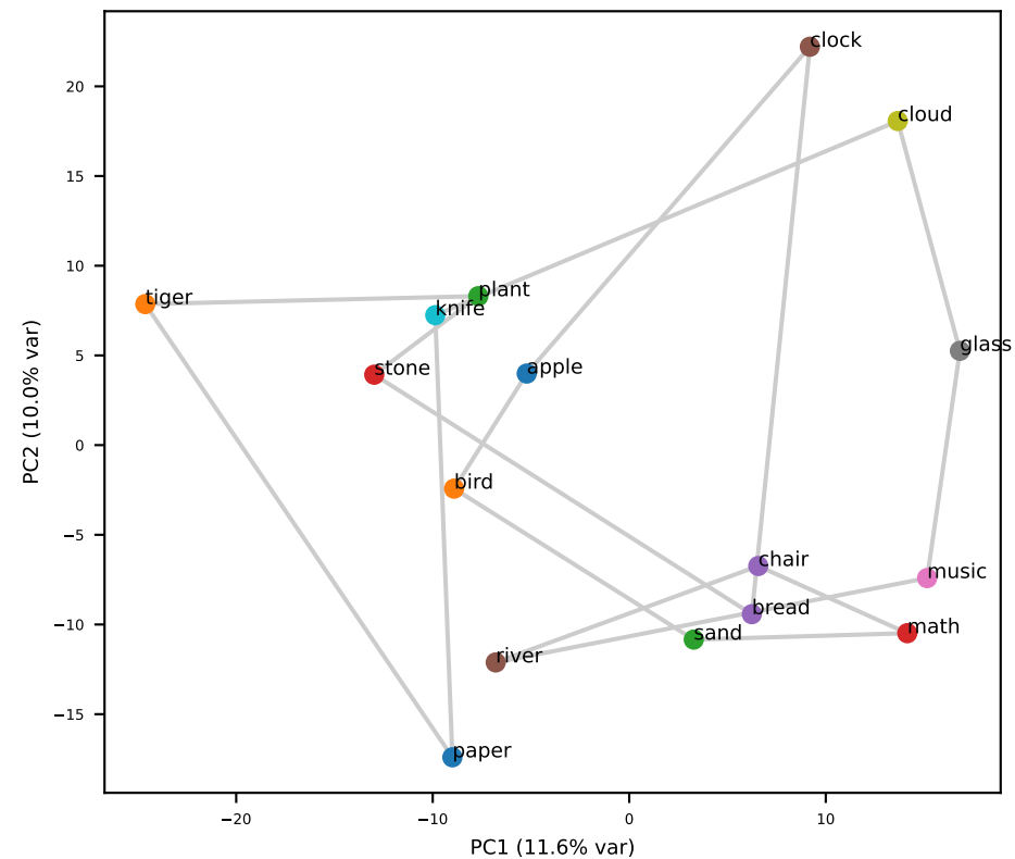
Qwen L18 (grid RSA=+0.24)
