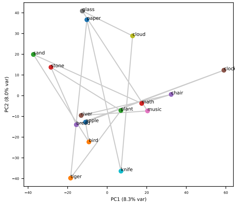
Gemma L0 (grid RSA=-0.14)
