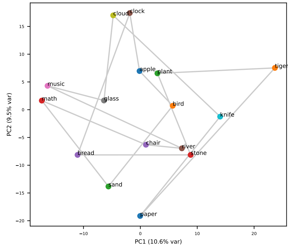
Qwen L9 (grid RSA=-0.04)
