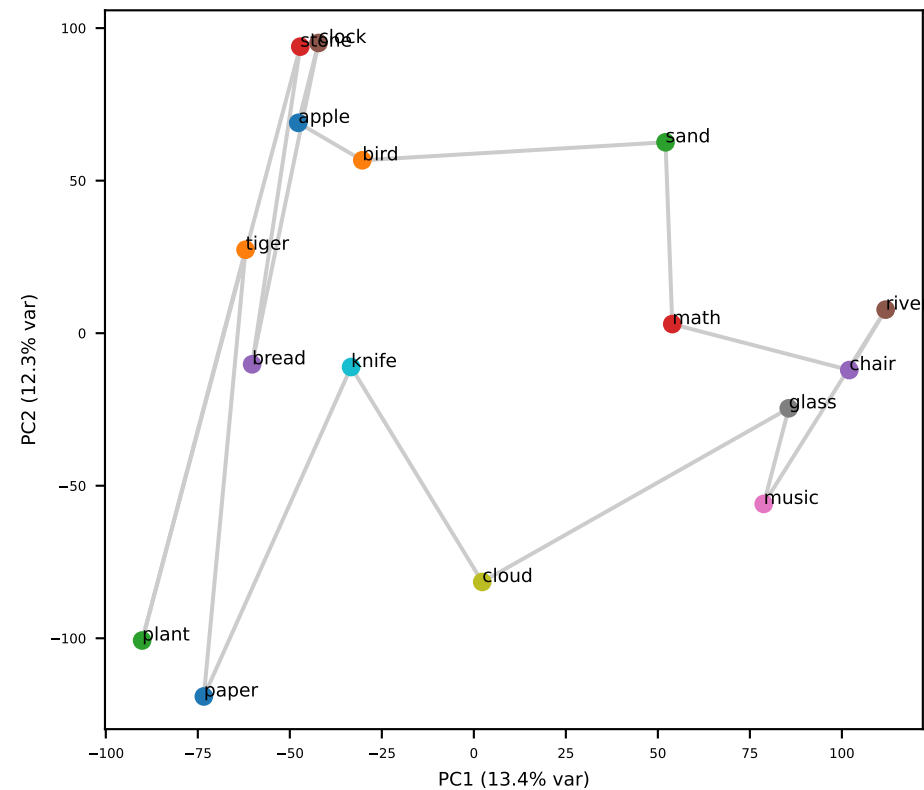
Qwen L30 (grid RSA=+0.49)
