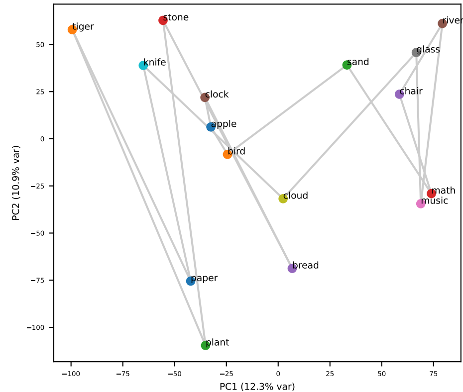
Qwen L29 (grid RSA=+0.40)
