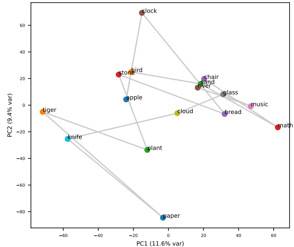
Qwen L26 (grid RSA=+0.23)
