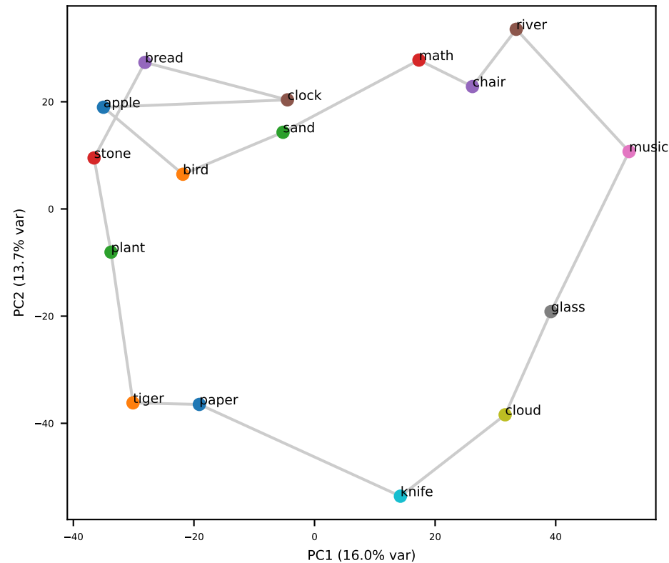
Gemma L26 (grid RSA=+0.57)
