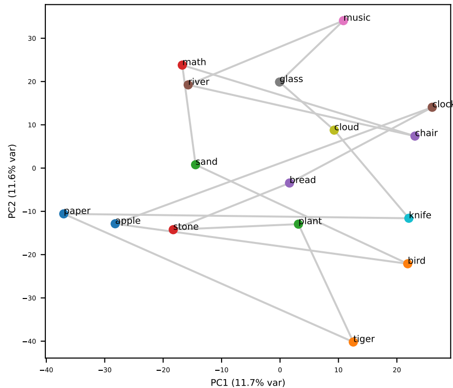
Gemma L14 (grid RSA=+0.16)
