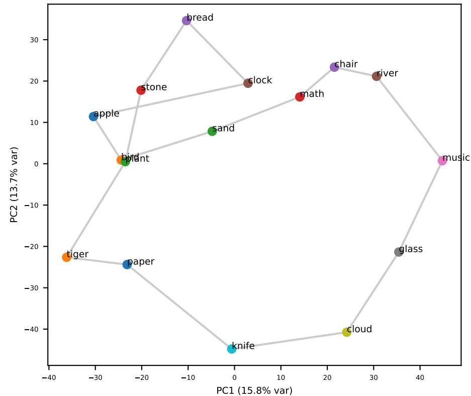
Gemma L17 (grid RSA=+0.47)
