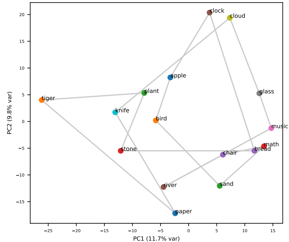
Qwen L17 (grid RSA=+0.15)
