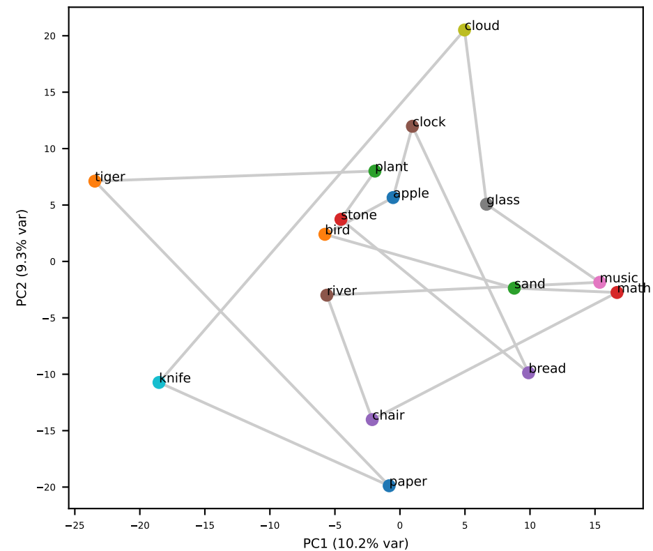
Qwen L8 (grid RSA=-0.02)
