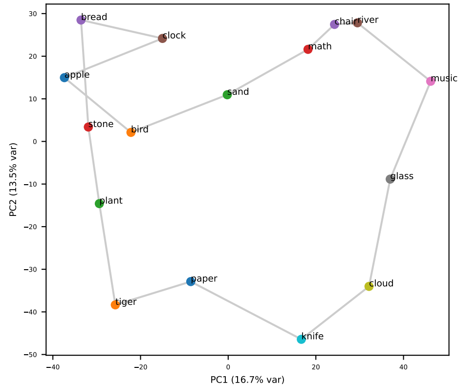
Gemma L20 (grid RSA=+0.59)
