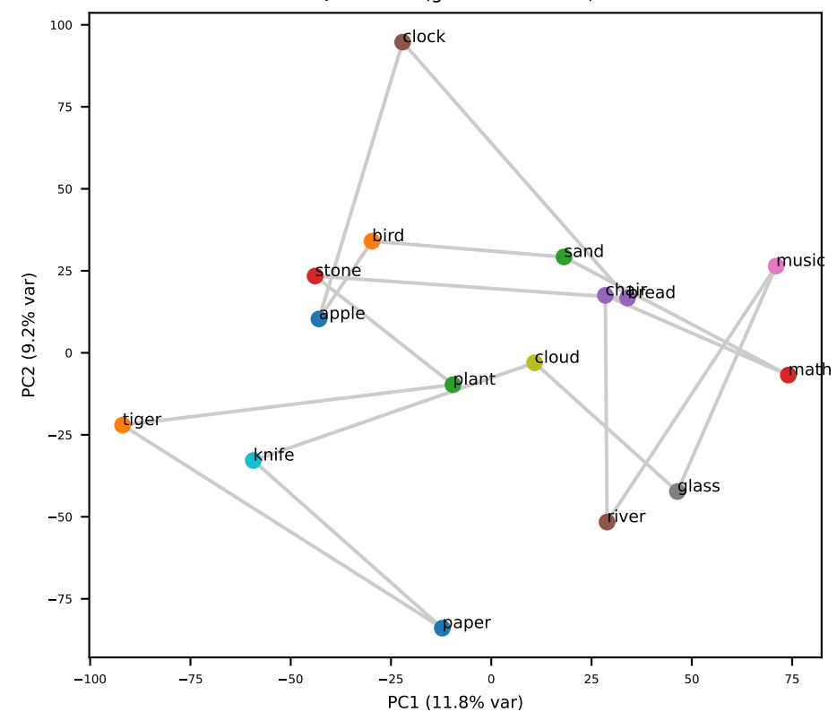
Qwen L28 (grid RSA=+0.29)
