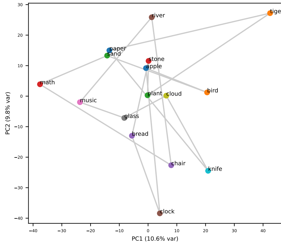
Gemma L8 (grid RSA=+0.02)
