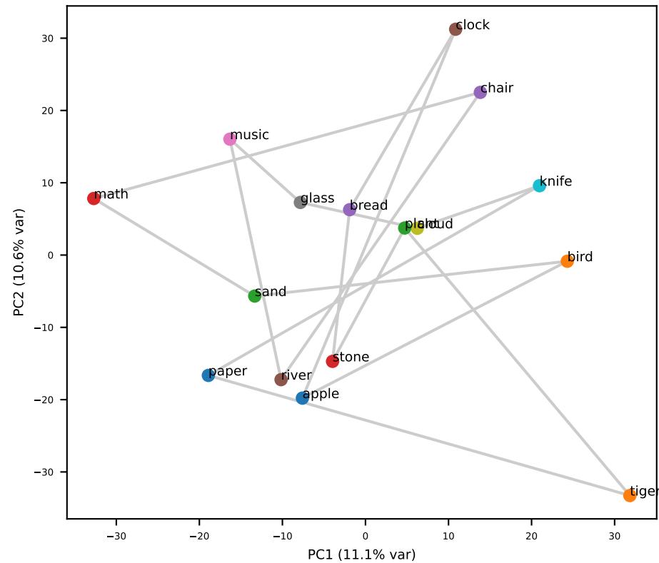
Gemma L11 (grid RSA=+0.04)
