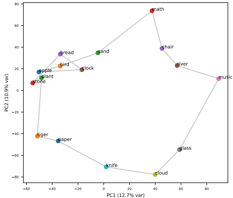
Gemma L30 (grid RSA=+0.54)
