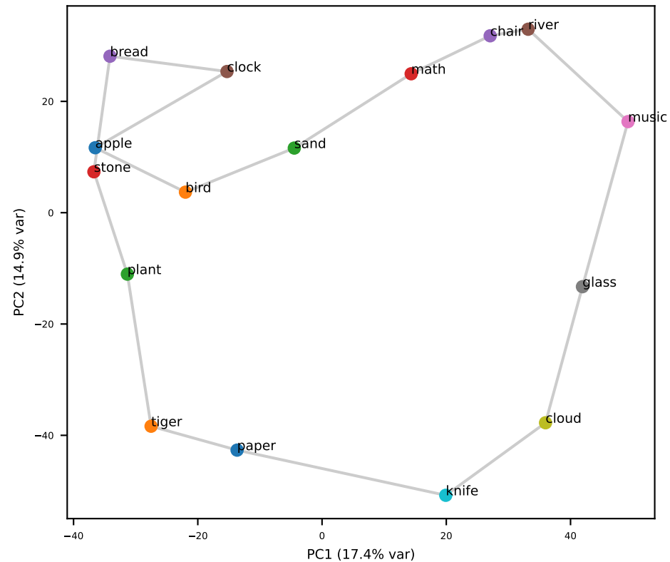
Gemma L25 (grid RSA=+0.58)
