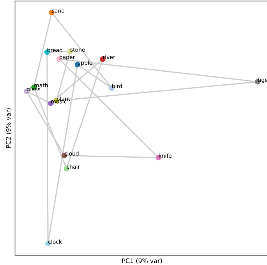
Gemma L2 (RSA -0.02)
