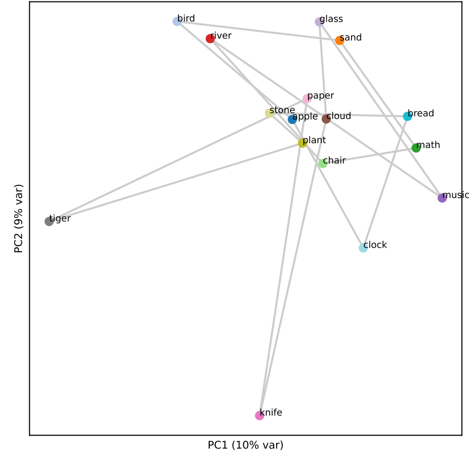
Qwen L6 (RSA -0.08)
