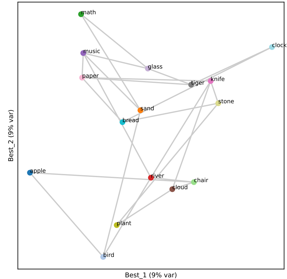
Qwen L16 (RSA 0.38)
