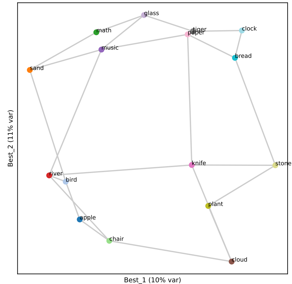
Qwen L34 (RSA 0.77)
