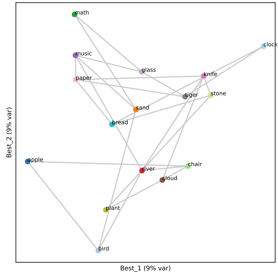
Qwen L15 (RSA 0.31)
