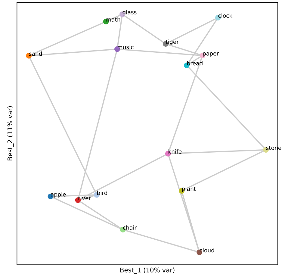
Qwen L32 (RSA 0.72)
