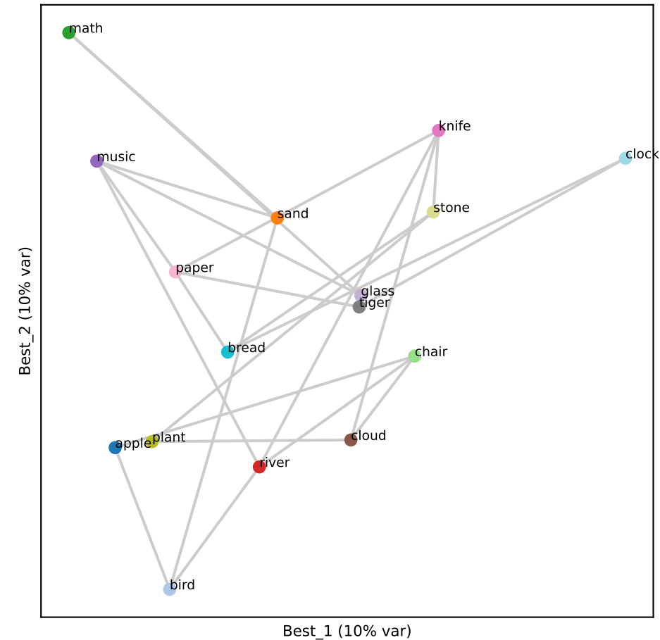
Qwen L11 (RSA 0.12)
