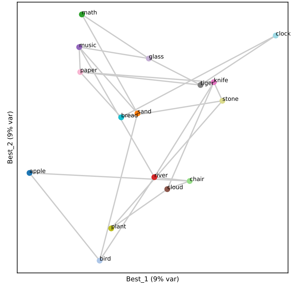
Qwen L17 (RSA 0.39)
