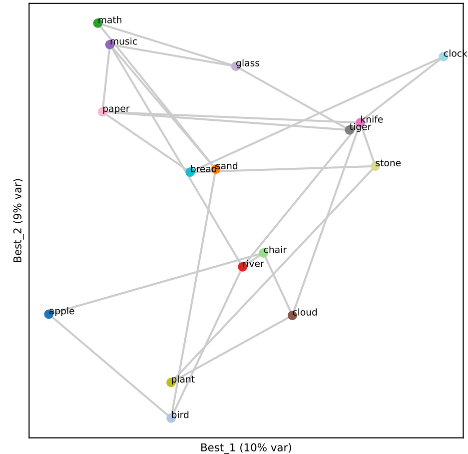
Qwen L18 (RSA 0.38)
