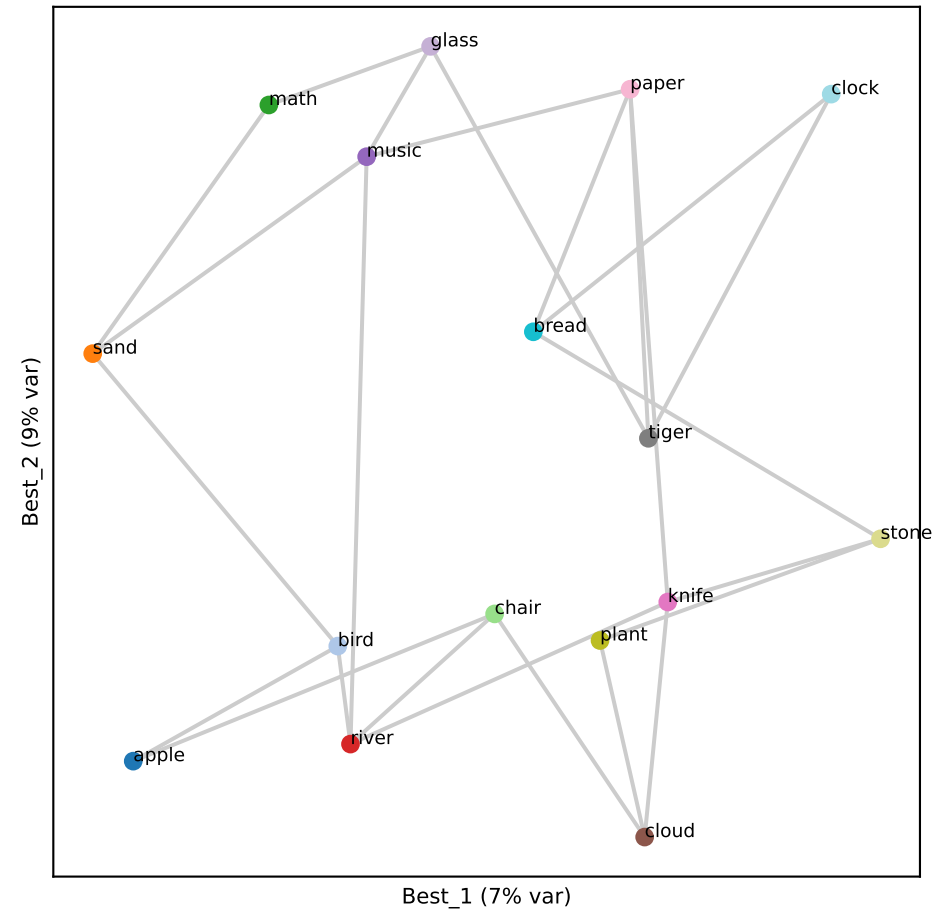
Qwen L29 (RSA 0.60)
