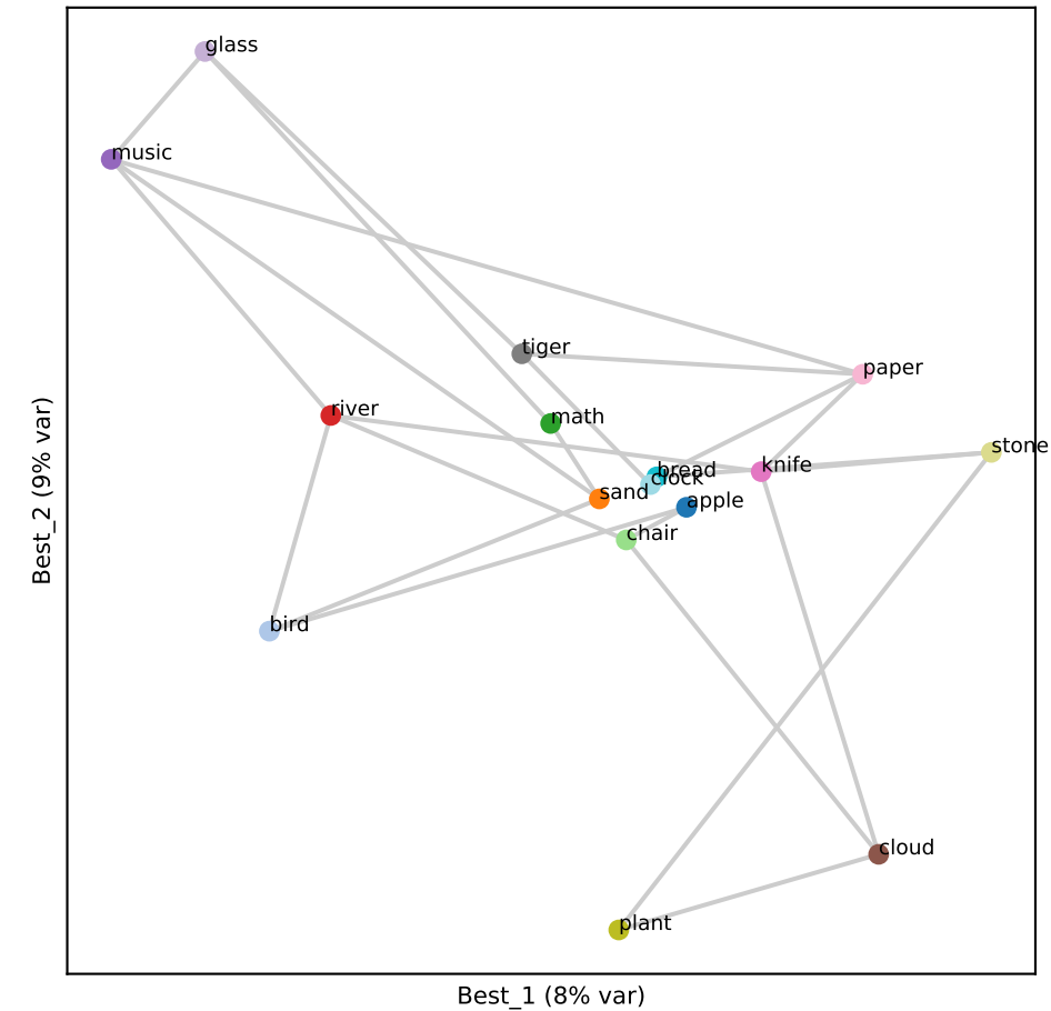
Qwen L0 (RSA 0.03)
