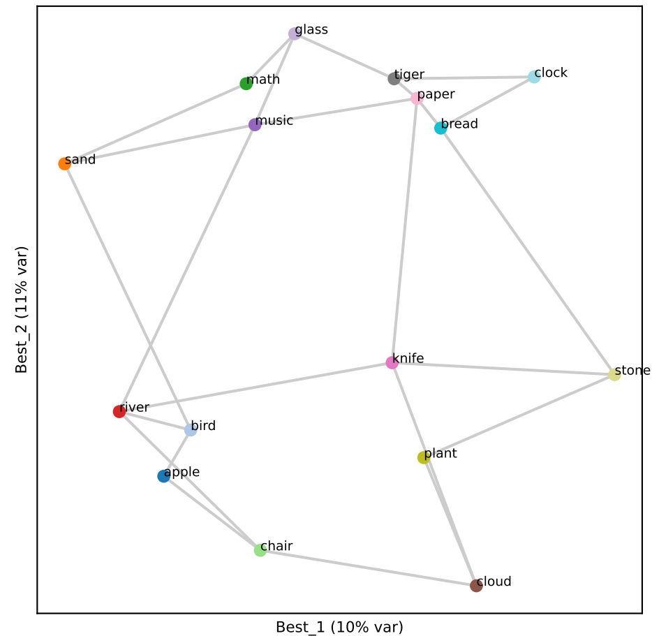
Qwen L33 (RSA 0.73)
