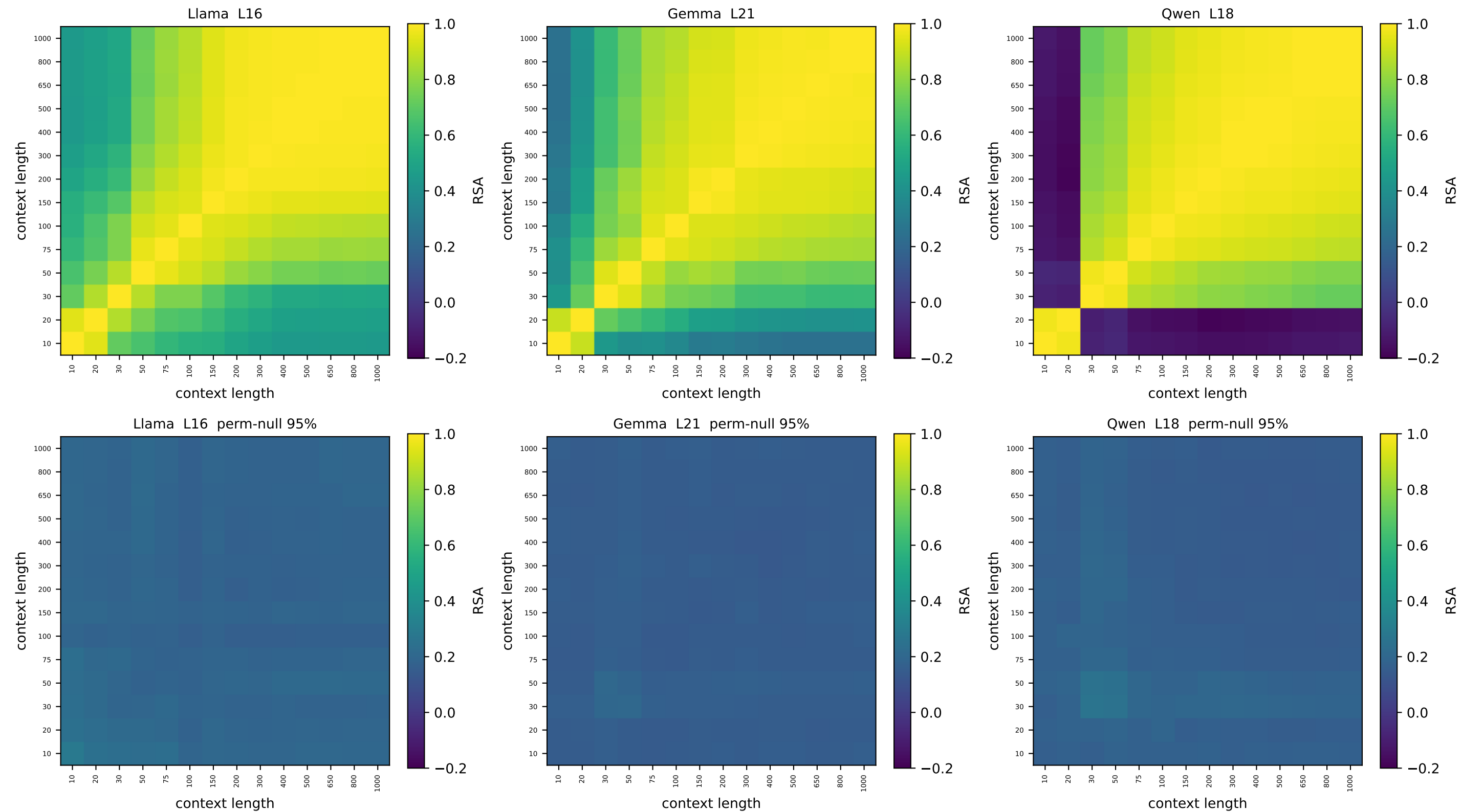
square_grid [v1] context-vs-context node-geometry RSA — relative depth 0.51 top: observed | bottom: node-label permutation null (95th pct)
