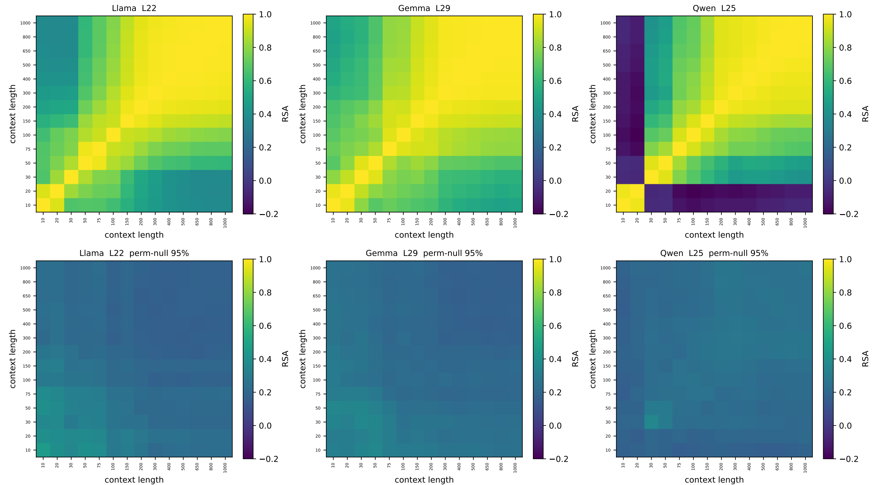
square_grid [v1] context-vs-context node-geometry RSA — relative depth 0.71 top: observed | bottom: node-label permutation null (95th pct)
