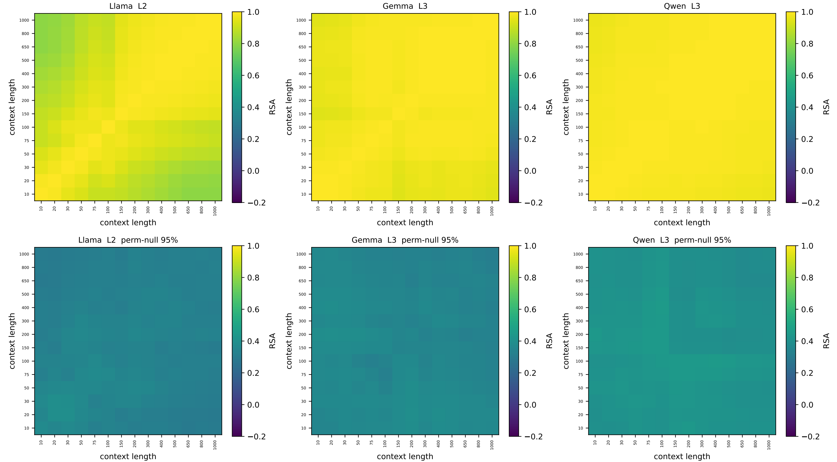
square_grid [v1] context-vs-context node-geometry RSA — relative depth 0.07 top: observed | bottom: node-label permutation null (95th pct)
