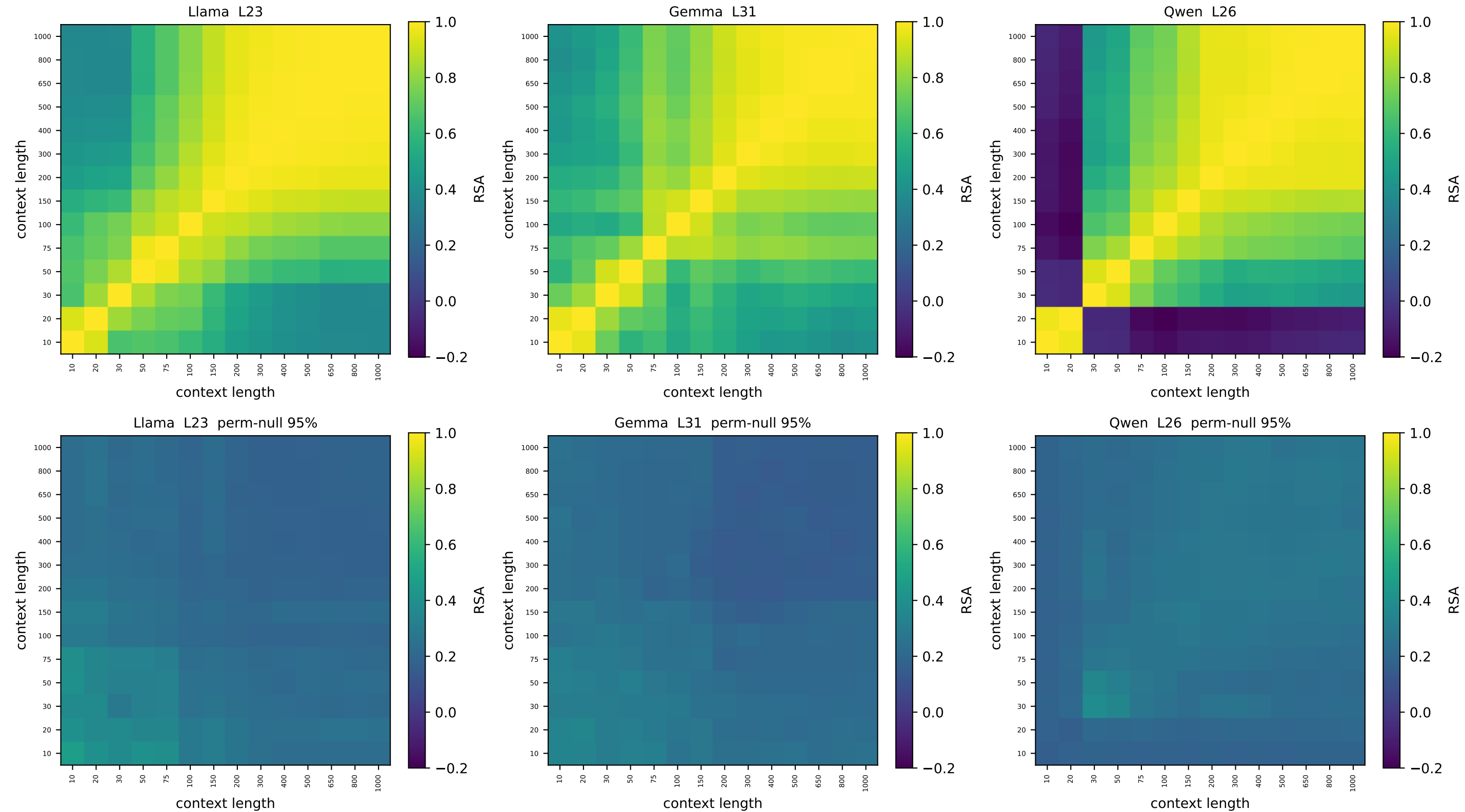
square_grid [v1] context-vs-context node-geometry RSA — relative depth 0.76 top: observed | bottom: node-label permutation null (95th pct)
