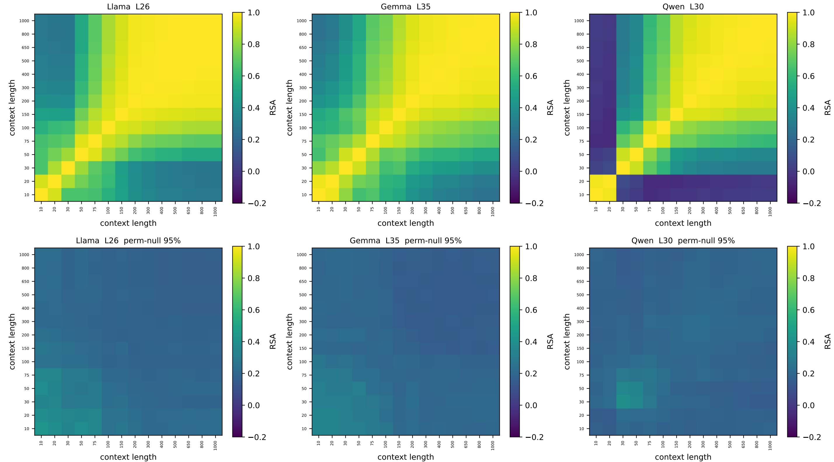
square_grid [v1] context-vs-context node-geometry RSA — relative depth 0.85 top: observed | bottom: node-label permutation null (95th pct)
