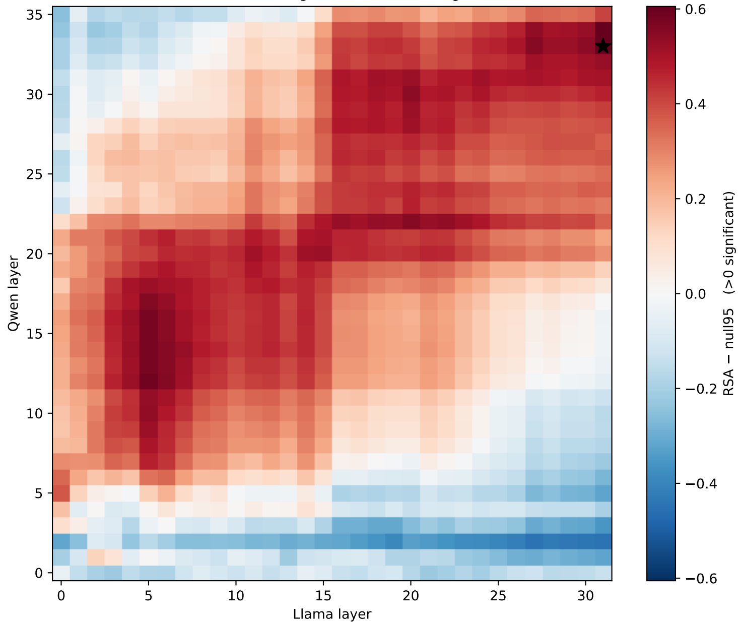
square_grid (n=16): Qwen vs Llama RSA – perm-null95 (0.18) red = above chance (significant); 74% of cells significant
