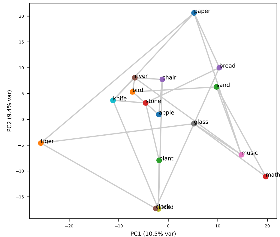
Qwen L8 (grid RSA=+0.08)
