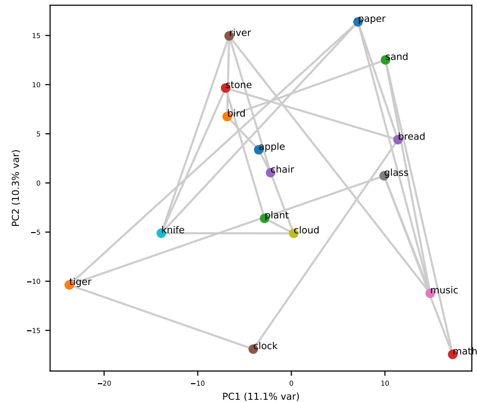
Qwen L16 (grid RSA=+0.19)
