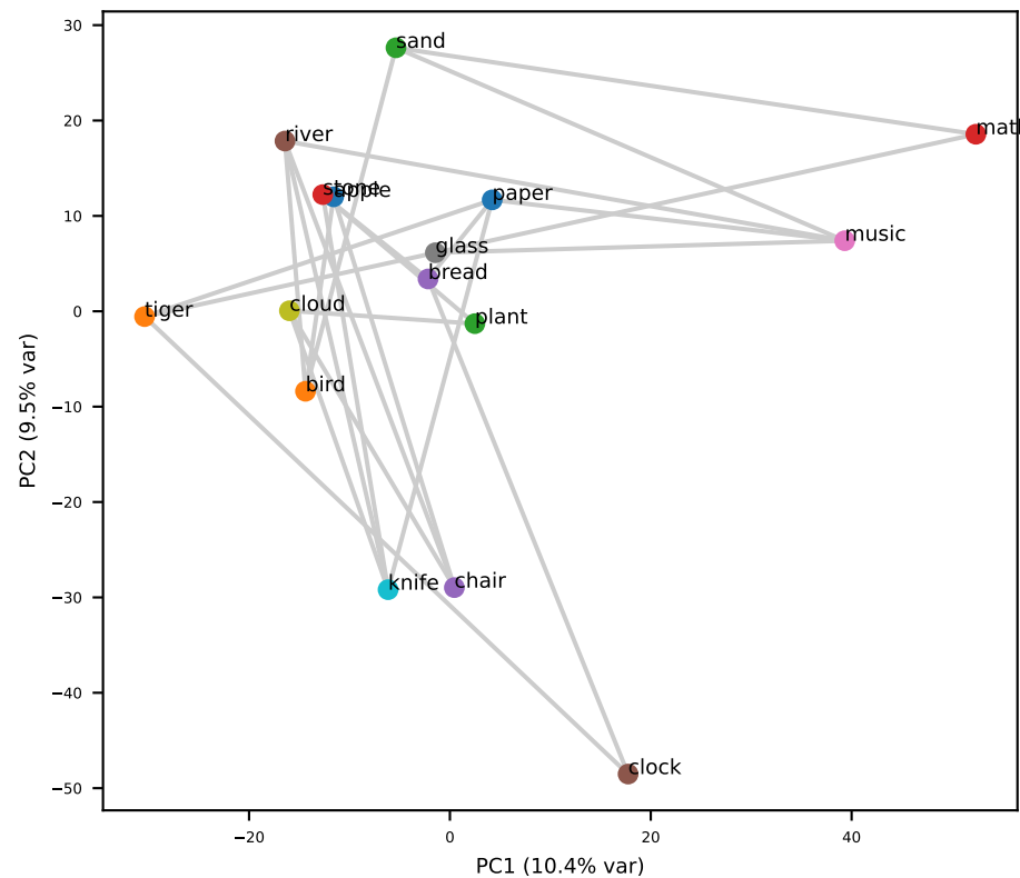
Gemma L6 (grid RSA=+0.07)
