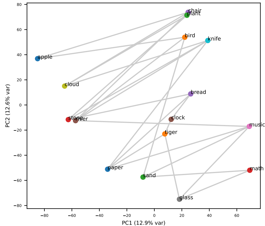
Gemma L31 (grid RSA=+0.52)
