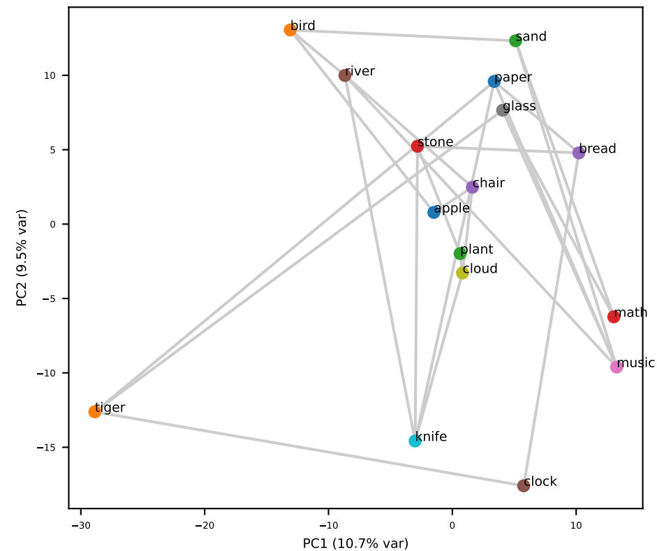
Qwen L6 (grid RSA=+0.04)
