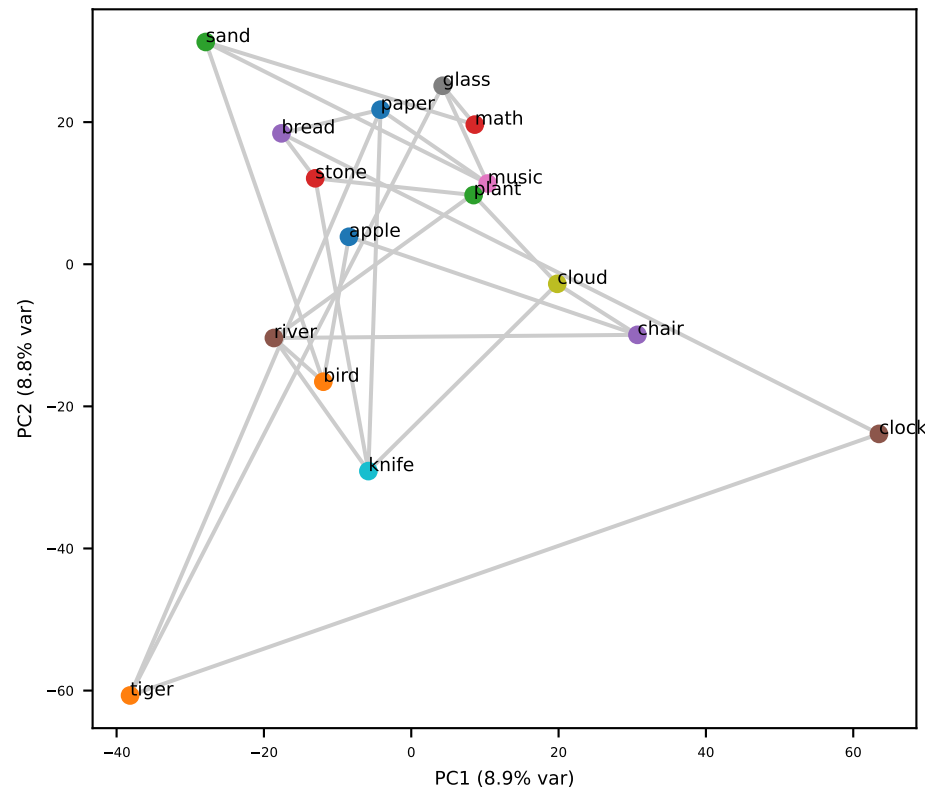
Gemma L2 (grid RSA=+0.09)
