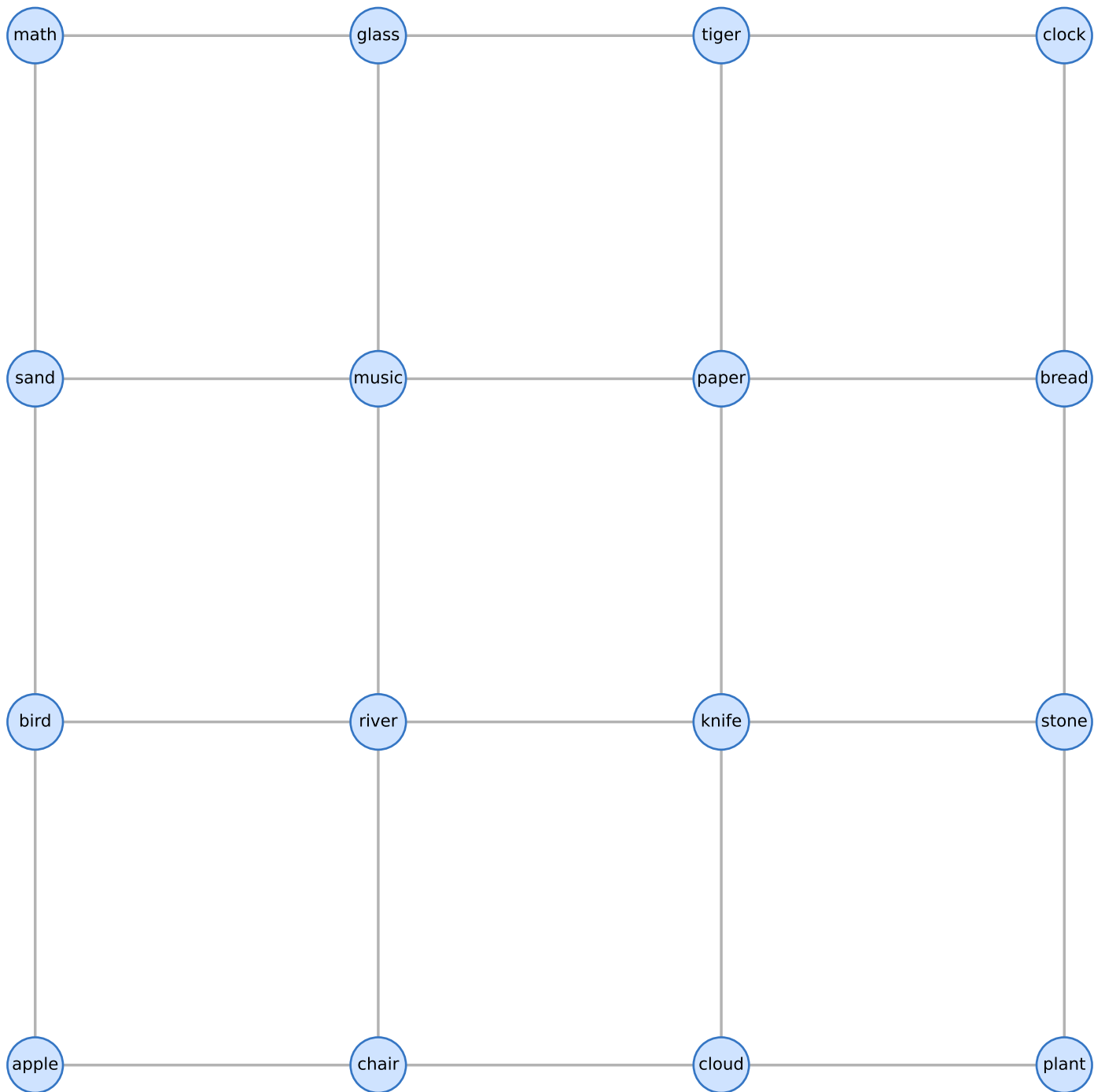
Graph: 16 nodes
