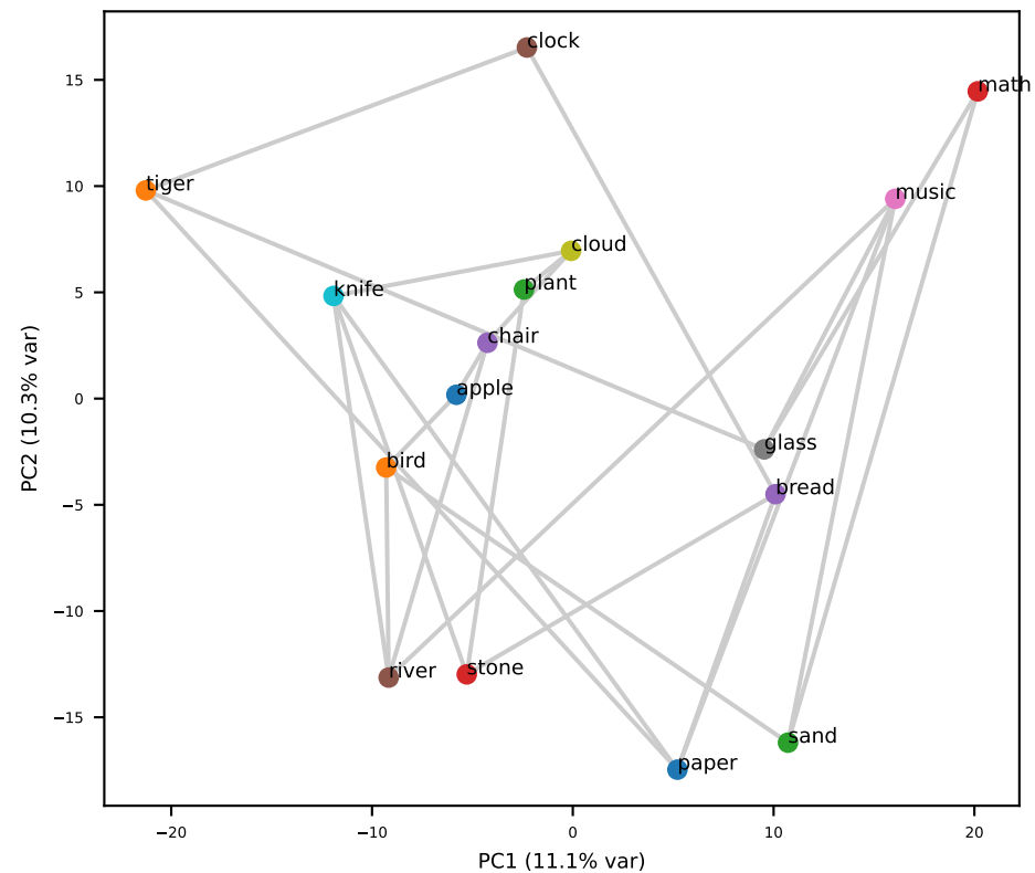
Qwen L14 (grid RSA=+0.19)
