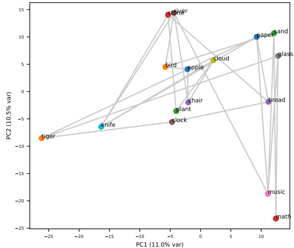
Qwen L17 (grid RSA=+0.19)
