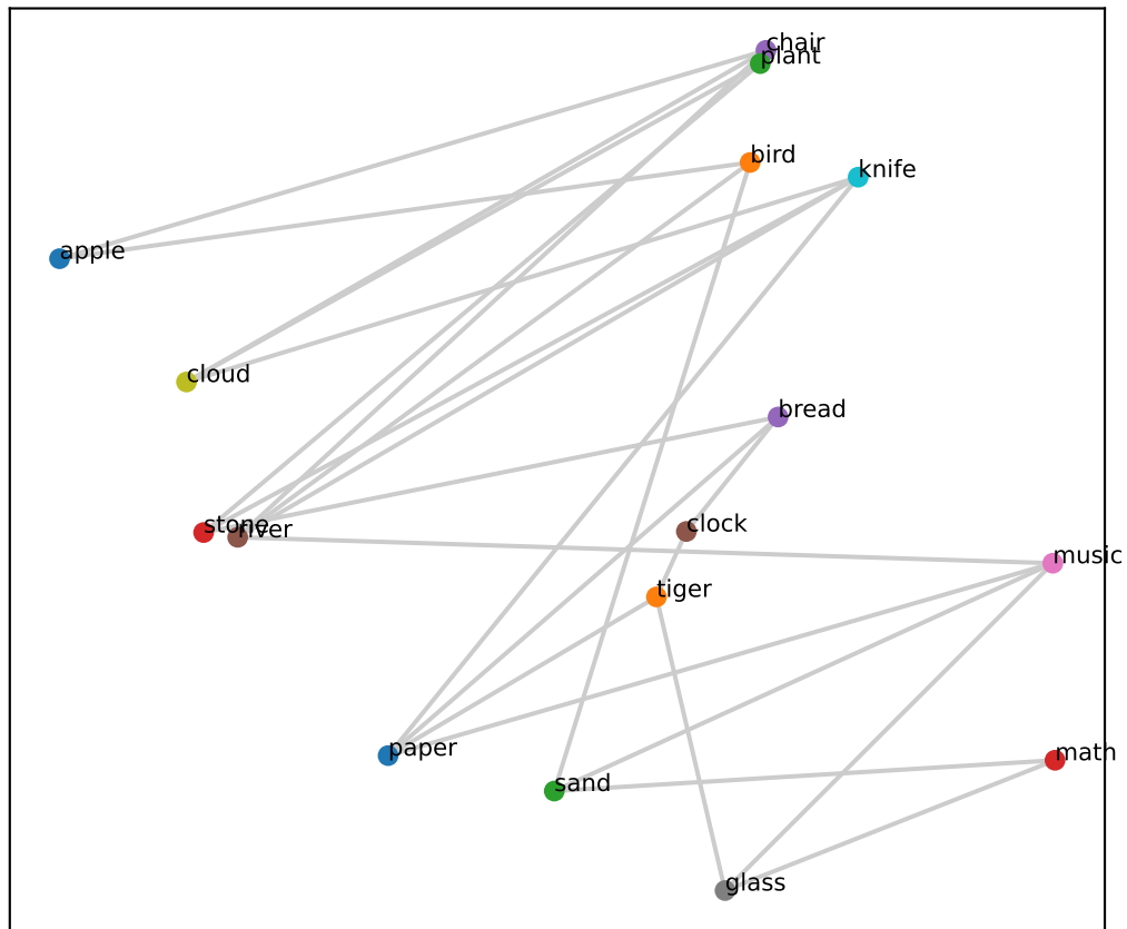
Gemma L31 (grid RSA=0.52, PCA corr=0.27)
