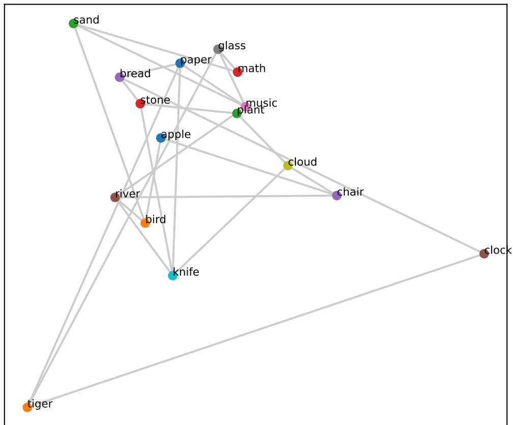
Gemma L2 (grid RSA=0.09, PCA corr=0.04)
