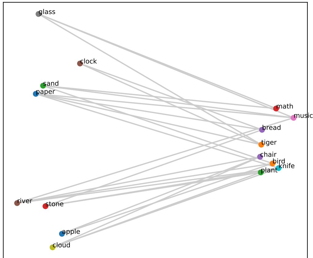
Qwen L31 (grid RSA=0.15, PCA corr=-0.01)
