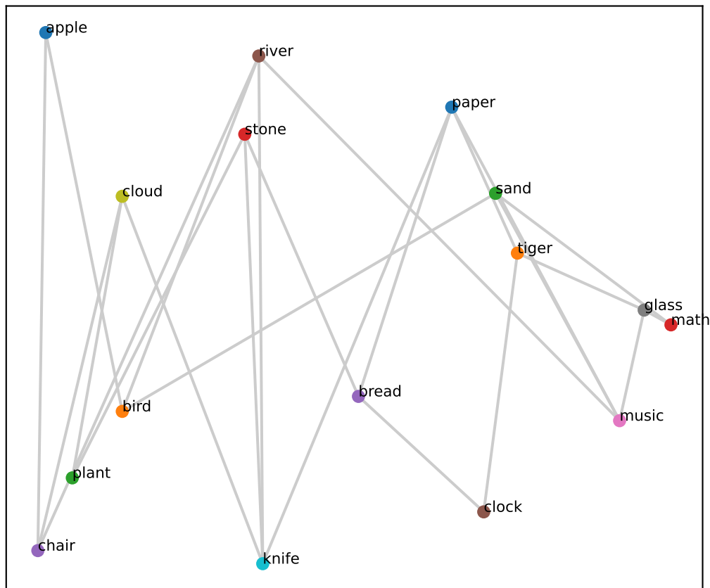
Gemma L24 (grid RSA=0.50, PCA corr=0.38)
