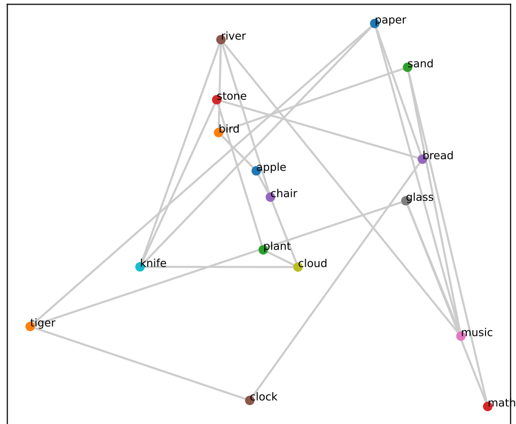
Qwen L16 (grid RSA=0.19, PCA corr=0.07)
