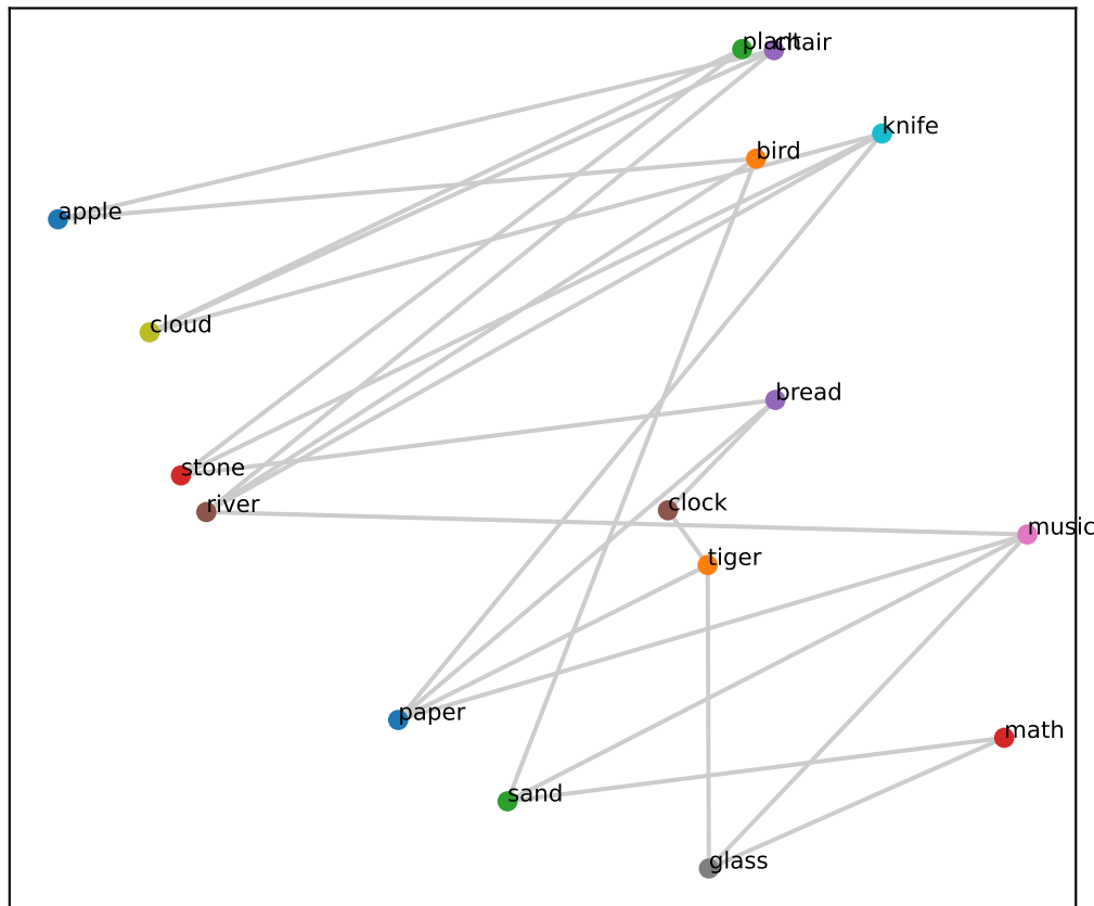
Gemma L32 (grid RSA=0.52, PCA corr=0.26)
