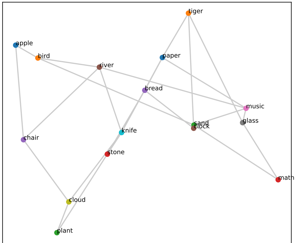
Gemma L17 (grid RSA=0.55, PCA corr=0.51)
