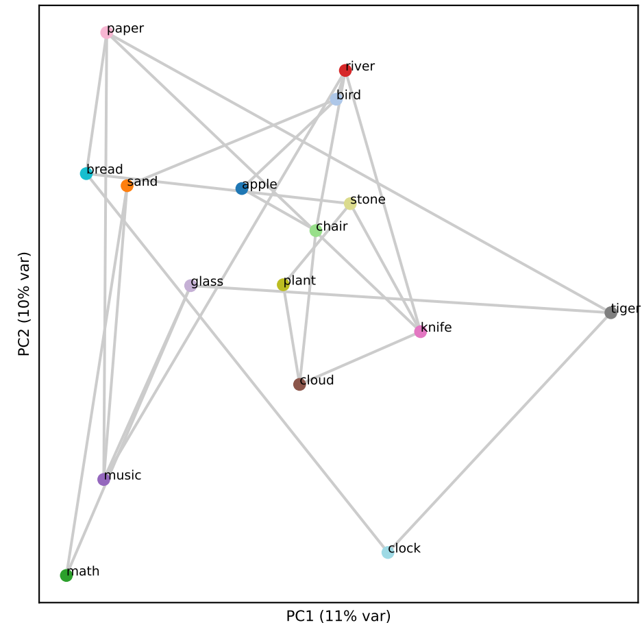
Qwen L11 (RSA 0.11)
