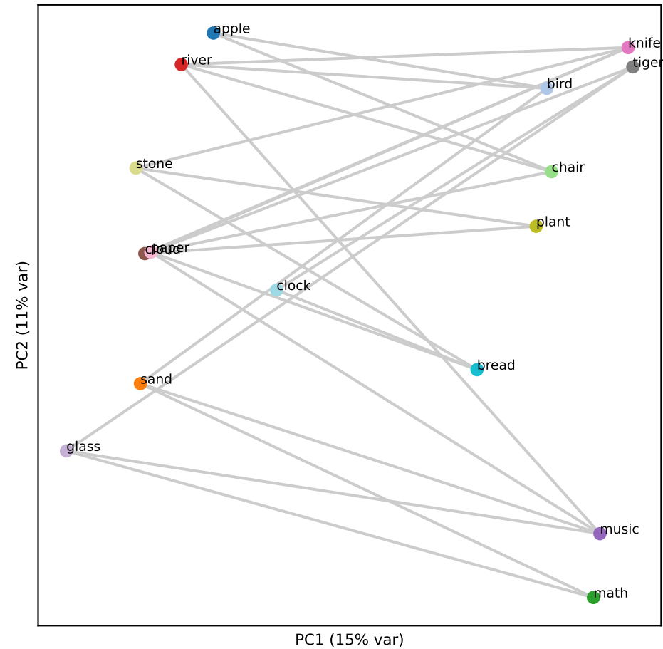
Qwen L20 (RSA -0.03)
