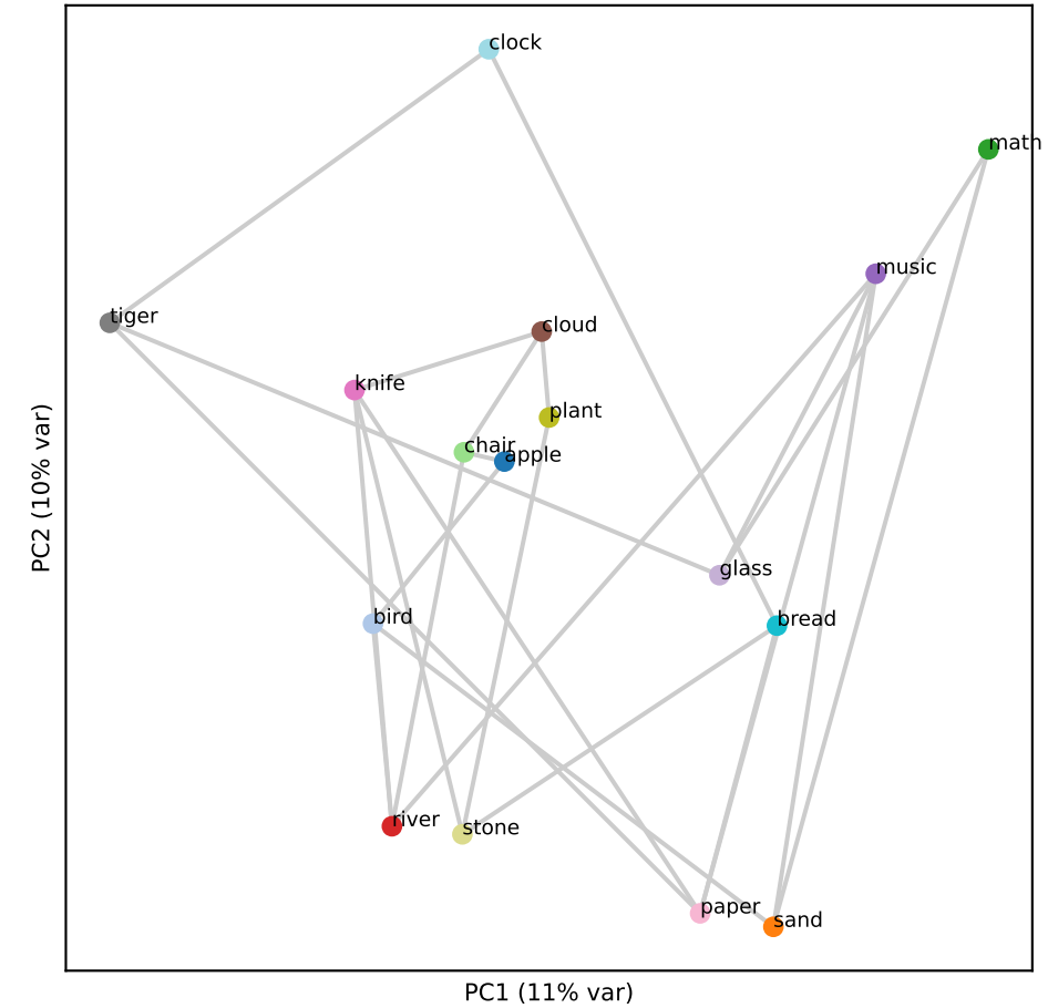
Qwen L12 (RSA 0.11)
