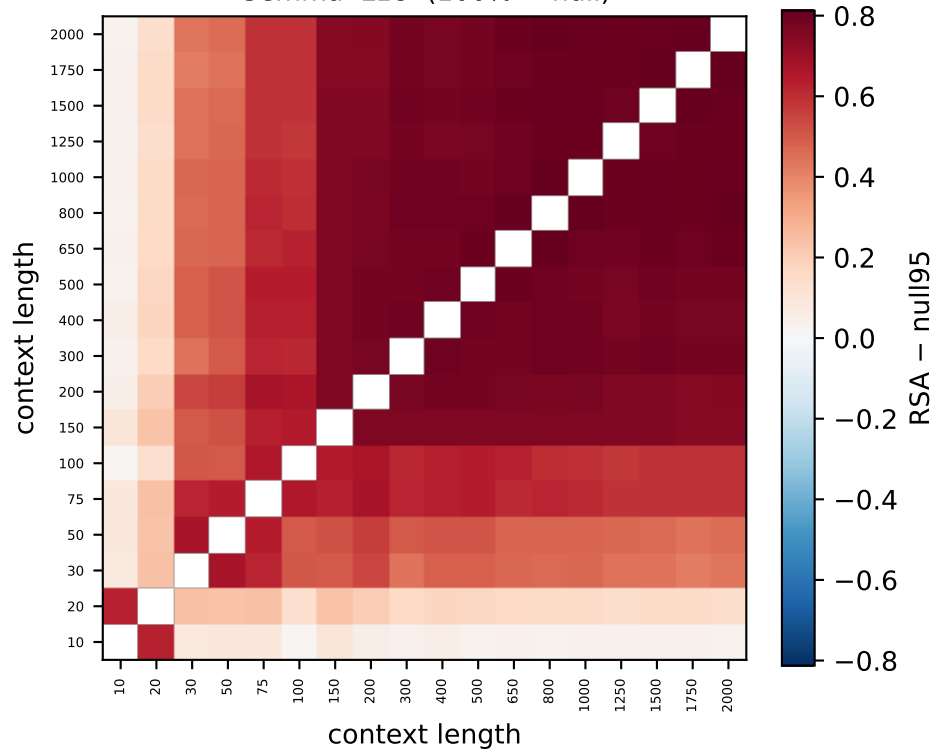
Gemma L18 (100% > null)
