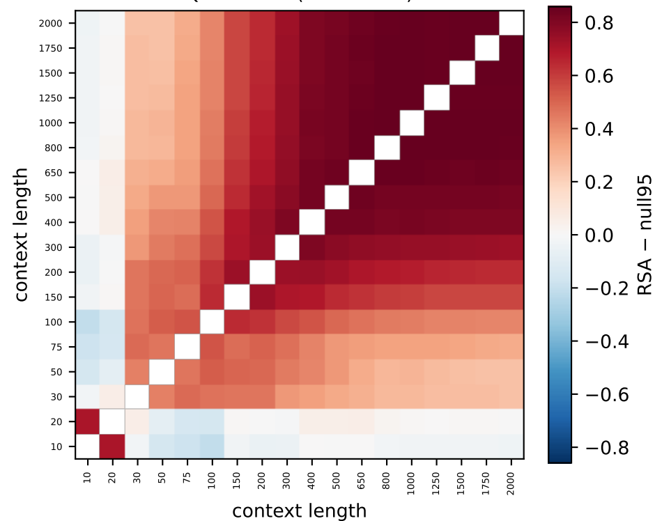
Qwen L33 (87% > null)
