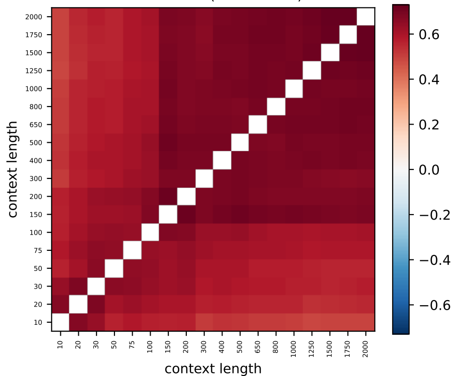
Gemma L6 (100% > null)
