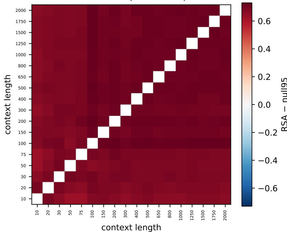
Gemma L2 (100% > null)
