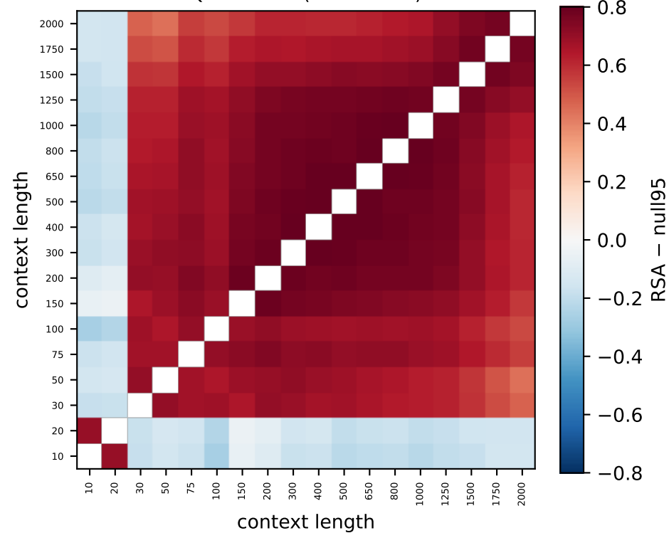
Qwen L16 (79% > null)
