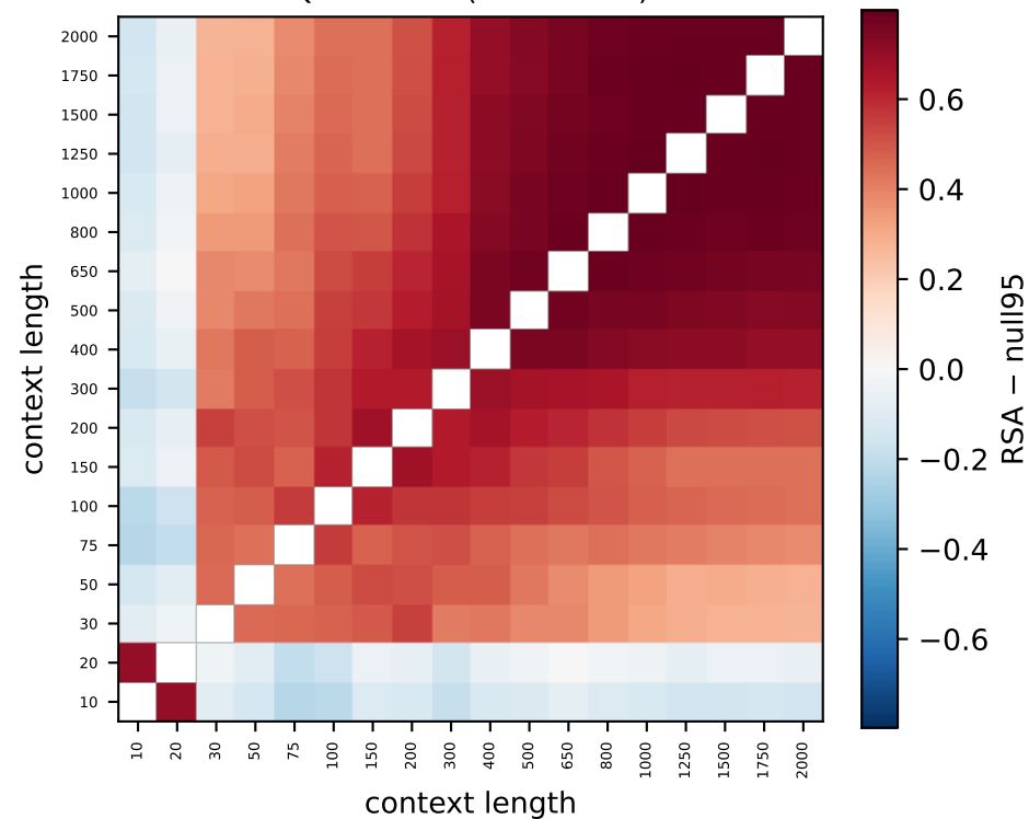
Qwen L31 (80% > null)
