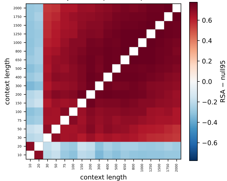
Qwen L21 (79% > null)
