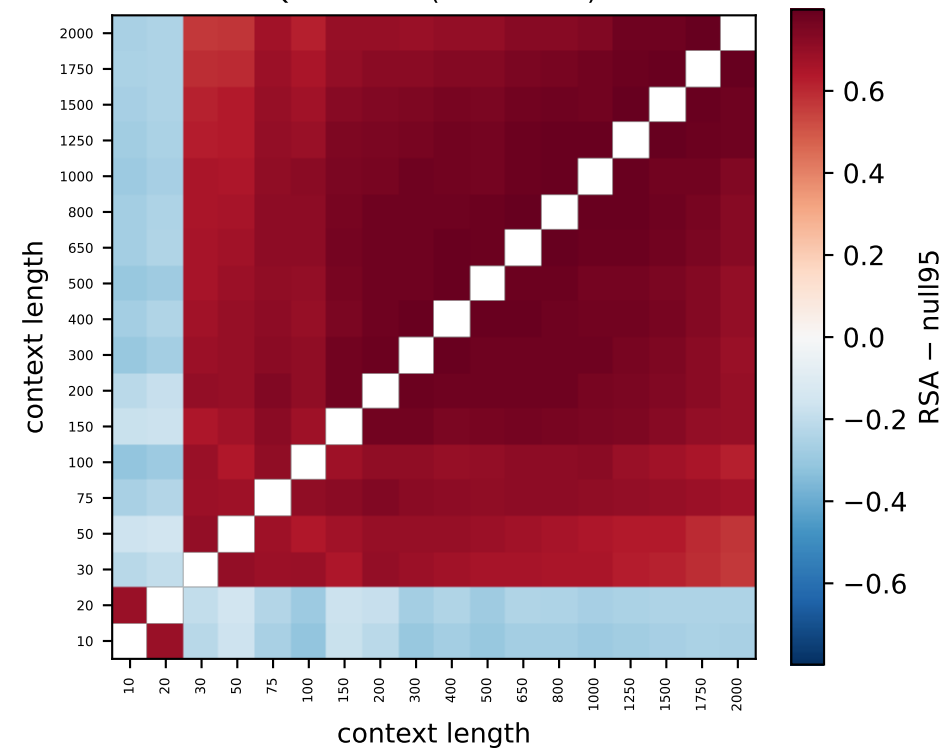
Qwen L19 (79% > null)
