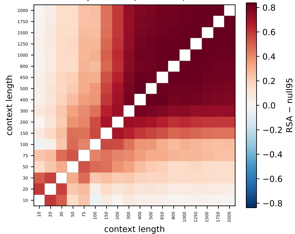
Qwen L35 (99% > null)
