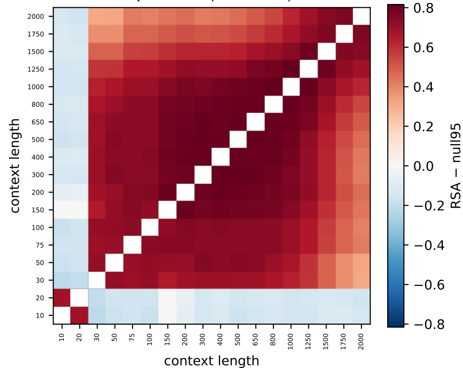
Qwen L12 (80% > null)
