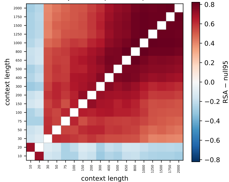
Qwen L24 (79% > null)
