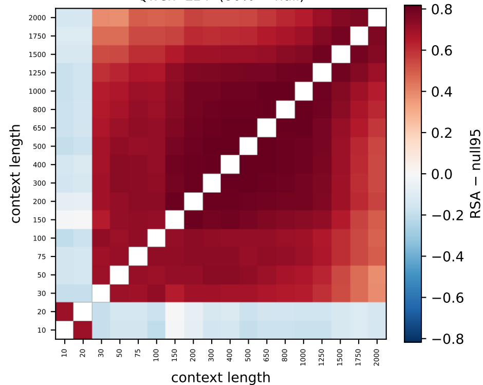
Qwen L14 (80% > null)
