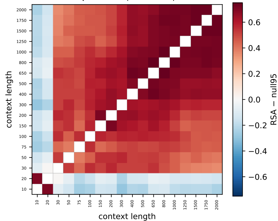
Qwen L28 (80% > null)
