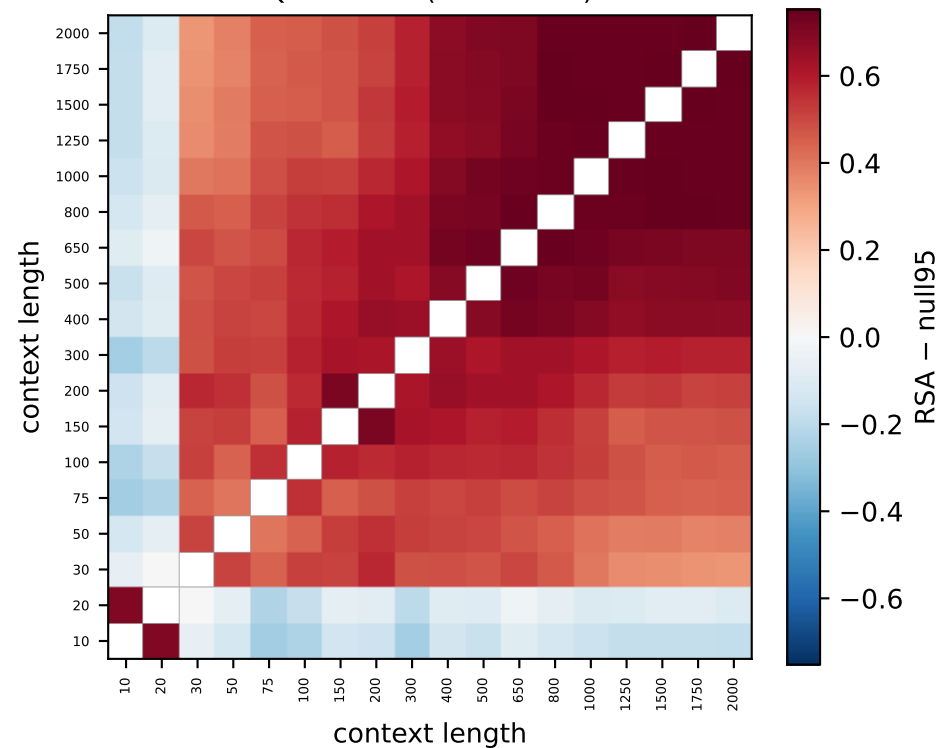
Qwen L29 (79% > null)
