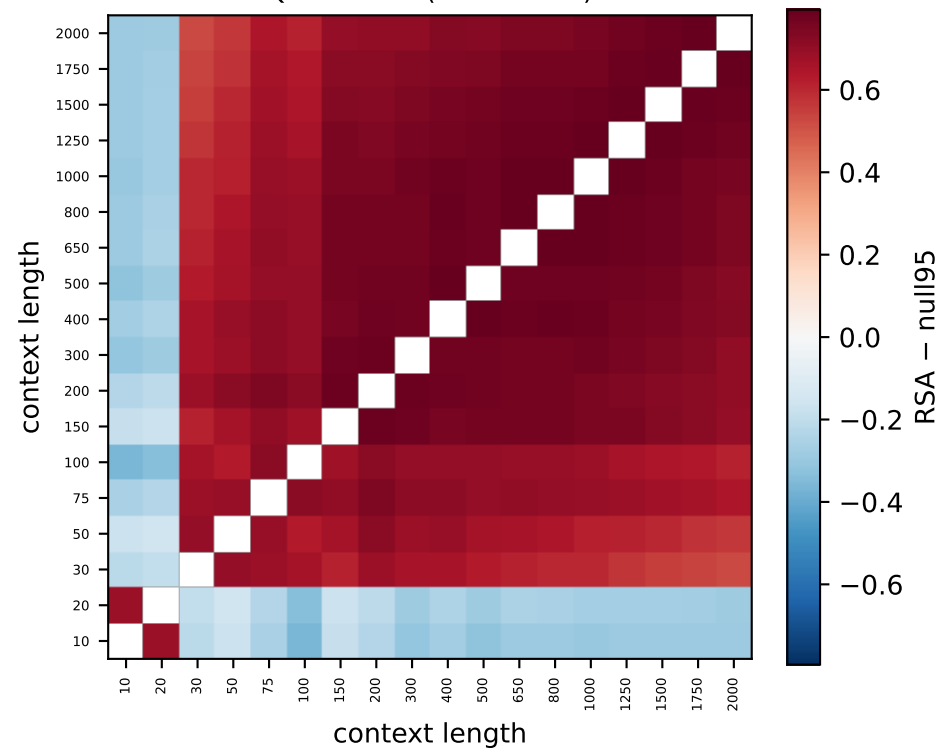
Qwen L20 (79% > null)
