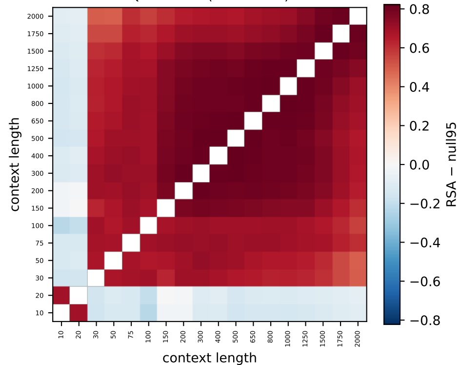
Qwen L18 (80% > null)
