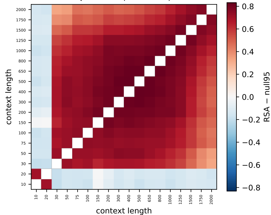
Qwen L13 (79% > null)
