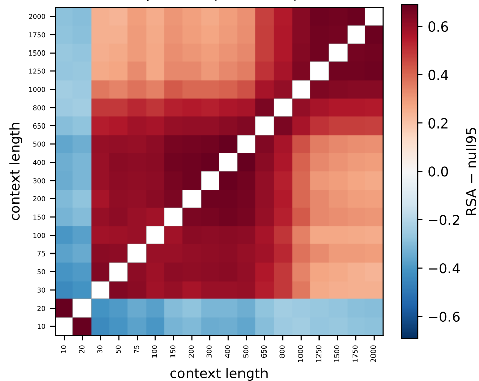
Qwen L6 (79% > null)
