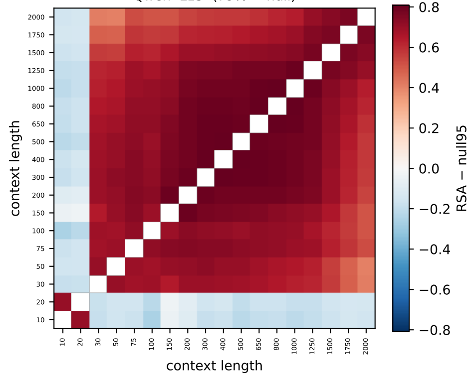
Qwen L15 (79% > null)
