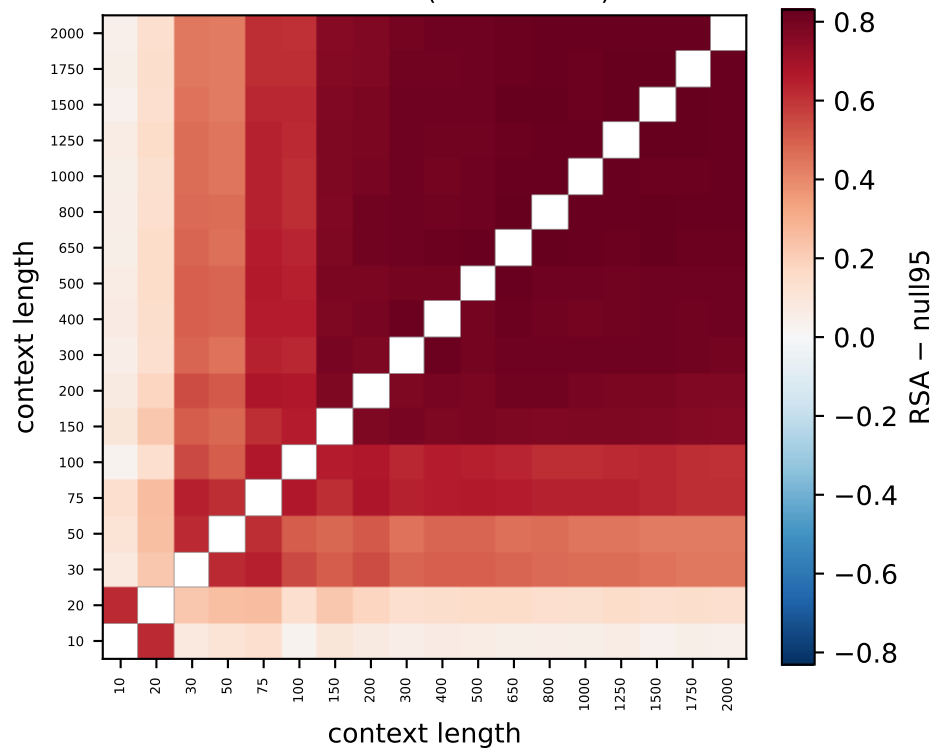
Gemma L22 (100% > null)
