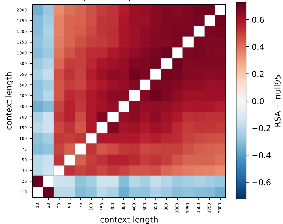
Qwen L25 (79% > null)
