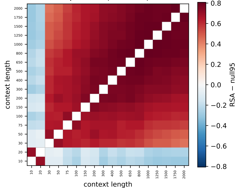
Qwen L22 (79% > null)
