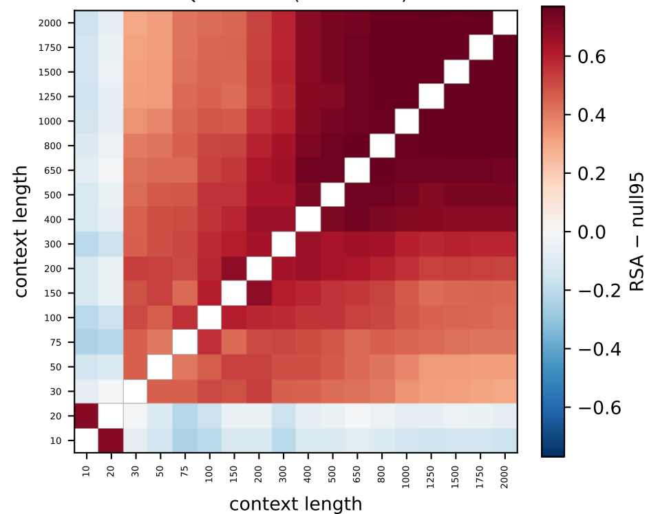
Qwen L30 (79% > null)
