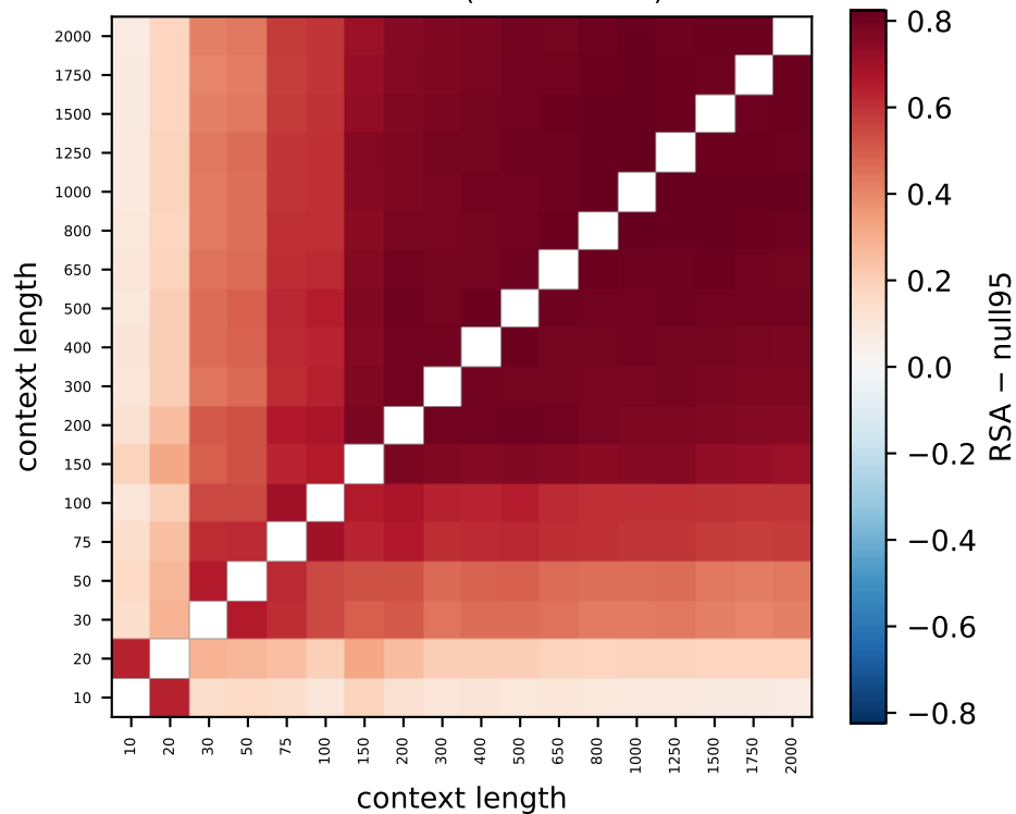
Gemma L17 (100% > null)
