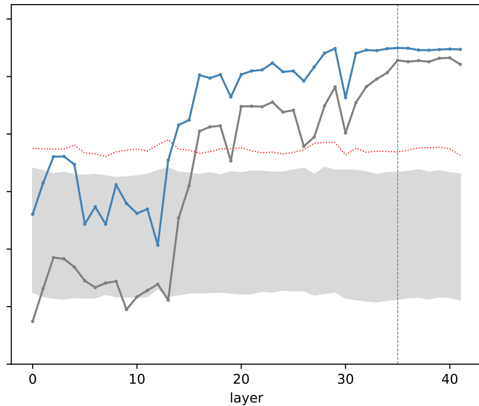
hex (best-2D peak L35)
