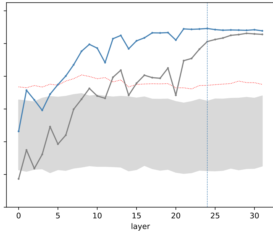
hex (best-2D peak L24)
