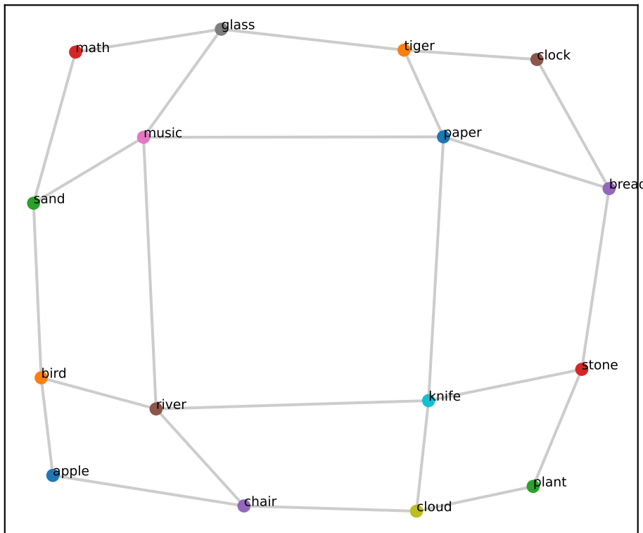
square_grid best-2D (RSA 0.88 | null95 0.47, p < .001 )
