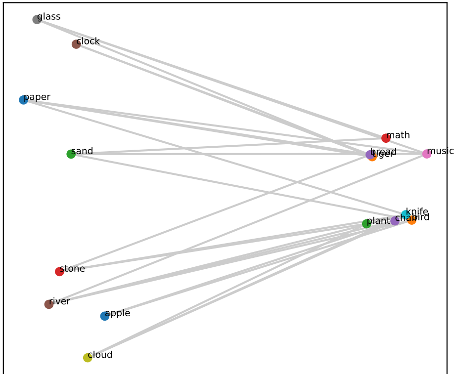
square_grid best-2D (RSA 0.72 | null95 0.45, p<.001)
