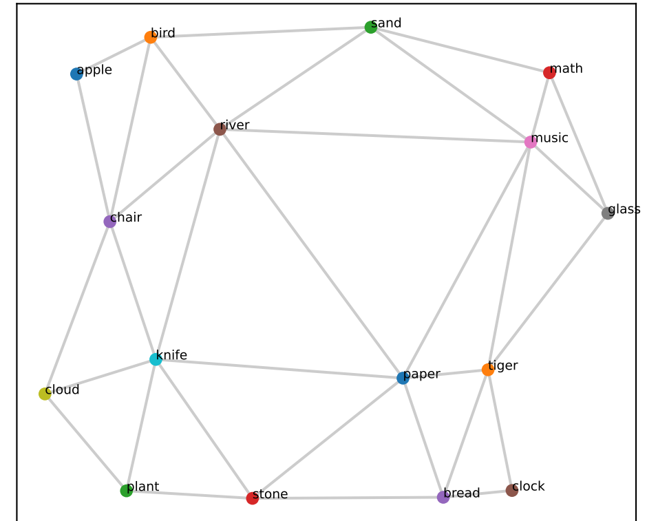
hex best-2D (RSA 0.88 | null95 0.46, p < .001 )
