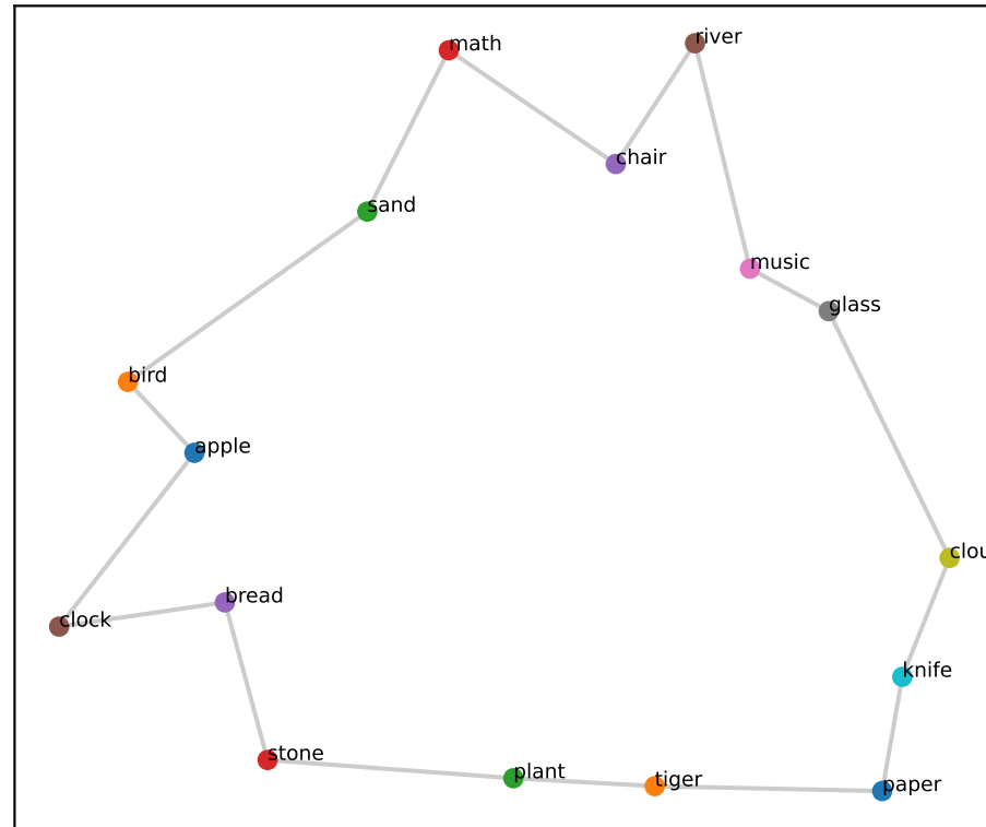
ring best-2D (RSA 0.94 | null95 0.49, p<.001)
