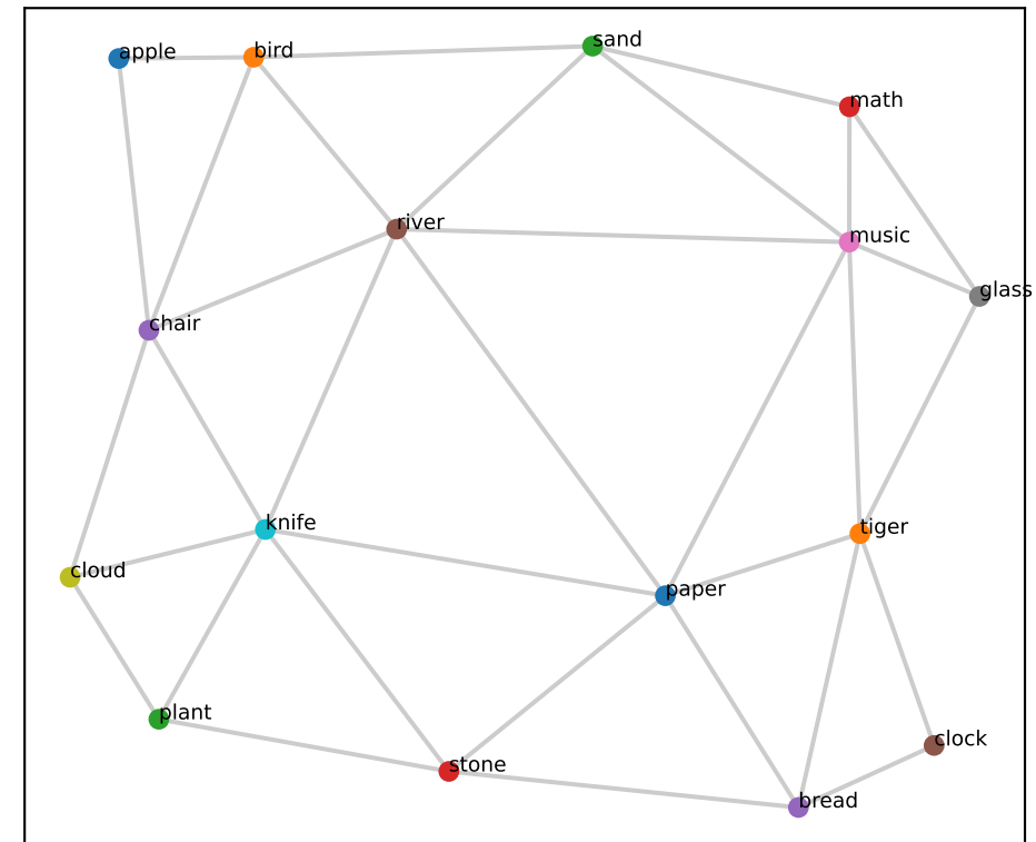
hex best-2D (RSA 0.90 | null95 0.47, p < .001 )
