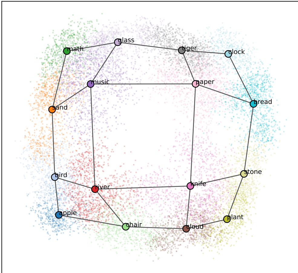
square_grid best-2D (RSA 0.88, p < .001 )
