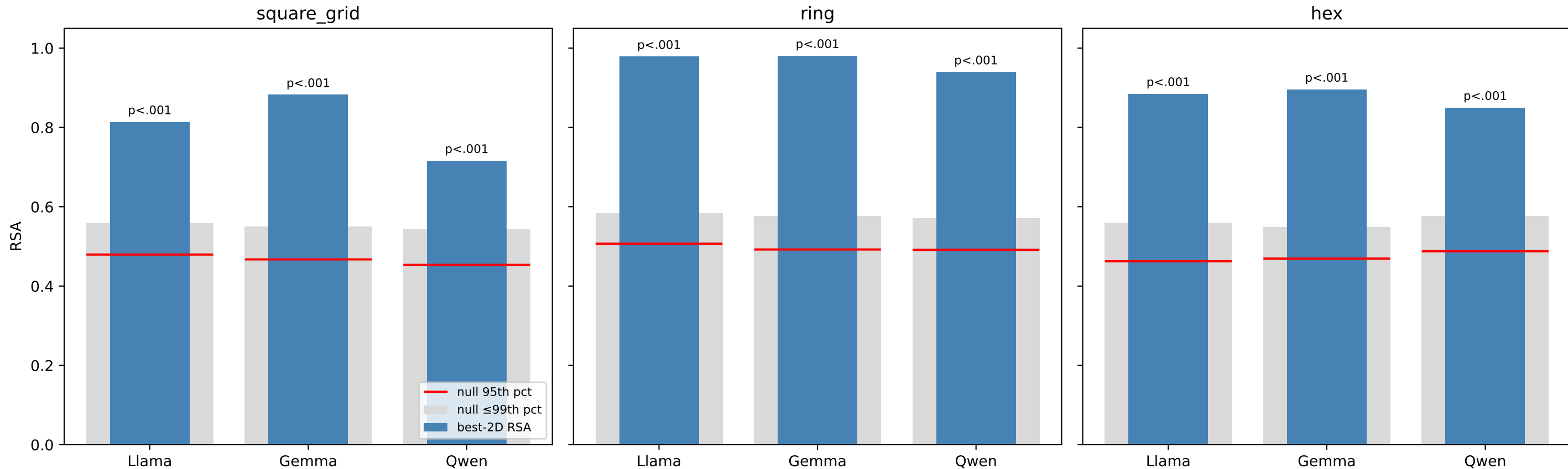
best-2D RSA vs label-permutation null (gray = null \leq 99th pct, red = null 95th pct)
