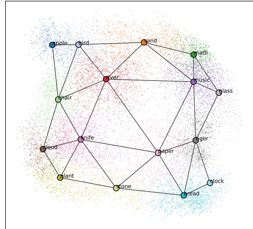
hex best-2D (RSA 0.90, p < .001 )
