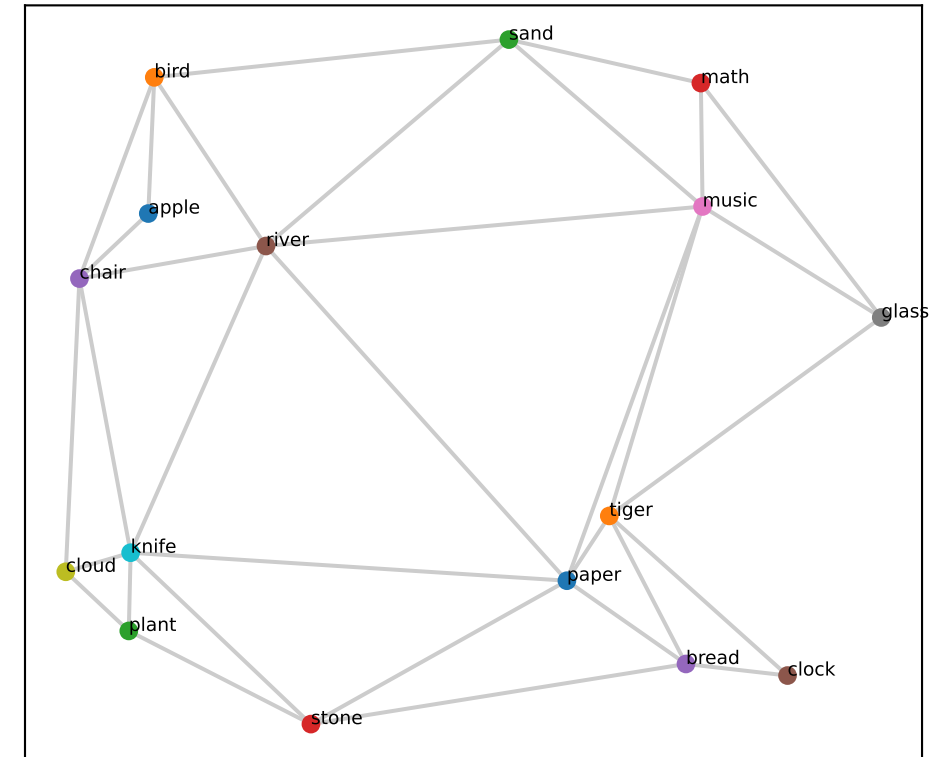
hex best-2D (RSA 0.85 | null95 0.49, p<.001)
