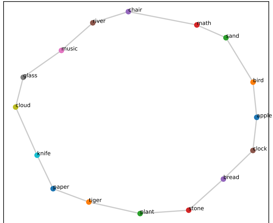
ring best-2D (RSA 0.98 | null95 0.51, p < .001 )
