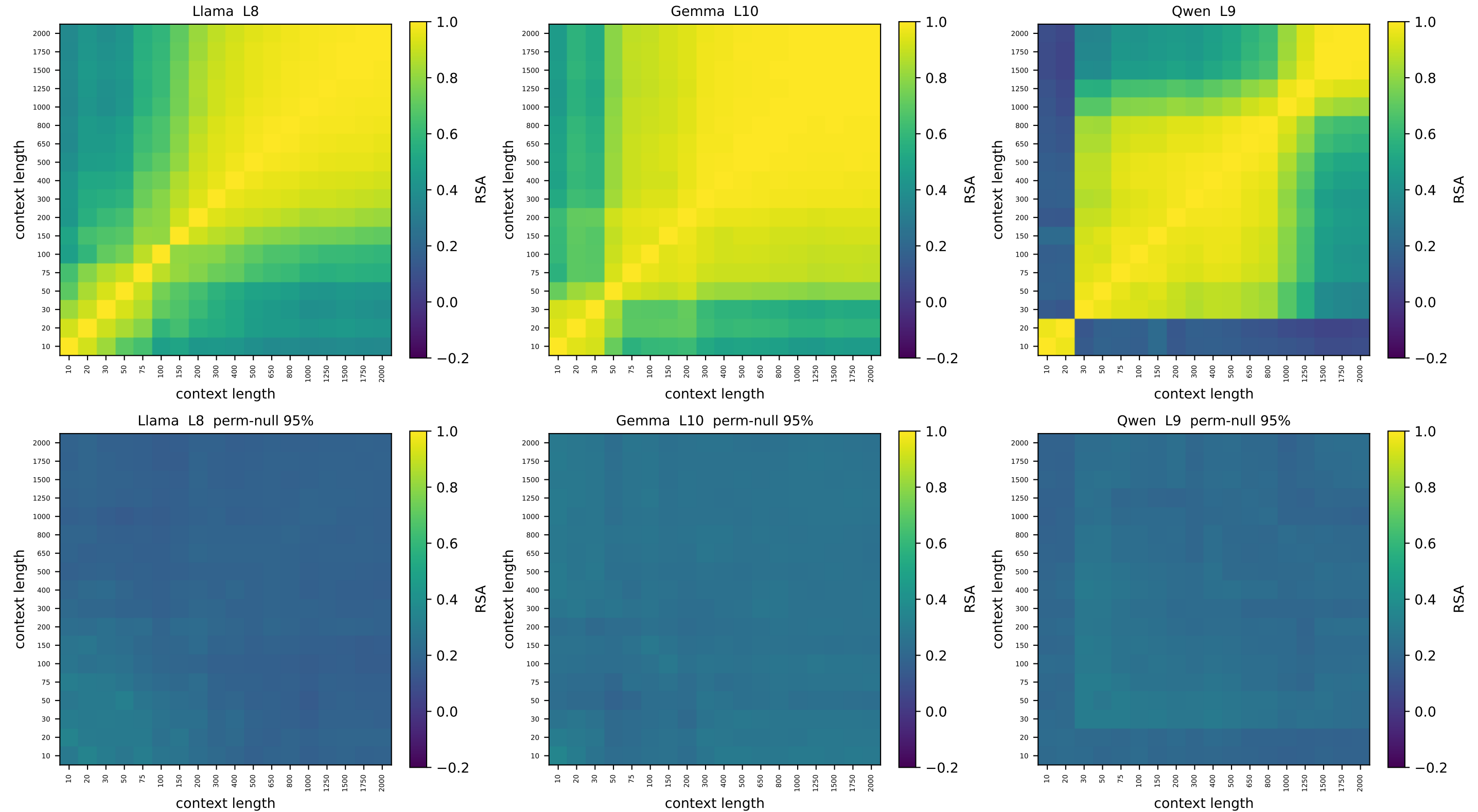
ring [v2] context-vs-context node-geometry RSA — relative depth 0.24 top: observed | bottom: node-label permutation null (95th pct)
