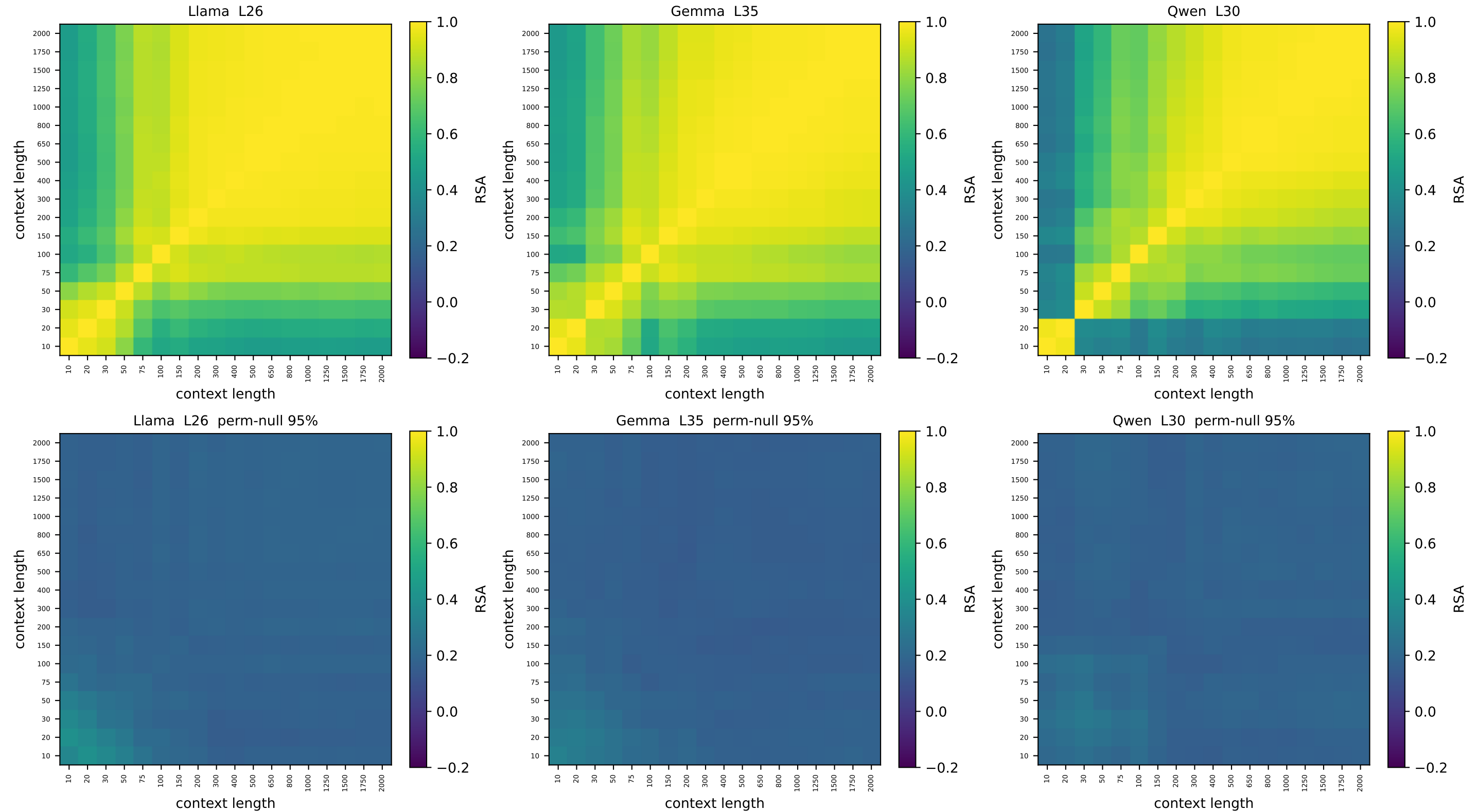
ring [v2] context-vs-context node-geometry RSA — relative depth 0.85 top: observed | bottom: node-label permutation null (95th pct)
