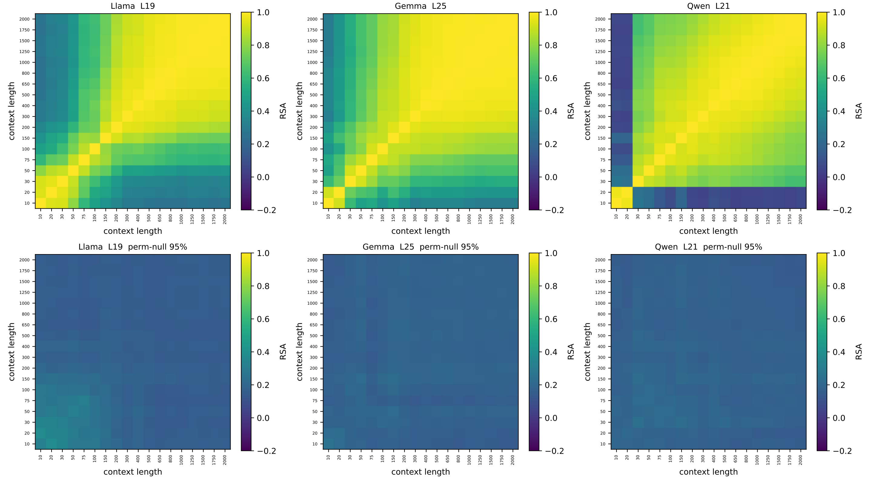
ring [v2] context-vs-context node-geometry RSA — relative depth 0.61 top: observed | bottom: node-label permutation null (95th pct)
