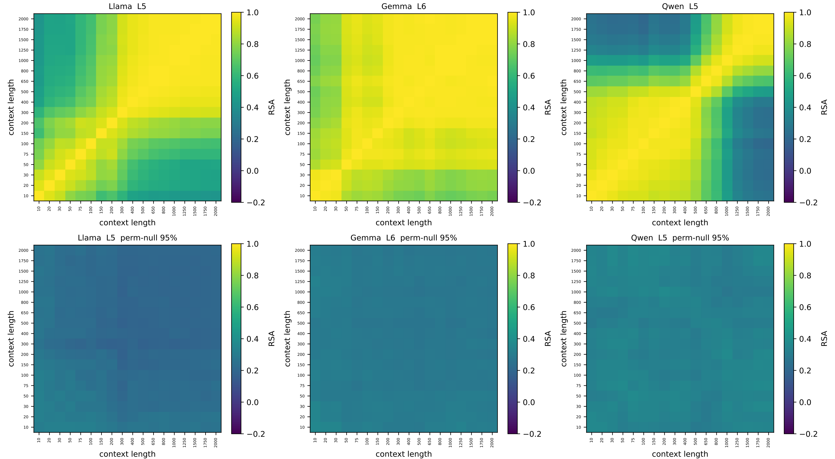
ring [v2] context-vs-context node-geometry RSA — relative depth 0.15 top: observed | bottom: node-label permutation null (95th pct)
