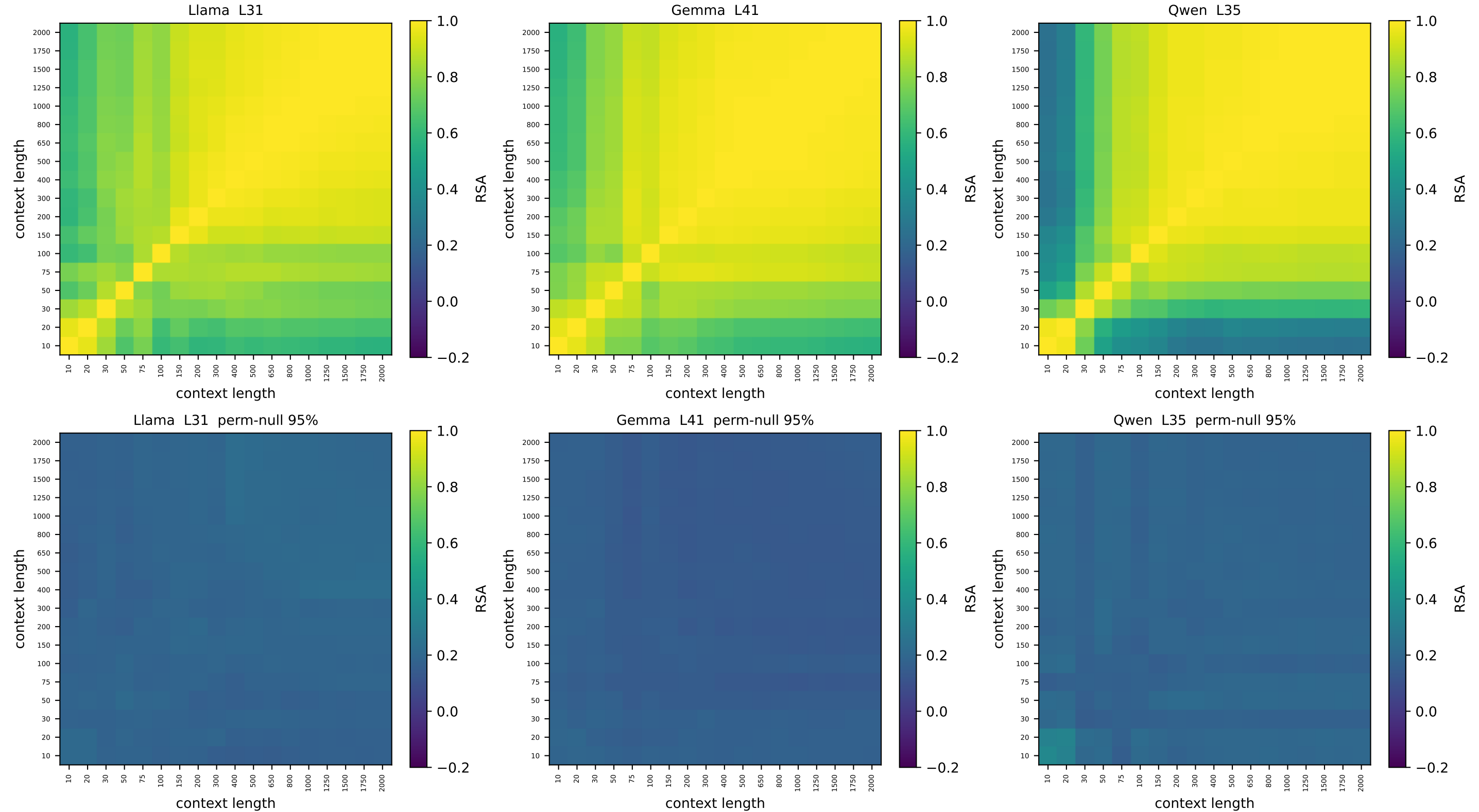
ring [v2] context-vs-context node-geometry RSA — relative depth 1.00 top: observed | bottom: node-label permutation null (95th pct)
