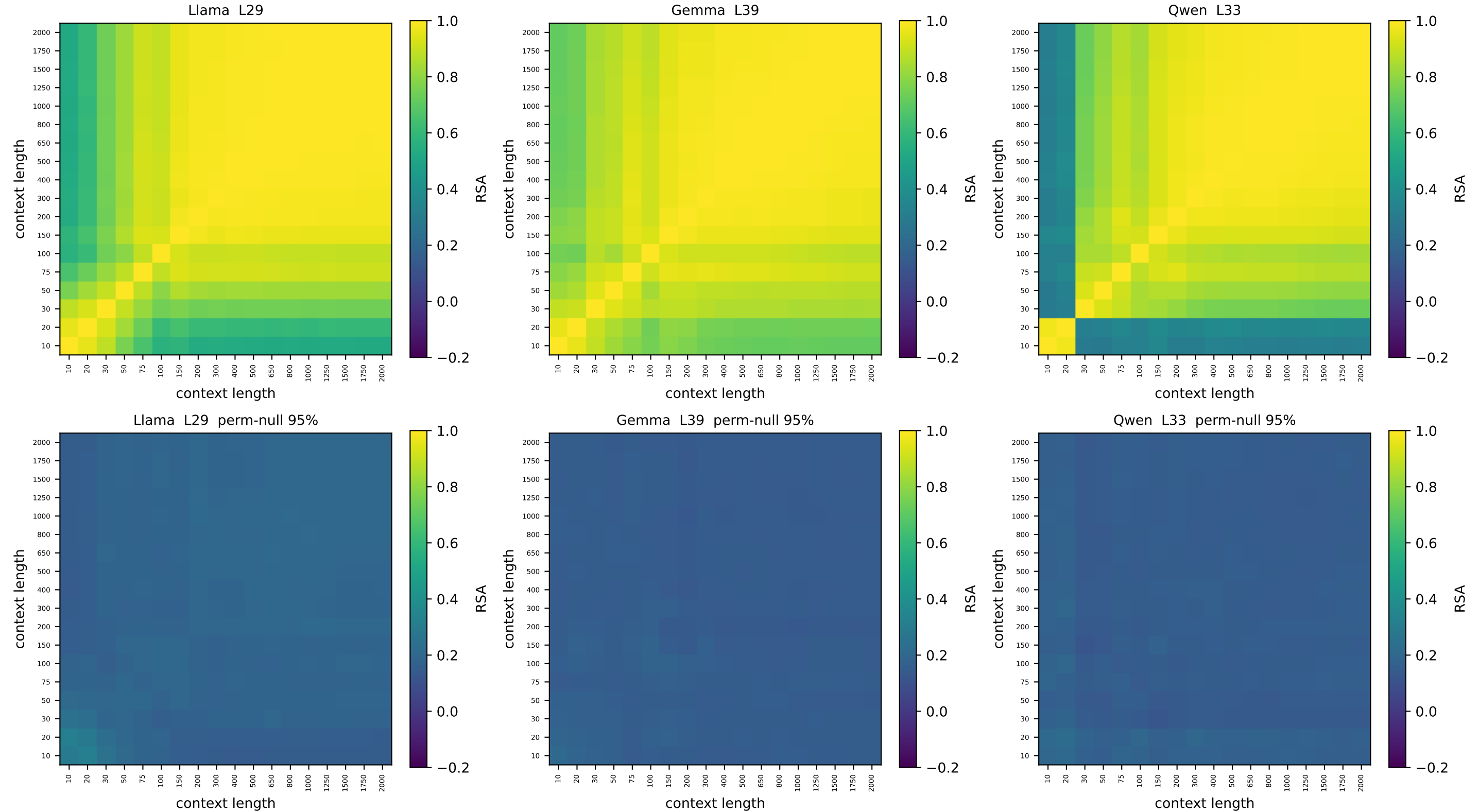
ring [v2] context-vs-context node-geometry RSA — relative depth 0.95 top: observed | bottom: node-label permutation null (95th pct)
