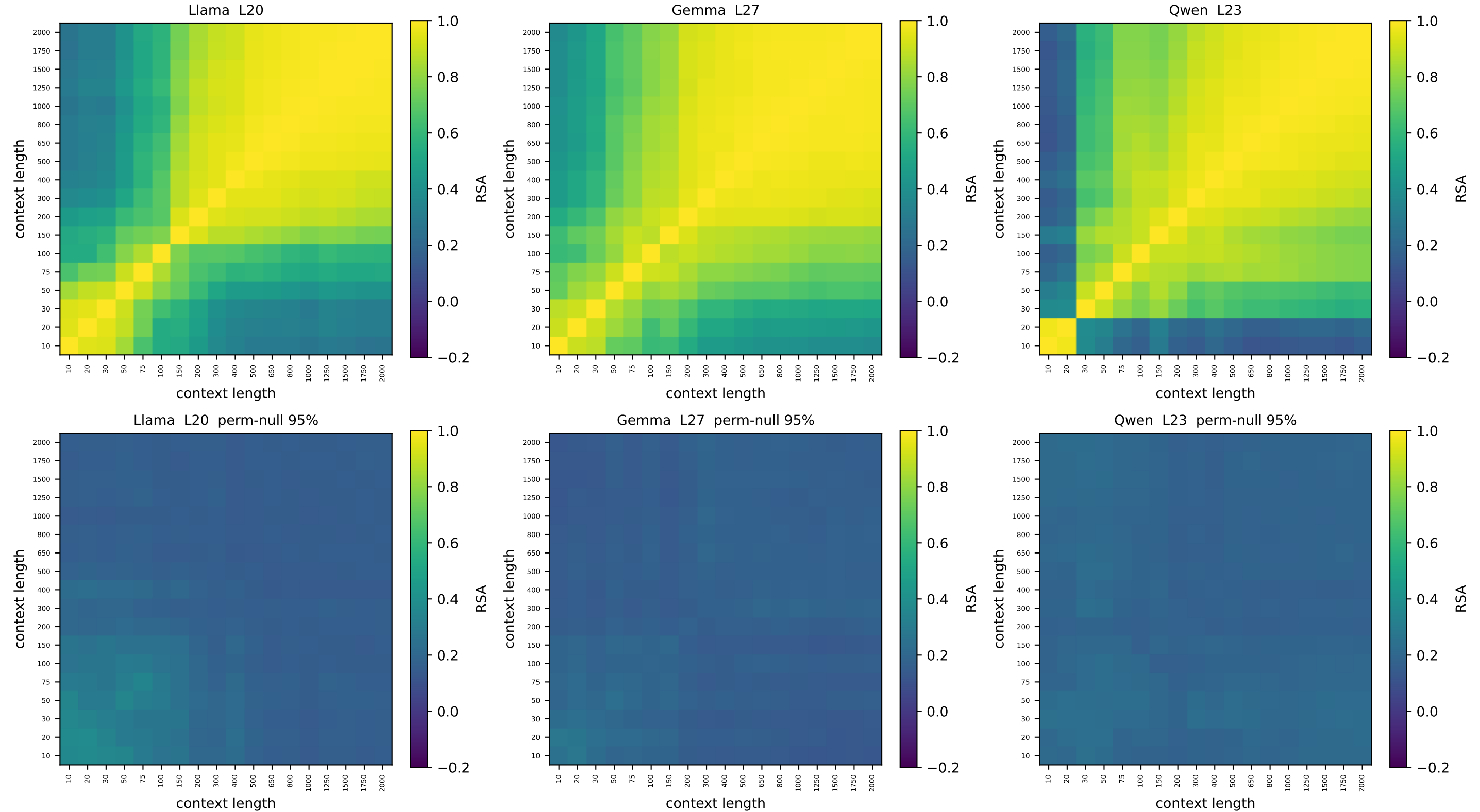
ring [v2] context-vs-context node-geometry RSA — relative depth 0.66 top: observed | bottom: node-label permutation null (95th pct)
