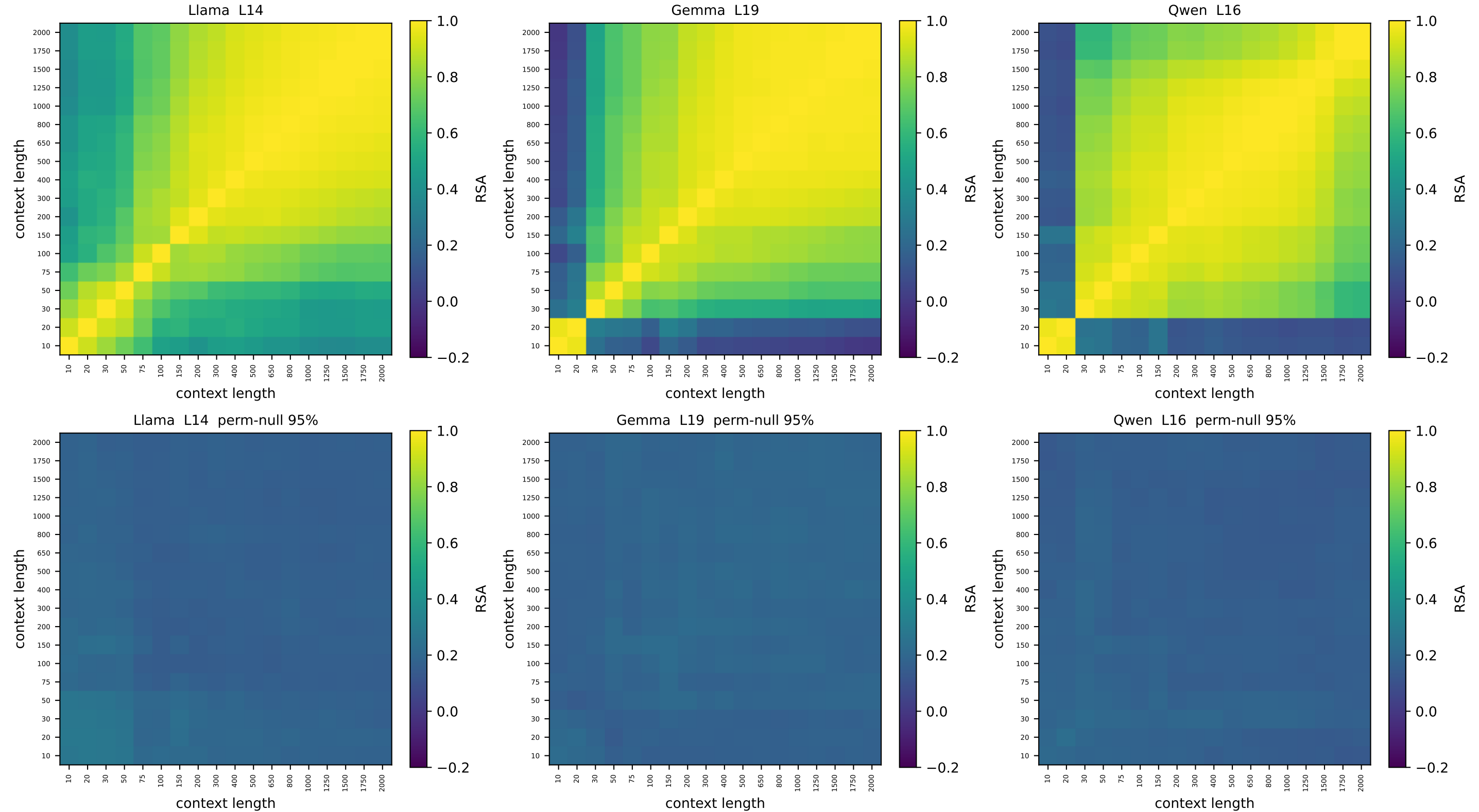
ring [v2] context-vs-context node-geometry RSA — relative depth 0.46 top: observed | bottom: node-label permutation null (95th pct)
