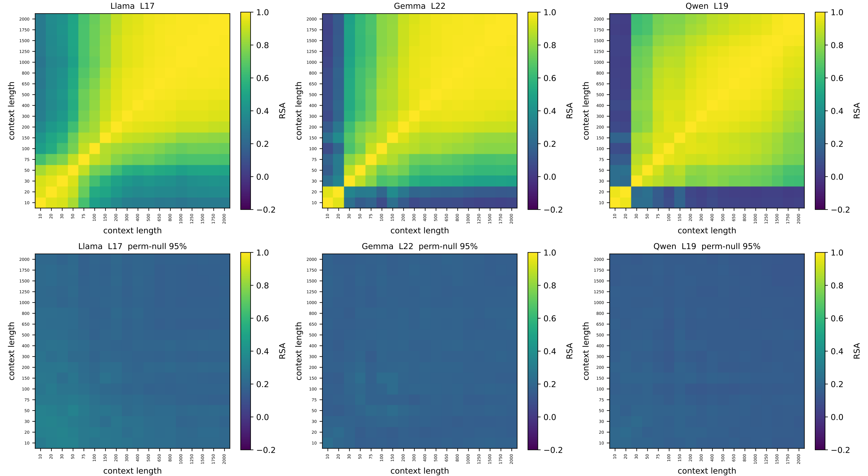
ring [v2] context-vs-context node-geometry RSA — relative depth 0.54 top: observed | bottom: node-label permutation null (95th pct)
