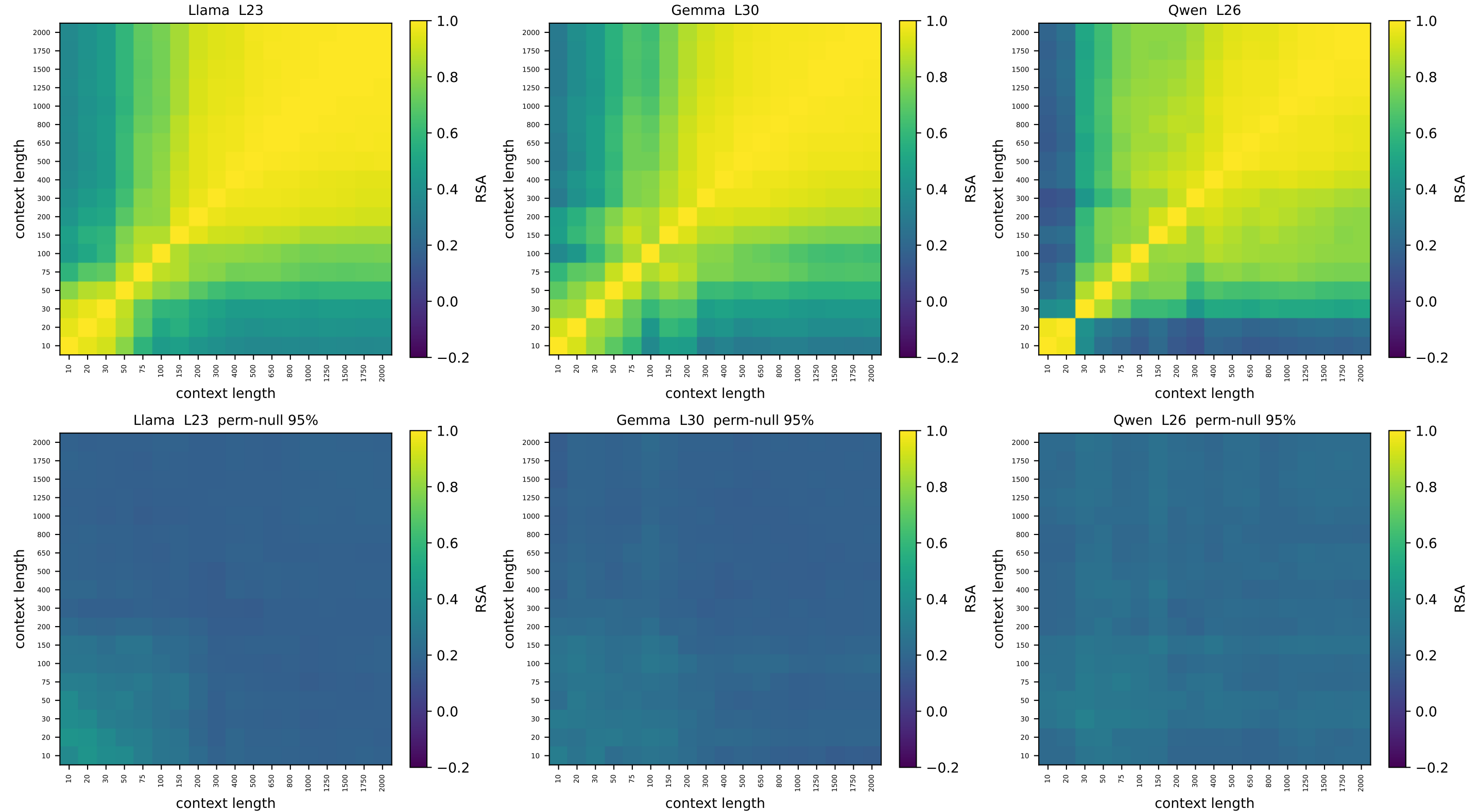
ring [v2] context-vs-context node-geometry RSA — relative depth 0.73 top: observed | bottom: node-label permutation null (95th pct)
