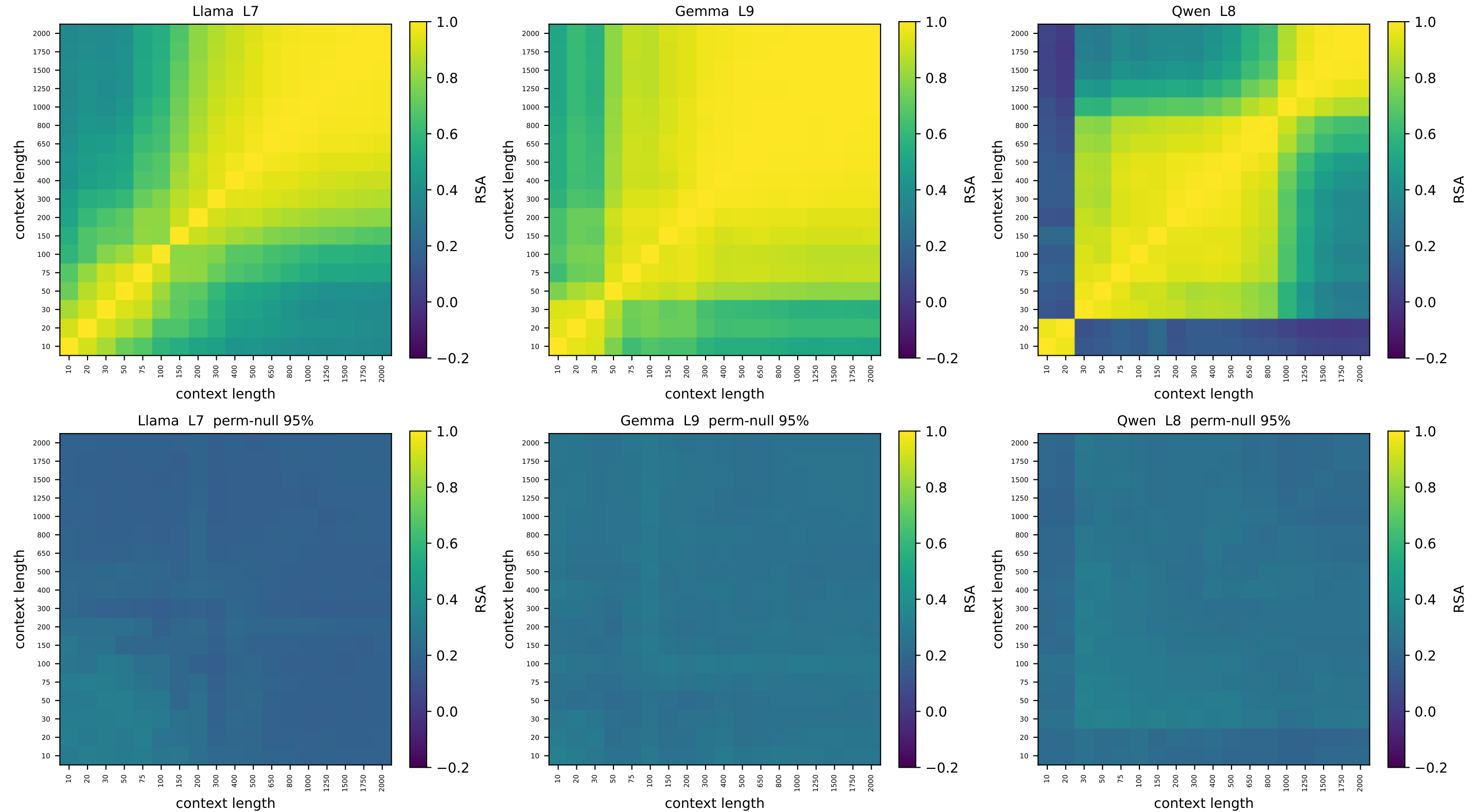
ring [v2] context-vs-context node-geometry RSA — relative depth 0.22 top: observed | bottom: node-label permutation null (95th pct)
