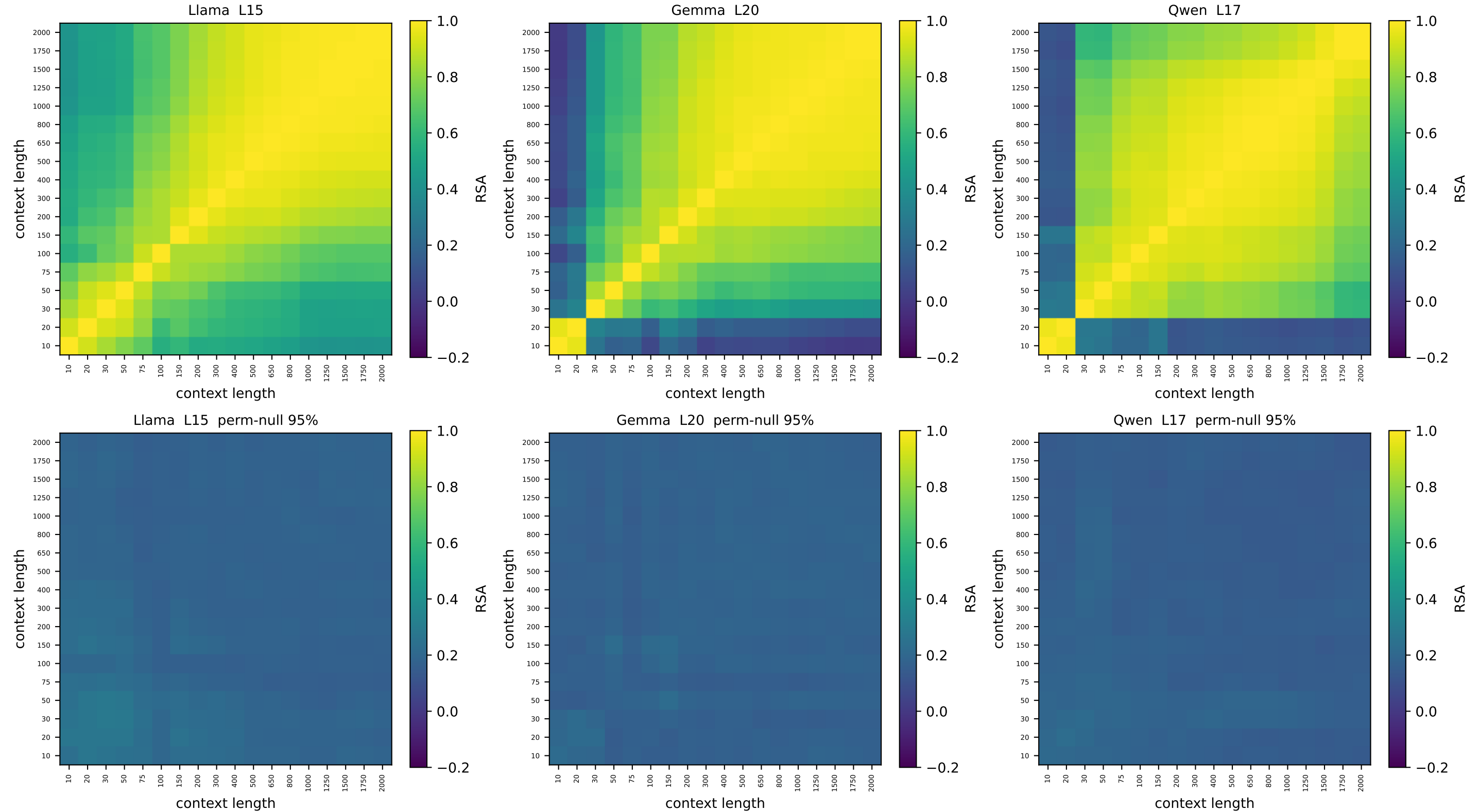
ring [v2] context-vs-context node-geometry RSA — relative depth 0.49 top: observed | bottom: node-label permutation null (95th pct)
