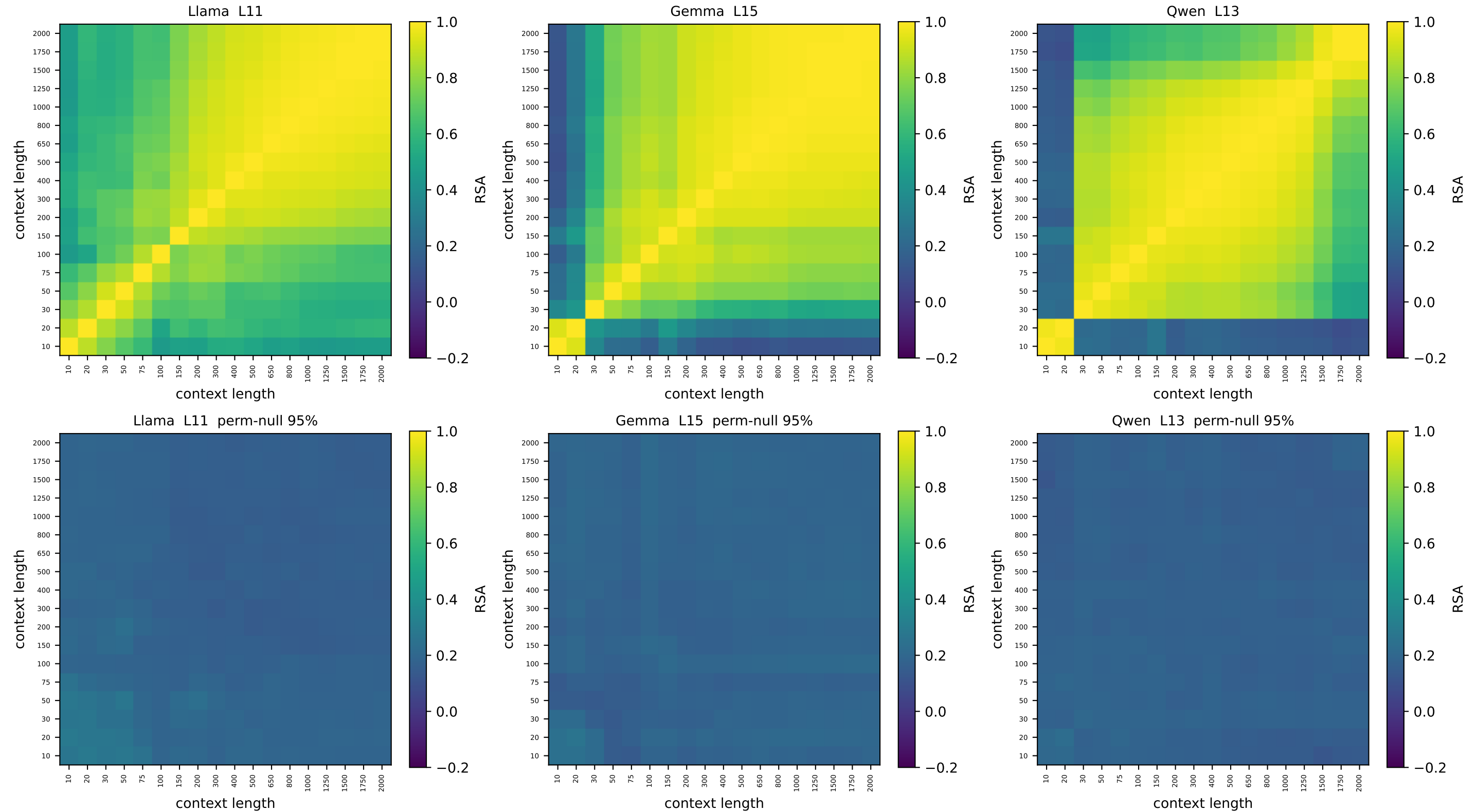
ring [v2] context-vs-context node-geometry RSA — relative depth 0.37 top: observed | bottom: node-label permutation null (95th pct)
