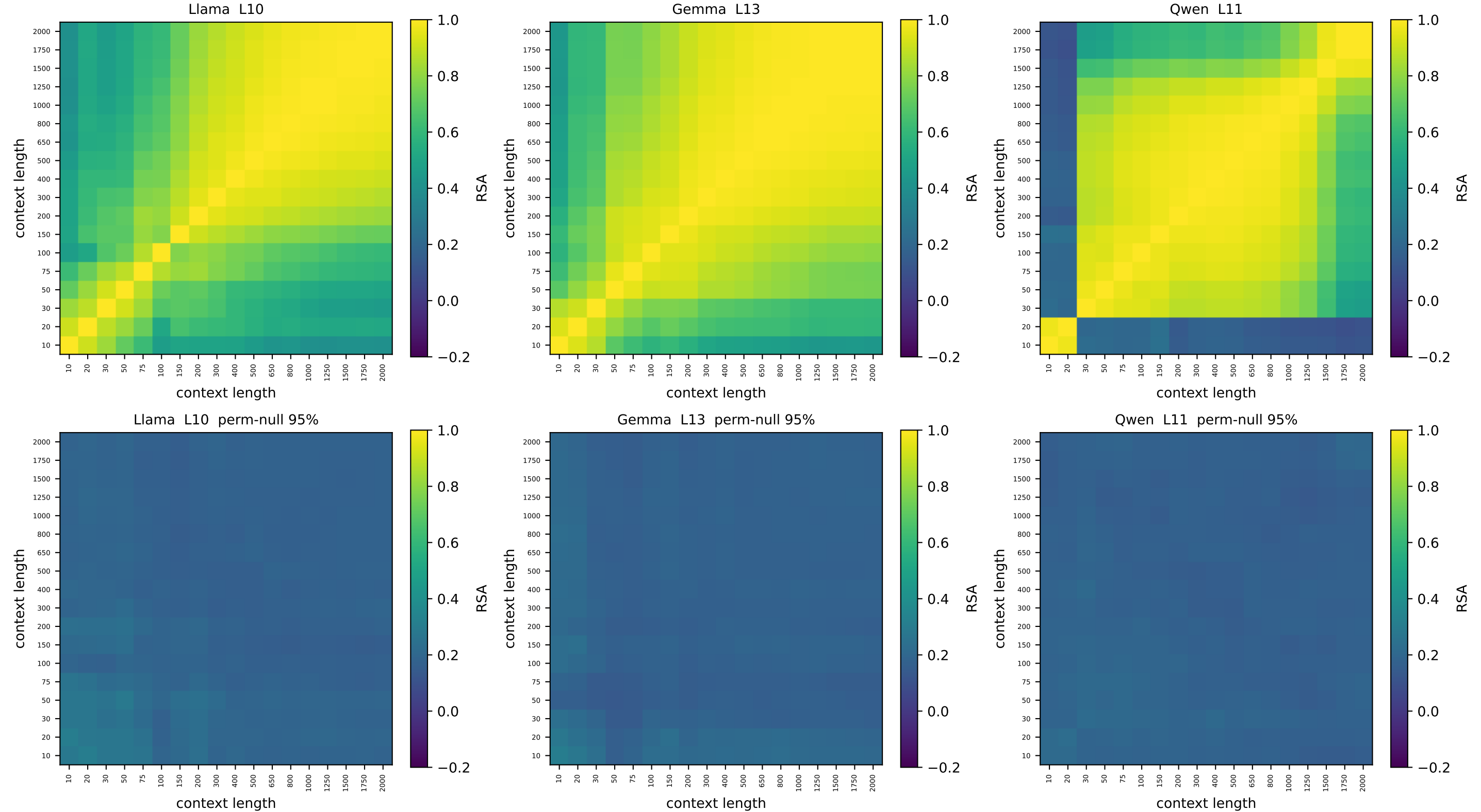
ring [v2] context-vs-context node-geometry RSA — relative depth 0.32 top: observed | bottom: node-label permutation null (95th pct)
