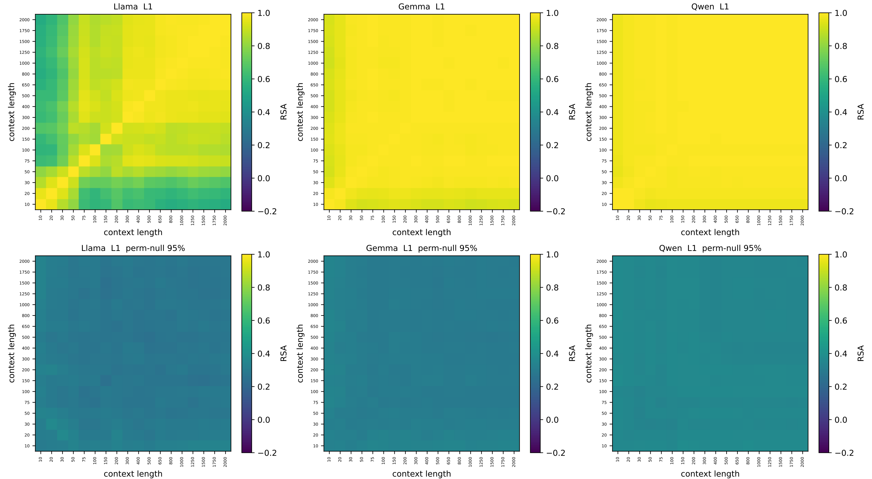
ring [v2] context-vs-context node-geometry RSA — relative depth 0.02 top: observed | bottom: node-label permutation null (95th pct)
