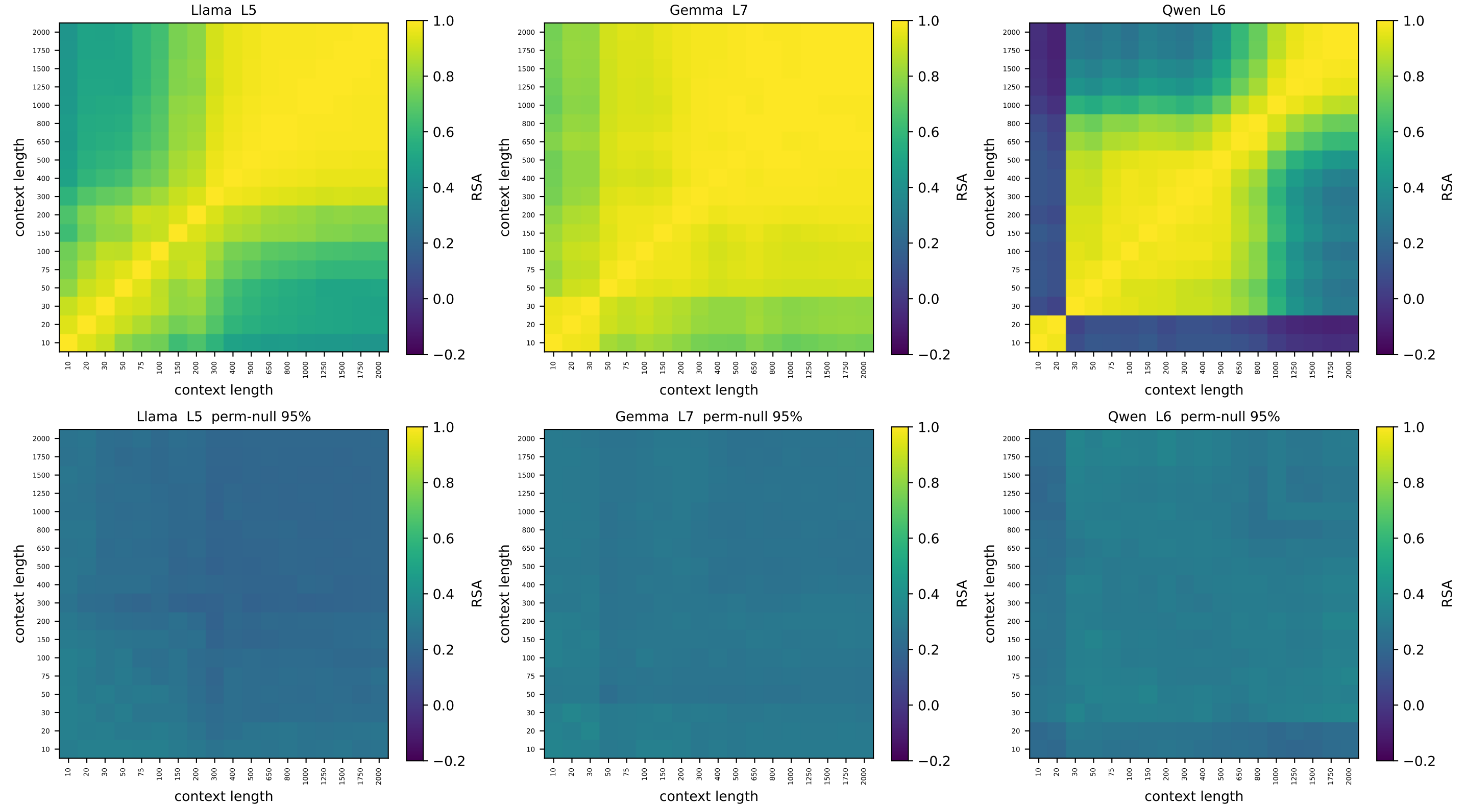
ring [v2] context-vs-context node-geometry RSA — relative depth 0.17 top: observed | bottom: node-label permutation null (95th pct)
