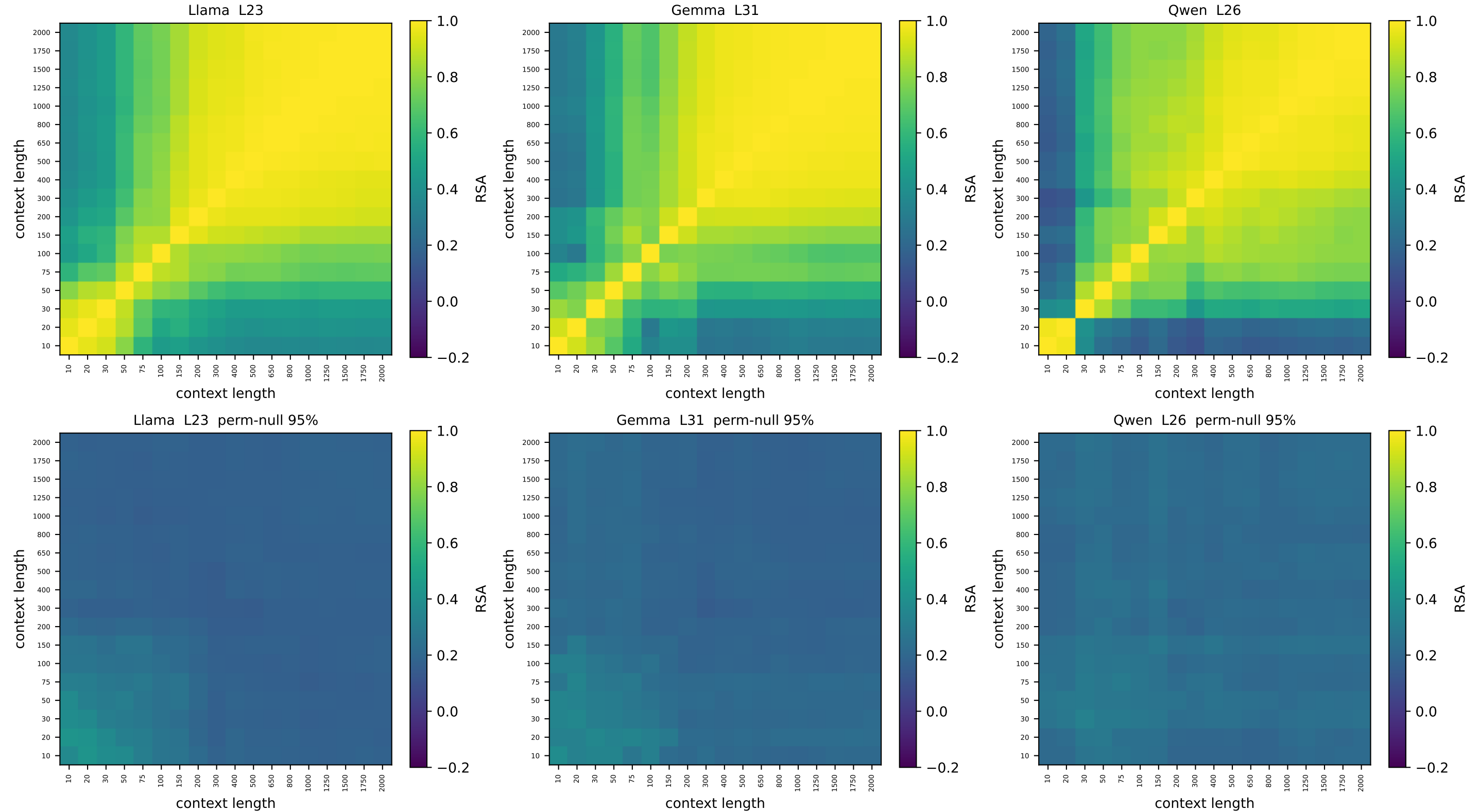
ring [v2] context-vs-context node-geometry RSA — relative depth 0.76 top: observed | bottom: node-label permutation null (95th pct)
