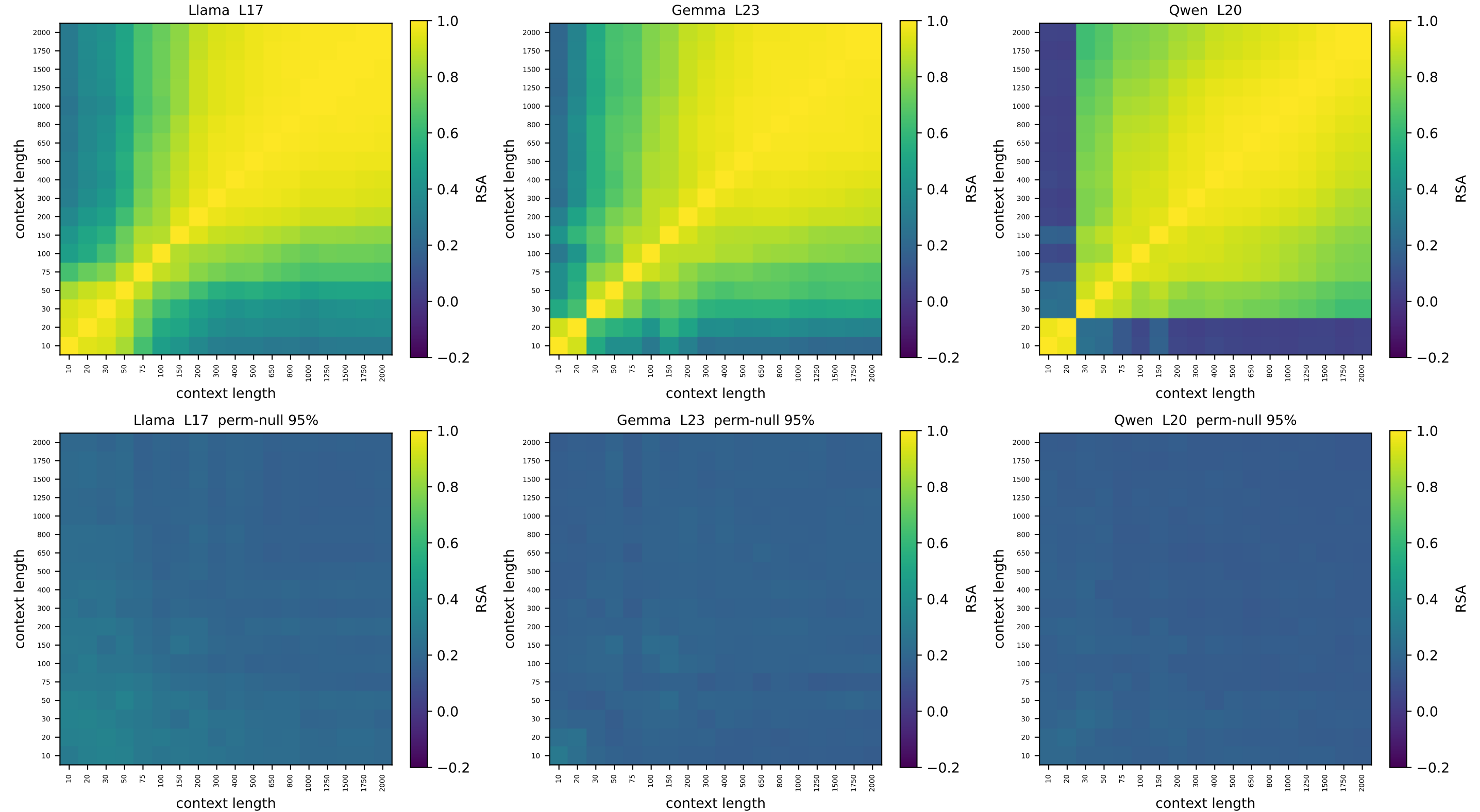
ring [v2] context-vs-context node-geometry RSA — relative depth 0.56 top: observed | bottom: node-label permutation null (95th pct)
