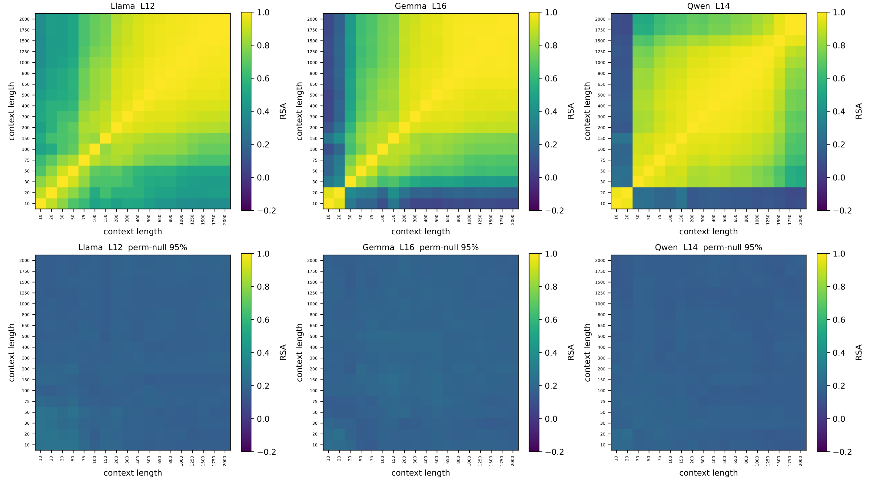
ring [v2] context-vs-context node-geometry RSA — relative depth 0.39 top: observed | bottom: node-label permutation null (95th pct)
