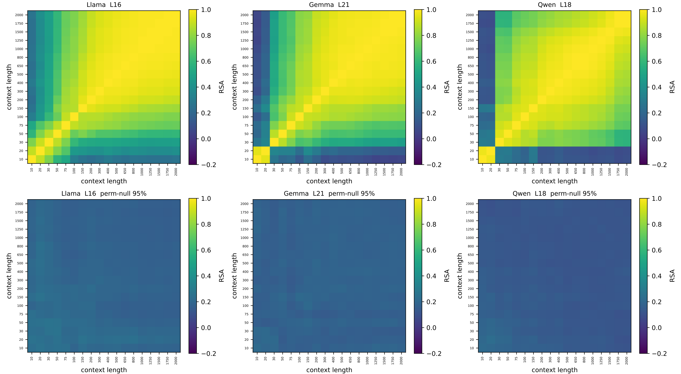
ring [v2] context-vs-context node-geometry RSA — relative depth 0.51 top: observed | bottom: node-label permutation null (95th pct)
