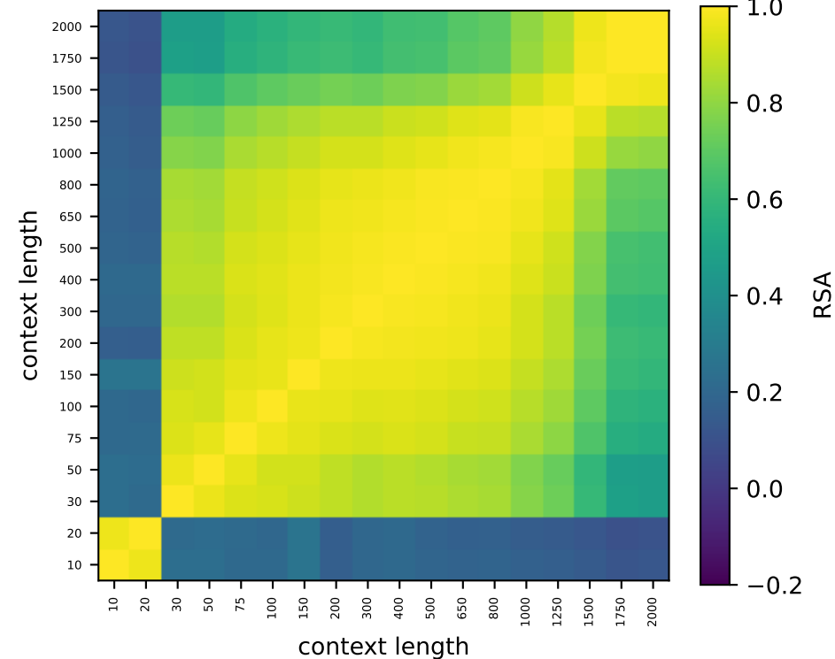
Qwen L12 perm-null 95%
