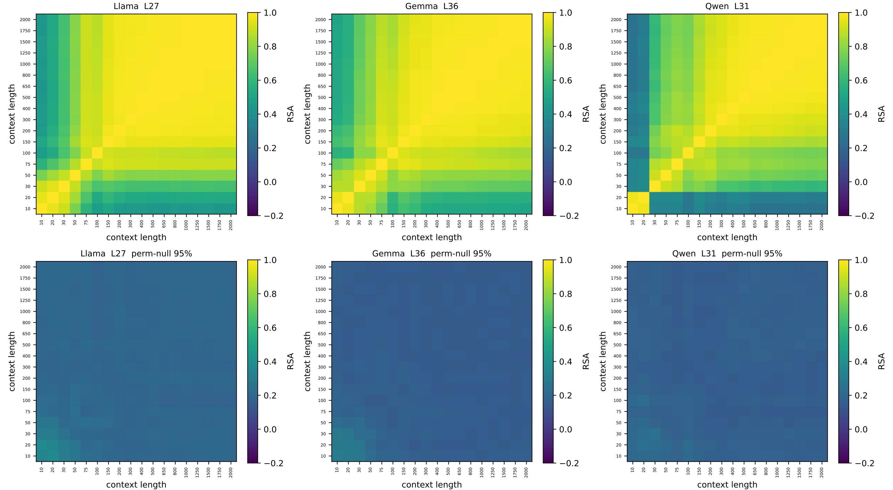
ring [v2] context-vs-context node-geometry RSA — relative depth 0.88 top: observed | bottom: node-label permutation null (95th pct)
