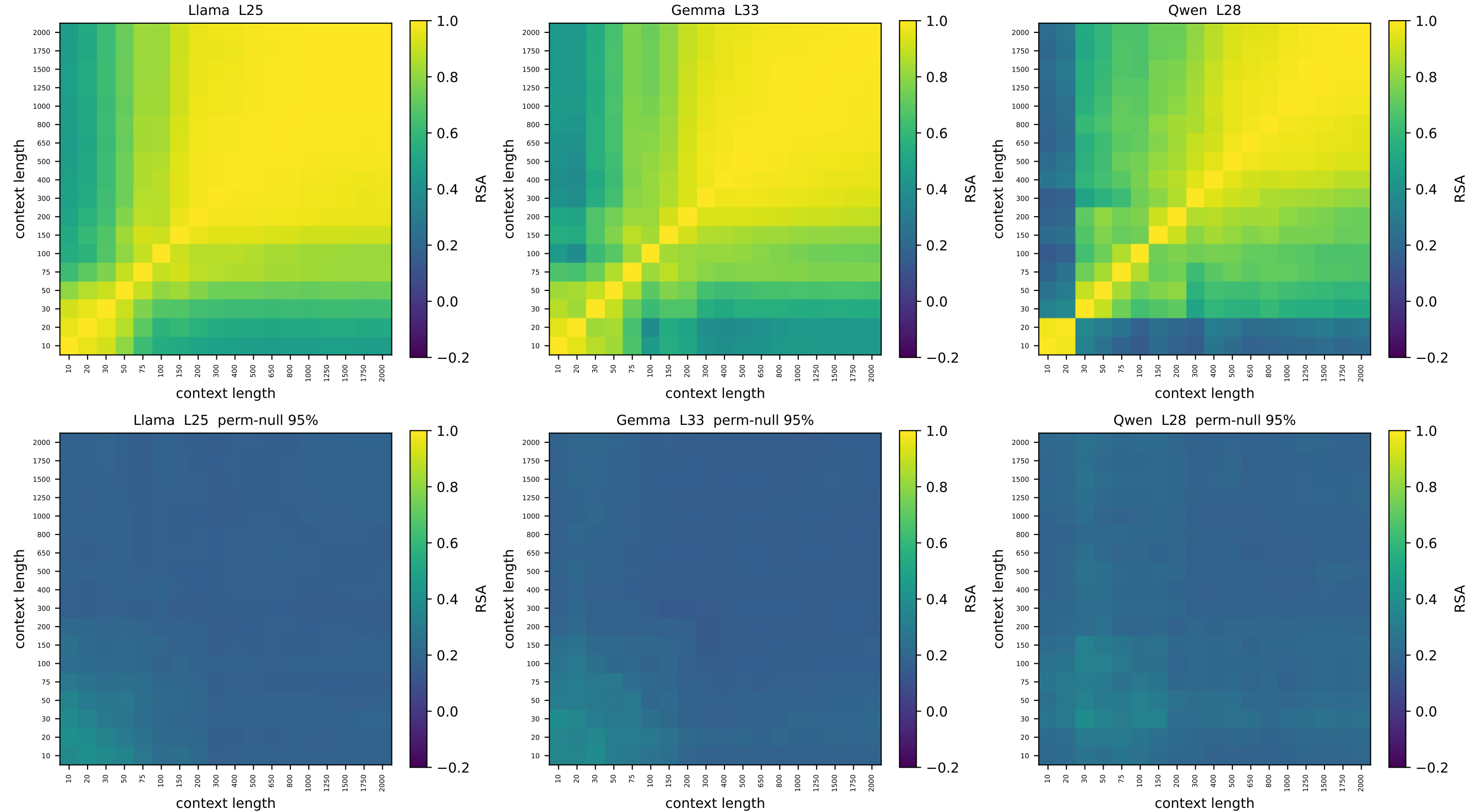
ring [v2] context-vs-context node-geometry RSA — relative depth 0.80 top: observed | bottom: node-label permutation null (95th pct)
