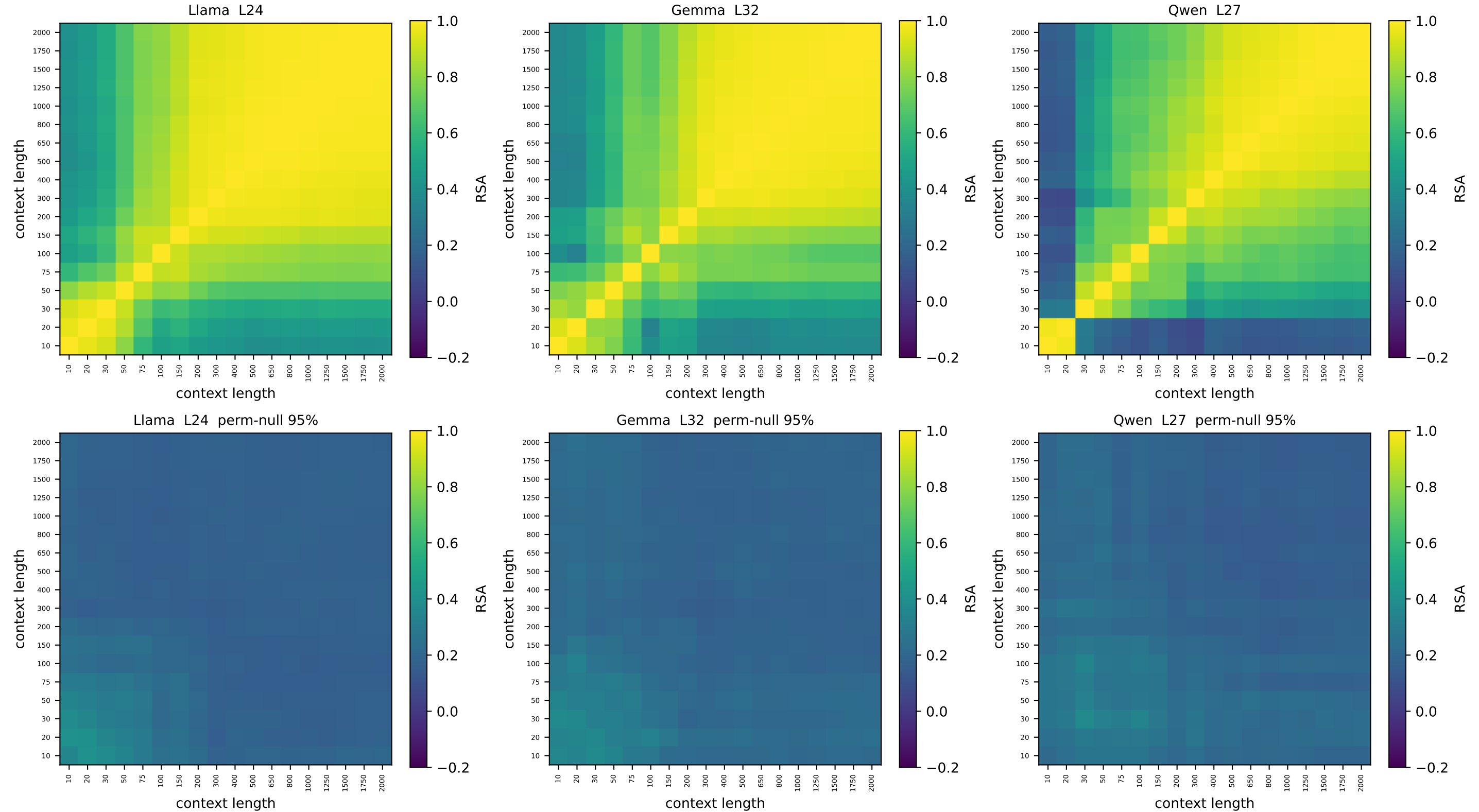
ring [v2] context-vs-context node-geometry RSA — relative depth 0.78 top: observed | bottom: node-label permutation null (95th pct)
