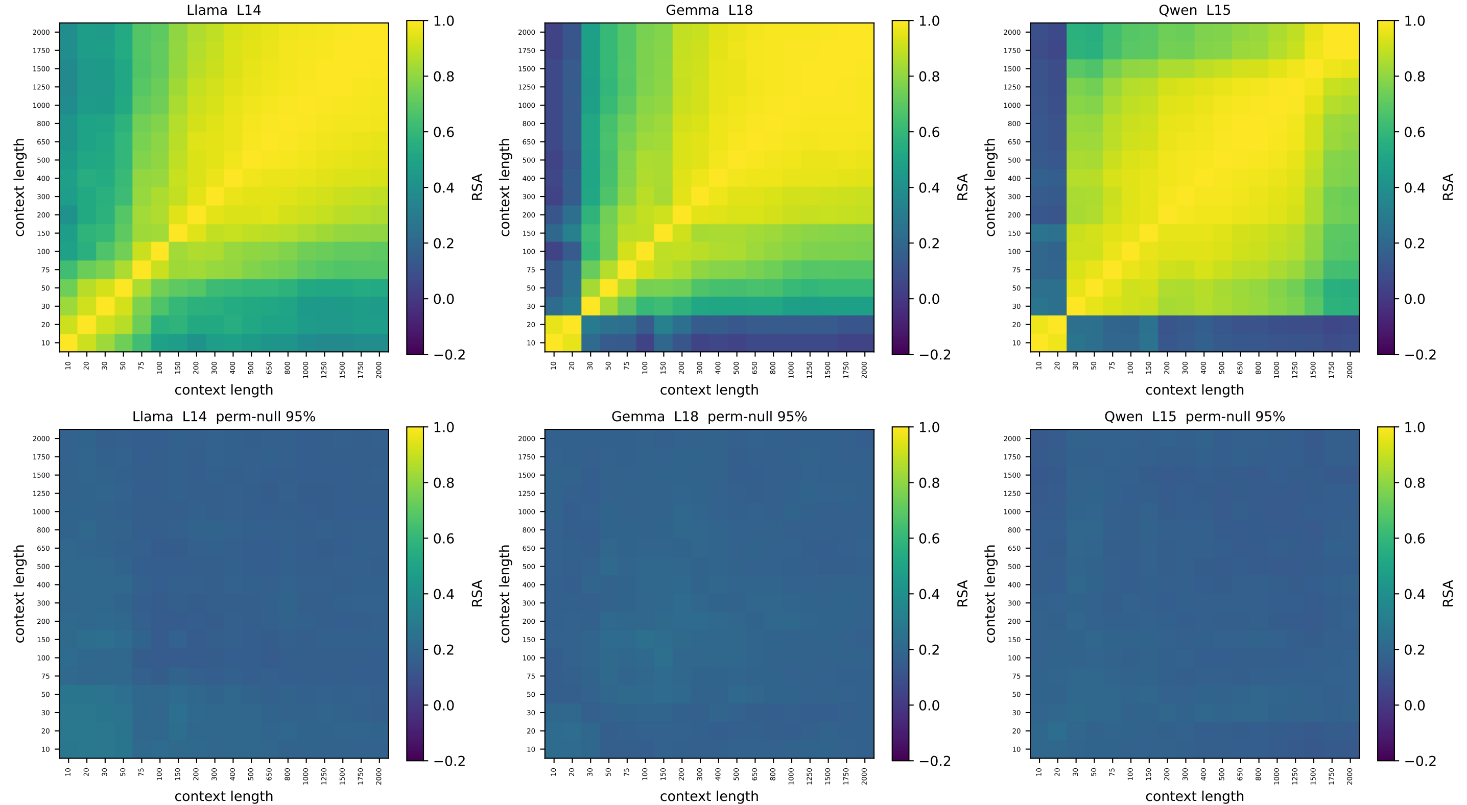
ring [v2] context-vs-context node-geometry RSA — relative depth 0.44 top: observed | bottom: node-label permutation null (95th pct)
