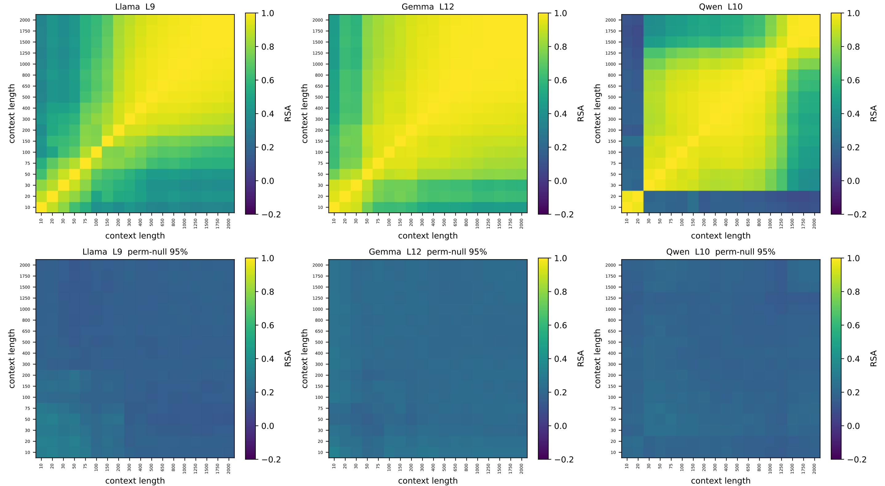
ring [v2] context-vs-context node-geometry RSA — relative depth 0.29 top: observed | bottom: node-label permutation null (95th pct)
