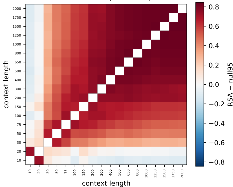
Gemma L17 (86% > null)
