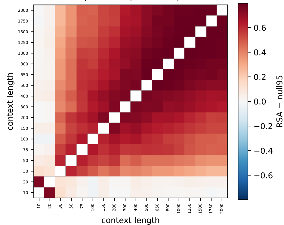
Qwen L24 (97% > null)
