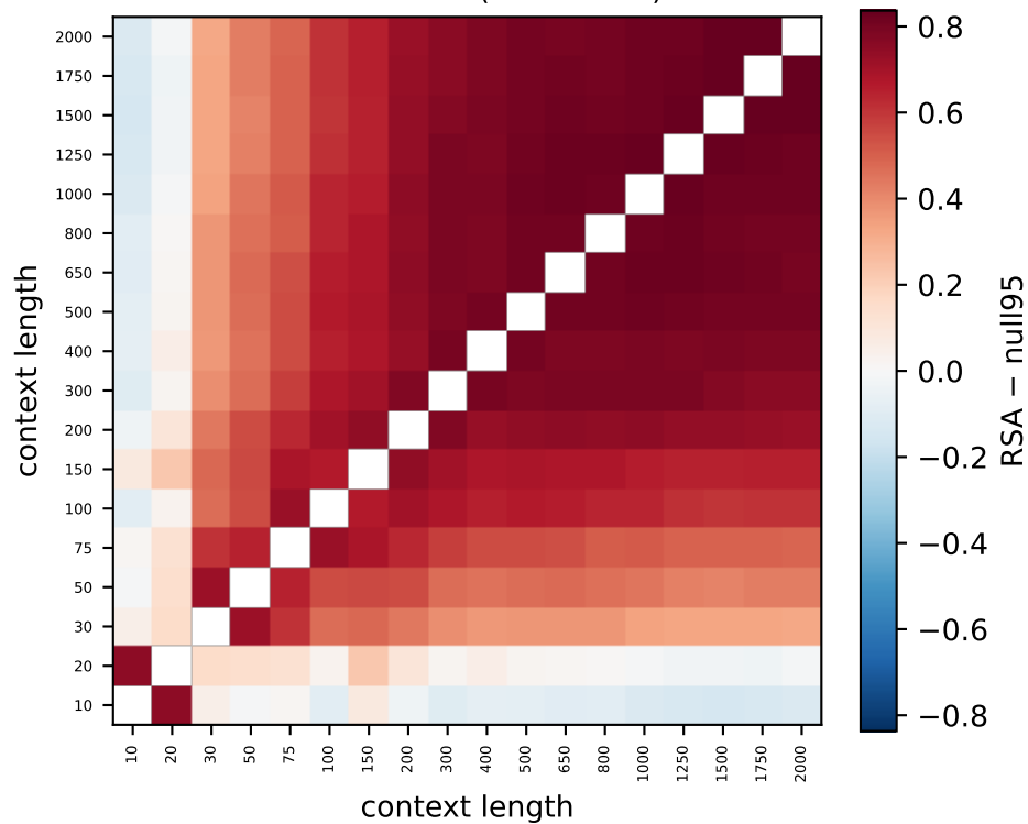
Gemma L22 (88% > null)
