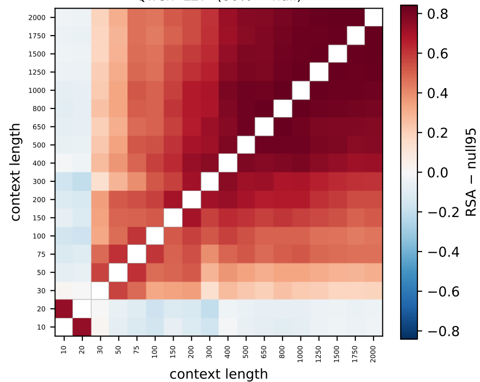
Qwen L27 (80% > null)
