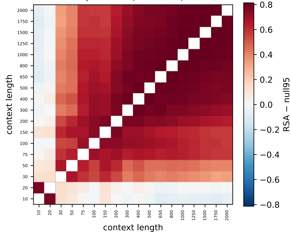
Qwen L23 (88% > null)
