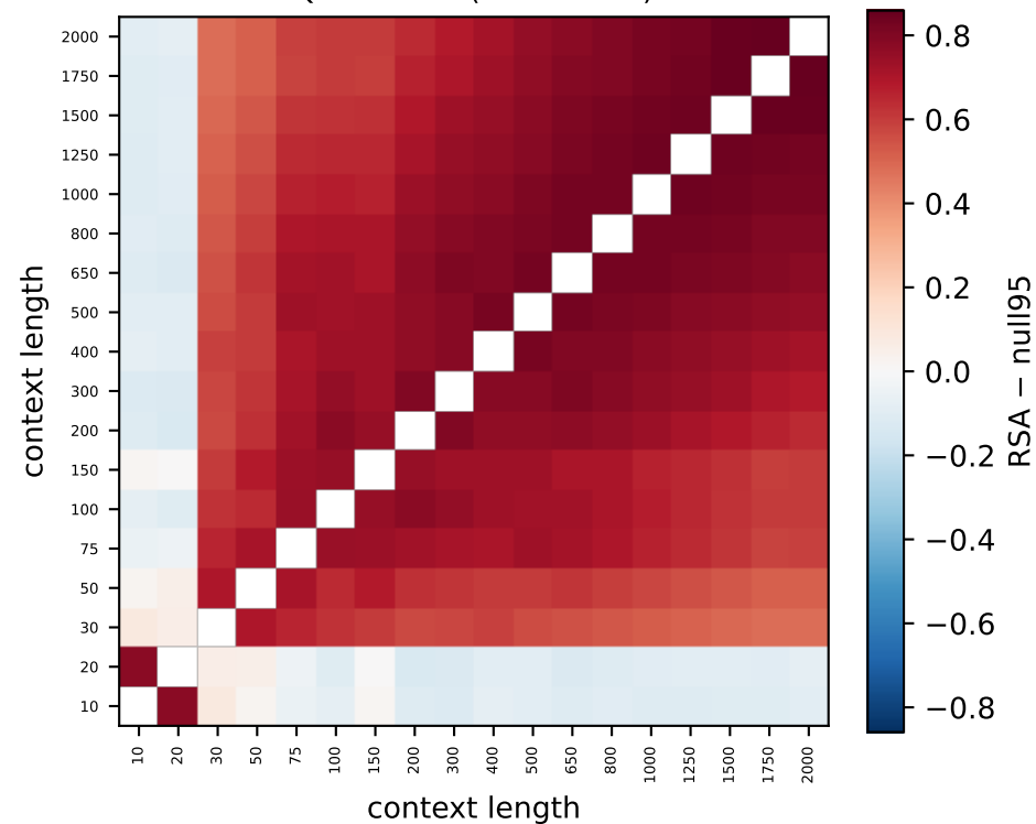
Qwen L21 (83% > null)
