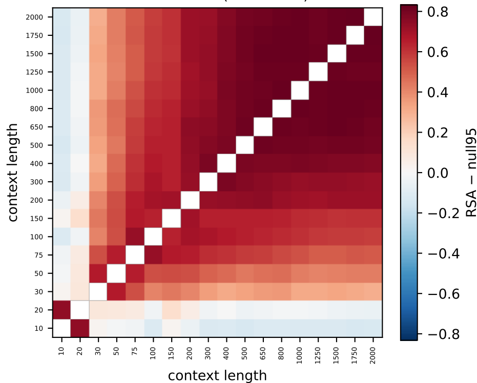
Gemma L18 (84% > null)
