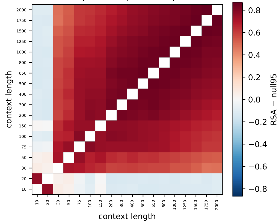
Qwen L20 (82% > null)
