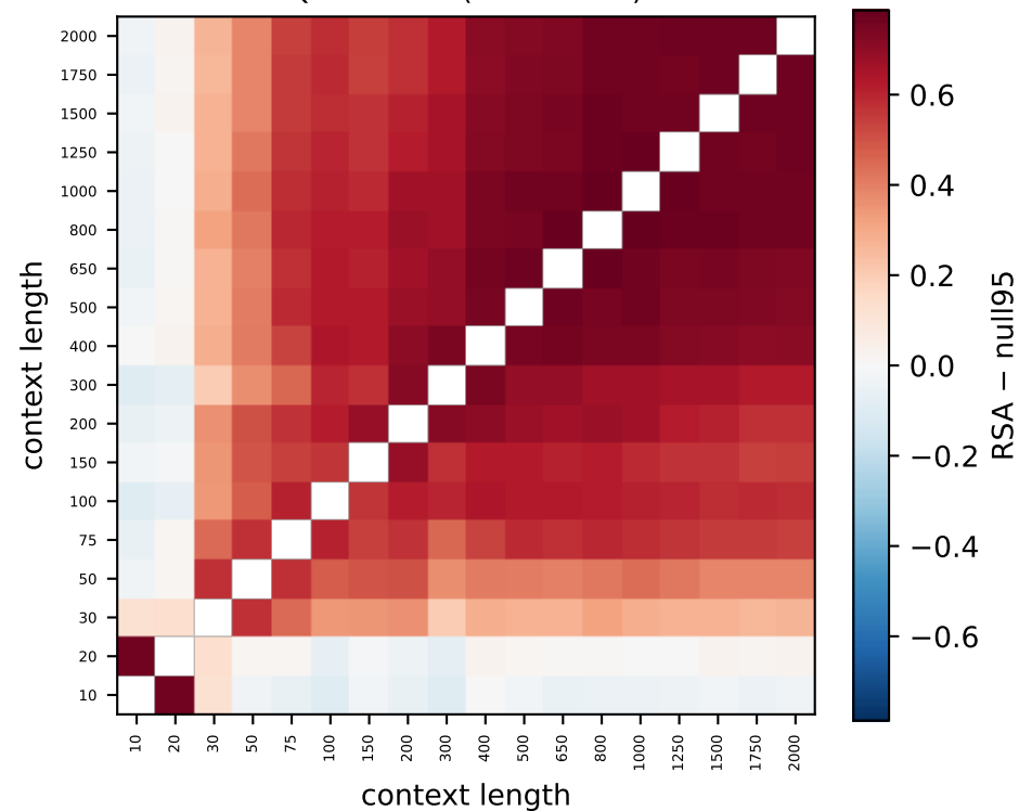
Qwen L26 (87% > null)
