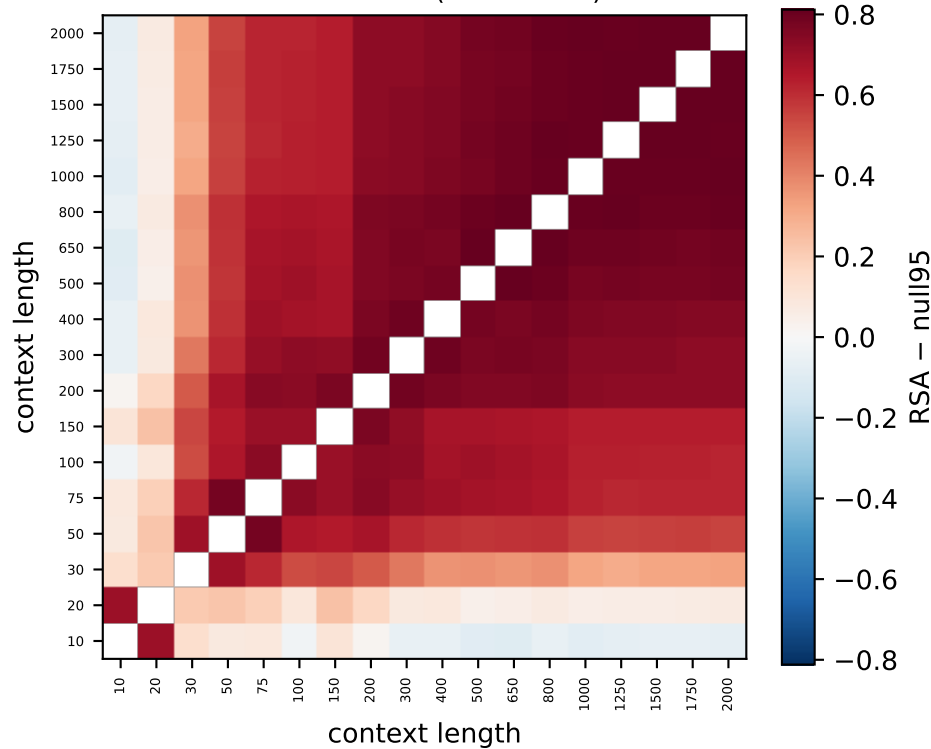
Gemma L15 (93% > null)
