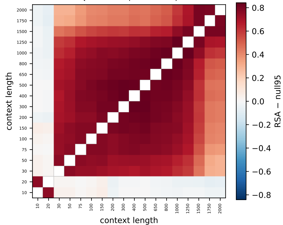
Qwen L11 (87% > null)
