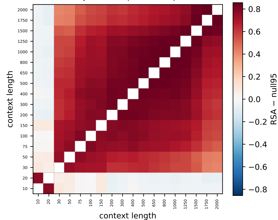
Qwen L16 (86% > null)
