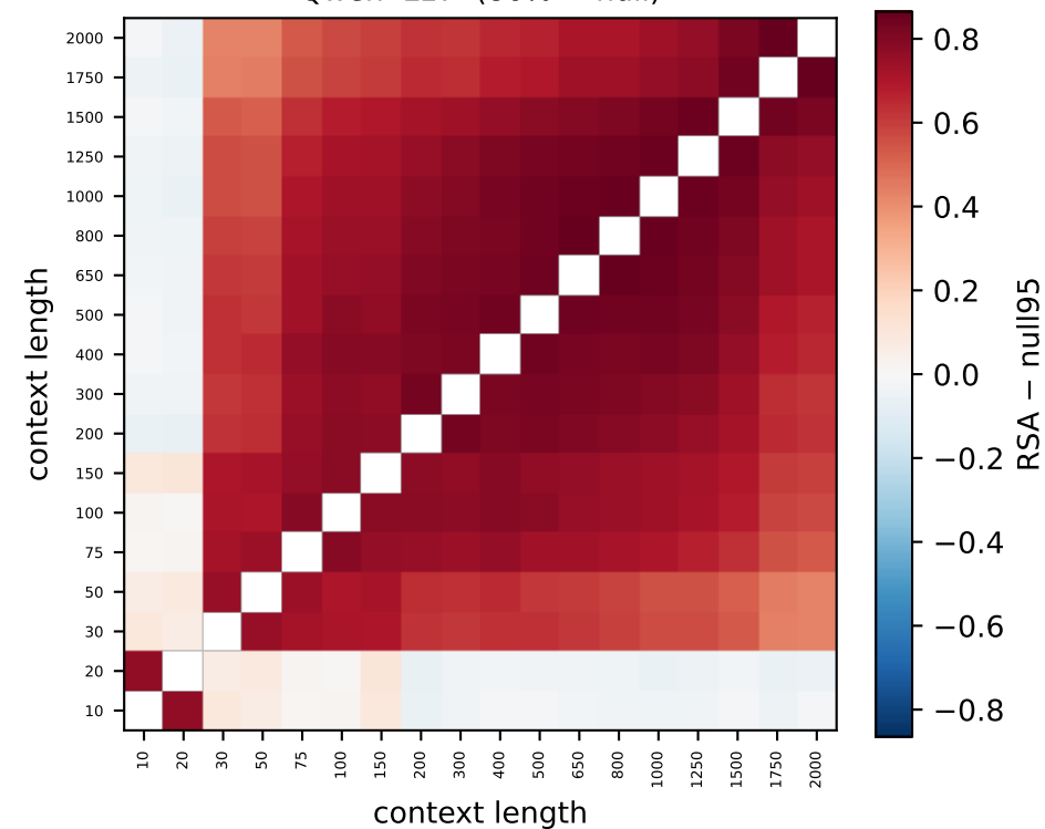
Qwen L17 (86% > null)
