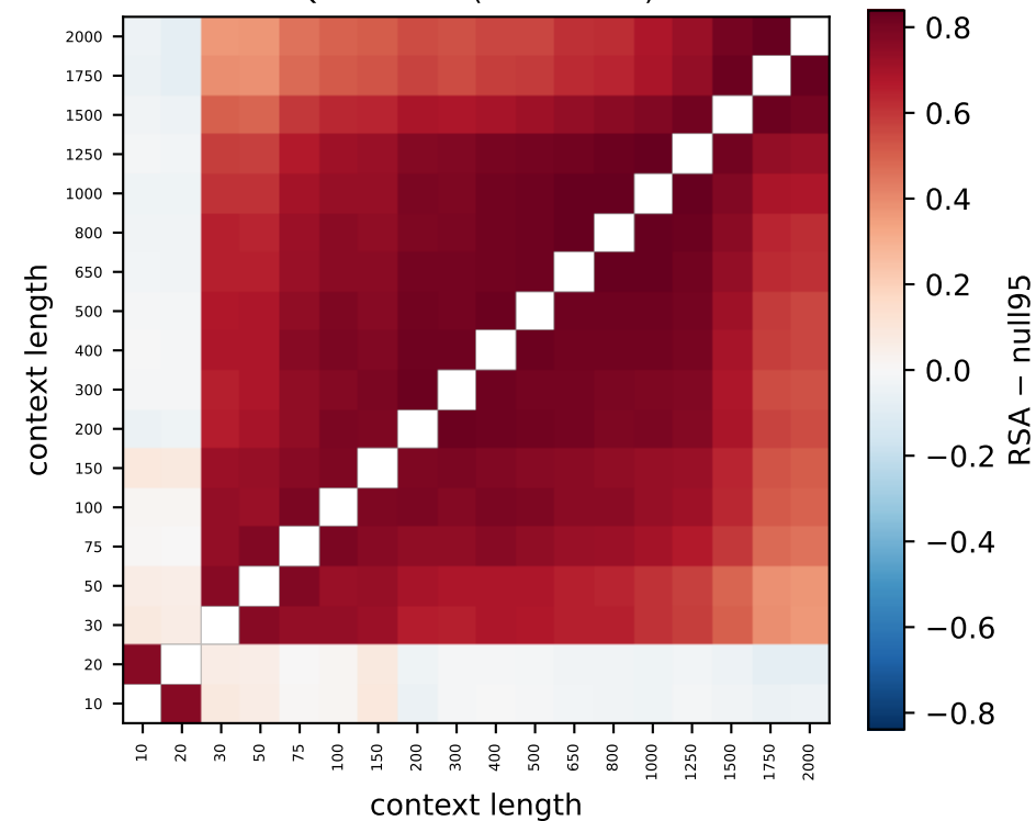
Qwen L14 (86% > null)
