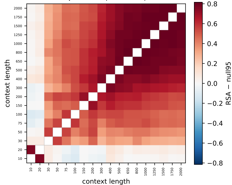
Qwen L28 (93% > null)
