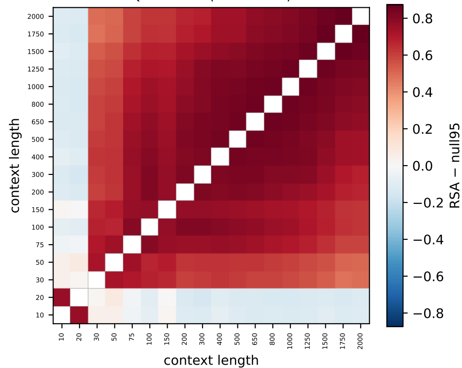
Qwen L19 (82% > null)
