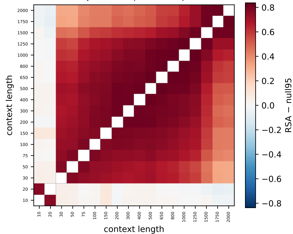
Qwen L13 (93% > null)
