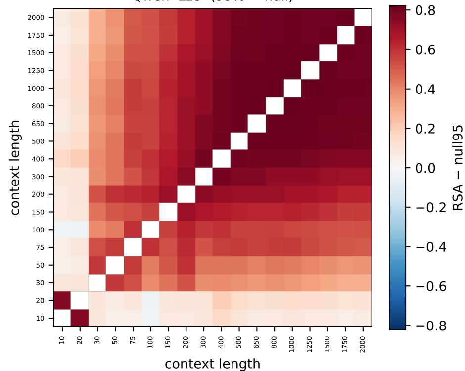
Qwen L29 (99% > null)
