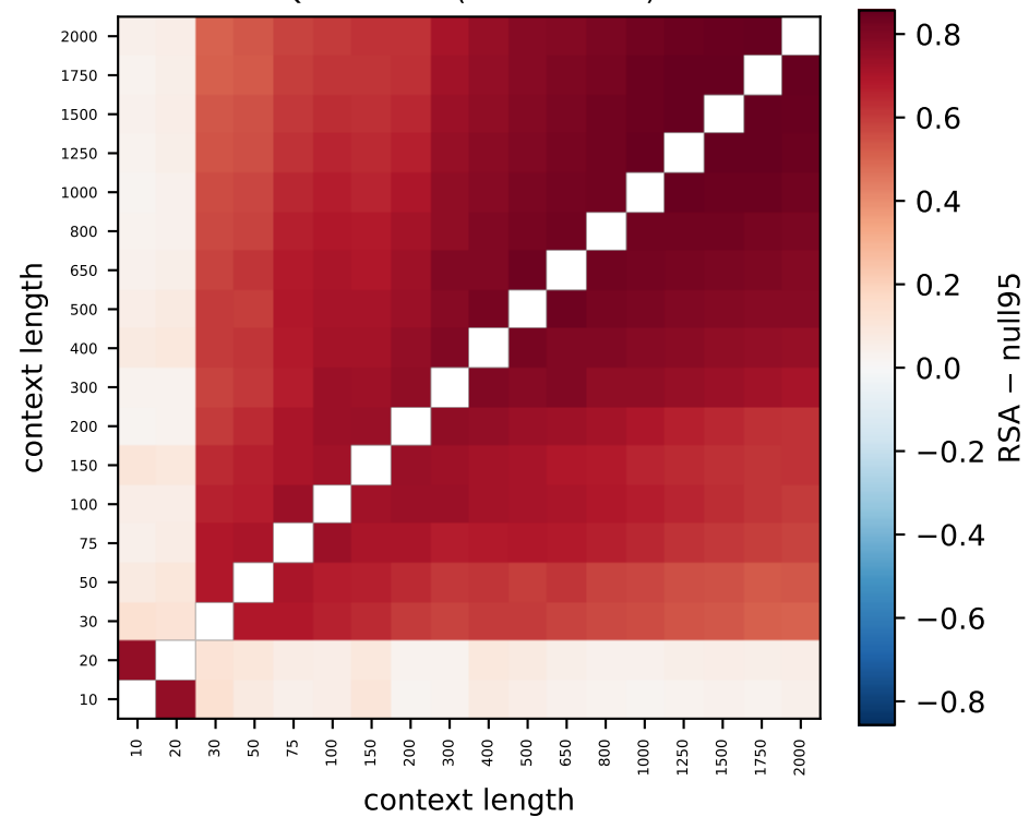
Qwen L22 (100% > null)
