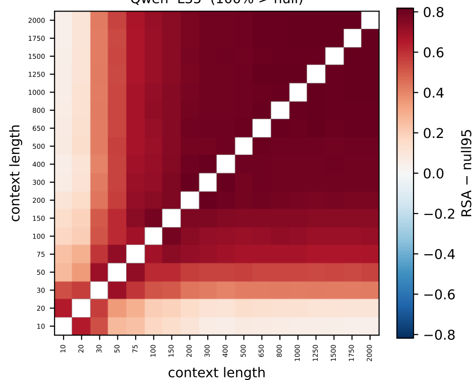
Qwen L35 (100% > null)
