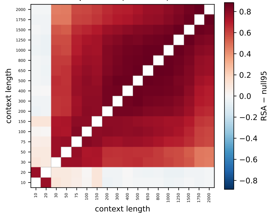
Qwen L18 (86% > null)
