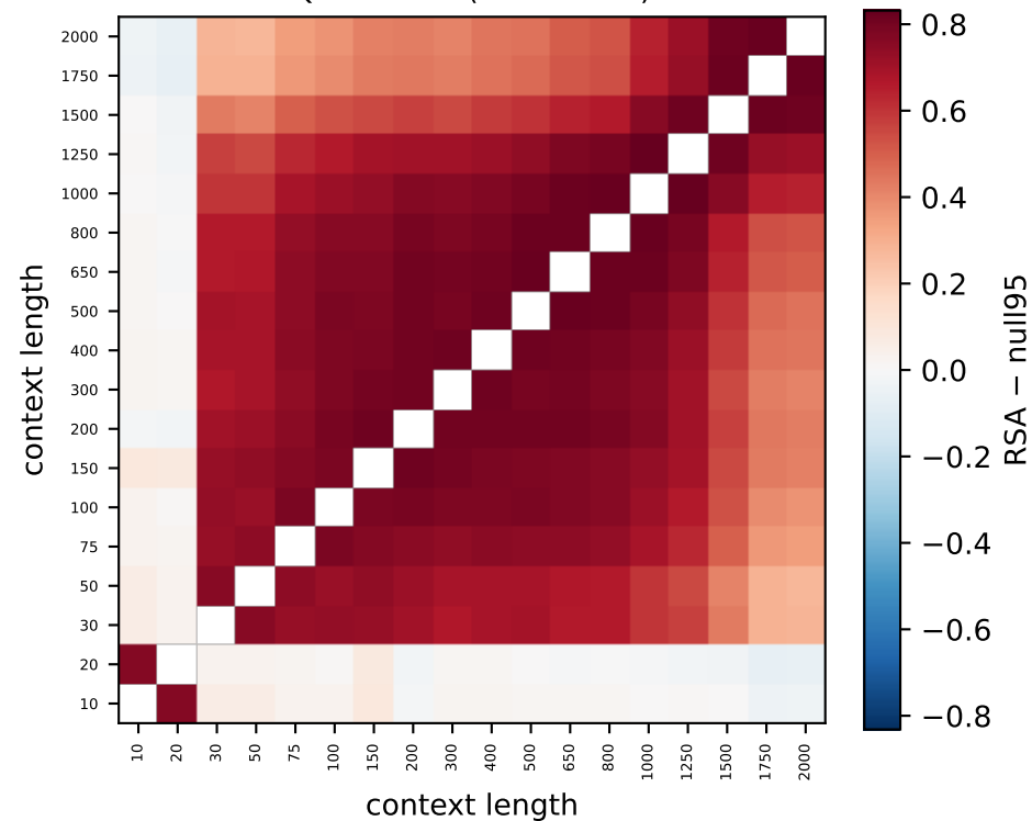
Qwen L12 (93% > null)
