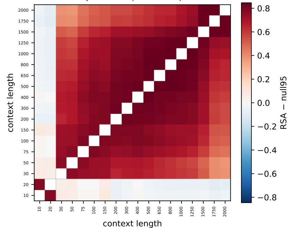
Qwen L15 (87% > null)
