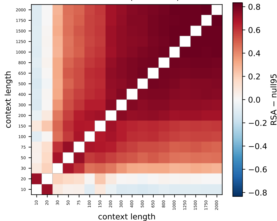
Gemma L16 (92% > null)
