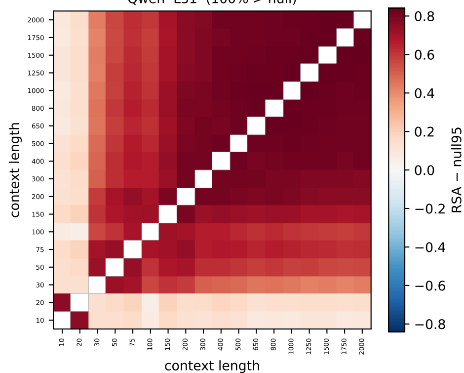
Qwen L31 (100% > null)
